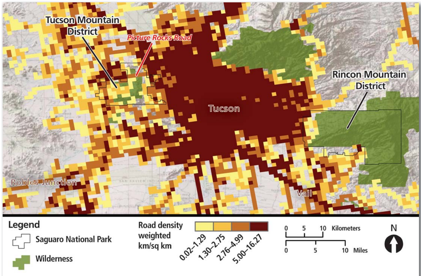
Figure 4. Weighted road density in the local area surrounding Saguaro National Park. Higher road densities are often associated with higher traffic volumes and larger areas of road clearings.
