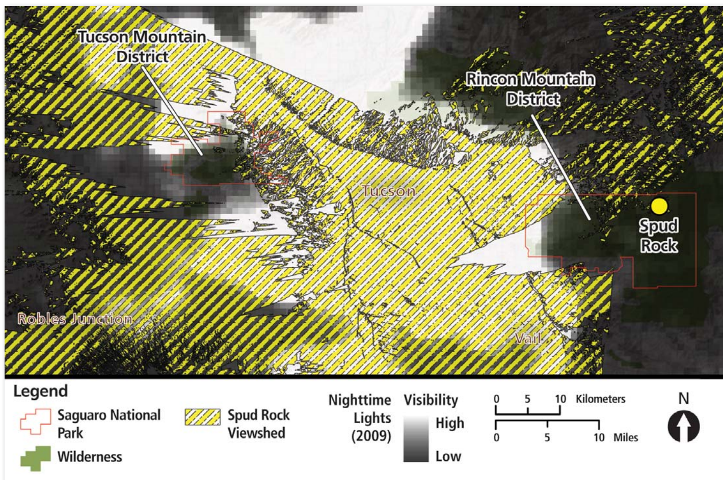
Figure 5. Viewshed from Spud Rock in the Saguaro Wilderness of Rincon Mountain District, considered in relation to nighttime light pollution (year 2009). Lighter areas (white and light gray) have more light pollution than dark areas (dark gray and black). Yellow hatching identifies all areas visible from Spud Rock; some of these areas are more challenged by nighttime lights than others. Saguaro is able to use maps such as this in wilderness planning.
