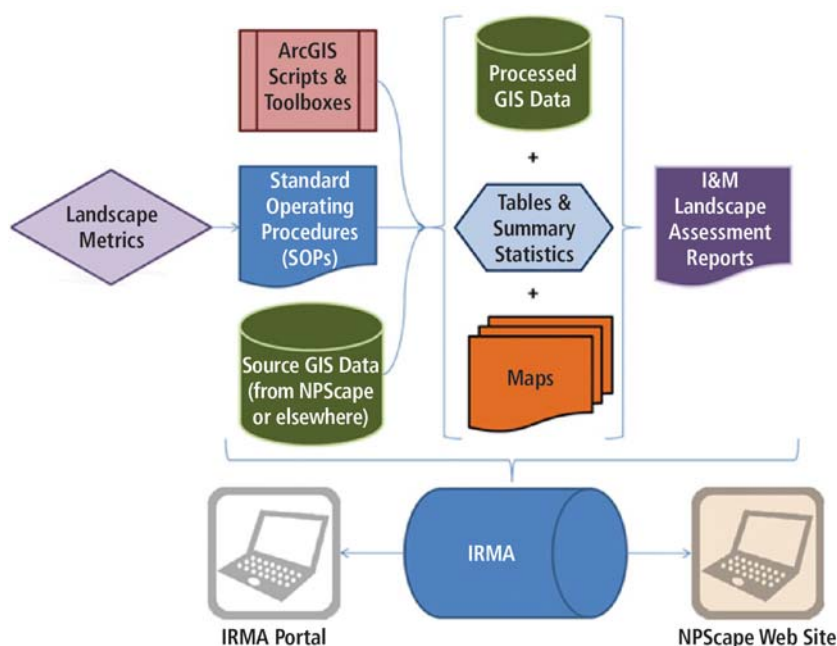
Figure 2. Overview of processing steps and products delivered by NPScape to I&M networks, parks, and others. We begin by defining a core set of landscape metrics that are of fundamental value to all or most parks (see table 1). We then document in great detail the GIS methods (SOPs) needed to quantify the landscape metrics, including the source GIS data inputs and ArcGIS scripts and toolboxes to assist with computations. Importantly, these methods enable others to recompute the landscape metrics using local source data, where available. Primary outputs from our methods include processed GIS data, tables with summary statistics, and maps to assist visualization by non-GIS audiences. These outputs are then used to generate I&M assessments and reports. All NPScape products are managed through the Integrated Resource Management Applications (IRMA) system and are available for public viewing and download through either the IRMA portal or the NPScape Web site (see sidebar).
