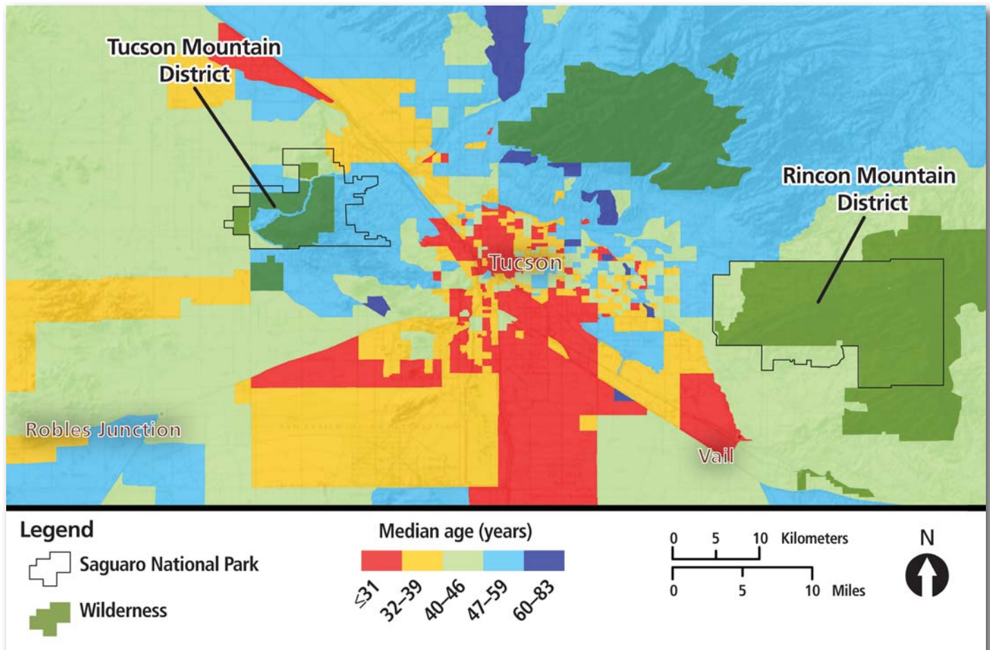
Figure 6. Median age of residents based on data from the 2010 U.S. Census for areas surrounding Saguaro National Park. Census-based demographic maps and analyses such as these provide important insights on where and how best to engage local communities as park recreational visitors. NPScope coordinates with the Social Science Branch of the Environmental Quality Division on the production and distribution of these metrics.
