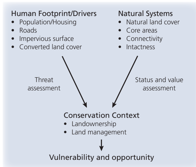
Figure 1. Broad categories of measures evaluated by NPScape and how they contribute to understanding the landscape context of parks and park resources.
