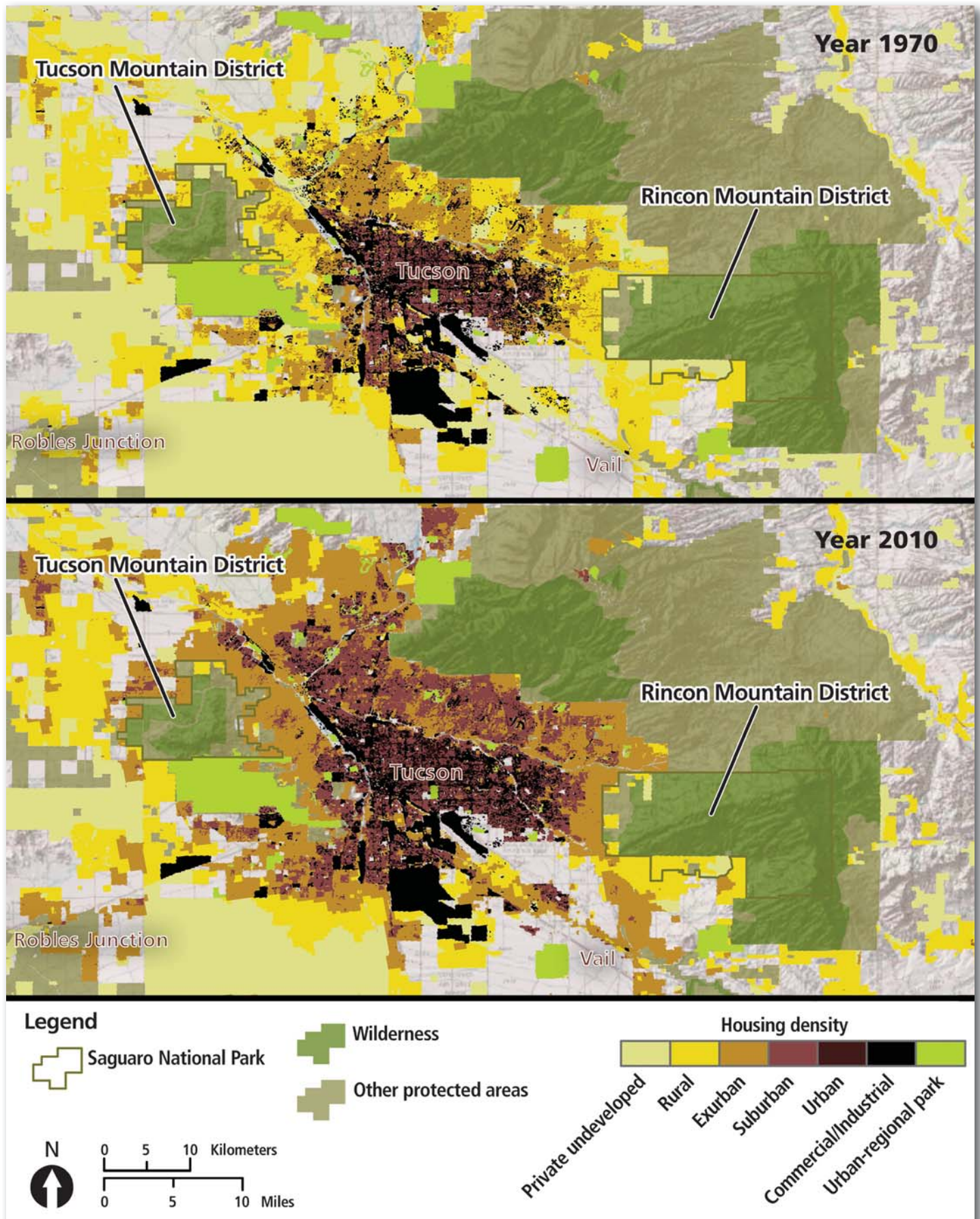
Figure 3. Housing density around Saguaro National Park in the recent past (1970, top map) and present (2010, bottom map). Housing density categories are defined by Theobald (2005): rural ( < 0.0618 housing units/ha [ < 0.1527 units/ac]), exurban ( 0.0618 – 1.47 units/ha [ 0.1527 – 3.63 units/ac]), suburban ( 1.47 – 10.0 units/ha [ 3.63 – 24.7 units/ac]), and urban ( > 10.0 units/ha [ > 24.7 units/ac]).
