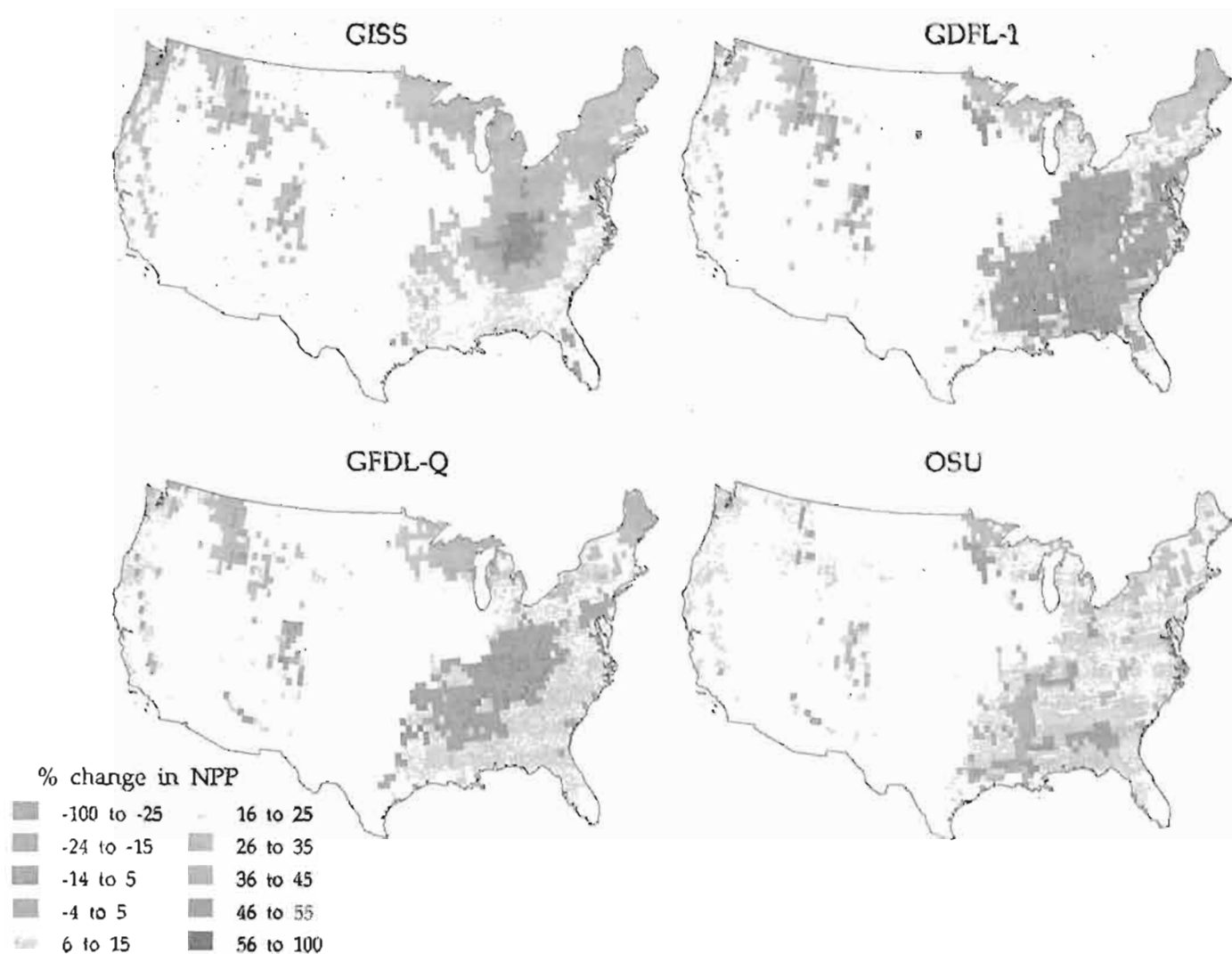
Figure 2.6.—Spatial comparison of the responses in annual net primary production (NPP) between contemporary climate of 355 ppmv CO 2 and the various GCM climates at 625 ppmv CO 2 as predicted by the Terrestrial Ecosystem Model for the 1443 grid cells (0.5° latitude by 0.5° longitude) that describe the historical range of temperate forests in the United States (see fig. 2.1).
