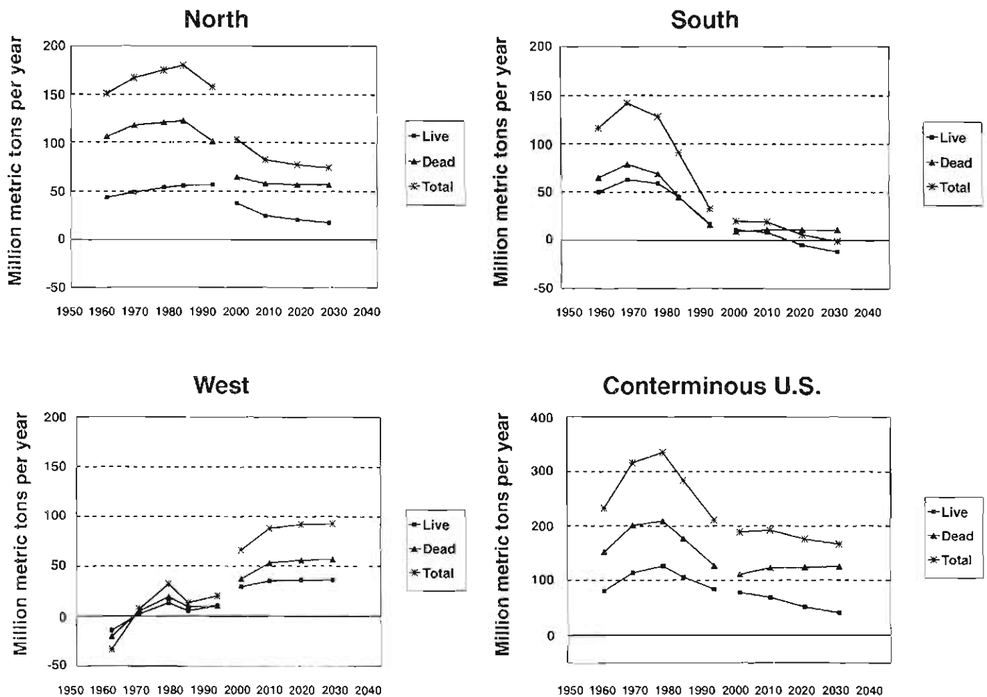
Figure 4.4. —Carbon flux in live (tree and understory) and dead (soil and forest floor) organic matter, conterminous U.S. forests, 1952-2040. A positive flux indicates increasing carbon storage in forest ecosystems.
