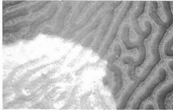
Coral disease (shown here in white) and coral bleaching, two threats to coral reefs, are being monitored with a digital video camera in Virgin Islands National Park. Quantitative and qualitative data can be derived from the videotapes and used by researchers and resource managers to address resource concerns in parks with coral reefs.
