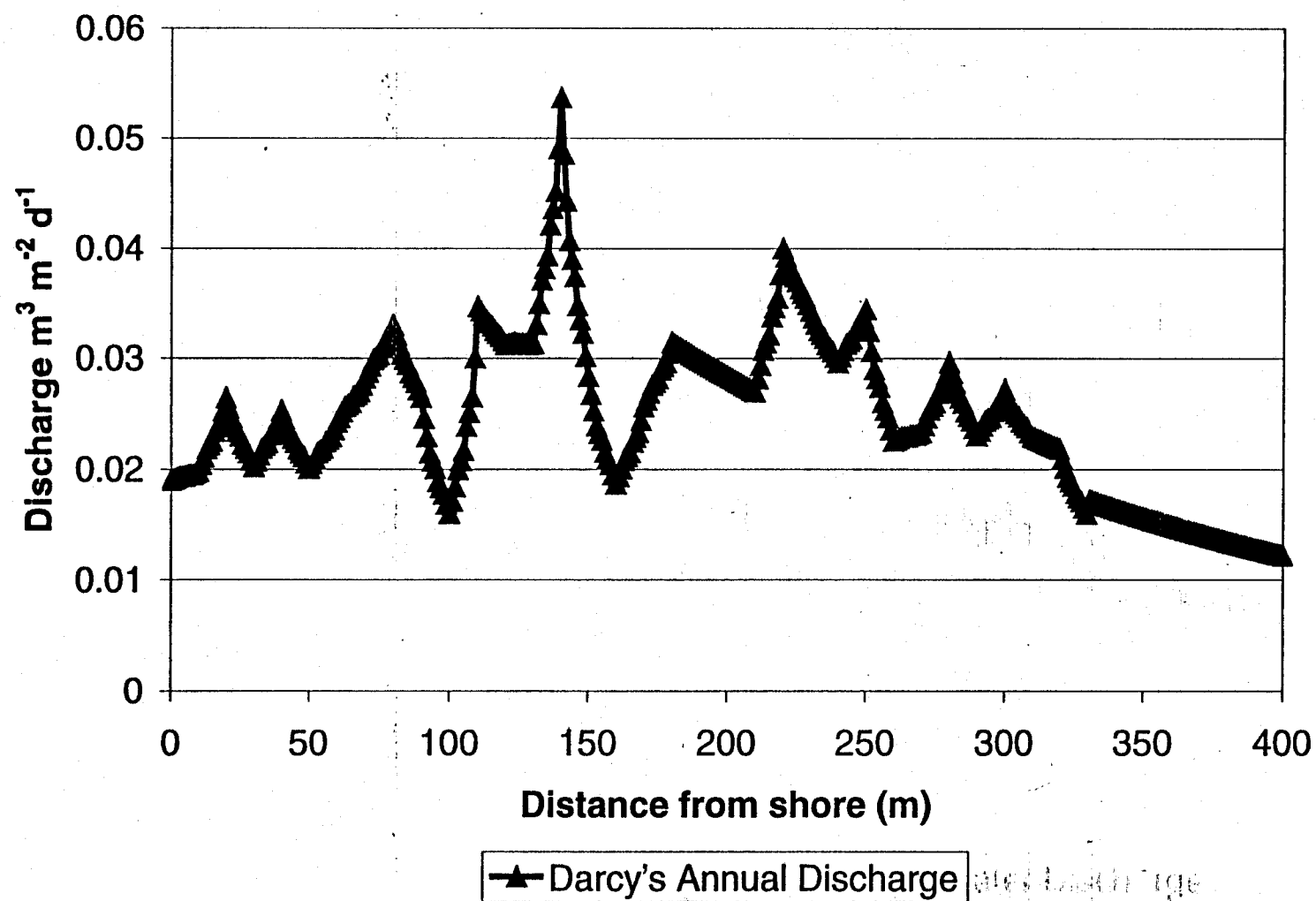
Figure 8. Darcy's Law Discharge
