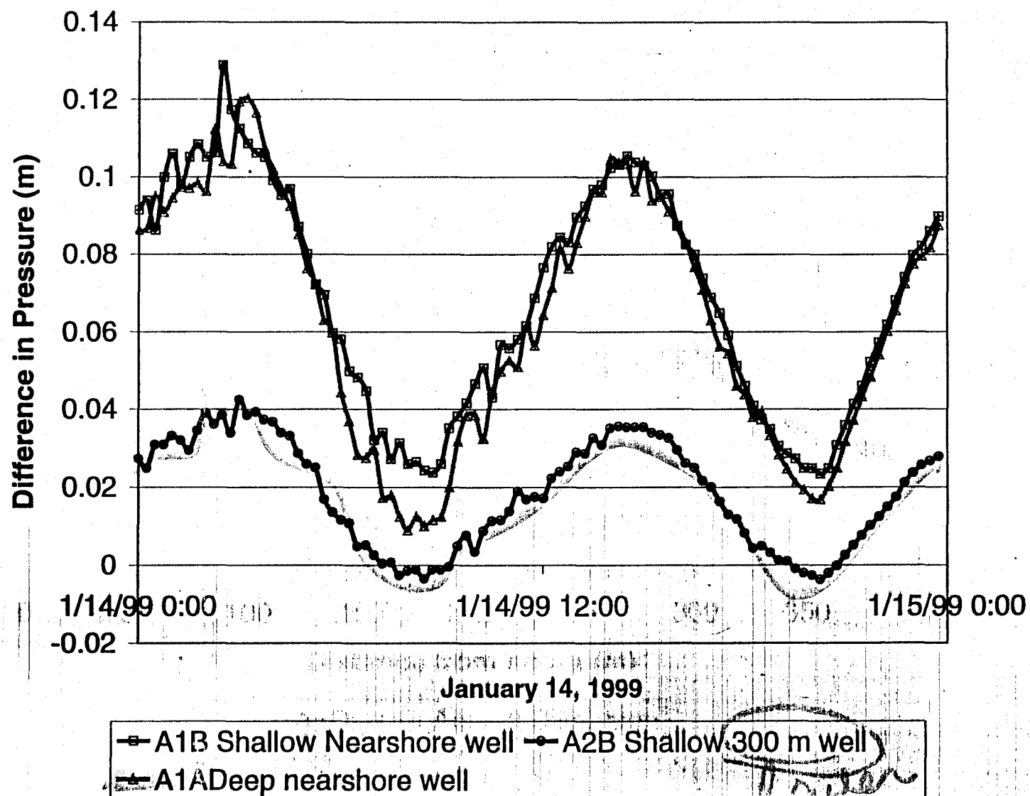
Figure 7. Difference in pressure head
