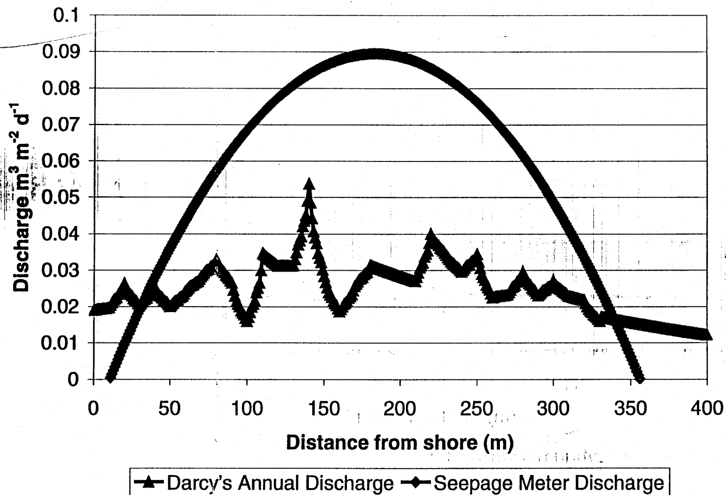
Figure 9. Comparison plot with Darcy's Law Discharge and Seepage Meter Discharge
