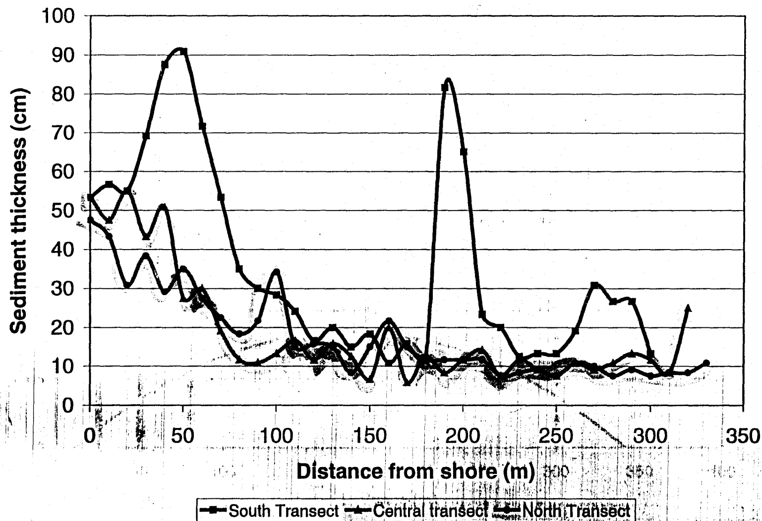
Figure 4. Sediment thickness versus distance
