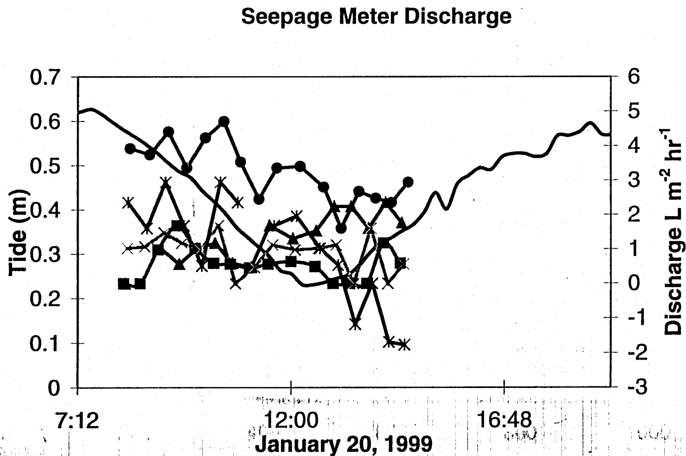
Figure 32. Tidal variation and seepage meter discharge
