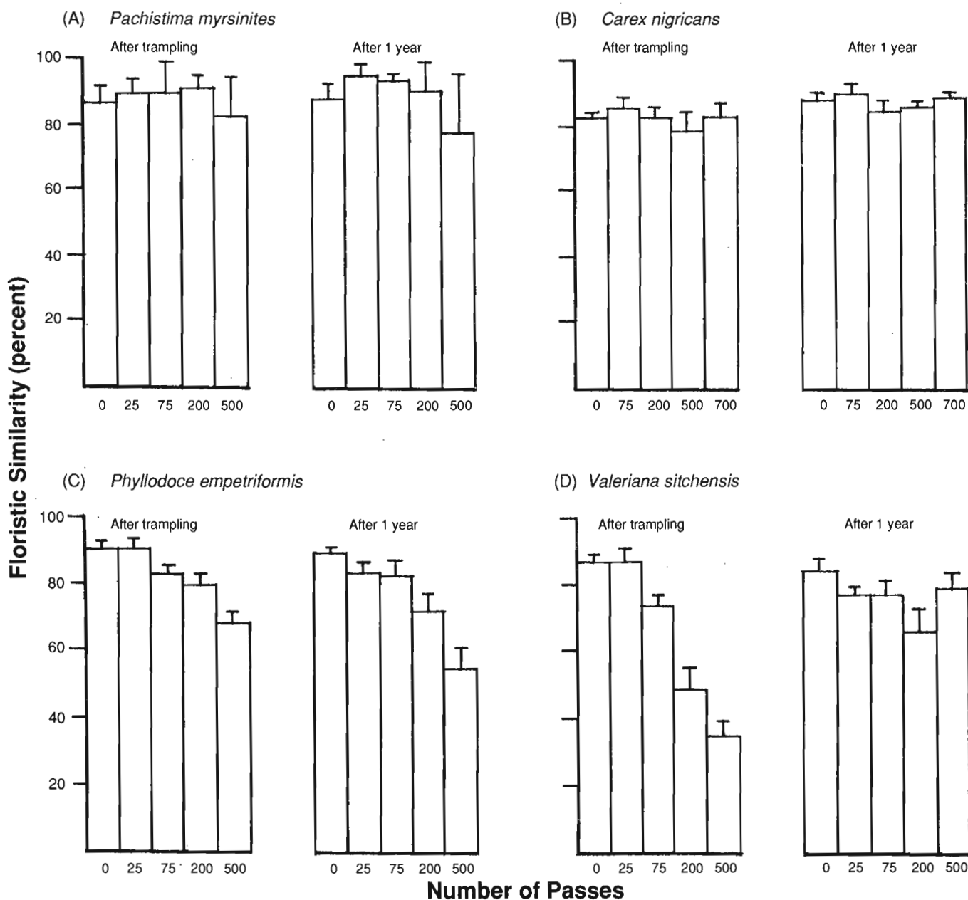
Figure 5 —Floristic similarity, comparing composition before and after disturbance, in four vegetation types in Washington's Cascade Mountains. Vertical bars represent 1 standard error above the mean.
