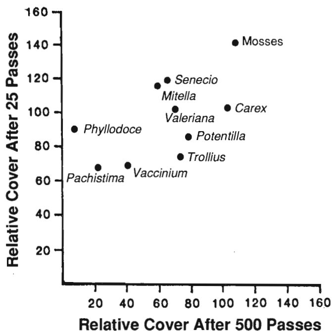
Figure 8 —Relative cover 1 year after light and heavy trampling for abundant species in four vegetation types in Washington's Cascade Mountains.
