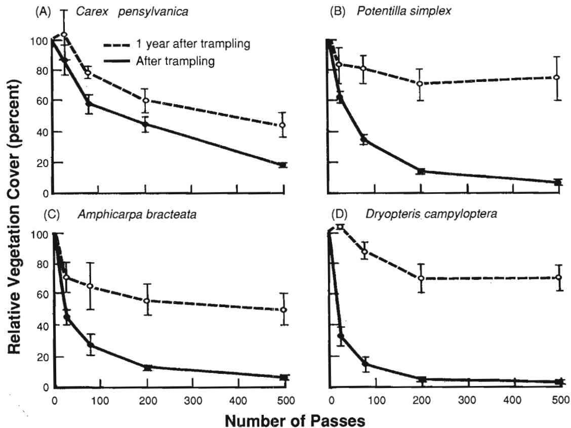
Fig. 19 —Relative vegetation cover after trampling and after 1 year of recovery for four vegetation types in North Carolina's Great Smoky Mountains. Vertical bars represent 1 standard error above and below the mean.
