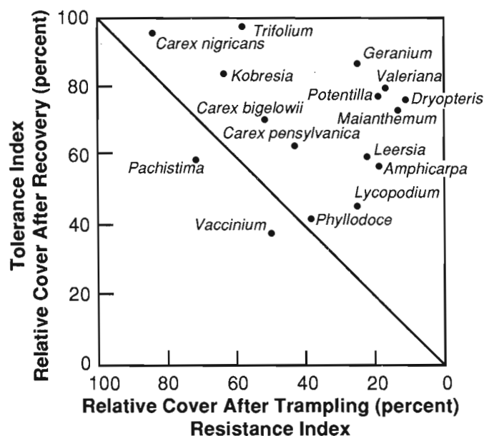
Figure 37 —Resistance, tolerance, and resilience of the 16 vegetation types in all four regions. Resilience is indicated by the perpendicular distance from the diagonal line of equal resistance and tolerance.
