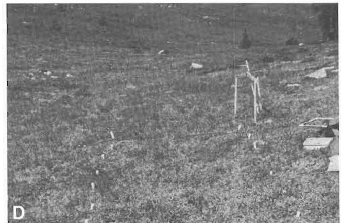
Figure 1 —Vegetation types in Washington's Cascade Mountains are (A) Pachistima , (B) Valeriana , (C) Phyllodoce , and (D) Carex .
