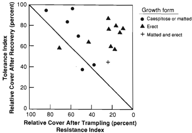
Figure 41 —Resistance, tolerance, and resilience of vegetation types in relation to the growth form of dominant species. Resilience is indicated by the perpendicular distance from the diagonal line of equal resistance and tolerance. Refer to figure 37 for names of each vegetation type.
