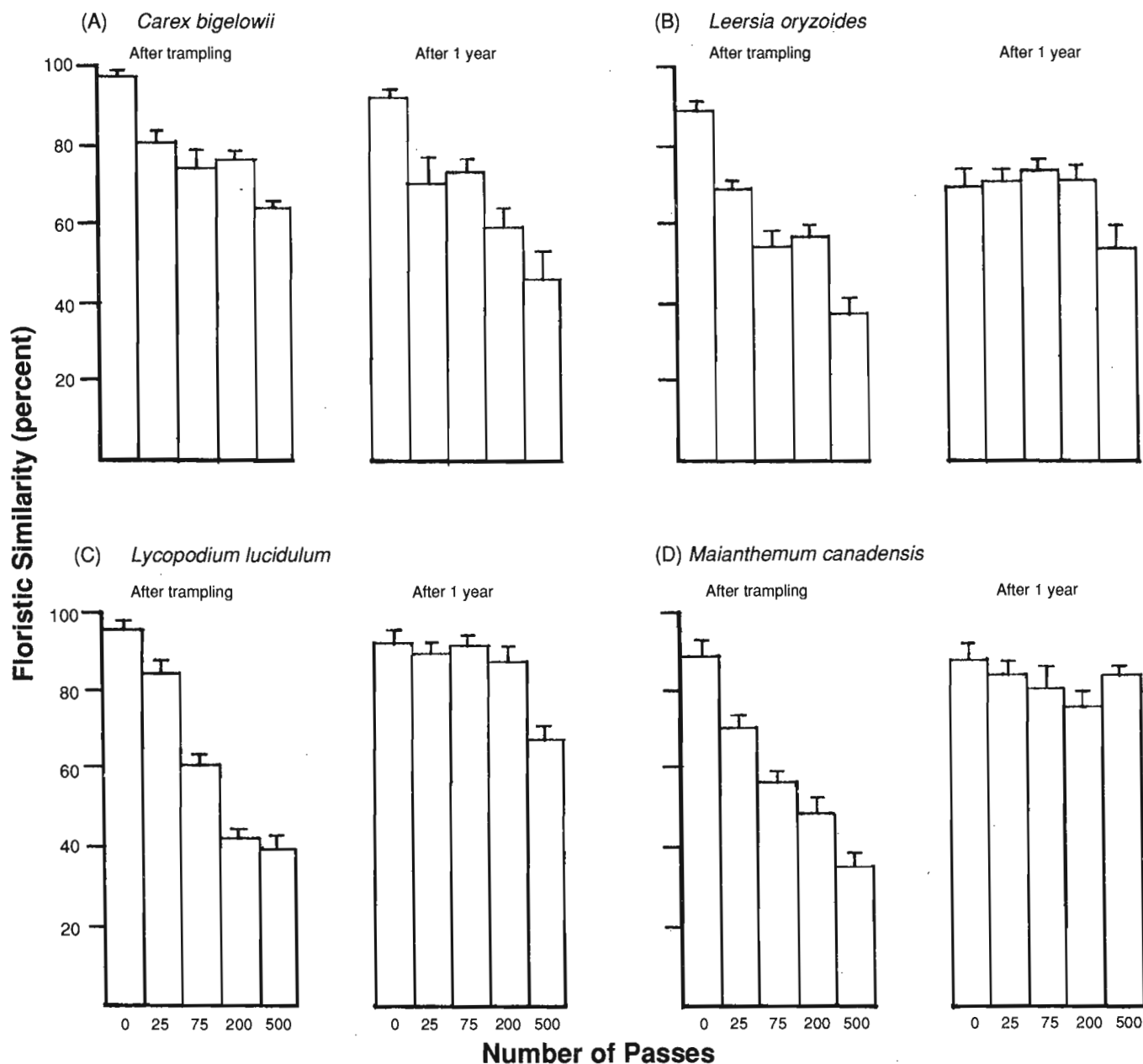
Figure 23 —Floristic similarity, comparing composition before and after disturbance, in four vegetation types in New Hampshire's White Mountains. Vertical bars represent 1 standard error above the mean.
