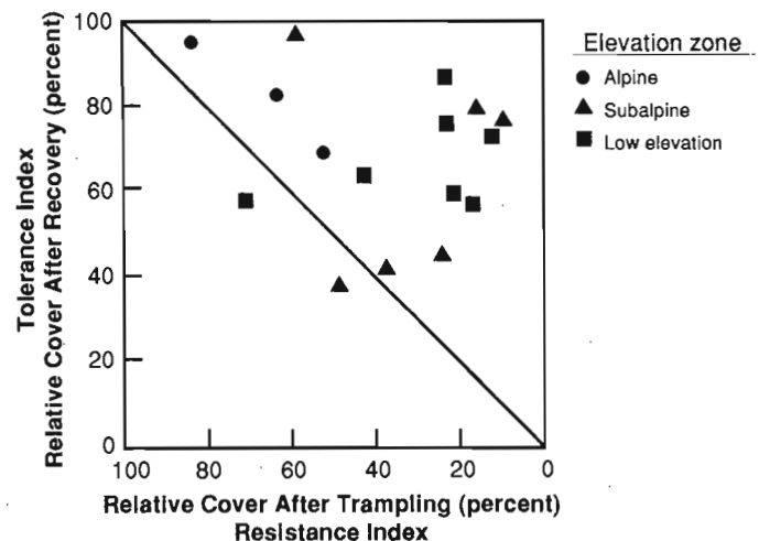
Figure 39 —Resistance, tolerance, and resilience of vegetation types in different elevation zones. Resilience is indicated by the perpendicular distance from the diagonal line of equal resistance and tolerance. Refer to figure 37 for names of each vegetation type.
