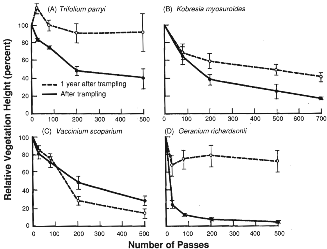
Figure 12 —Relative vegetation height after trampling and after 1 year of recovery in four vegetation types in Colorado's Rocky Mountains. Vertical bars represent 1 standard error above and below the mean.
