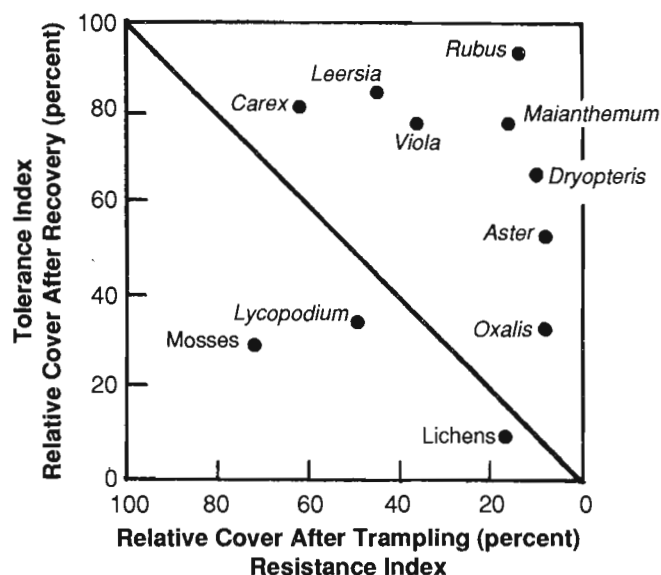
Figure 27 —Resistance, tolerance, and resilience of abundant species in four vegetation types in New Hampshire's White Mountains. Resilience is indicated by the perpendicular distance from the diagonal line of equal resistance and tolerance.
