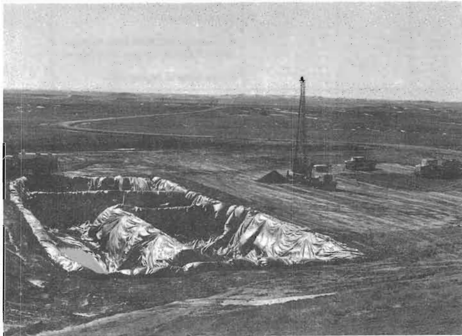
Photograph 1 - Properly Constructed Drillsite
