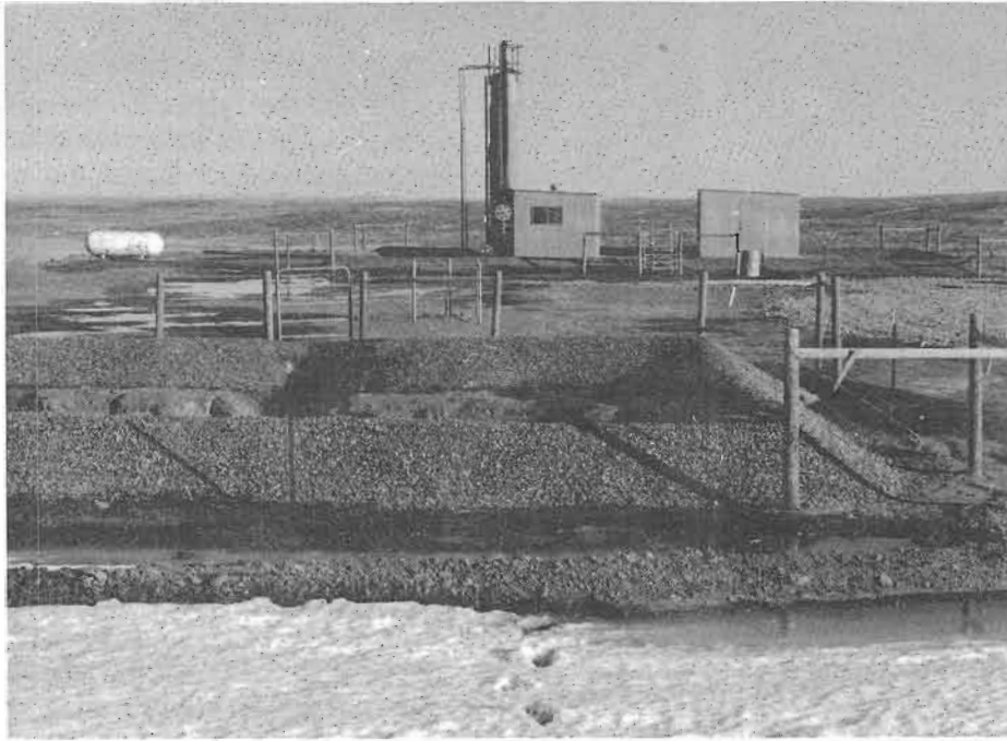
PHOTOGRAPH 4. TYPICAL ONSITE PRODUCED WATER DISPOSAL PITS
