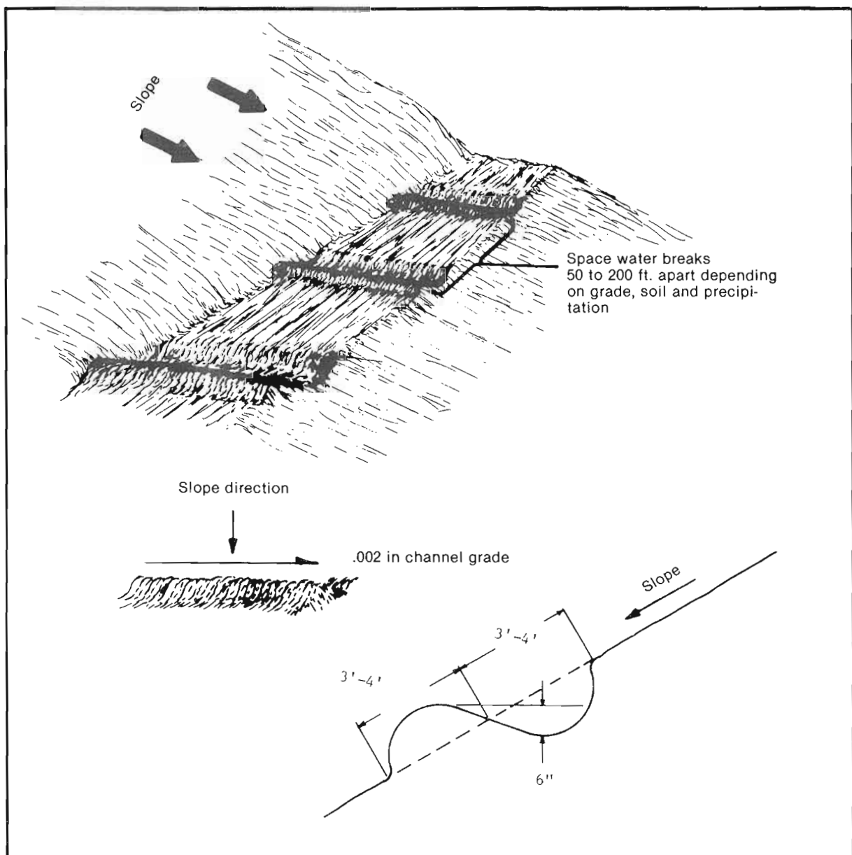
FIGURE 10. WATERBREAK CONSTRUCTION FOR PIPELINE AND BURIED CABLES
