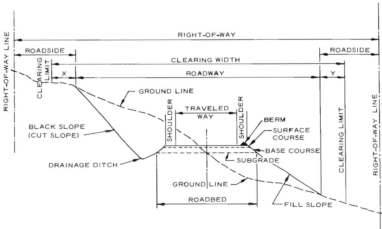
FIGURE 2. ILLUSTRATION OF COMMONLY USED TERMS IN ROAD DESIGN AND POTENTIALLY DISTURBED AREA WITHIN THE RIGHT-OF-WAY
