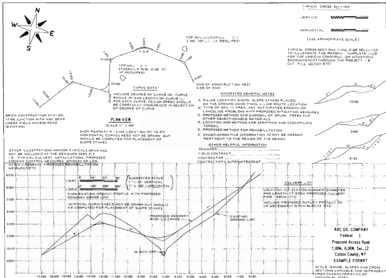
FIGURE 4. TYPICAL ROAD PLAN AND PROFILE DRAWING FOR AN OIL AND GAS ROAD
