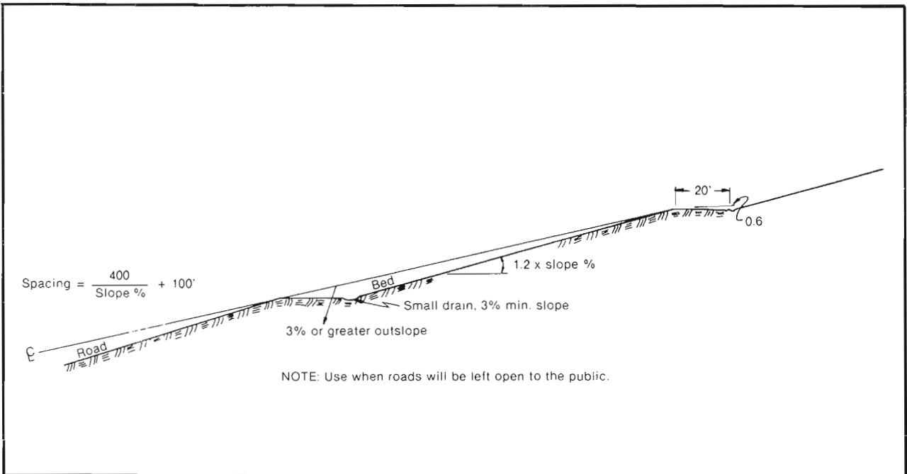
FIGURE 6. PROFILE VIEW OF BROAD BASED DRAINAGE DIP USE FOR PERMANENT ROADS WHERE ROAD GRADIENT DOES NOT EXCEED 10 PERCENT
