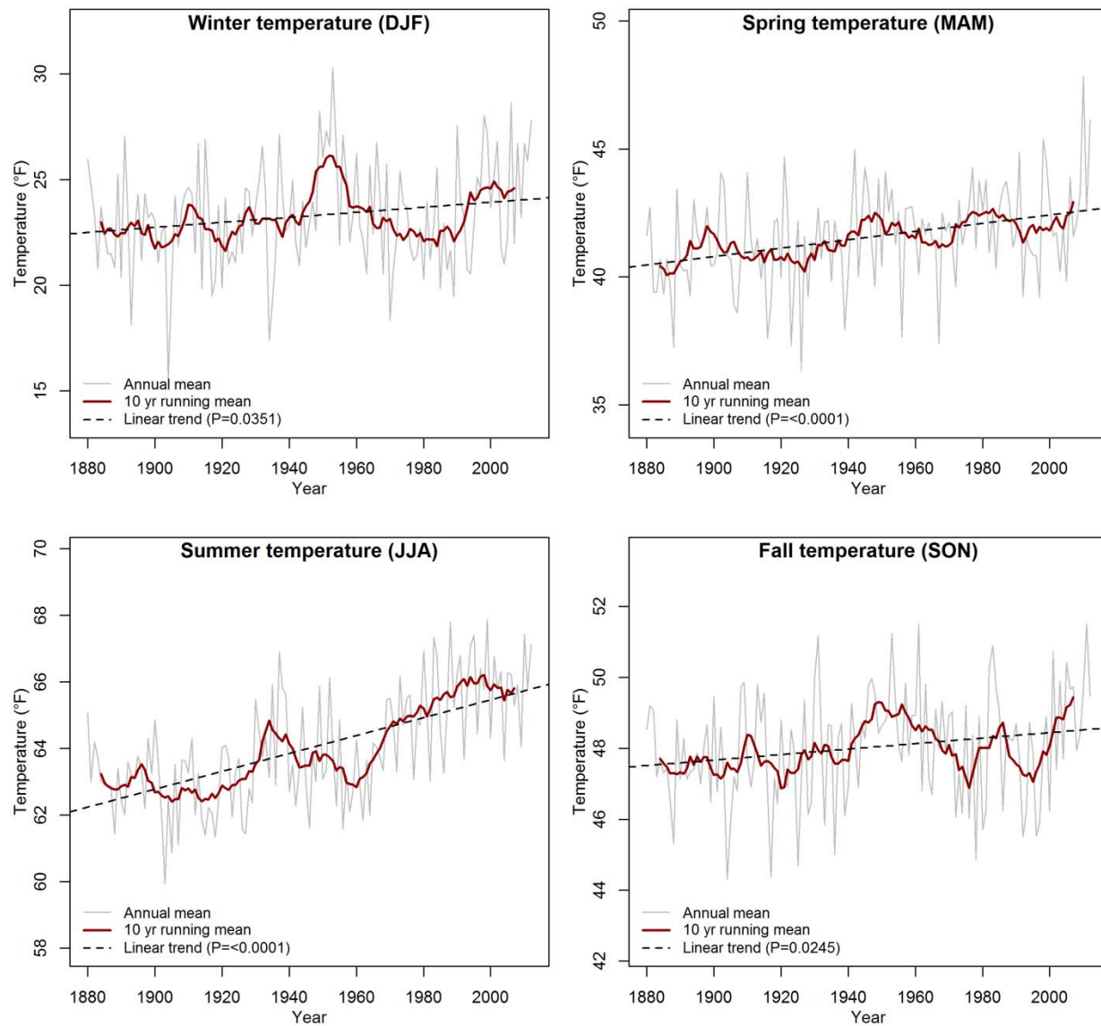
Figure 6. Seasonal temperature trends (1880-2012) from the Acadia NP, ME long-term weather station ( cdiac.ornl.gov ).
