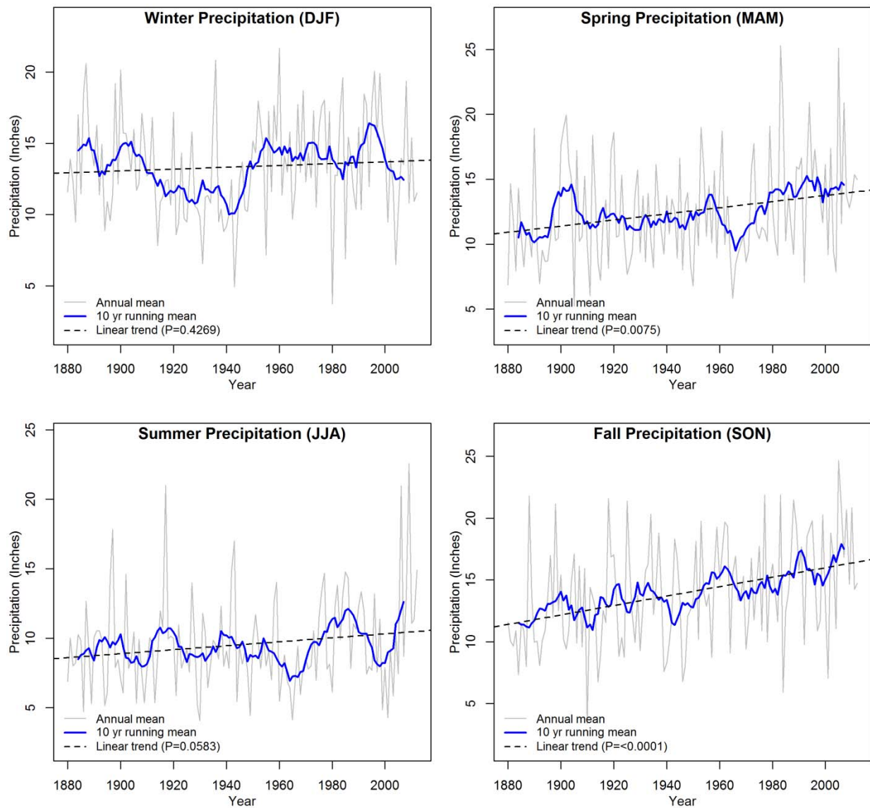
Figure 7. Seasonal precipitation trends (1880-2012) from the Acadia NP, ME long-term weather station ( cdiac.ornl.gov ).
