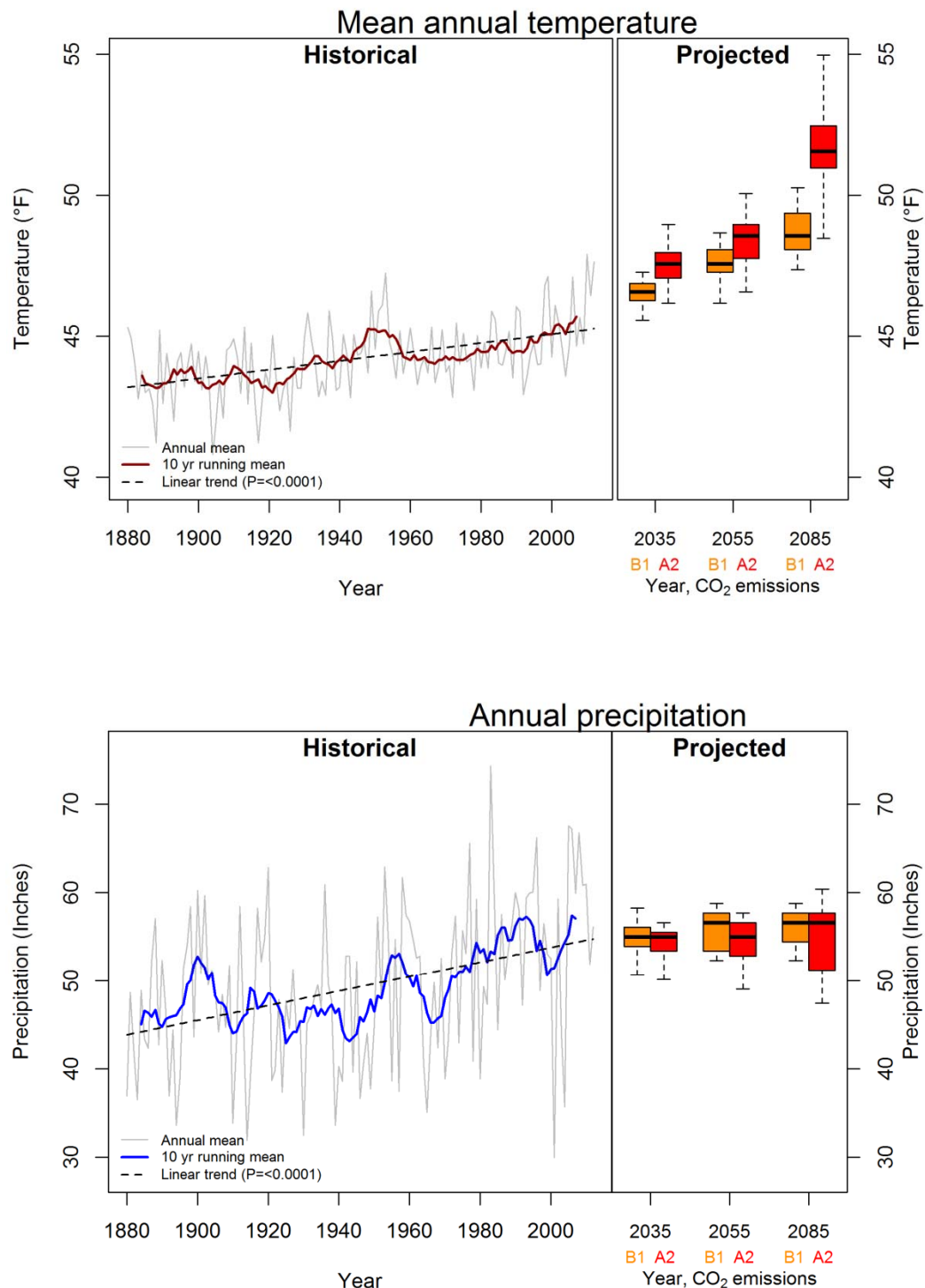
Figure 5. Historical and projected mean annual temperature and annual precipitation for Acadia National Park. Historical data (1880-2012) are from the Acadia NP, ME long-term weather station ( cdiac.ornl.gov ). Projected climate change for the Acadia National Park area (data from Kunkel et al. 2013, see Tables 4, 6 and Figures 16, 27) are for three future 30 year time periods centered on 2035 (2021-2050), 2055 (2041-2070), and 2085 (2070-2099). Two greenhouse gas emissions scenarios are presented, the low (B1) and high (A2) scenarios (IPCC 2007). Projected climate boxplots indicate the variability in future projections among 14-15 CMIP3 climate models across the northeast region: the bold horizontal black line represents the mean among all models, the upper and lower ends of the boxes indicate the 25 th and 75 th percentile model output values and the whiskers show the minimum and maximum model values.
