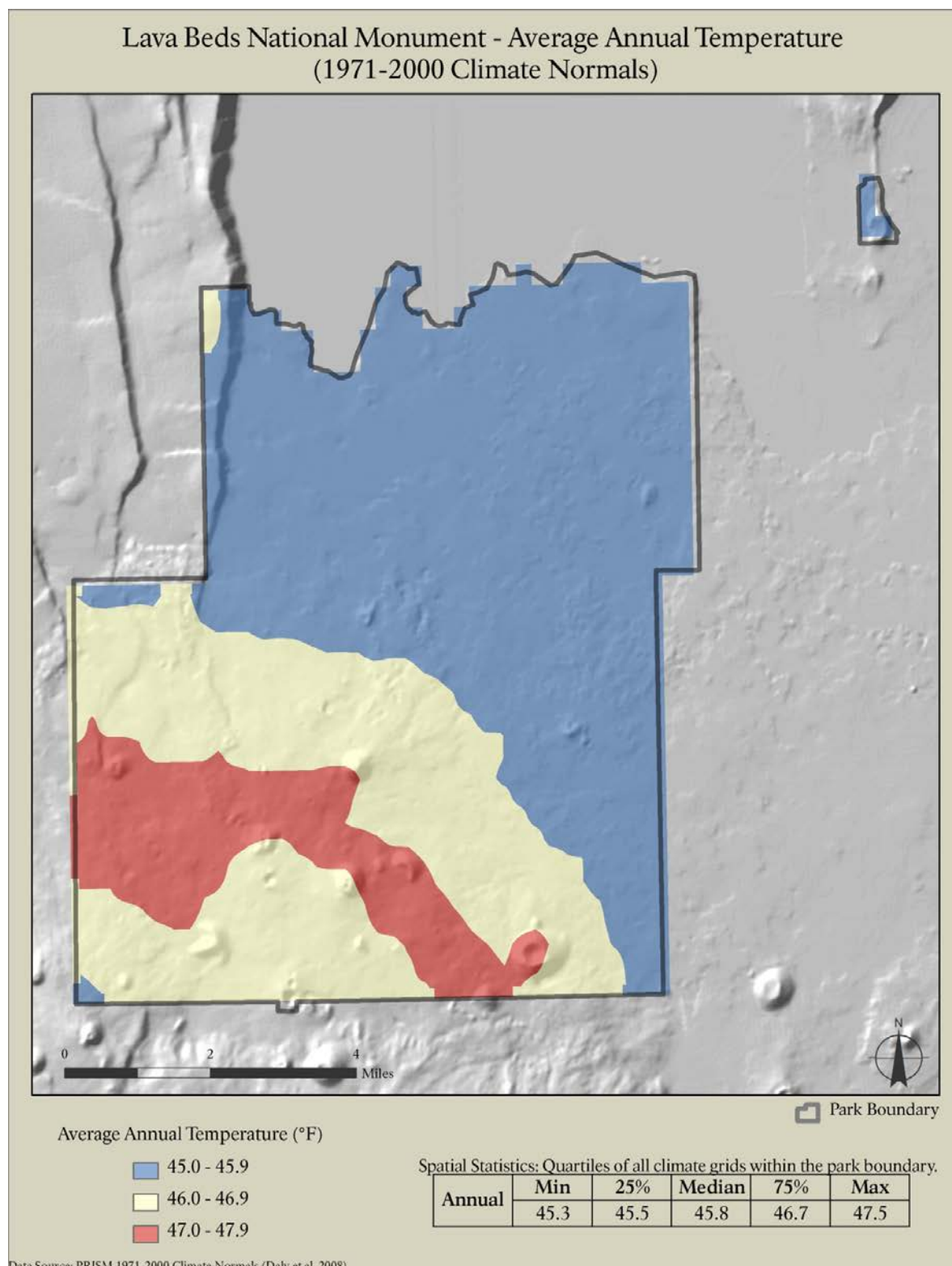
Figure A2. Average annual temperatures for Lava Beds National Monument (LBE) from the PRISM 1971-2000 Climate Normals (Daly et al. 2008). This map was prepared by investigators for the LANDFIRE project who extrapolated information using Landsat Thematic Mapper and other data. The inset table gives the spatially derived quartiles of all grids that fall within the park boundary.
