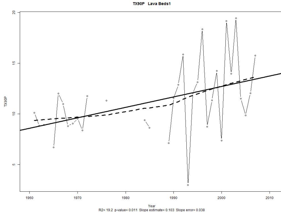
Figure A20. Example time series of the number of days when the maximum temperature is above the 90 th percentile during the reference period observed each year at Lava Beds National Monument, California, during 1960-2011. Trends are computed by linear least square (solid line) and locally weighted linear regression (dashed line). Missing data is handled as discussed in the text.
