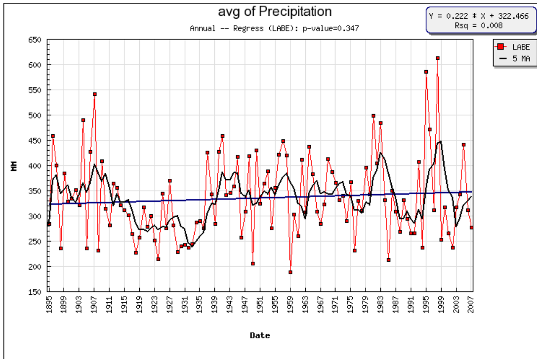
Figure A19. Time series of annual precipitation for CRLA from the park average of the PRISM modeled data (Daly et al. 2009). Black line is a five year moving average and the blue line is the trend associated with the regression parameters (inset). Date refers to year.
