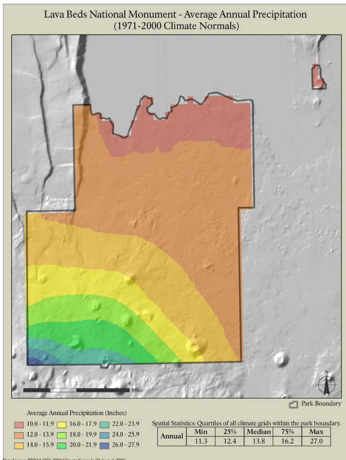
Figure A1. Annual precipitation for Lava Beds National Monument (LBE) from the PRISM 1971-2000 Climate Normals (Daly et al. 2008). This map was prepared by investigators for the LANDFIRE project who extrapolated information using Landsat Thematic Mapper and other data. The inset table gives the spatially derived quartiles of all grids that fall within the park boundary.
