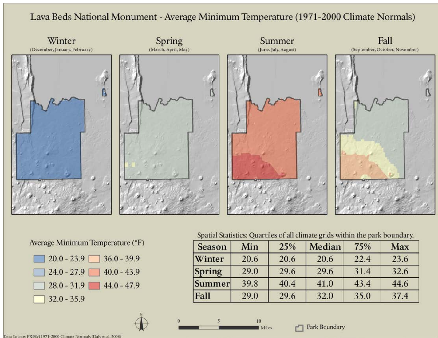
Figure A8. Average minimum temperatures for the winter (DJF), spring (MAM), summer (JJA), and fall (SON) seasons for Lava Beds National Monument (LBE) from the PRISM 1971-2000 Climate Normals (Daly et al. 2008). This map was prepared by investigators for the LANDFIRE project who extrapolated information using Landsat Thematic Mapper and other data. The inset table gives the spatially derived quartiles of all grids that fall within the park boundary.
