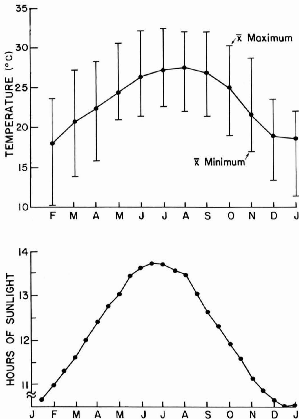
Figure 3. Annual patterns of mean monthly temperatures and hours of sunlight near study site.
