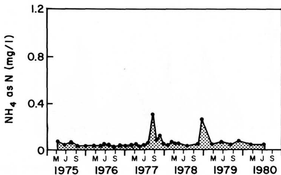
Figure 16a. Ammonia nitrogen concentration (mg l -1 ) at USGS Mowry Canal station 02290725 (1975-1980).
