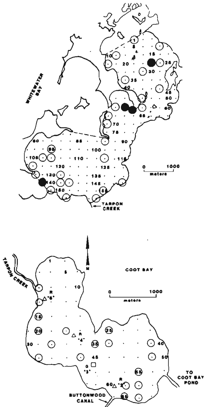
Figure 10. Diagram of Whitewater Bay (upper) and Coot Bay (lower). Stations with open circles were sampled once while darkened circles indicate stations sampled twice.
