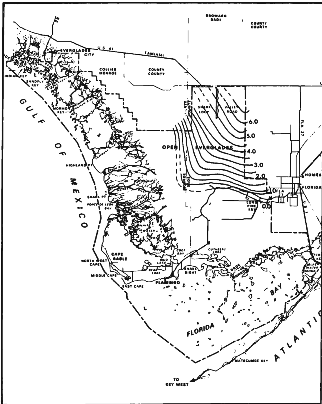
Figure 7: April 1, 1976: Low Water Contours (Contour Interval 0.5 Feet)
