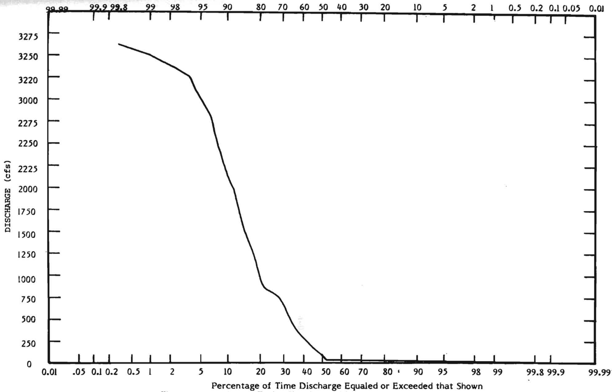
Figure 2l: 1976 Flow Duration Curve, Taylor Slough at Bridge
