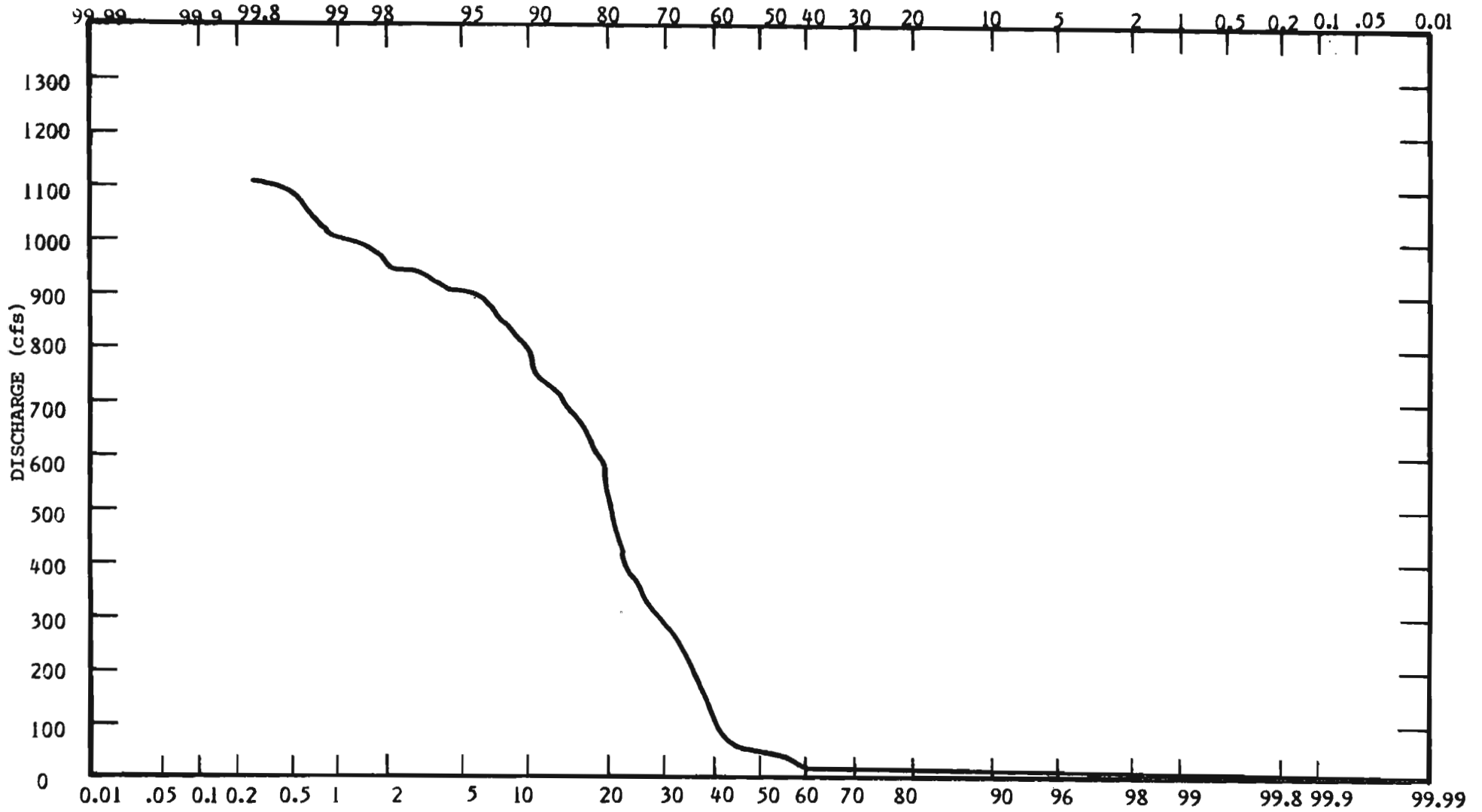
Percentage of Time Discharge equaled or Exceeded that Shown Figure 19: 1976 Flow Duration Curve, 40 Mile Bend to Monroe
