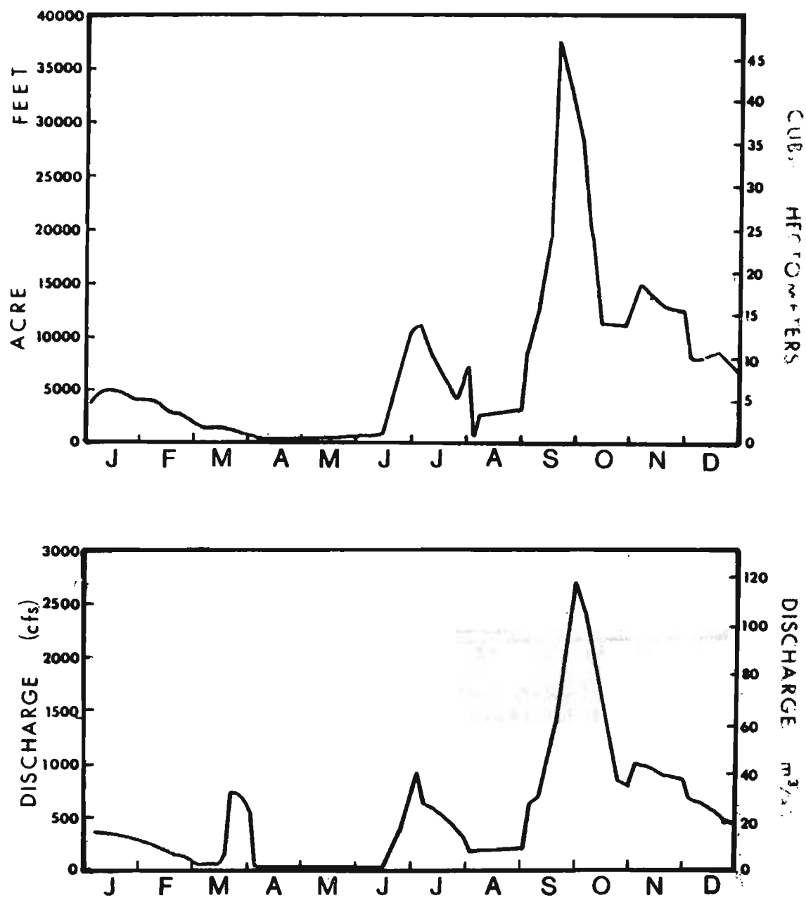
Figure 15: 1976 S-12 Discharge into Everglades National Park
