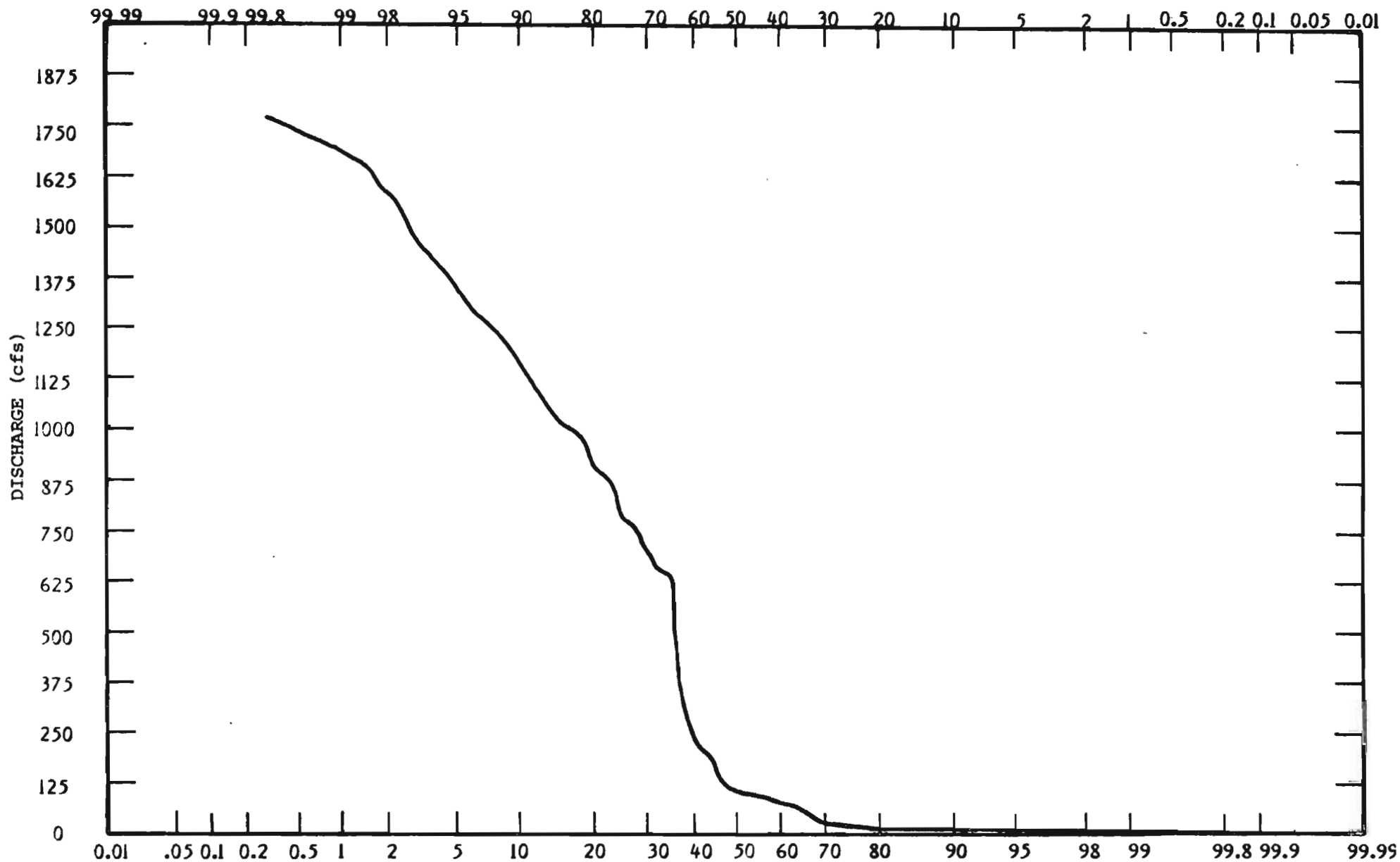
Percentage of Time Discharge Equaled or Exceeded that Shown Figure 20: 1976 Flow Duration Curve, Monroe to Carnestown
