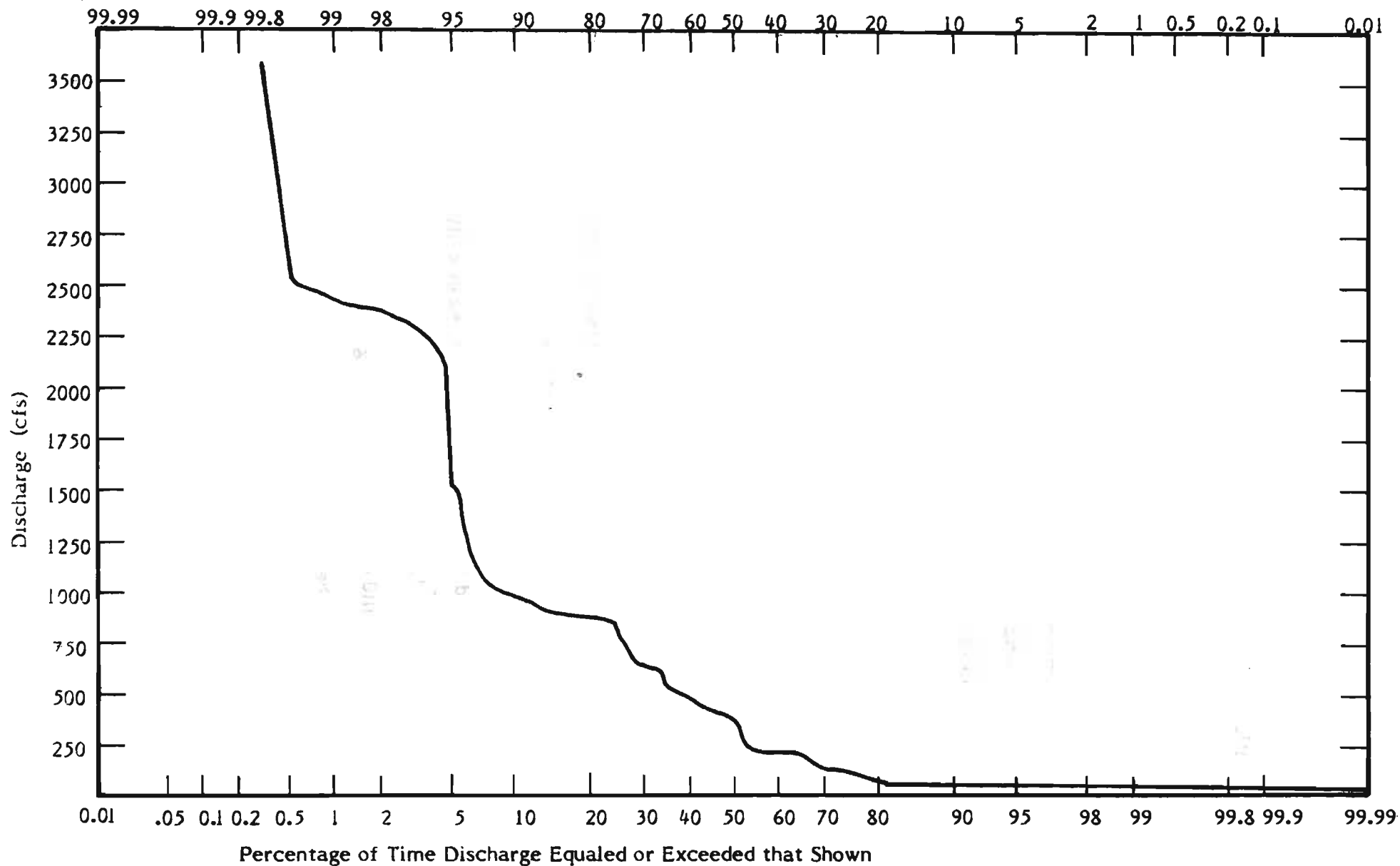
Figure 17: 1976 Flow Duration Curve, Tamiami Canal Outlets, L67-A to 40 Mile Bend
