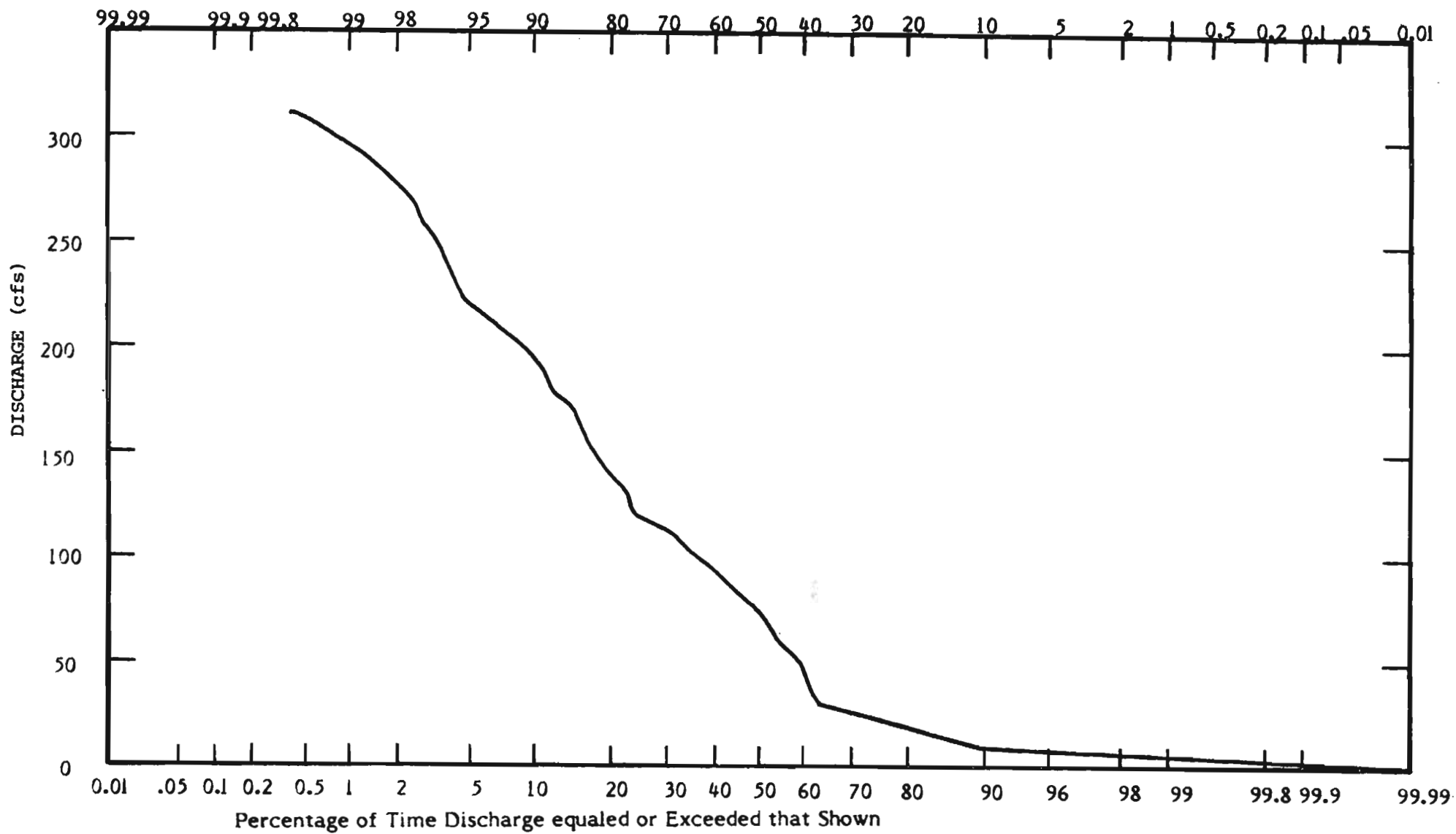
Figure 18: 1976 Flow Duration Curve, Levee 30 to Levee 67A
