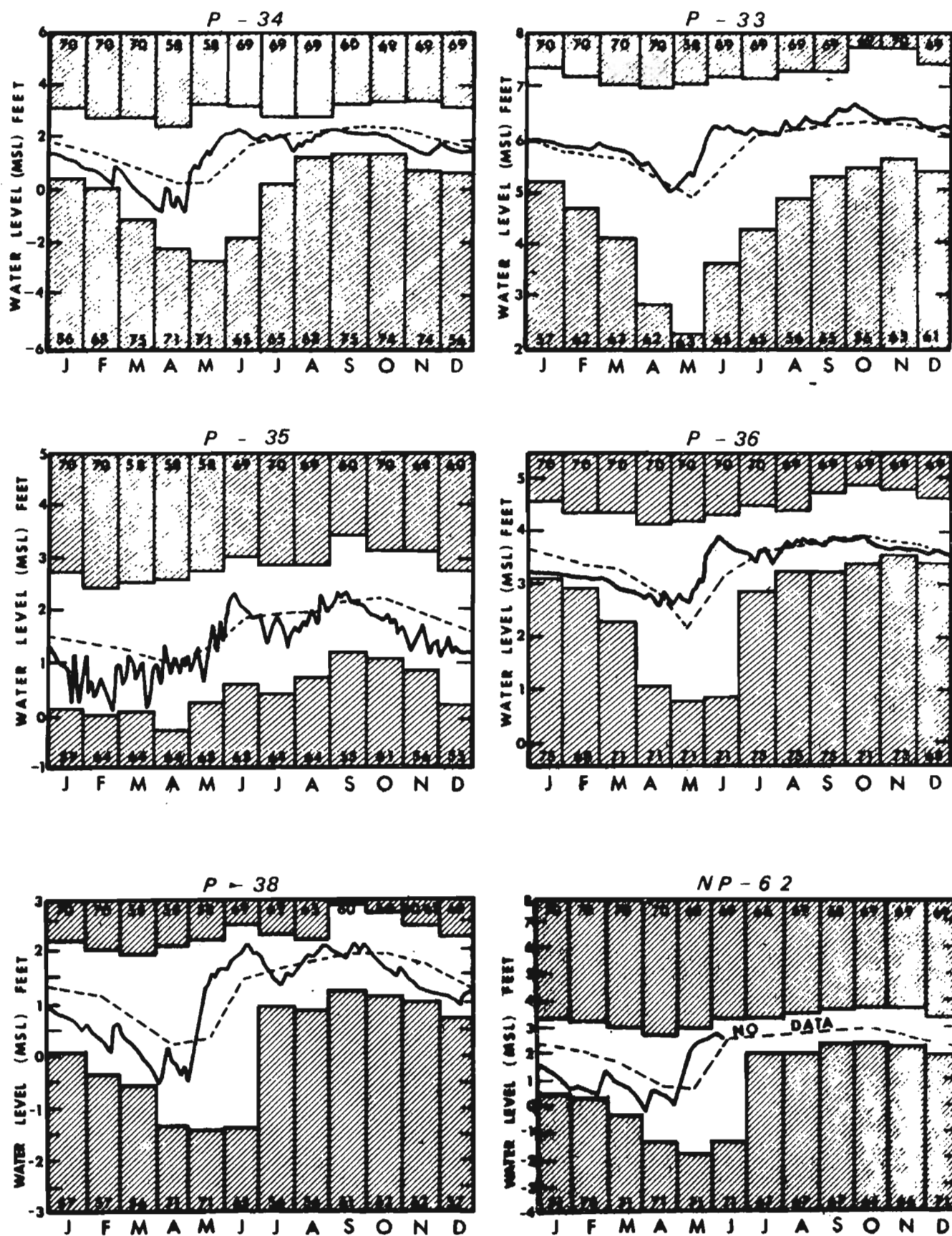
Figure 9: 1976 Hydrographs, Shark River Slough Monitoring Stations
