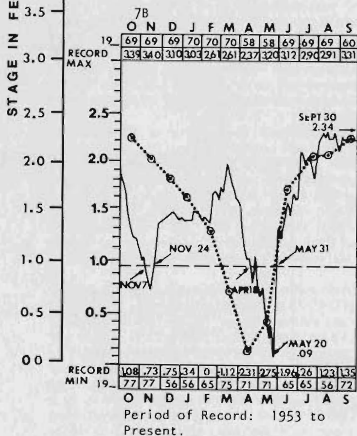
Figure 7. Water levels at (7A) Shark Slough station G-620 and (7B) P-34, West of Shark Slough.
