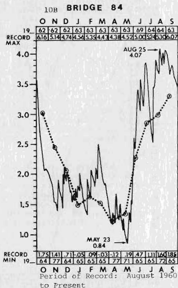
Figure 10. Water levels in Big Cypress at (10A) Bridge 105, (10B) Bridge 84 and (10C) Bridge 77.
