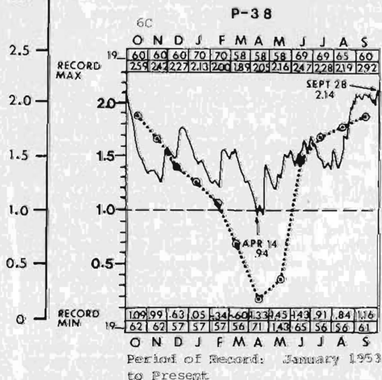
Figure 6. Water levels in Shark Slough at (6A) P-33, (6B) P-36, and (6C) P-38.
