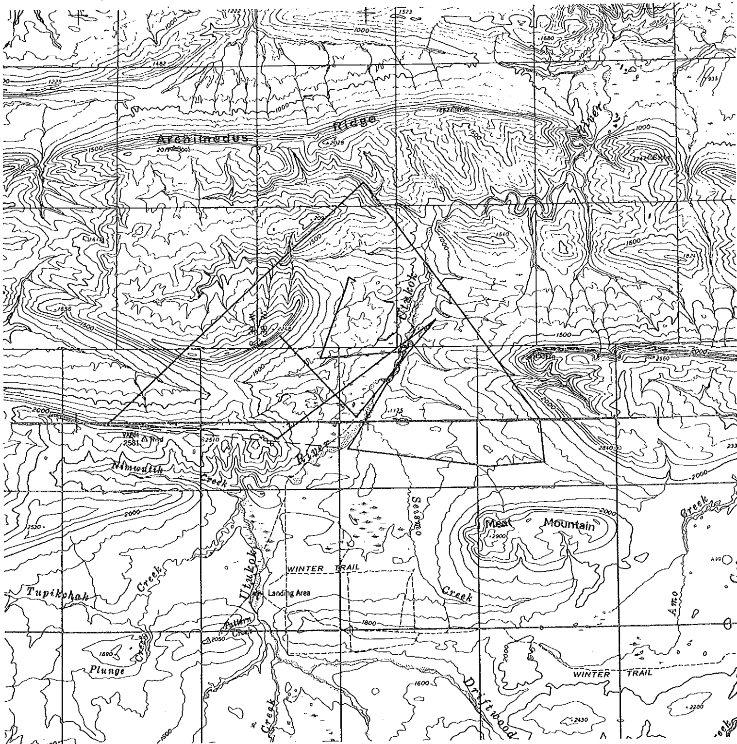
Fig. 2. Observed movement and home range size of grizzly bear No. 1097 in 1977, using the minimum home range method.
