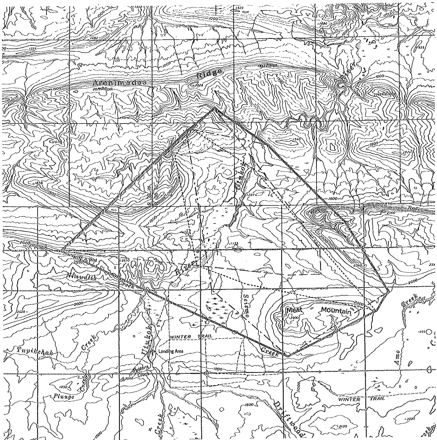
Fig. 5. Observed home range size of grizzly bear No. 1097 for 1977, 1978, 1979 and 1977-1979, using the minimum home range polygon method.
