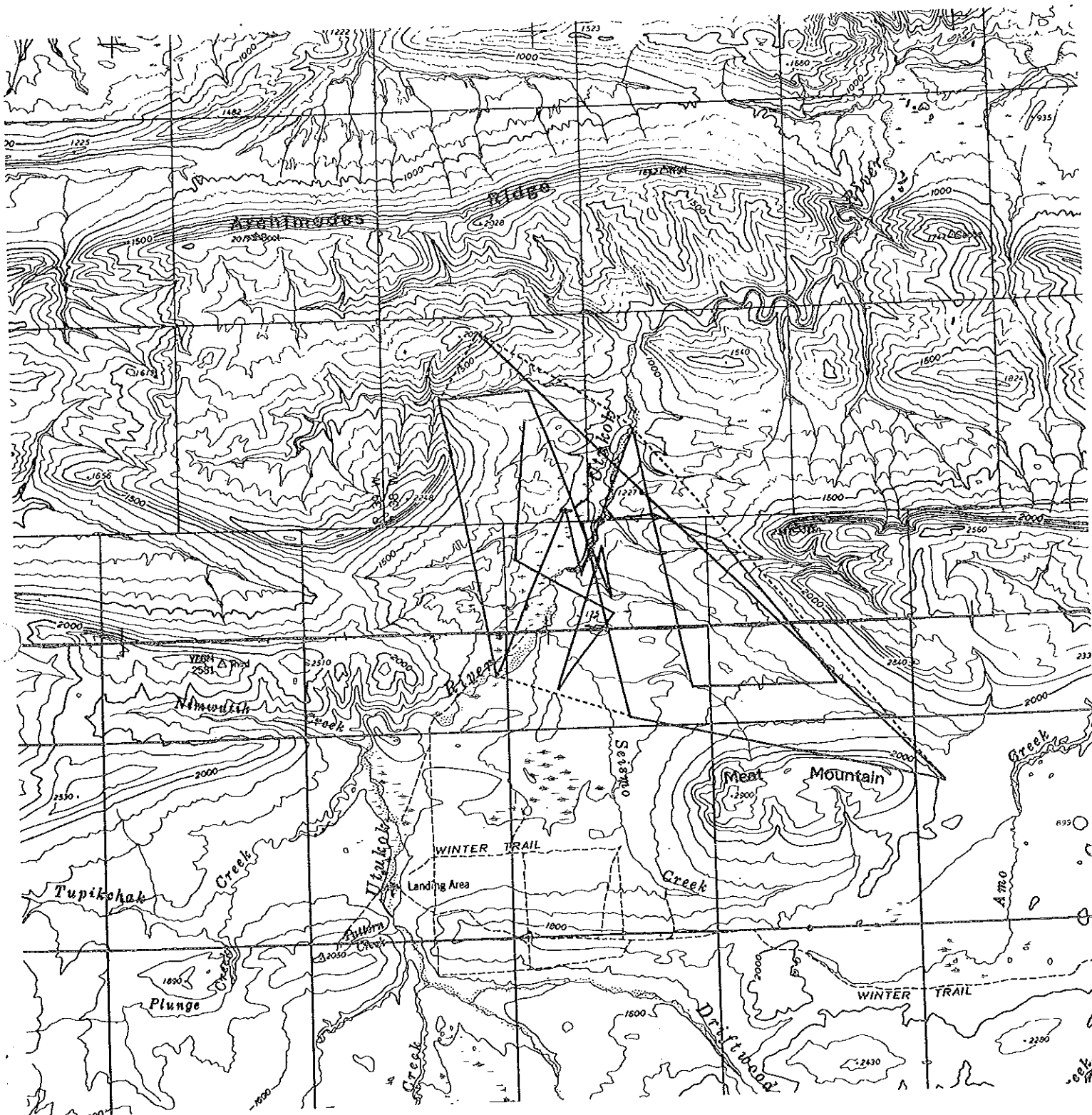
Fig. 4. Observed movement and home range size of grizzly bear No. 1097 in 1979, using the minimum home range polygon method.
