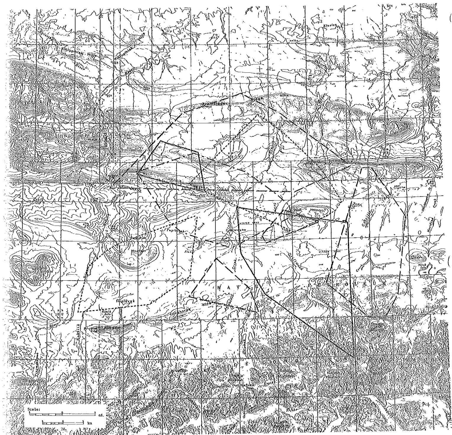
Fig. 8. The home ranges of nine females without offspring in the study area.
