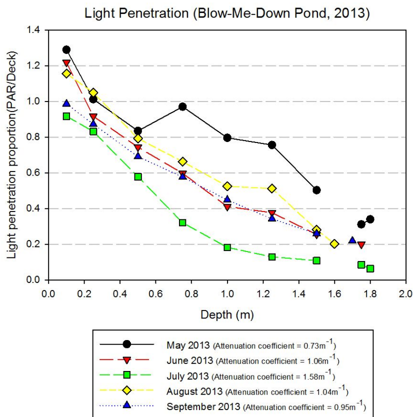
Figure 10. Light penetration profiles from Blow-Me-Down Pond.
