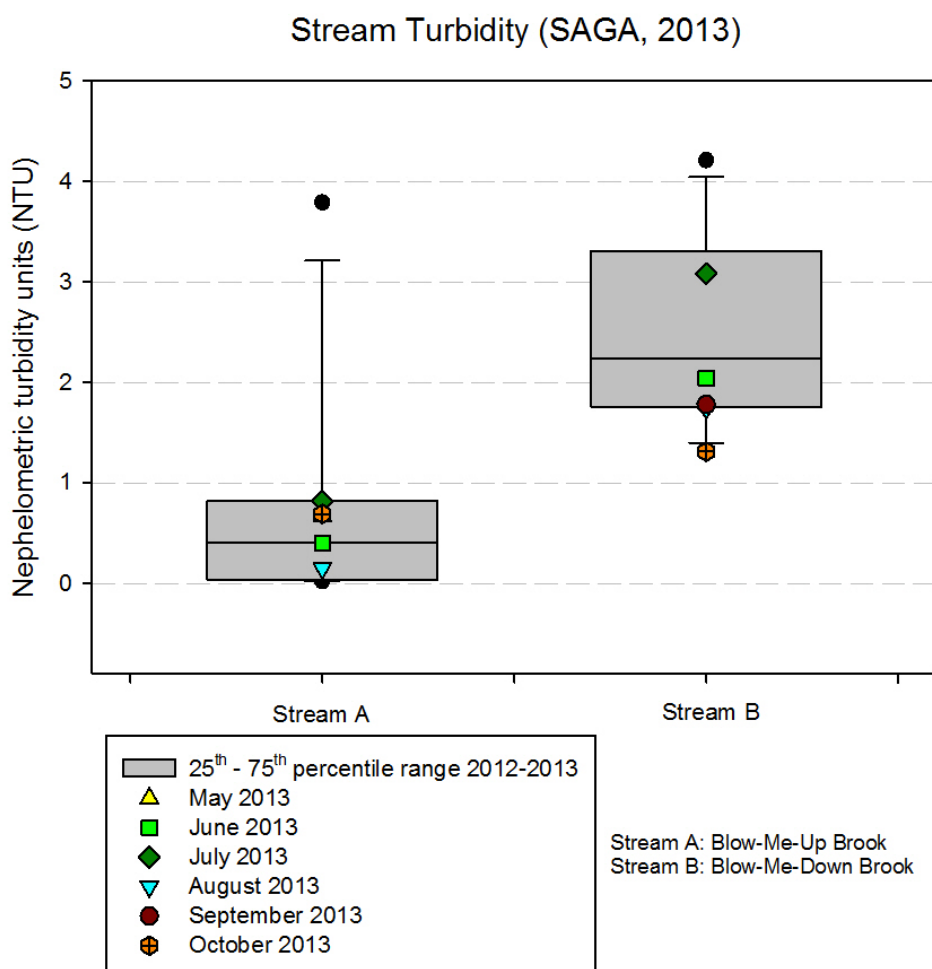
Figure 11. Stream turbidity from 2013 monthly measurements. The data are overlaid on a box plot of measurements taken from 2012-2013.
