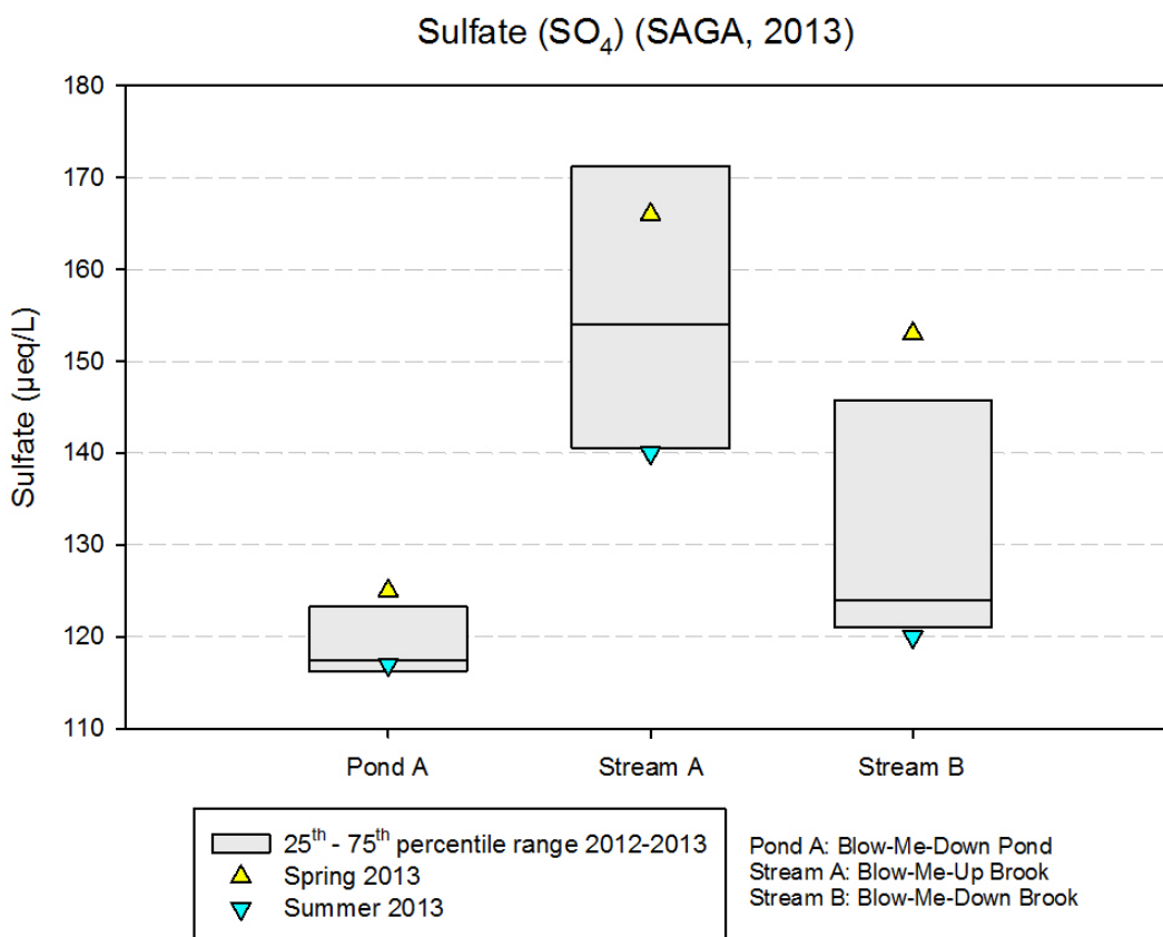
Figure 16. Sulfate from 2012-2013 spring and summer water samples. The data are overlaid on a box plot of measurements taken from 2012-2013.
