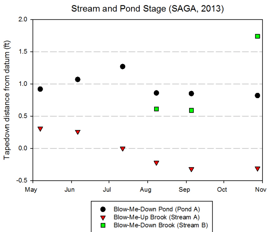
Figure 17. Stream and pond stage obtained in 2013 by measuring from a permanent datum point to the water surface.
