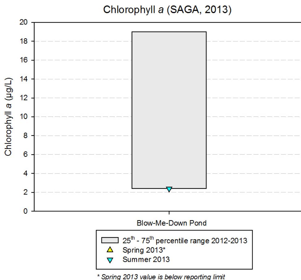
Figure 14. Chlorophyll a from 2013 spring and summer water samples. The data are overlaid on a box plot of measurements taken from 2012-2013.
