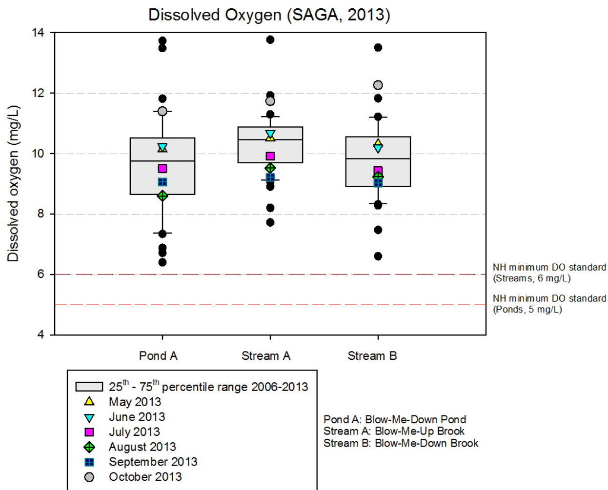
Figure 6. Dissolved oxygen (surface) from 2013 YSI sonde in-situ measurements overlaid on a box plot of measurements taken from 2006-2013.
