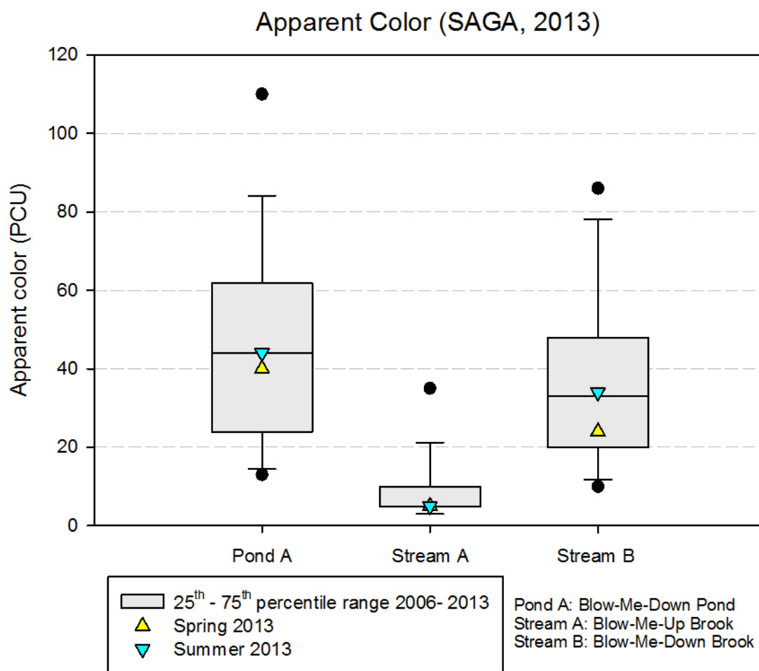
Figure 8. Apparent color from 2013 water samples overlaid on a box plot of measurements taken from 2006-2013.
