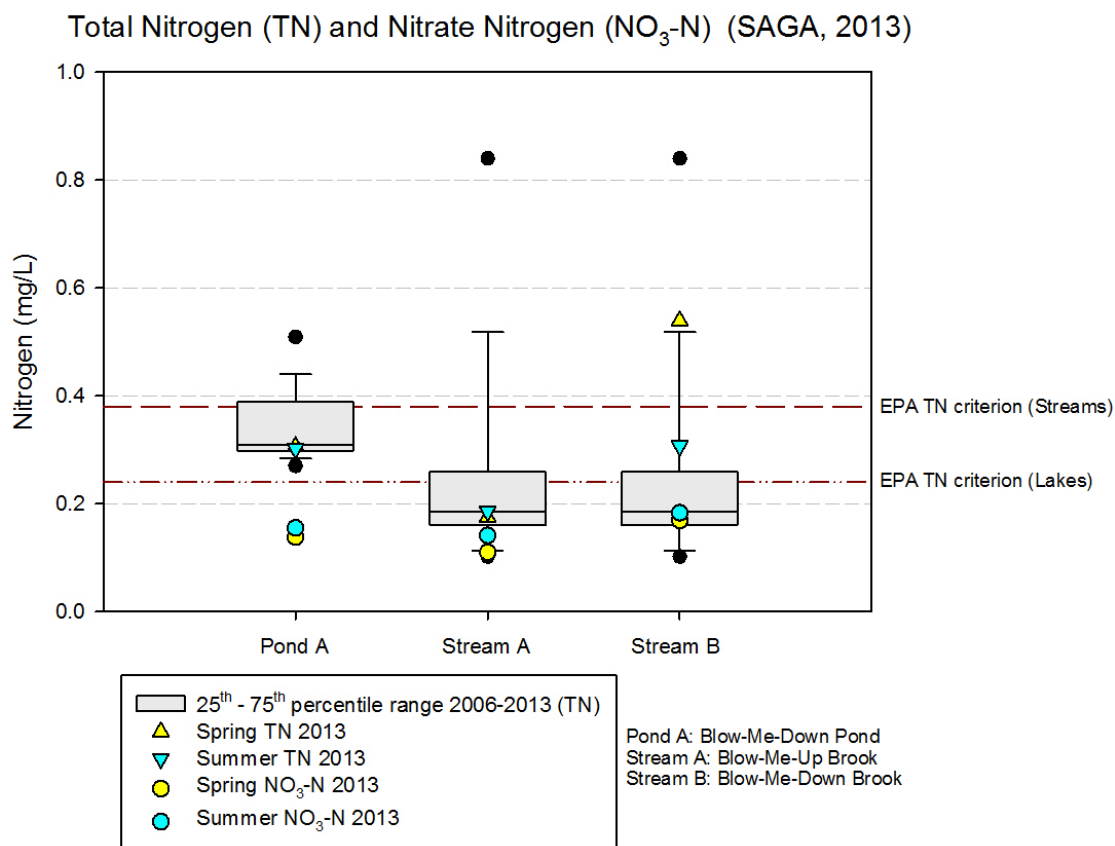
Figure 13. Total nitrogen (TN) and the nitrogen component of nitrate ( \text{NO}_3\text{-N} ) from 2013 water samples. The data are overlaid on a box plot of TN measurements taken from 2006-2013.
