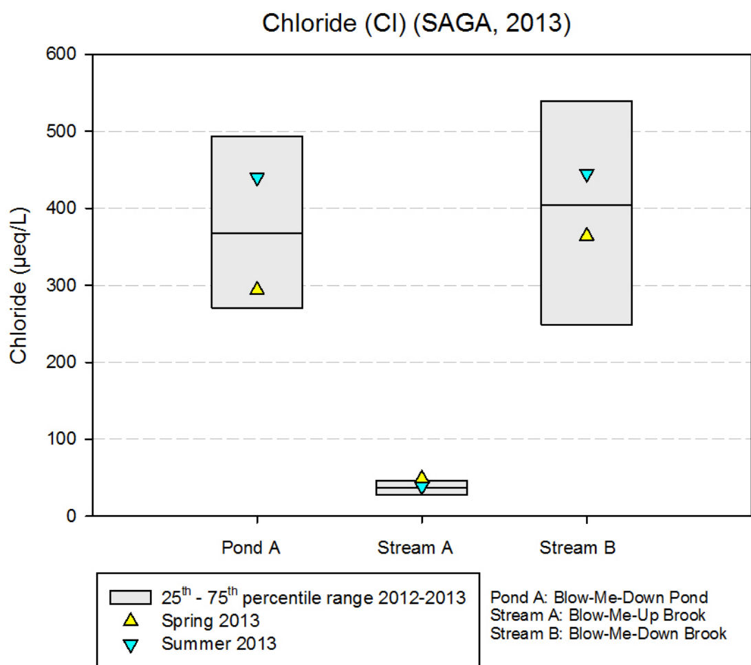
Figure 15. Chloride from 2012-2013 spring and summer water samples. The data are overlaid on a box plot of measurements taken from 2012-2013.
