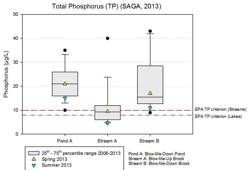
Figure 12. Total phosphorus (TP) from spring and summer water samples. The data are overlaid on a box plot of measurements taken from 2006-2013.
