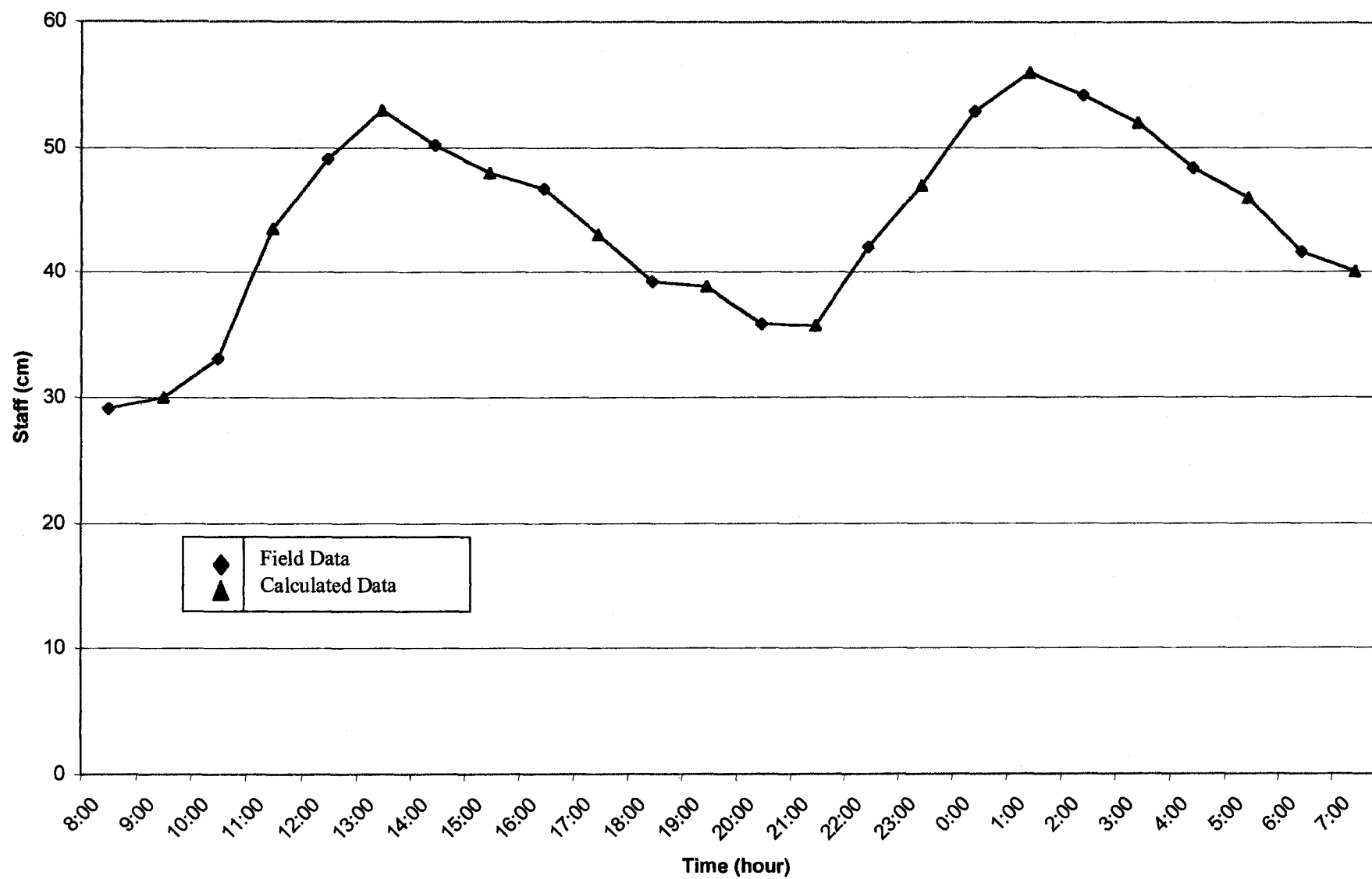
Figure 9. Control scrub December stage-time curve.
