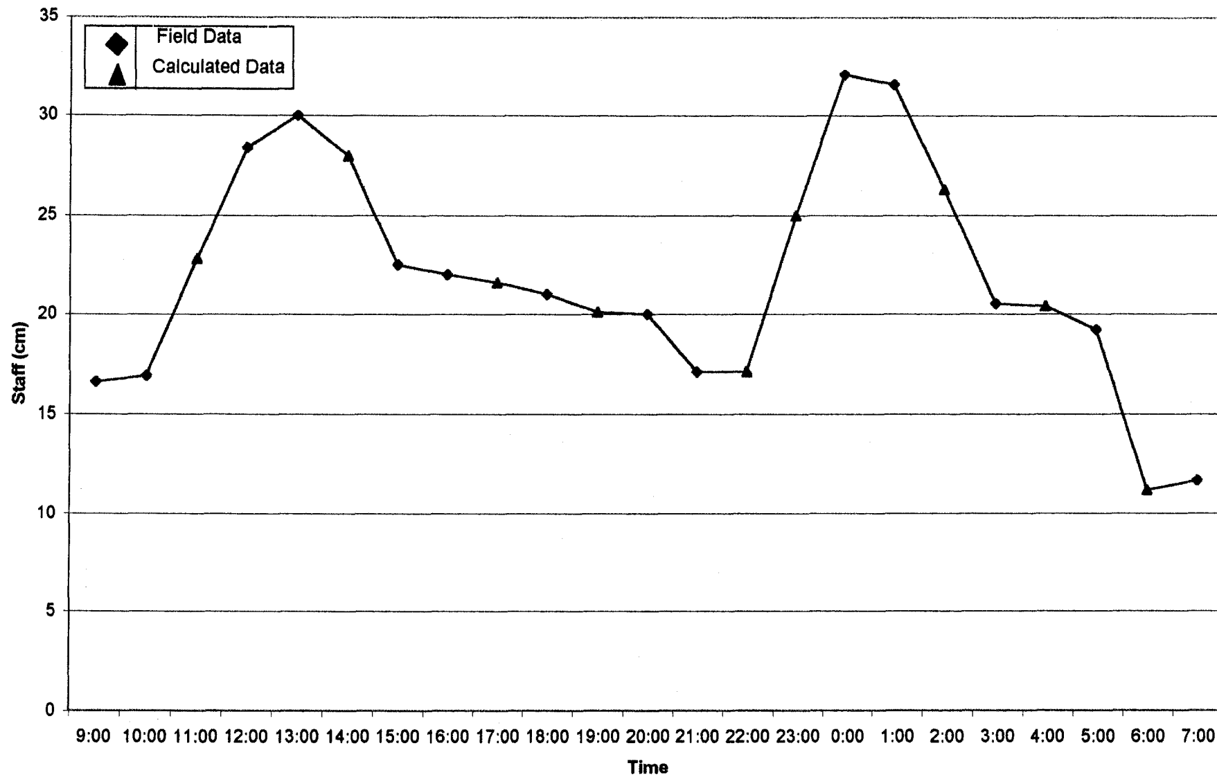
Figure 7. Treatment scrub December stage-time curve.
