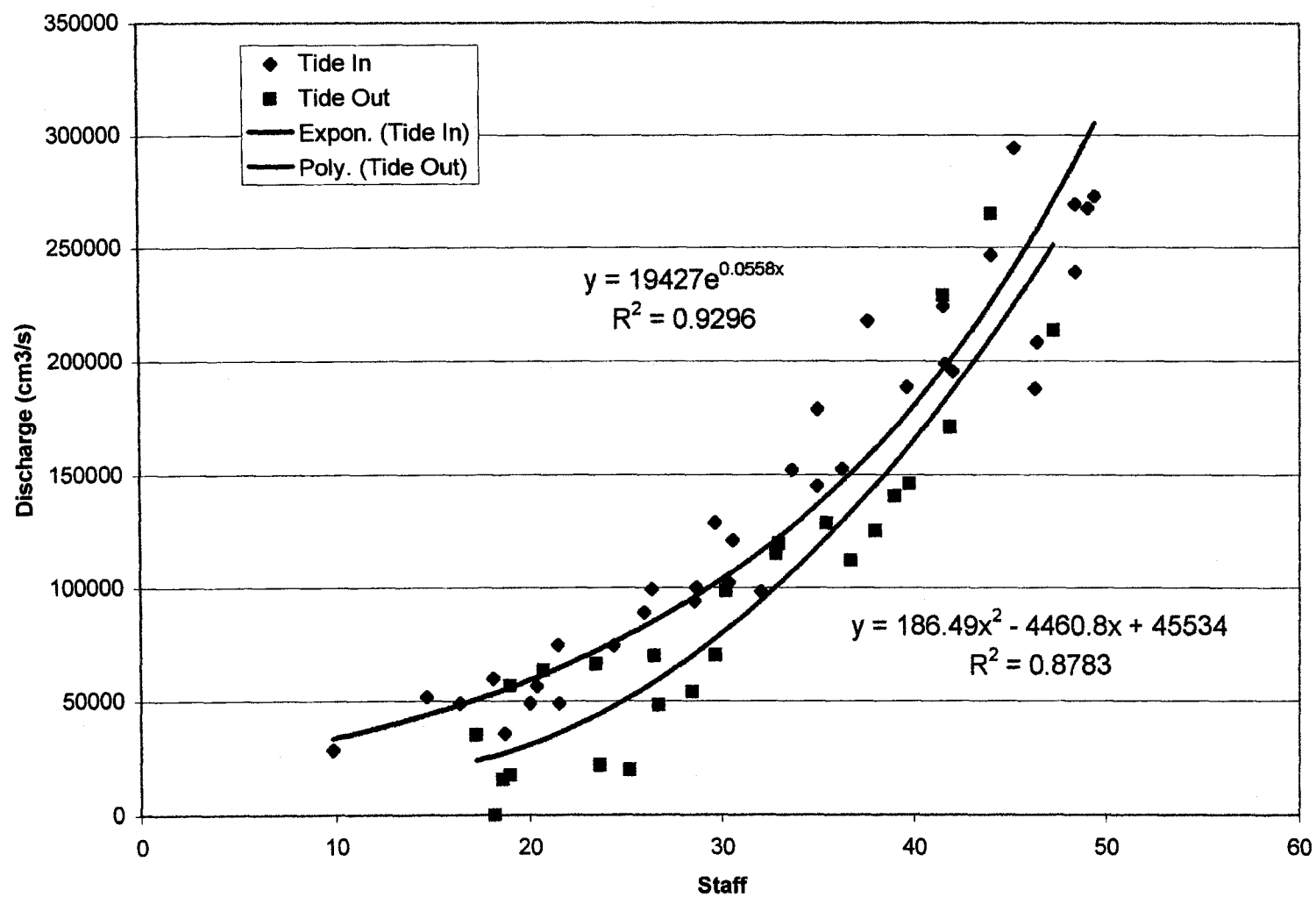
Figure 4. Control fringe stage-discharge curve for both rising and falling tides.
