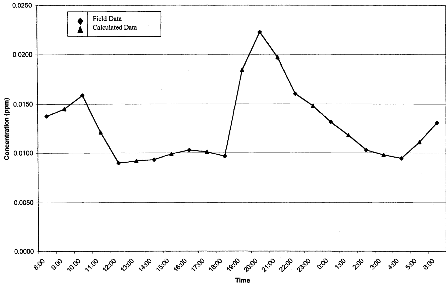
Figure 28. Treatment scrub December instantaneous \text{NH}_3 concentration-time plot.
