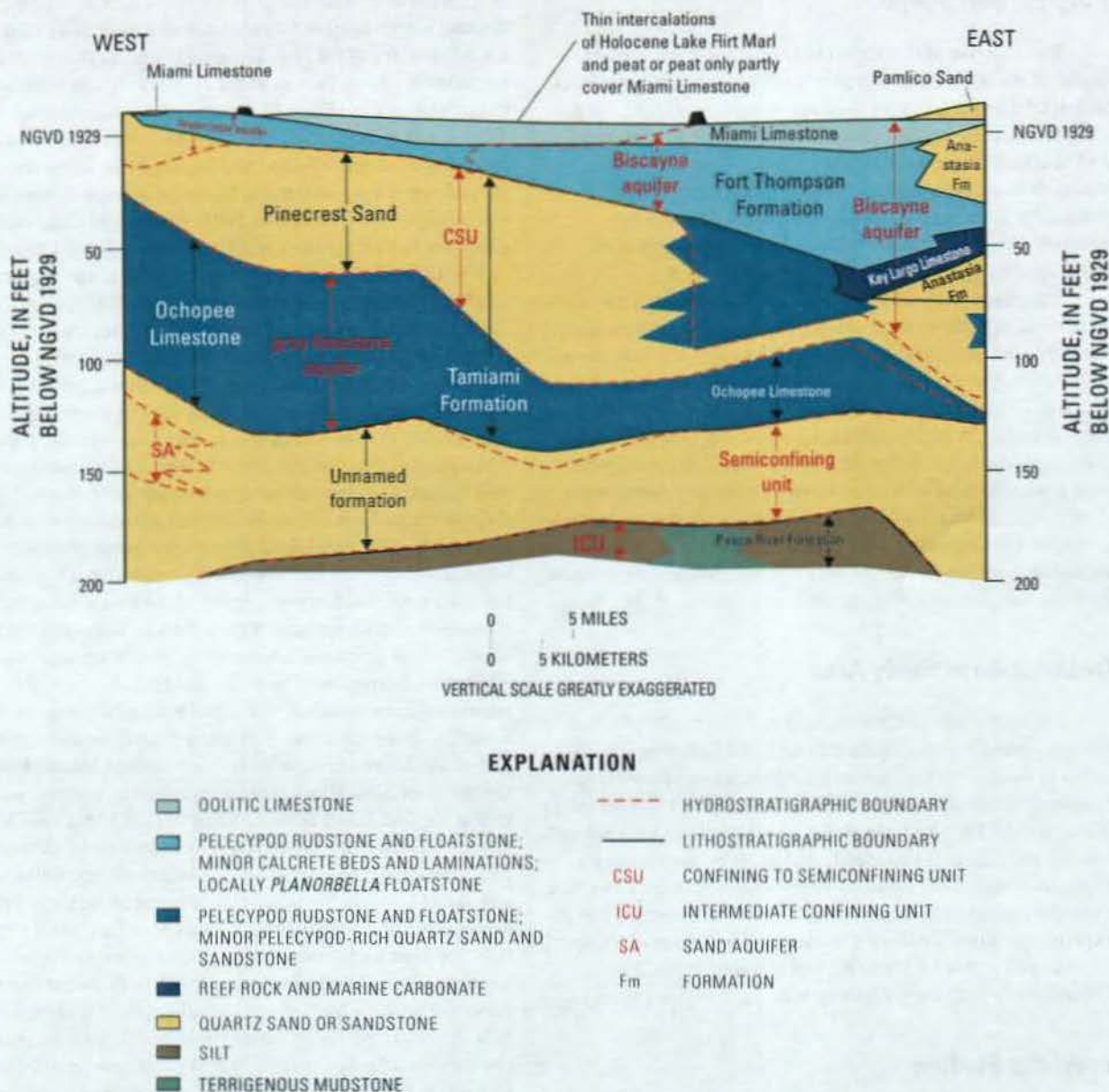
Figure 3. Relation of geologic and hydrogeologic units of the surficial aquifer system across central Miami-Dade County (modified from Reese and Cunningham, 2000).
