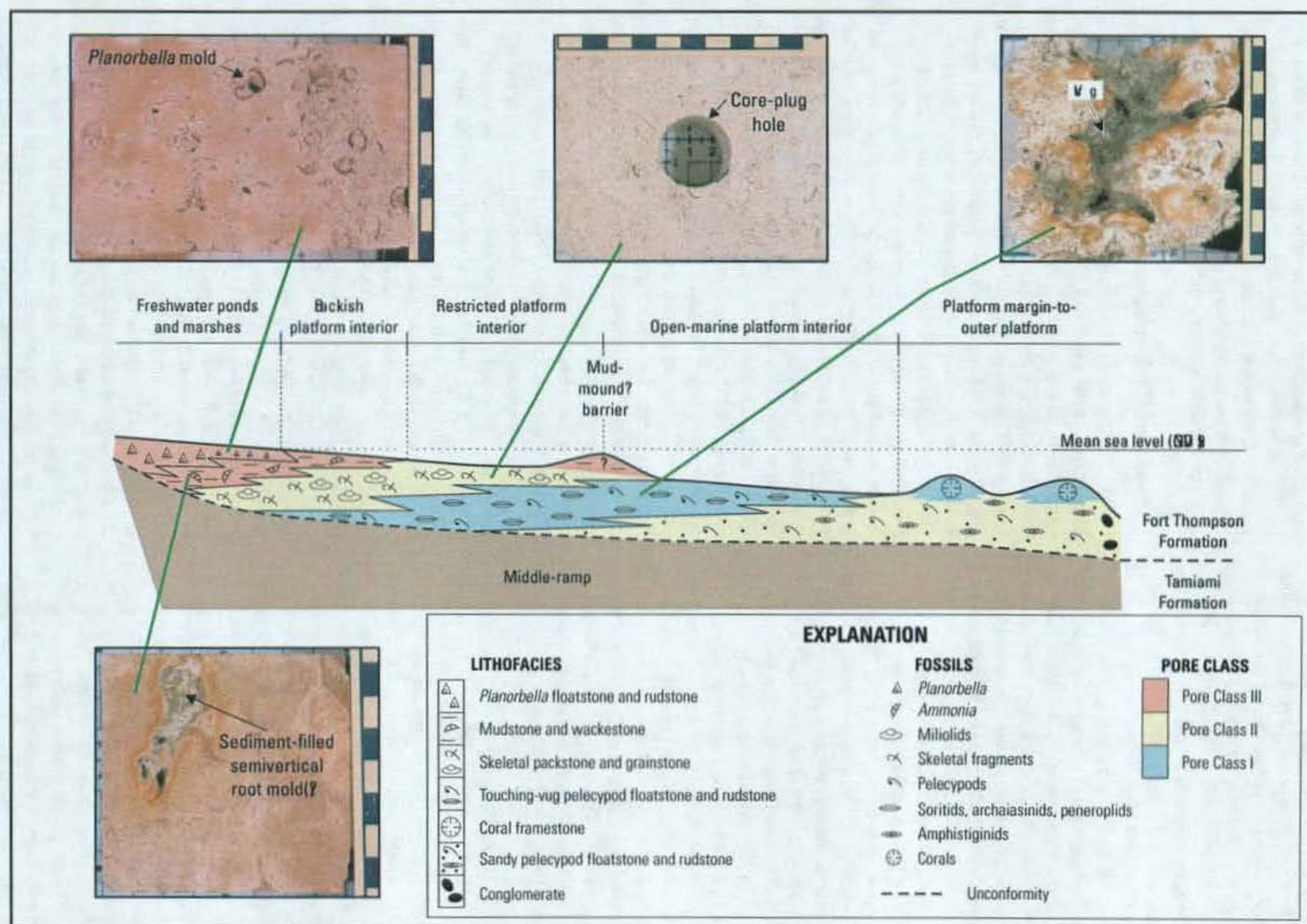
Figure 9. Conceptual facies model showing relations between major lithofacies, depositional environments, and pore classes for the study area. The four photographs of characteristic slabbed-core samples from the Fort Thompson Formation illustrate some of the carbonate textures and diagenetic features associated with key lithofacies. Each incremental color change represents 1 cm (0.394 in.) on the scale bars.
