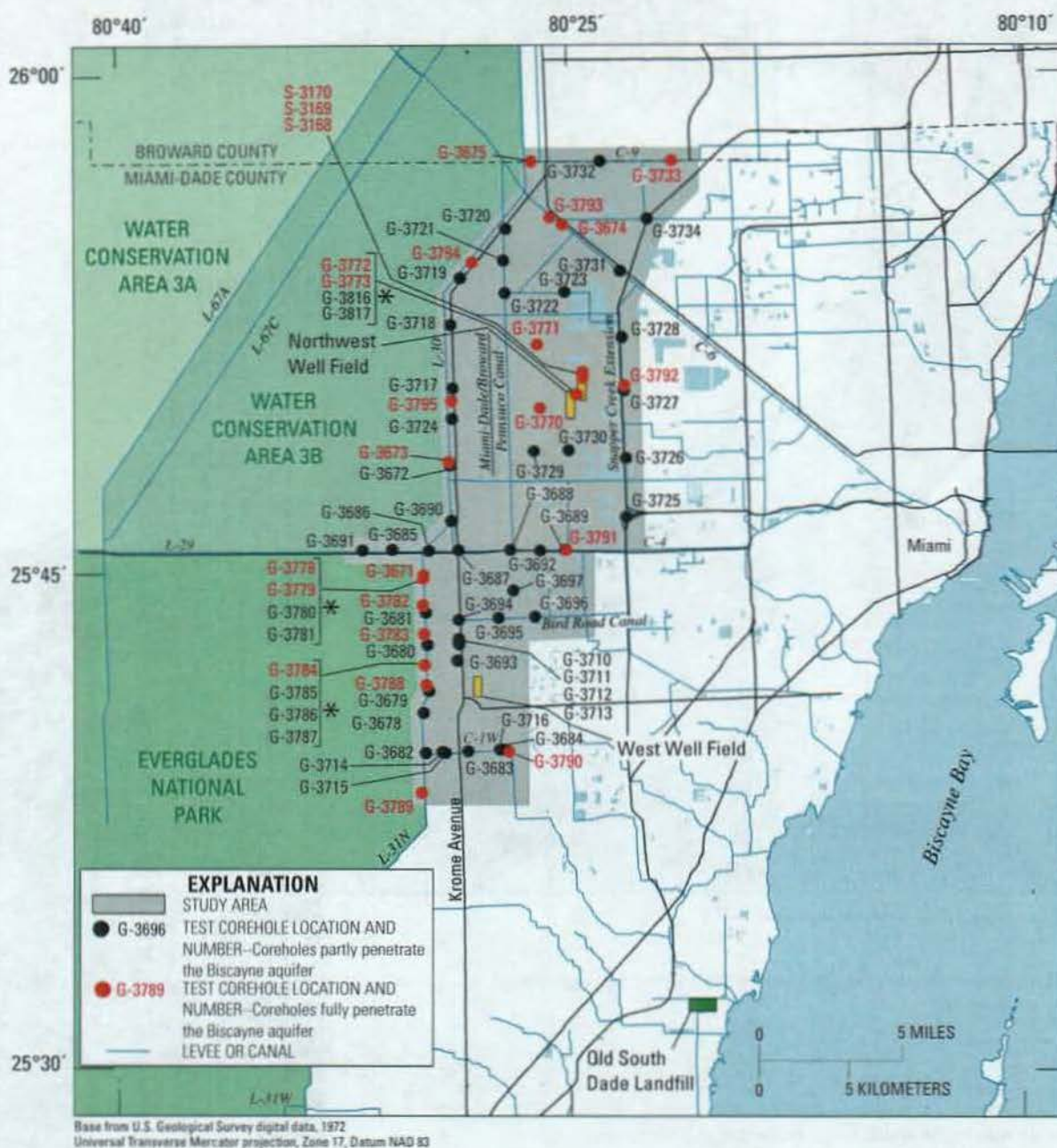
Figure 2. Study area in Miami-Dade County showing location of major canals and levees, Northwest Well Field, Old South Dade Landfill, and test coreholes used in this study. Asterisk indicates that some test coreholes are grouped together at the same location, and partly or fully penetrate the Biscayne aquifer.
