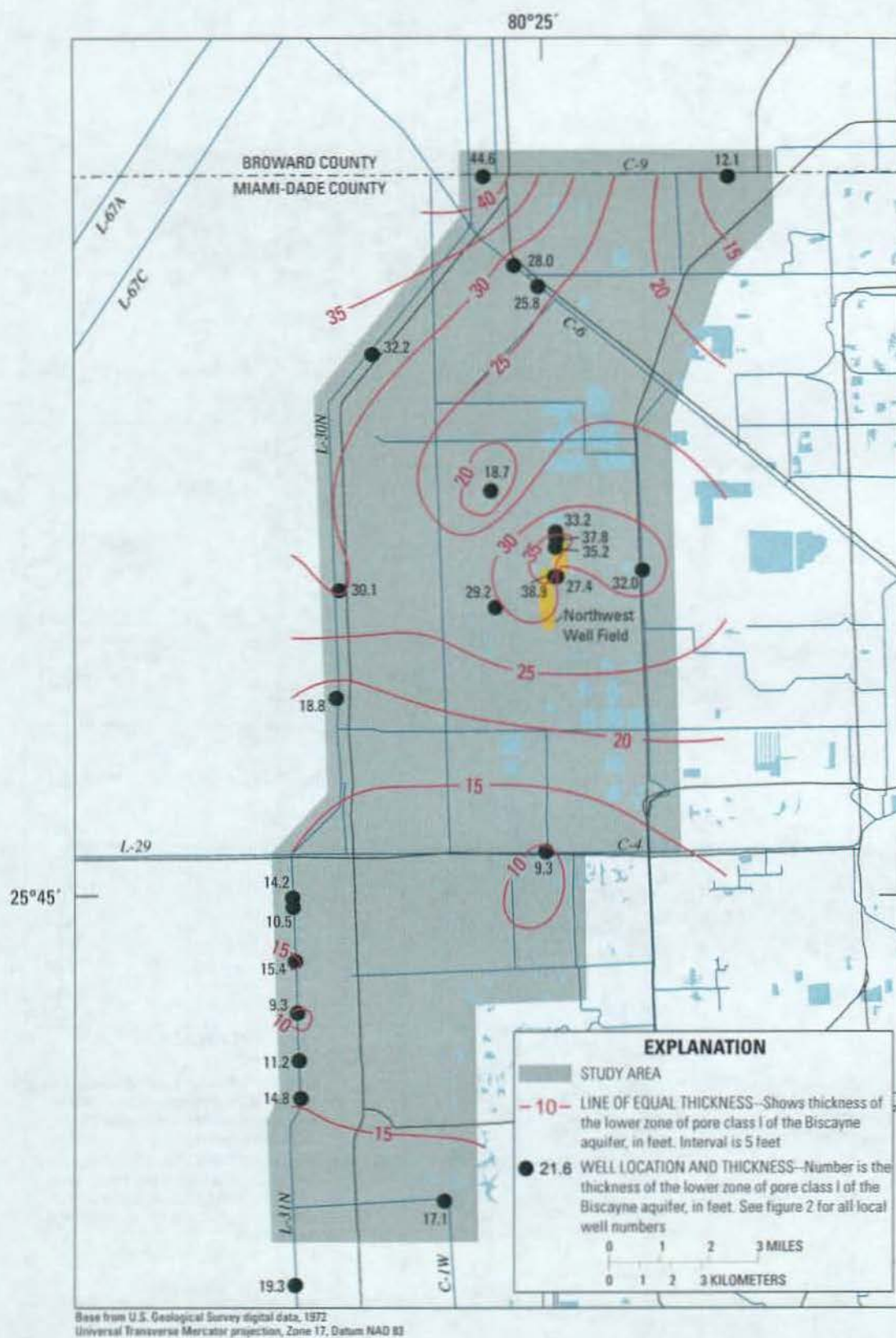
Figure 30. Thickness of the lower zone of pore class I of the Biscayne aquifer. This zone is shown as layer 8 in figure 15.
