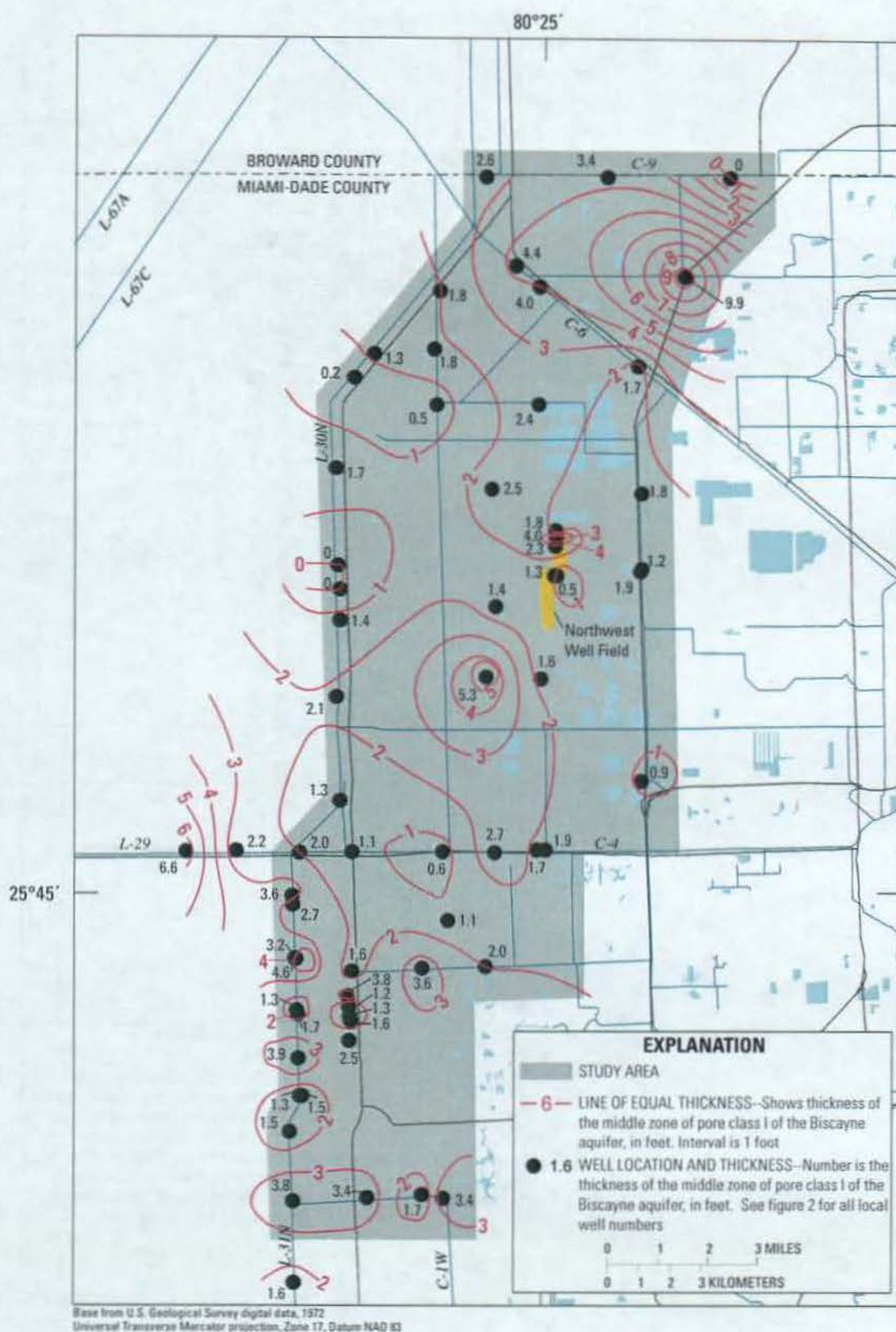
Figure 24. Thickness of the middle zone of pore class I of the Biscayne aquifer. This zone is shown as layer 5 in figure 15.
