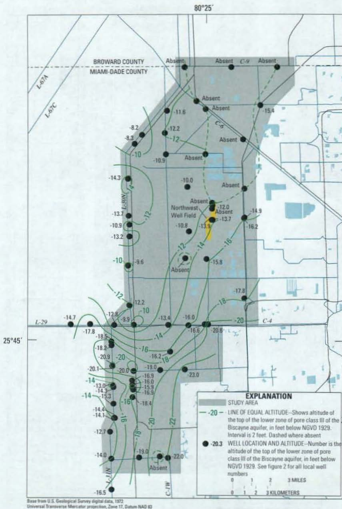
Figure 25. Altitude of the top of the lower zone of pore class III of the Biscayne aquifer. This zone is shown as layer 6 in figure 15.
