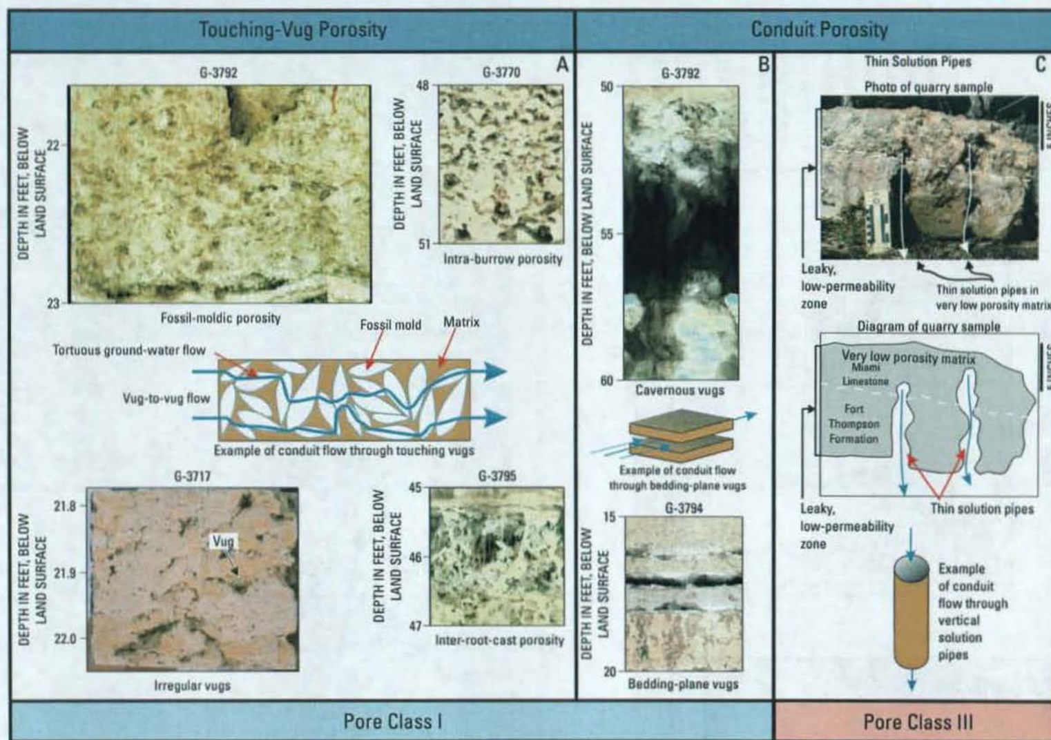
Figure 11. Relation between pore classes I and III and touching-vug and conduit pore types, respectively, for the Fort Thompson Formation and Miami Limestone of the Biscayne aquifer in the study area. (A) Four common types of touching-vug porosity: fossil moldic, intra-burrow, irregular vugs, and inter-root-cast porosity for pore class I; (B) Two types of conduit porosity (cavernous and bedding-plane vugs) that are rather untypical for pore class I; (C) Thin, vertical conduits that are a typical pore type of pore class III.
