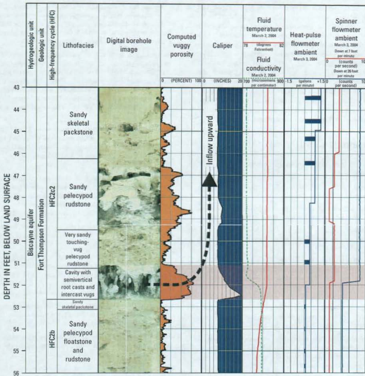
Figure 35. Comparison of borehole image, computed vuggy porosity, geophysical, and flowmeter logs showing evidence for inflow of ground water from a preferential flow zone into the borehole of the G-3793 test corehole. Most of the inflow seems to occur at a vuggy cavity at the base of HFC2c2 between the depths of about 51.1 and 52.7 feet below land surface (shaded in pale red).
