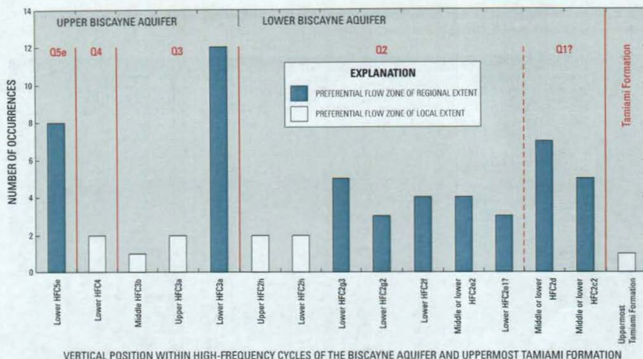
Figure 32. Number of occurrences of various preferential flow zones in 16 test coreholes fully penetrating the Biscayne aquifer in the study area, verified with heat-pulse or spinner flowmeter measurements, or both. Q units of Perkins (1977) also shown.
