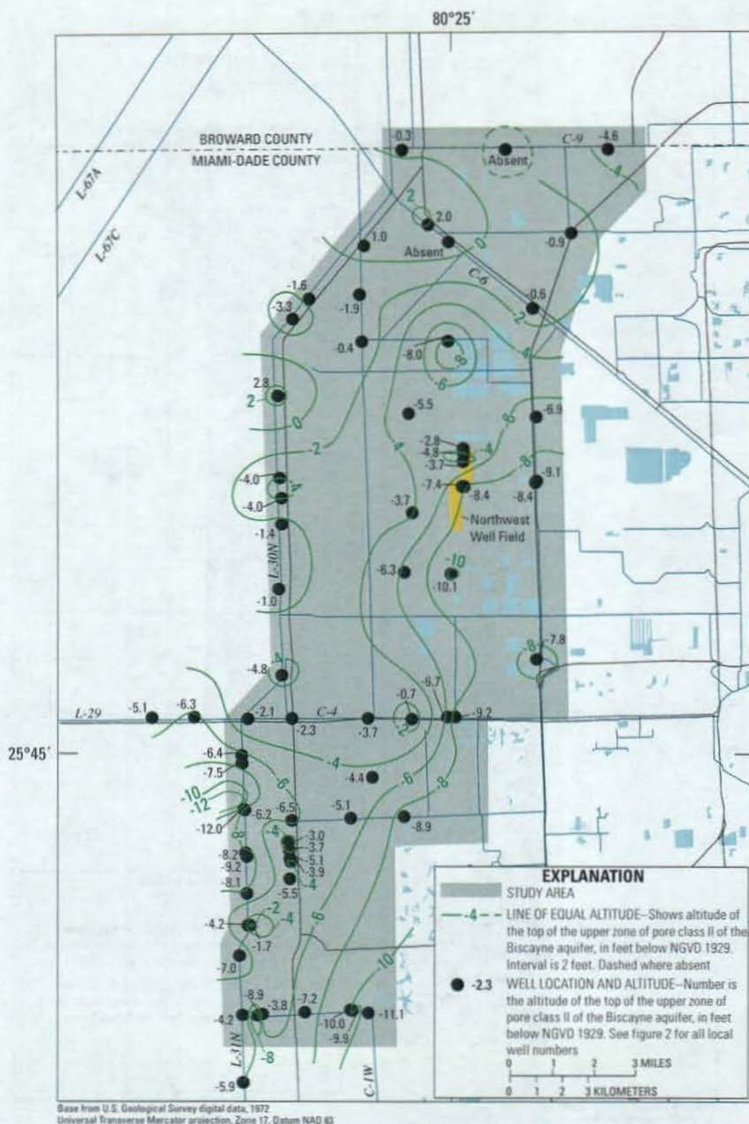
Figure 21. Altitude of the top of the upper zone of pore class II of the Biscayne aquifer. This zone is shown as layer 4 in figure 15.
