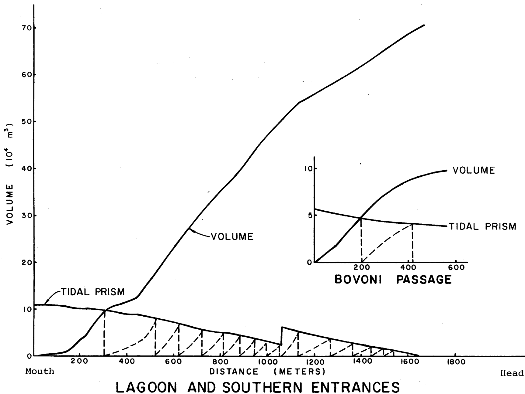
Figure 10. Accumulated volume and tidal prism of the Mangrove Lagoon.
