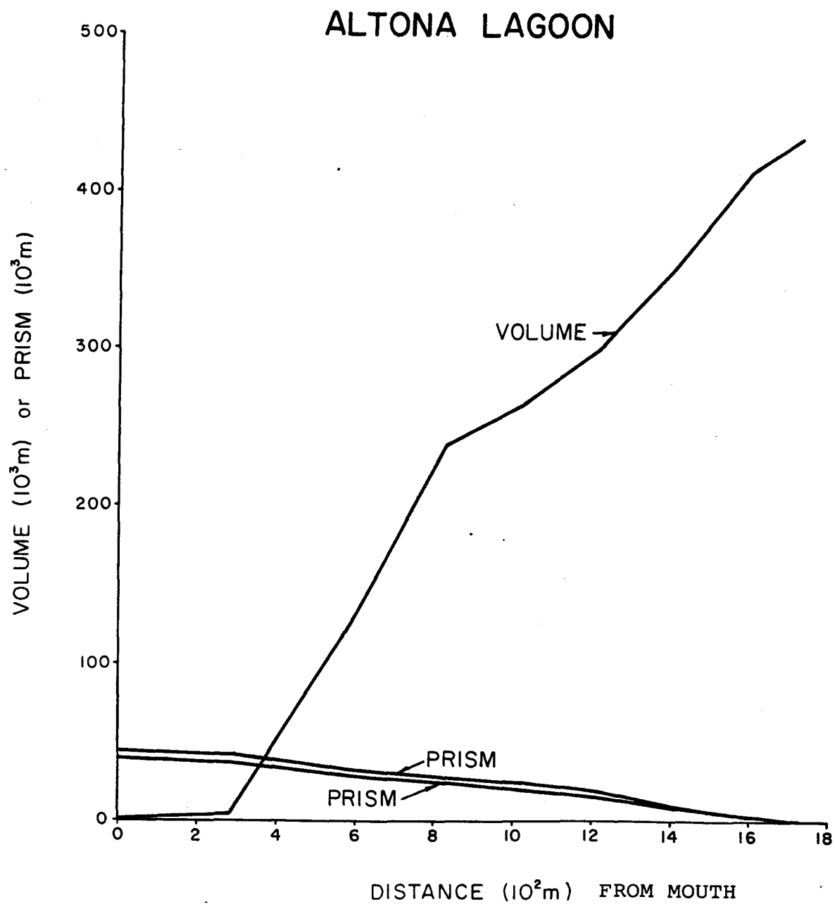
Figure 18. Accumulated volume and tidal prism of the Altona Lagoon.
