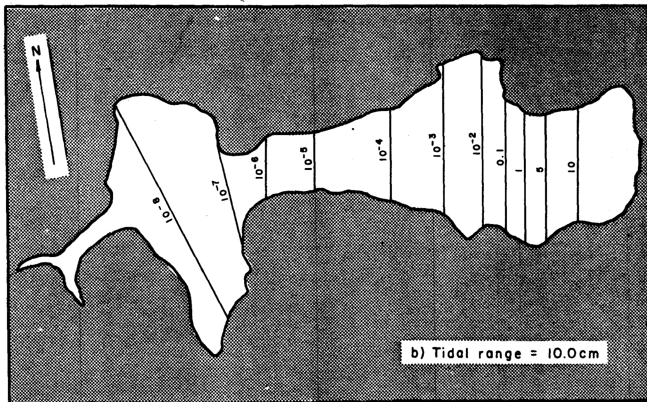
Figure 21. Pollution susceptibility of the Altona Lagoon for a nonconservative pollutant, decay rate = 1.0/tidal cycle, source = 1000 kg/tidal cycle, concentration in mg/l. A. upper for 8.8 cm tide range, B. lower for 10.0 cm tide range. Numbers in segments are average concentrations in mg/l.
