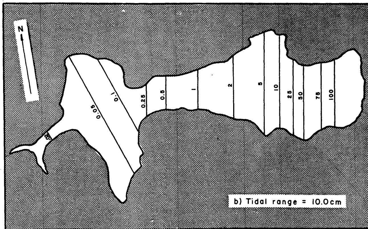
Figure 20. Pollution susceptibility of the Altona Lagoon for a nonconservative pollutant, decay rate = 0.1/tidal cycle, source = 1000 kg/tidal cycle, concentration in mg/l. A. upper, for 8.8 cm tide range; and B. lower, for 10.0 cm tide range. Numbers in segments are average concentrations in mg/l.
