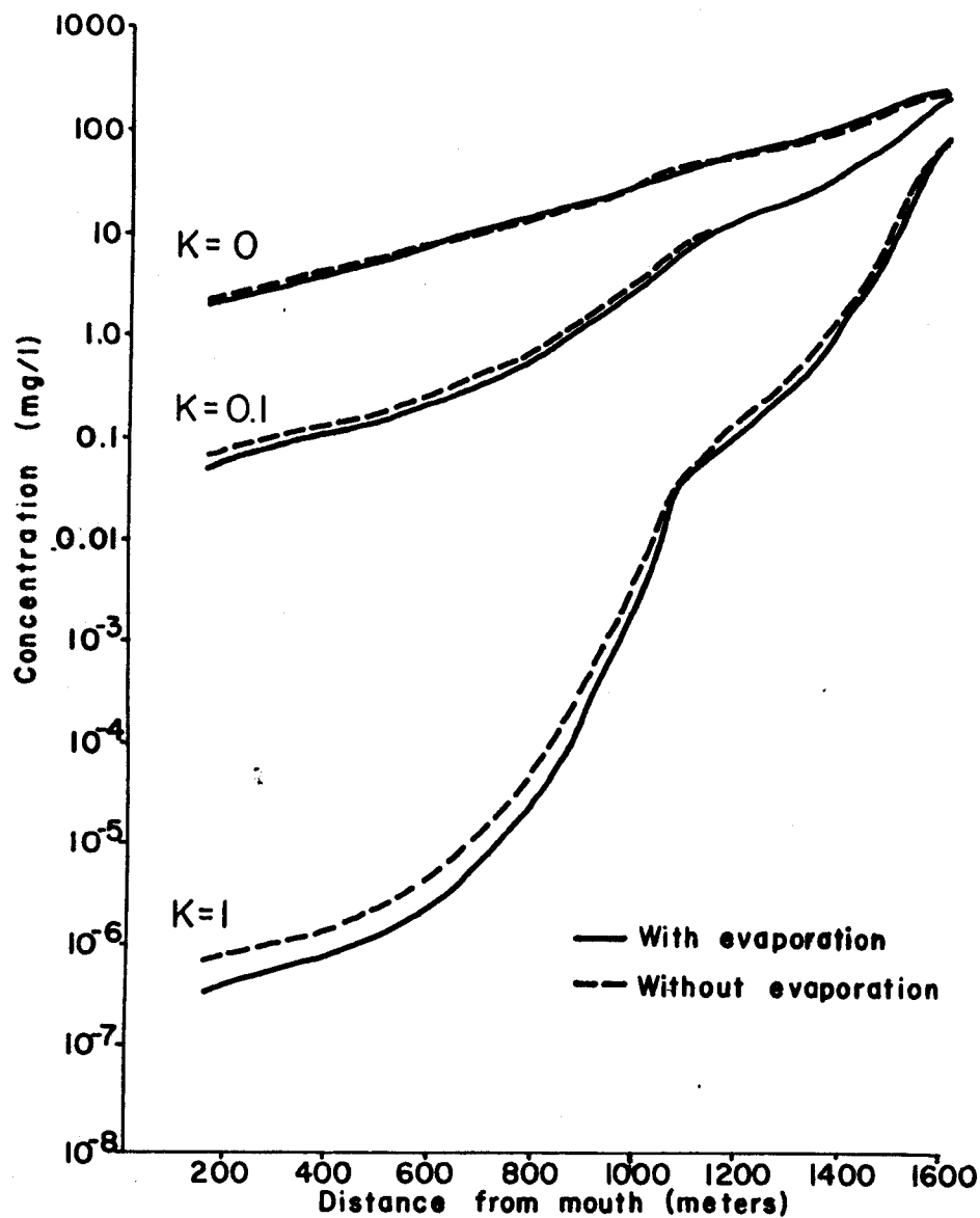
A3. Comparison of pollution susceptibility of the Mangrove Lagoon with and without evaporation. k is the decay rate, \frac{1}{\text{day}} .
