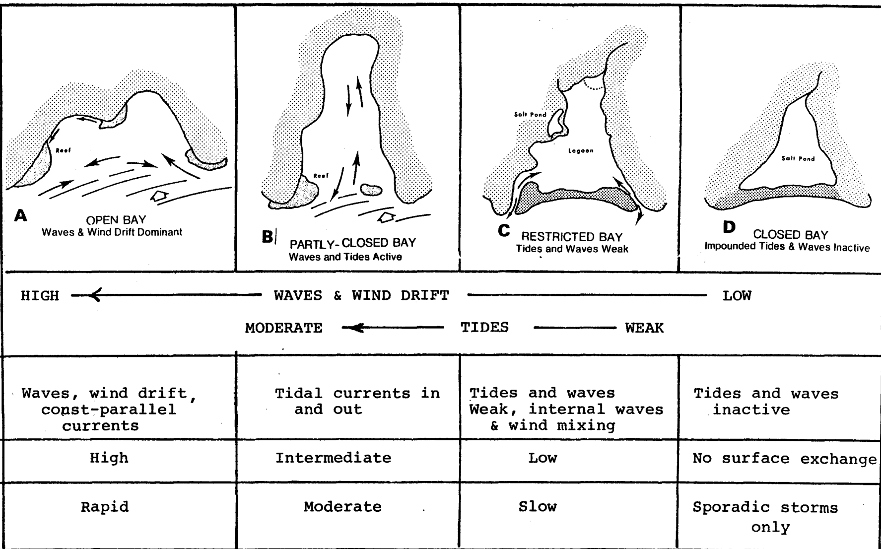
Figure 1. Different types of Virgin Island bays in a sequence organized according to closure, dominate processes and flushing efficiency.
