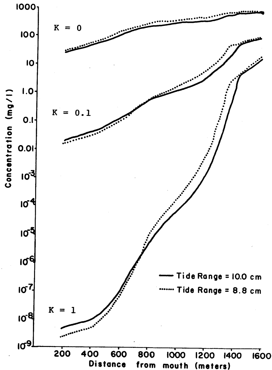
A6. Comparison of pollution susceptibility of the Altona Lagoon with tidal ranges of 8.8 cm and 10.0 cm.
