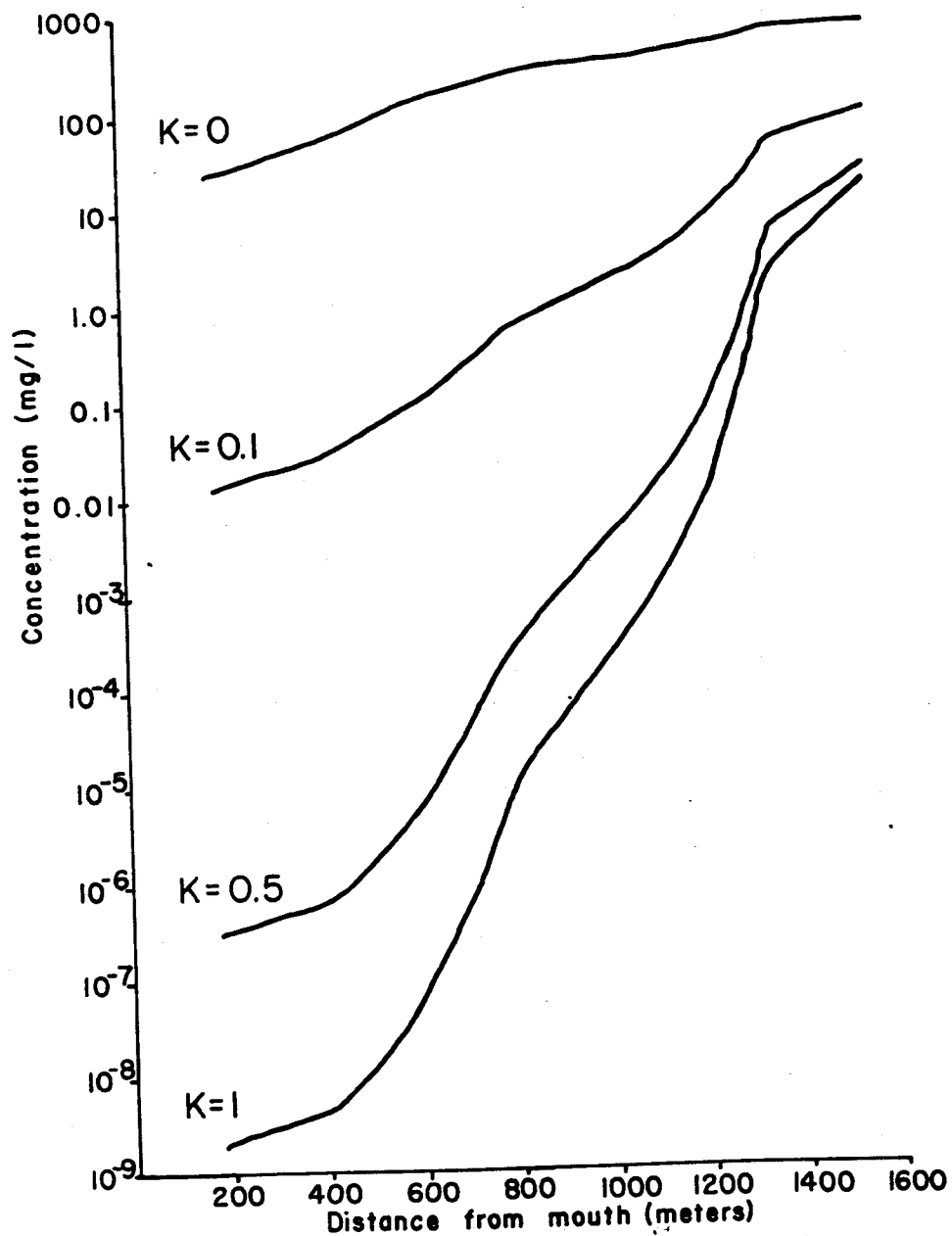
A7. Pollution susceptibility of the Altona Lagoon with tidal range of 8.8 cm. k is the decay rate.
