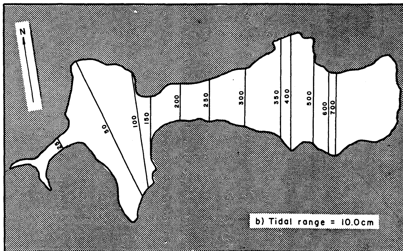
Figure 19. Pollution susceptibility of the Altona Lagoon for a conservative pollutant, source = 1000 kg/tidal cycle, concentration in mg/l. A. upper for 8.8 cm tide range; B. lower for 10.0 cm tide range. Numbers in segments are average concentrations in mg/l.
