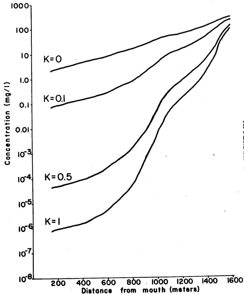
A2. Pollution susceptibility of the Mangrove Lagoon with pollutant discharged at the lagoon head, without evaporation. k is the decay rate, \frac{1}{\text{day}} .
