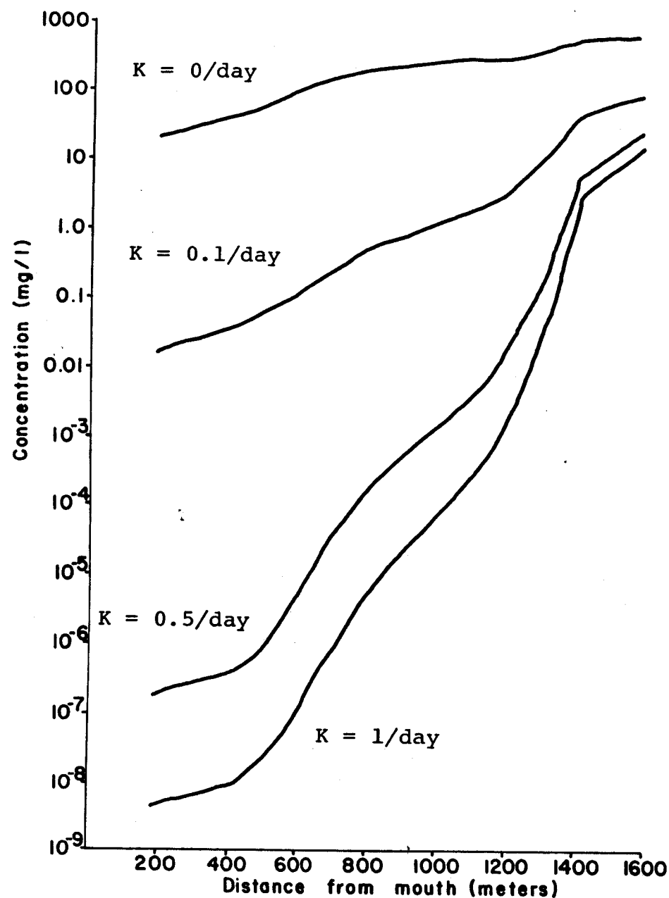
A5. Pollution susceptibility of the Altona Lagoon with tidal range of 10.0 cm.
