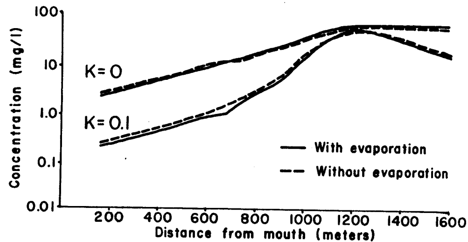
A4. Pollution susceptibility of the Mangrove Lagoon with pollutant discharged from the Turpentine Run, with and without evaporation.
