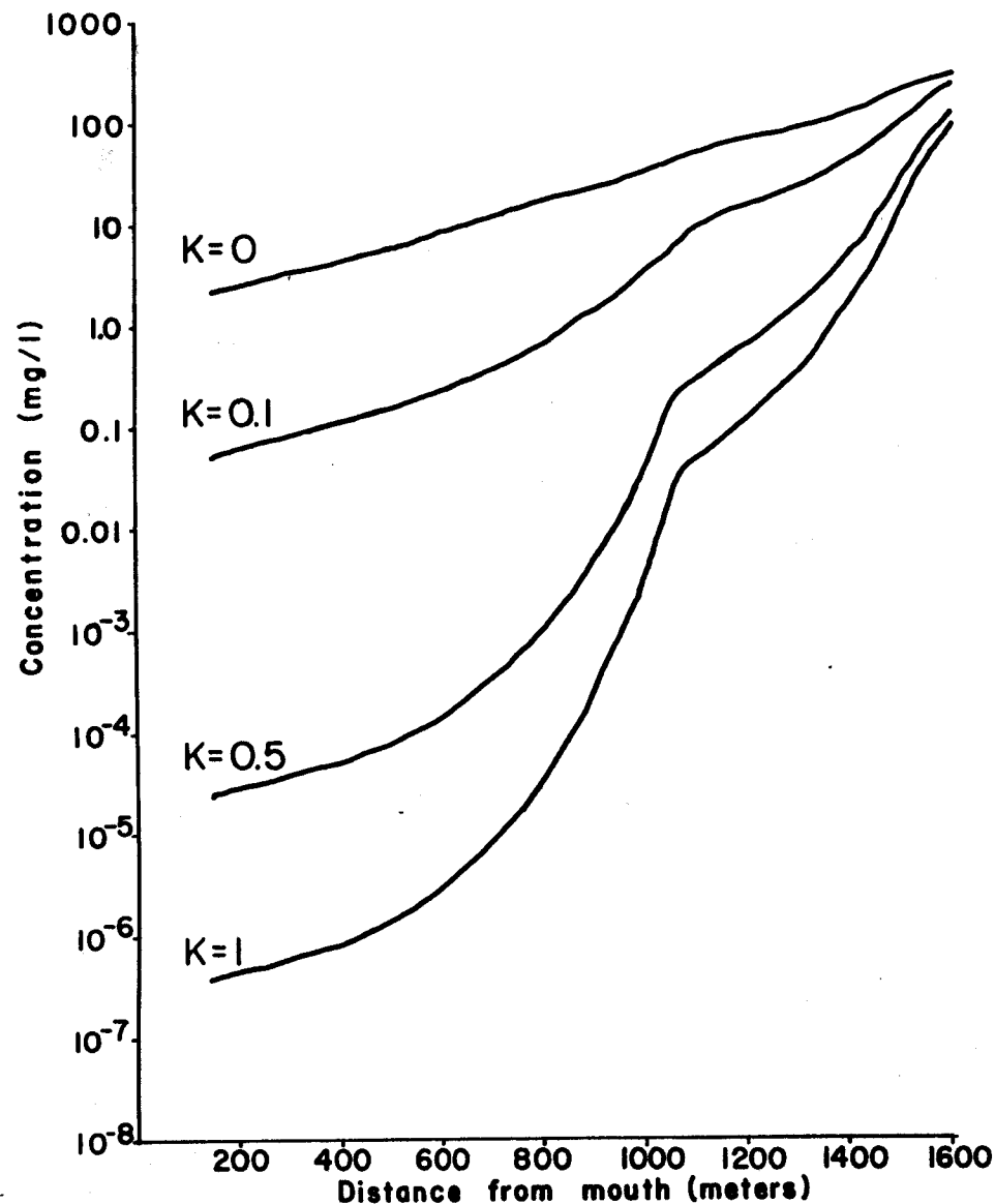
A1. Pollution susceptibility of the Mangrove Lagoon with pollutant discharged at the lagoon head, with evaporation.
