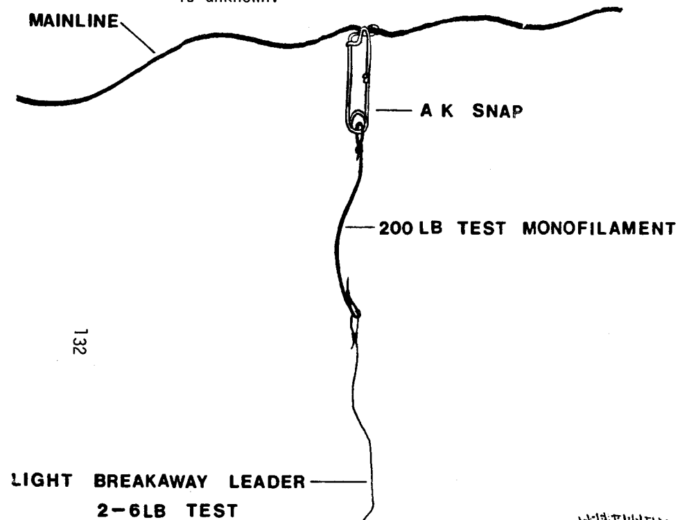
Figure 4. Break away tag hook-up on main line, construction, and tagged fish. Note, proportion of main gangion material (200 lb. test monofilament) accounts for about 90% of total gangion length. Hook retention time is unknown.
