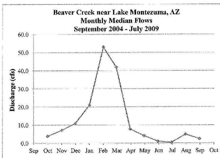
Figure 6. Beaver Creek monthly median discharge developed from Beaver Creek near Lake Montezuma, AZ discharge data and requested in the application.
