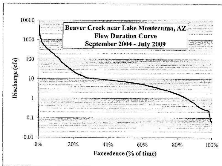
Figure 5. Flow Duration Curve calculated for the Beaver Creek near Lake Montezuma, AZ gage, September 2004 – July 2009.
