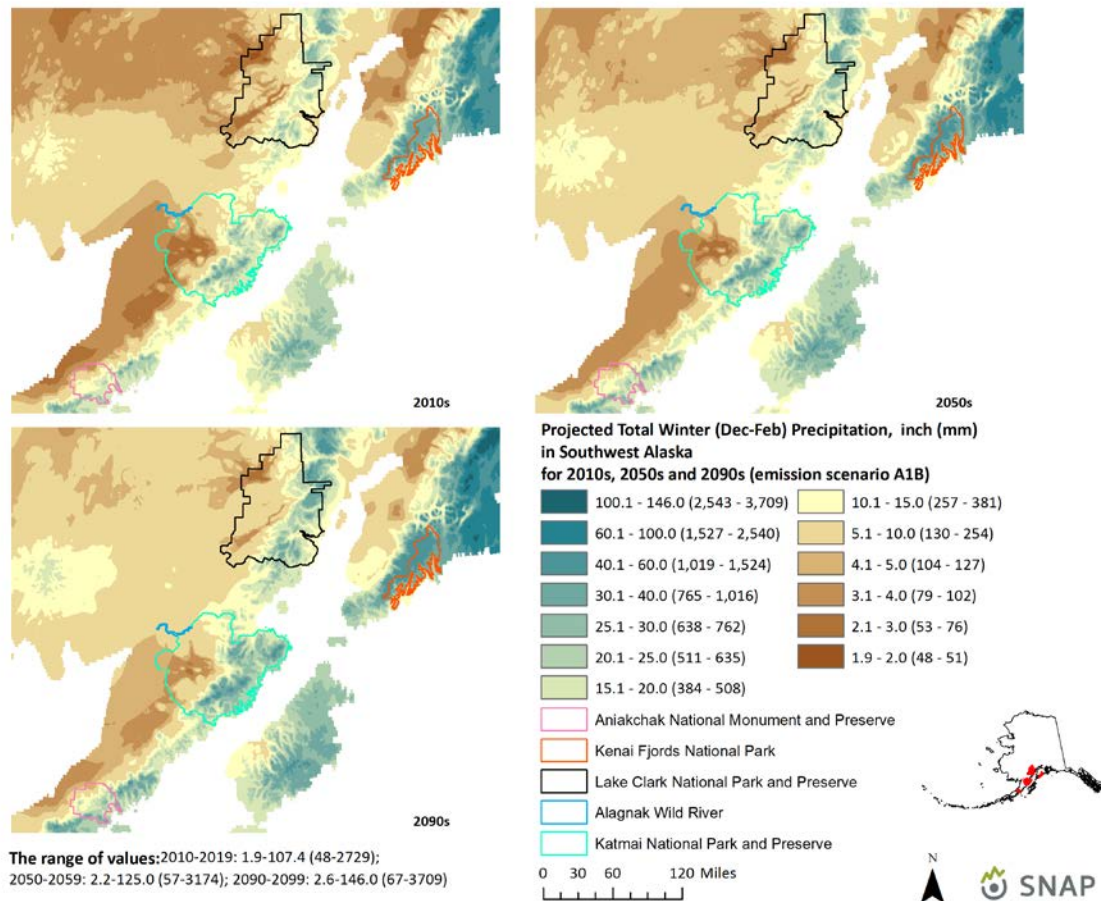
Figure 7: Mean winter precipitation. These maps show the projected precipitation for December, January, and February for selected decades. Although increased precipitation is expected, warmer temperatures may result in less snow. For additional maps, see Appendix E.
