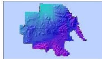
Total Annual Precipitation (inches)
