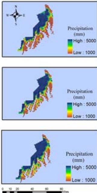
Total Annual Precipitation
