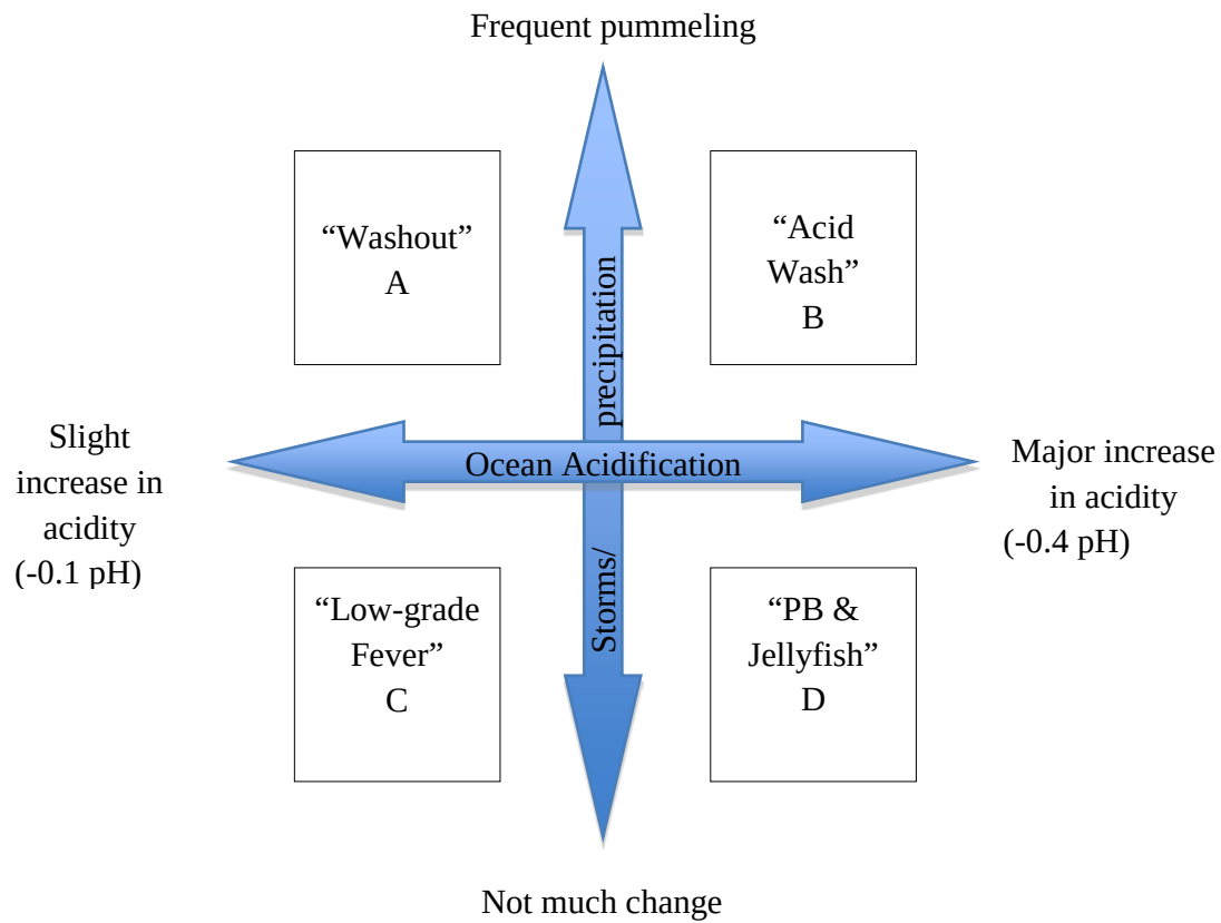
Figure 9: Matrix showing the intersection of changes in storms and precipitation and changes in ocean acidification, as each pertains to coastal regions. Each quadrant yields a set of future conditions which are plausible, challenging, relevant, and divergent. The details of each quadrant are described in the text.
