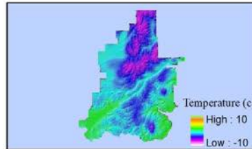
Average Annual Temperature (C)
