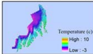
Average Annual Temperature (C)
