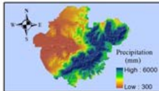
Total Annual Precipitation
