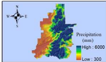
Total Annual Precipitation
