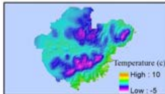
Average Annual Temperature (C)
