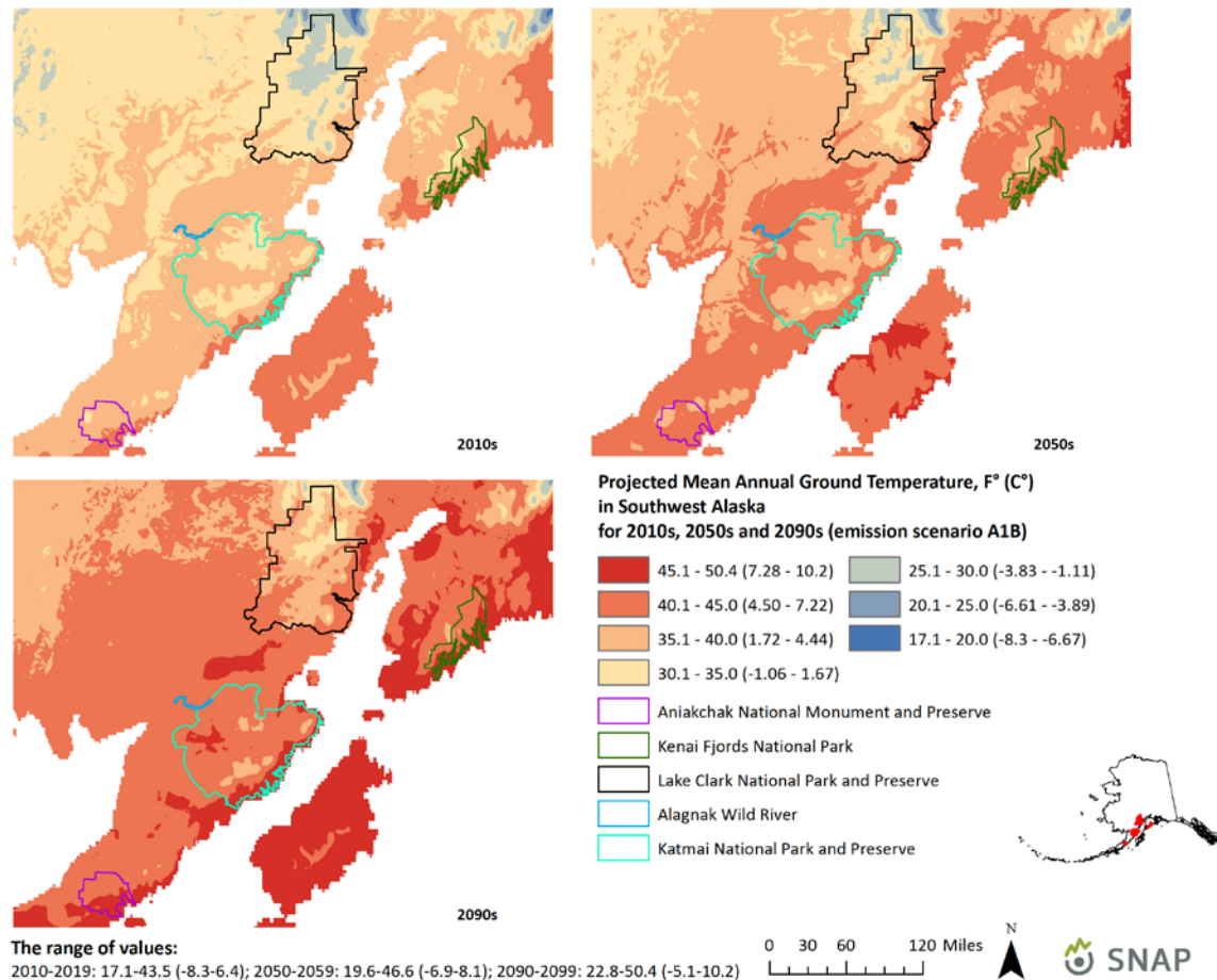
Figure 8: Mean annual ground temperature at one meter depth. Based on SNAP climate data and GIPL permafrost modeling, these maps depict likely ground temperature conditions. Widespread loss of frozen ground is likely by the end of the century.
