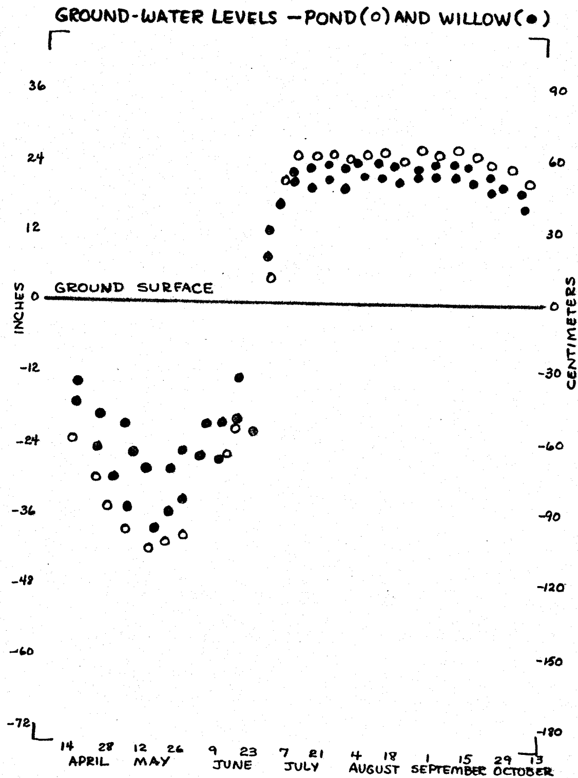
FIGURE 8 CHANGES IN GROUND WATER LEVELS AT THE POND AND WILLOW SITES
