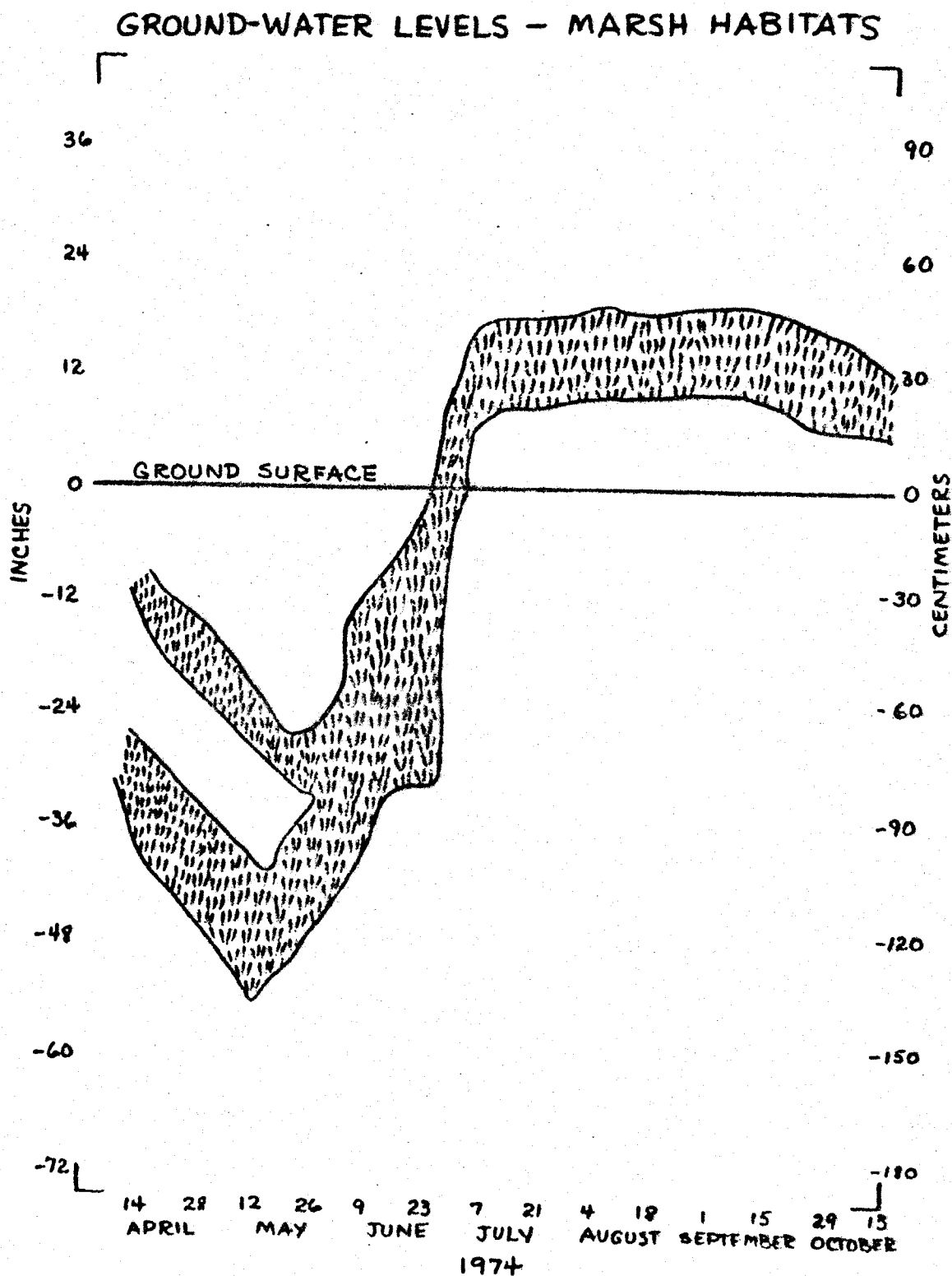
FIGURE 10 CHANGES IN GROUND WATER LEVELS IN THE MARSH HABITATS
