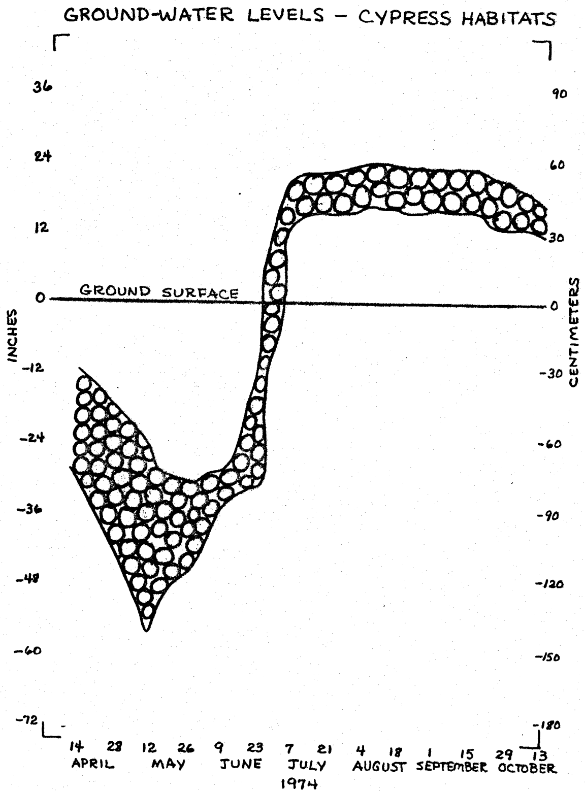
FIGURE 11 CHANGES IN GROUND WATER LEVELS AT THE CYPRESS HABITATS
