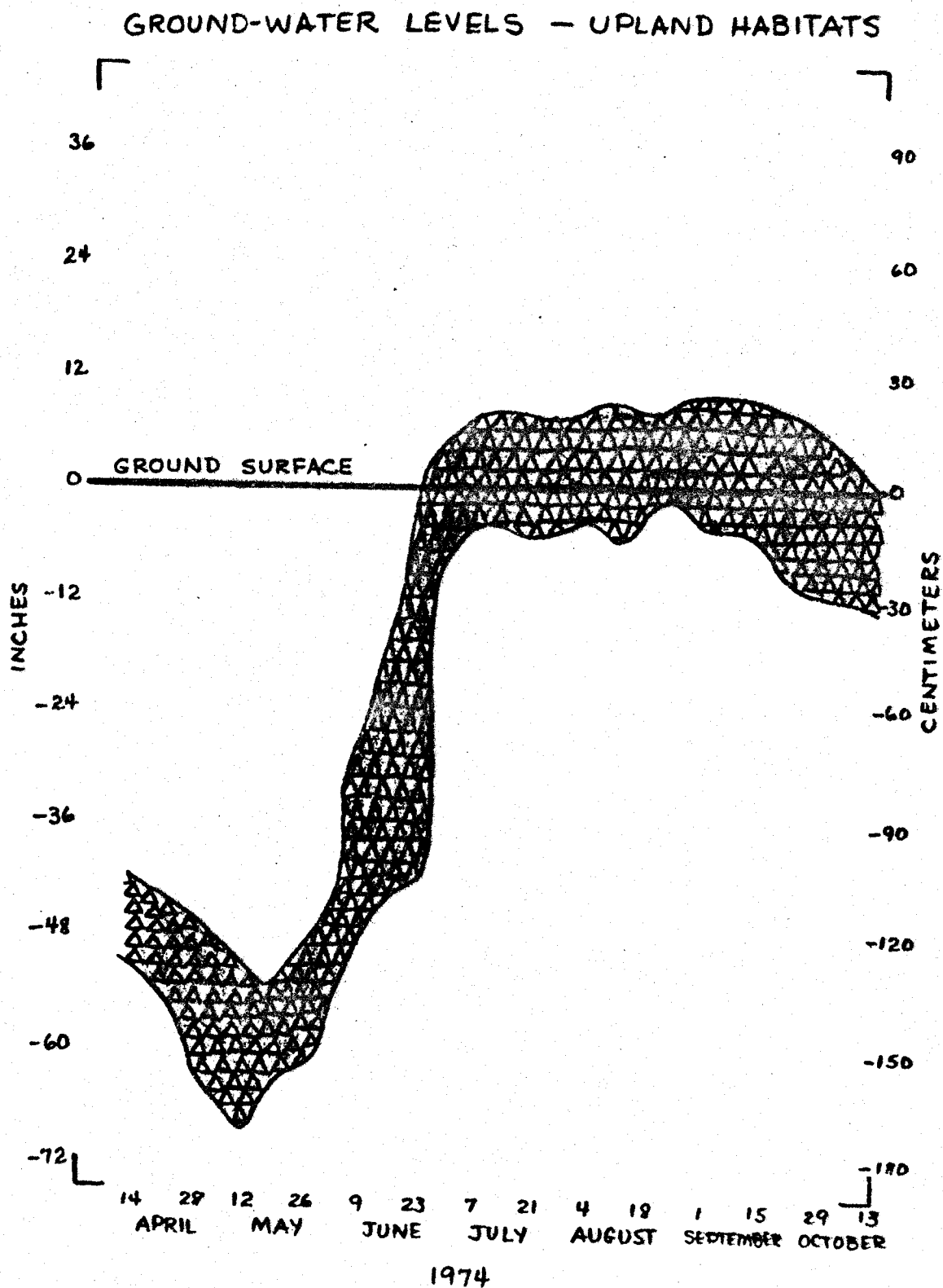
FIGURE 9 CHANGES IN GROUND WATER LEVELS AT THE UPLAND HABITATS
