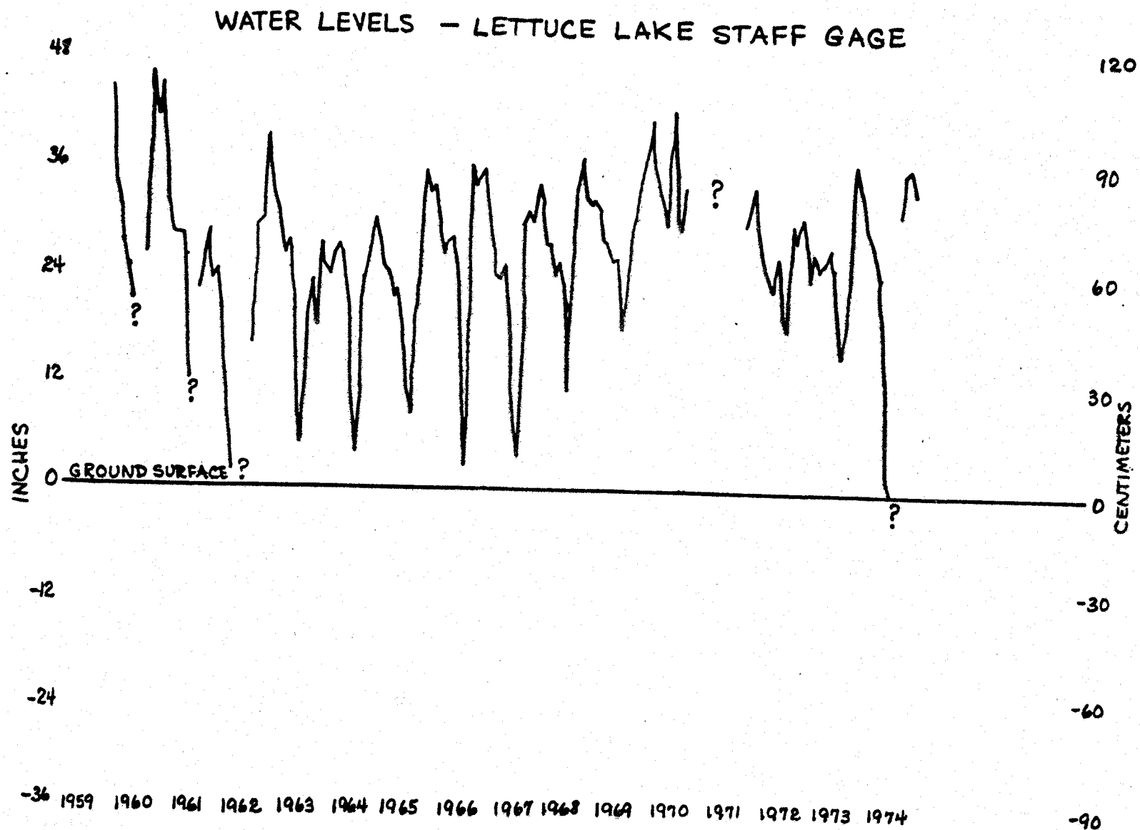
FIGURE 6 CHANGES IN THE WATER LEVEL AT LETTUCE LAKE
