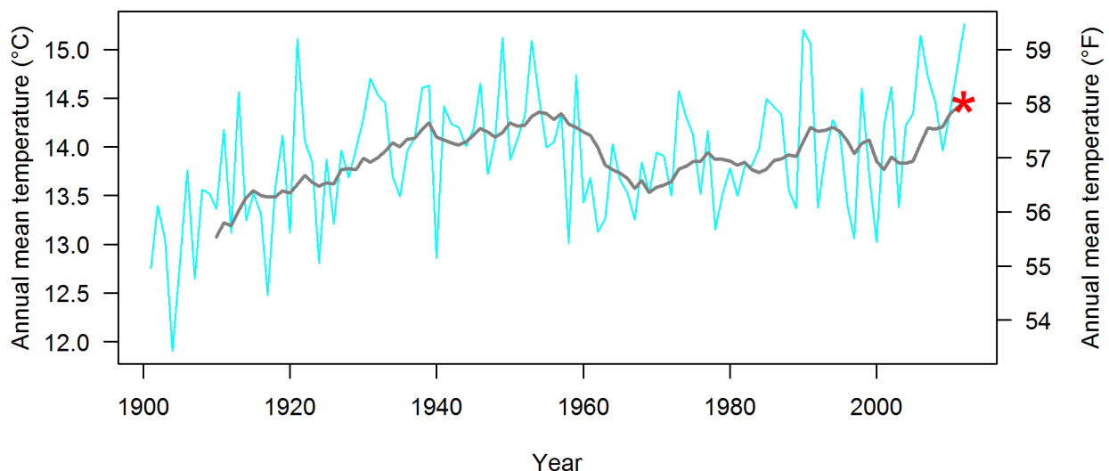
Figure 1. Time series used to characterize the historical range of variability and most recent percentile for annual mean temperature at Thomas Stone National Historic Site (including areas within 30-km [18.6-mi] of the park’s boundary). The blue line shows temperature for each year, the gray line shows temperature averaged over progressive 10-year intervals (10-year moving windows), and the red asterisk shows the average temperature of the most recent 10-year moving window (2003–2012). The most recent percentile is calculated as the percentage of values on the gray line that fall below the red asterisk (see results of most recent percentiles for all temperature and precipitation variables in Figure 2).
