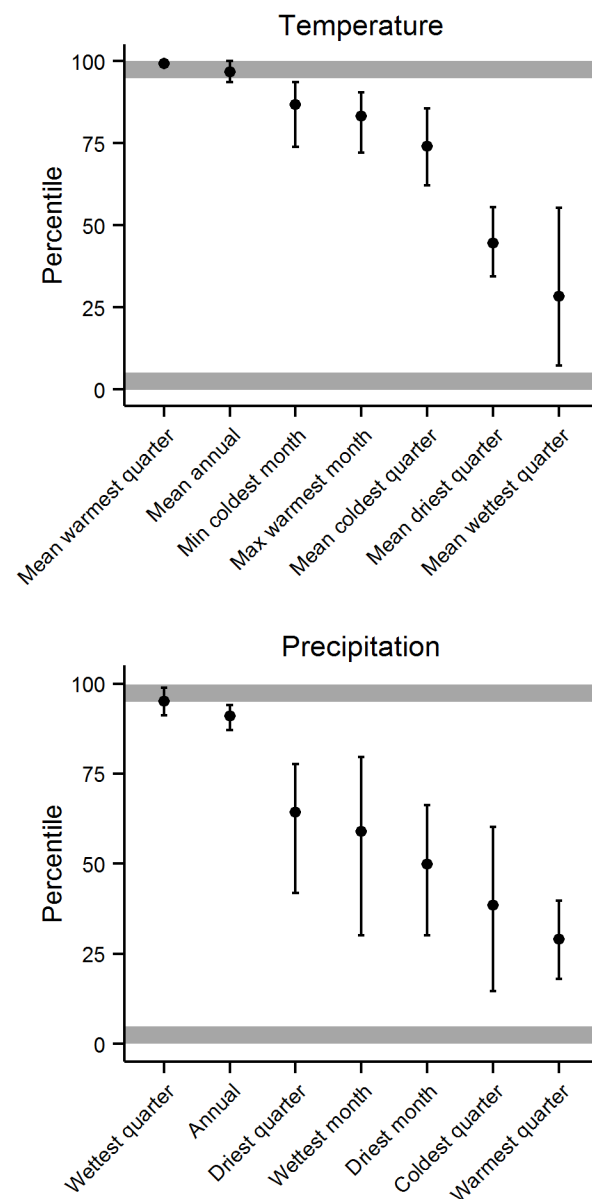
Figure 2. Recent temperature and precipitation percentiles at Thomas Stone National Historic Site (including areas within 30-km [18.6-mi] of the park’s boundary). Black dots indicate average recent percentiles across the 10, 20, and 30-year intervals (moving windows). Variables are considered “extreme” if the mean percentiles are <5 th percentile or >95 th percentile (i.e., the gray zones, where recent climate is pushing the limits of all observed climates since the year 1901). Black bars indicate the range of recent percentiles across 10, 20, and 30-year moving windows (larger bars indicate higher sensitivity to moving window size).
