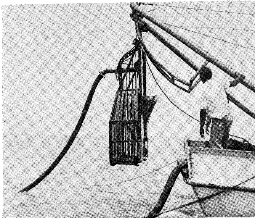
Figure 3. The 27-inch Nantucket dredge.
