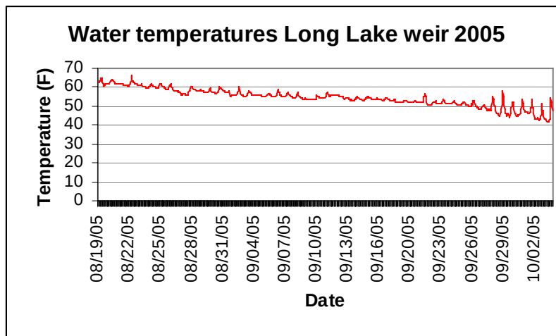
Figure 7. Water temperature data 2005.
