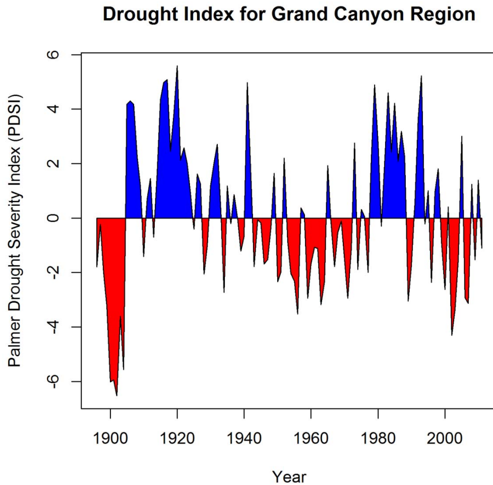
Figure 8. Palmer Drought Severity Index (PDSI) for the region including Grand Canyon National Park (1896-2011). Positive values indicate adequate moisture and negative values (red) indicate drought conditions. Values below -3 denote severe drought. Data from the National Oceanic and Atmospheric Administration ( http://www7.ncdc.noaa.gov ).
