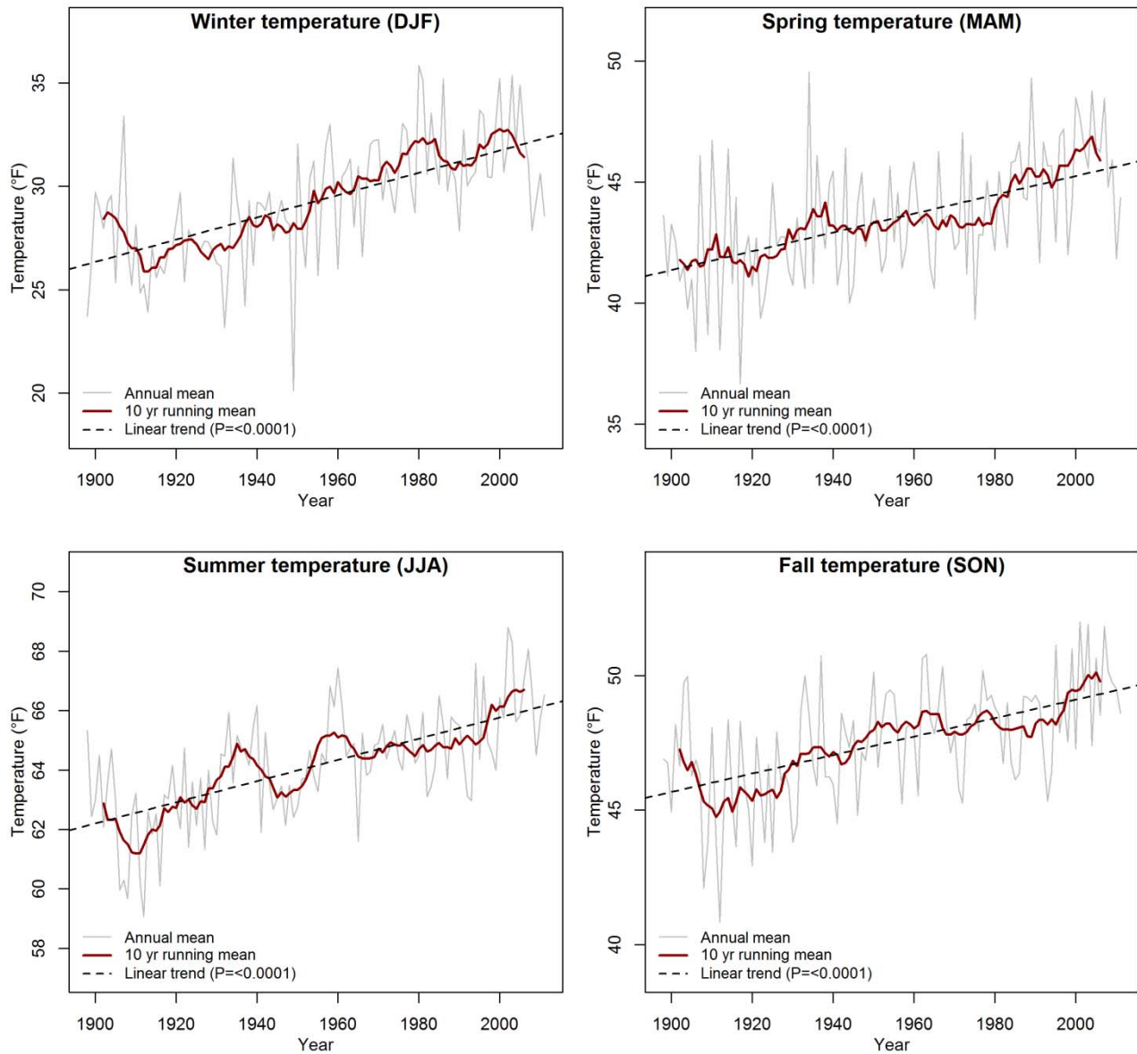
Figure 6. Seasonal temperature trends (1898-2011) from the Grand Canyon NP long-term weather station (cdiac.ornl.gov).
