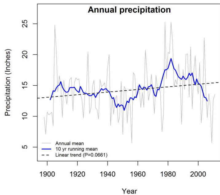
Figure 5. Mean annual temperature and annual precipitation (1898-2011) from the Grand Canyon NP long-term weather station ( cdiac.ornl.gov ).
