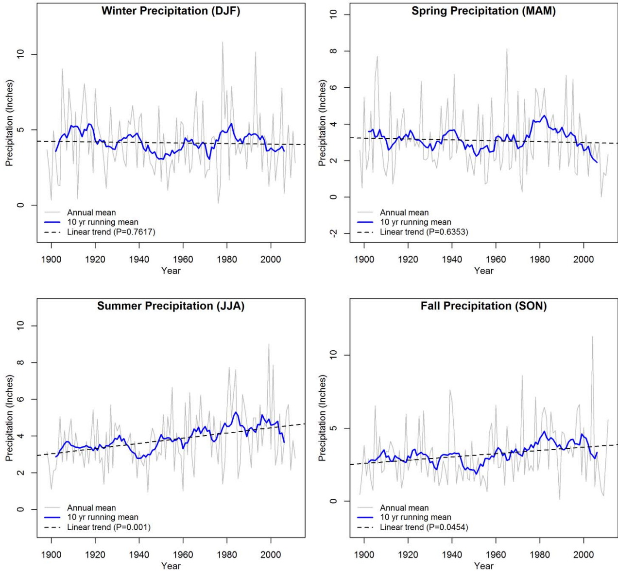
Figure 7. Seasonal precipitation trends (1898-2011) from the Grand Canyon NP long-term weather station ( cdiac.ornl.gov ).
