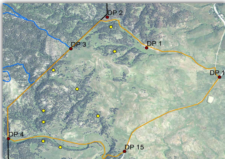
Wind Cave NP Cold Brook burn boundary. Yellow points indicate burn severity plots that are incorporated in the NGPN database.
