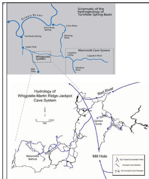
Figure 3: Schematic of the hydrology of Whigpistle Cave System with inset showing schematic of hydrology of Turnhole Spring Basin.
