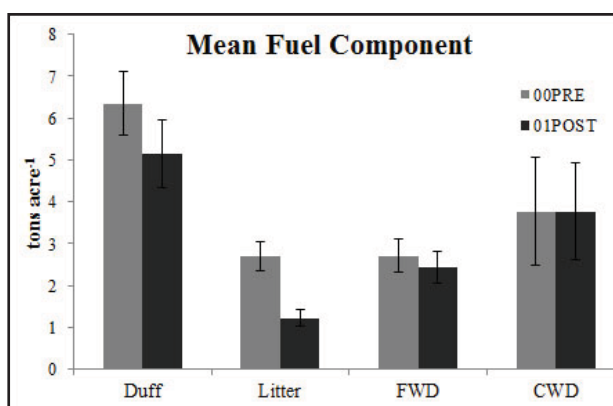
Figure 4: Changes in wildland fuels after a single prescribed fire. Total fuel load was reduced ~18%; however, as separate constituents (duff; leaf, needle, and herbaceous litter; fine woody debris (dead unattached woody stems < 3 in; FWD); and coarse woody debris (dead unattached woody stems ≥ 3 in, CWD), litter was the only significantly reduced component.
