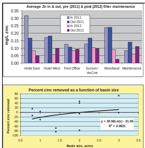
Figure 2: 2a (top graph): Average concentration of zinc ( \text{Zn}^{2+} ) dissolved in storm runoff at the filter inlets and outlets prior to and after the filters had been serviced in the late fall of 2011. [Sunset / Visitor bars are for Sunset Lodge in 2011, and, Visitors Center in 2012; n = 3 or more]. 2b (bottom graph): Regression analysis comparing the percent zinc removed by the filter as a function of parking lot size.
