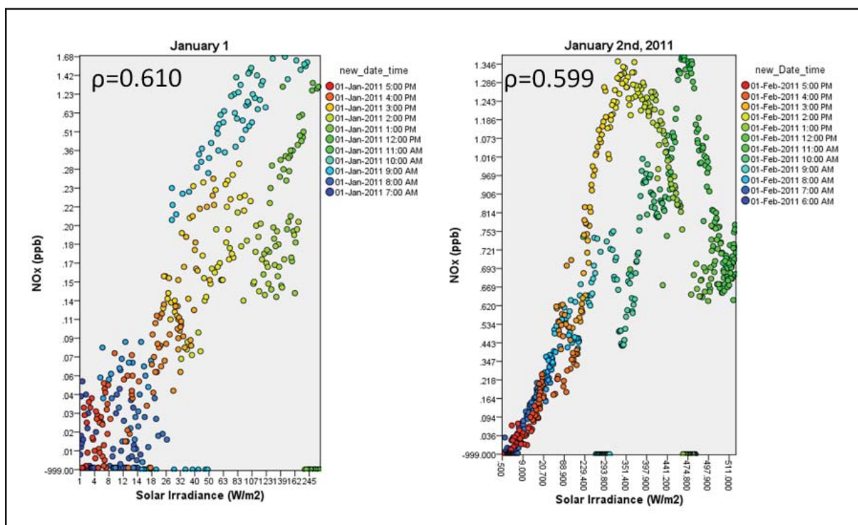
Figure 2: \text{NO}_x levels as a function of solar irradiance (log-log scale) for two different days in January of 2011. On the left, the relationship between \text{NO}_x and solar irradiance is relatively consistent. On the right, a single event drives \text{NO}_x levels high temporarily.
