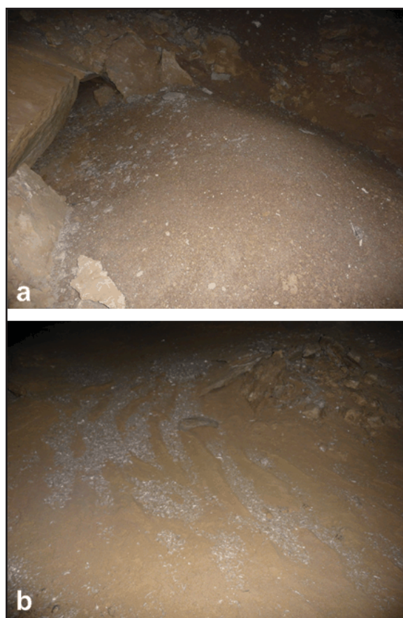
Figure 2: Photos of aeolian phenomena from 2010; a) one of the apparent “dunes” in Turner Avenue, and b) gypsum fluff in the troughs of ripple marks in Swinnerton Avenue.
