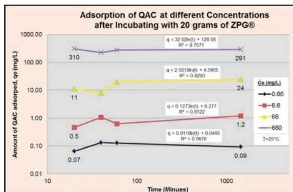
Figure 6: The amount of QAC adsorbed over time with different concentrations was compared. The process is best described by natural logarithm which means the rate of change of QAC adsorbed decreases over time. Also, the adsorption rate is higher with higher initial concentration. The difference in adsorption rate is due to the diffusion effect. The higher concentration of QAC has higher possibility to be adsorbed onto the filter media.
