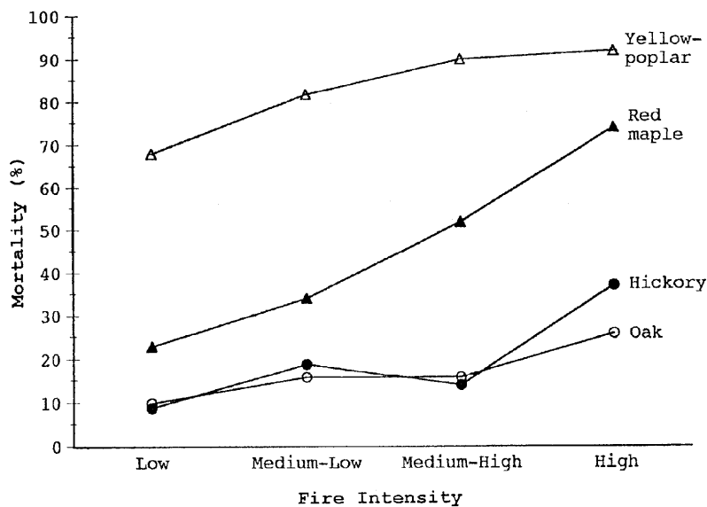
Figure 3.—Mortality (%) of hickory, oak, red maple, and yellow-poplar advance regeneration as fire intensity increases within spring prescribed burns conducted in shelterwood stands.
