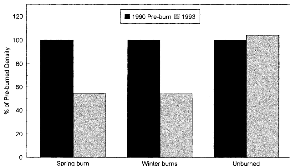
Figure 1.—Reduction of midstory/understory densities following three winter burns and one spring burn in mixed hardwood stands in the South Carolina Piedmont.
