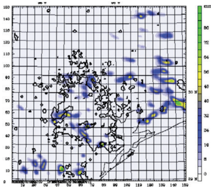
Figure 5.3 Difference (2025 Current Land Cover) in simulated rainfall amount for a typical case day in Houston, Texas. Black outline represents 2025 urban land cover. Rainfall amounts illustrated in the image correspond to the bar graph on the right hand side of the figure (Shepherd et al. 2010a).
