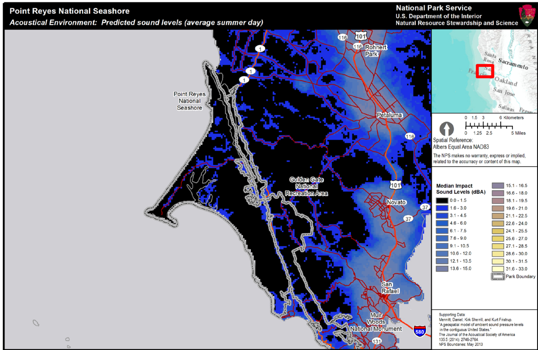
Figure 1a. Median sound level impact map for Point Reyes NS. This park-specific acoustic impact map as generated by version 3.0 of the geospatial model. The color scale indicates how much human-caused noise raises the existing sound pressure levels in a given location (measured in A-weighted decibels, or dBA), with 270 meter resolution. Black and dark blue colors indicate low impacts while yellow or white colors indicate greater impacts. Note that due to the national scale of the model inputs, this graphic may not reflect recent localized changes such as new access roads or development. (note: although the color ramps are similar, each figure has different legend values)
