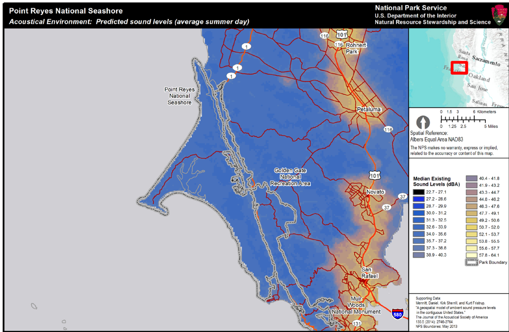
Figure 3a. Median existing sound pressure levels for Point Reyes NS. This park-specific existing sound level map is generated by version 3.0 of the geospatial model. The color scale indicates the decibel level that is predicted in the park based only on both human-caused and natural sound sources. Sound level is measured in A-weighted decibels, or dBA, with 270 meter resolution. Black and dark blue colors indicate low existing decibel levels while yellow or white colors indicate higher existing decibel levels. Sound levels in national parks can vary greatly, depending on location, topography, vegetation, biological activity, weather conditions and other factors. For example, the din of a typical suburban area fluctuates between 50 and 60 decibels (dBA), while the crater of Haleakala National Park is intensely quiet, with levels around 10 dBA. Note that due to the national scale of the model inputs, this graphic may not reflect recent localized changes (such as new access roads or development). (note: although the color ramps are similar, each figure has different legend values)
