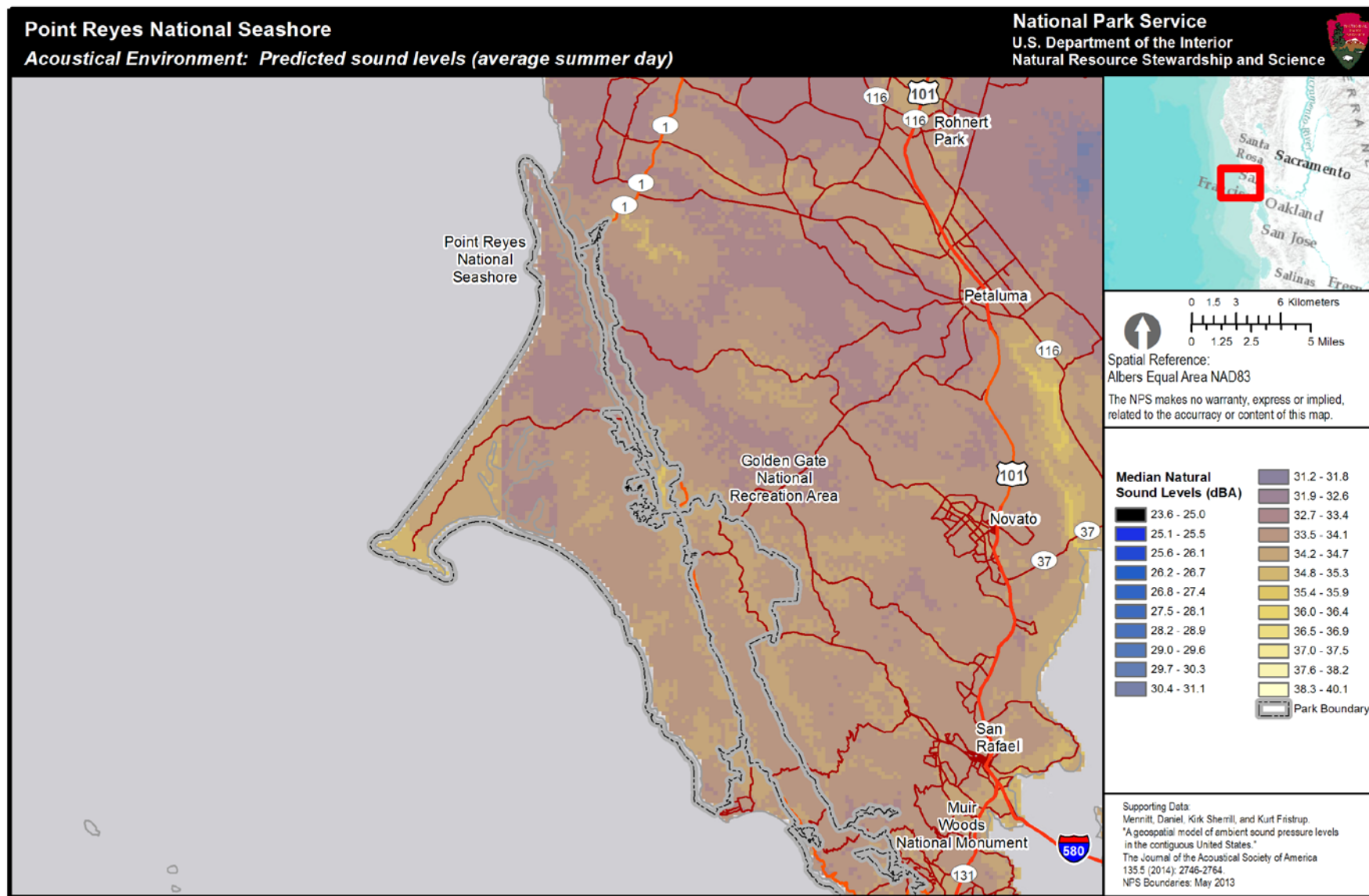
Figure 2a. Median natural sound pressure levels for Point Reyes NS. This park-specific natural sound level map is generated by version 3.0 of the geospatial model. The color scale indicates the decibel level that is predicted in the park based only on natural sound sources. Sound level is measured in A-weighted decibels, or dBA, with 270 meter resolution. Black and dark blue colors indicate low decibel impact levels while yellow or white colors indicate higher decibel impact levels. Note that due to the national scale of the model inputs, this graphic may not reflect recent localized changes (such as new access roads or development). (note: although the color ramps are similar, each figure has different legend values)
