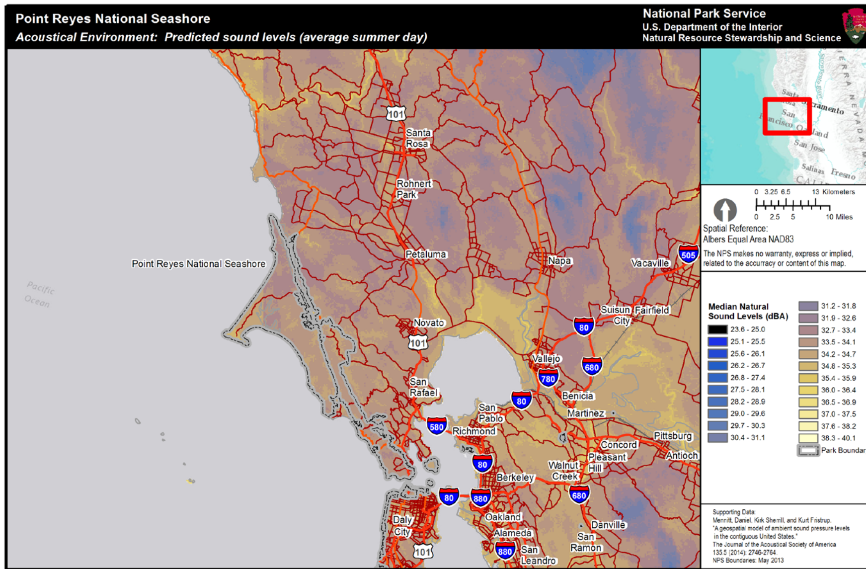
Figure 2b. Median natural sound pressure levels, small scale of figure above.
