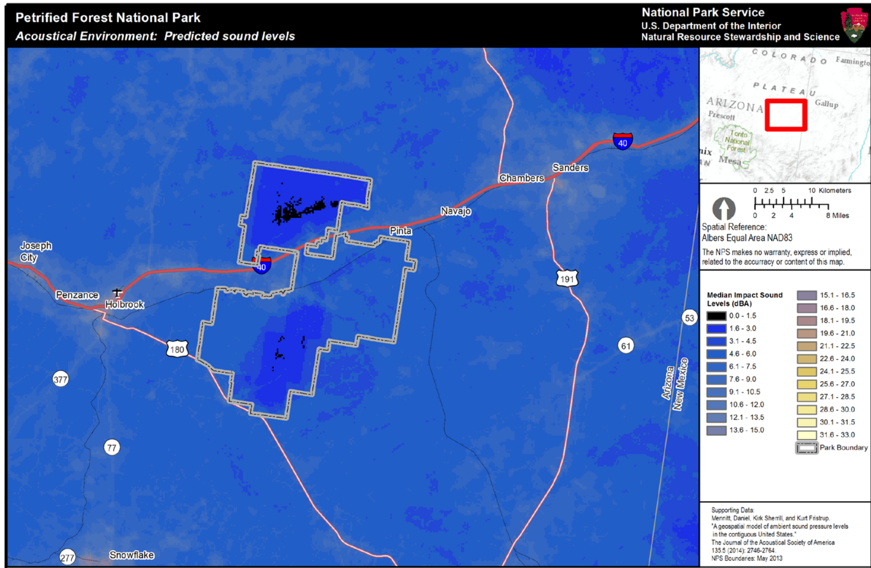
Figure 1. Median sound level impact map for Petrified Forest National Park. This park-specific L50 dBA impact map is generated by ver. 3 of the geospatial model. The color scale indicates how much anthropogenic noise raises the existing sound pressure levels in a given location (measured in A-weighted decibels, or dBA), with 270 meter resolution. Black and dark blue colors indicate low impacts while yellow or white colors indicate greater impacts. (note: each figure has different scale values)
