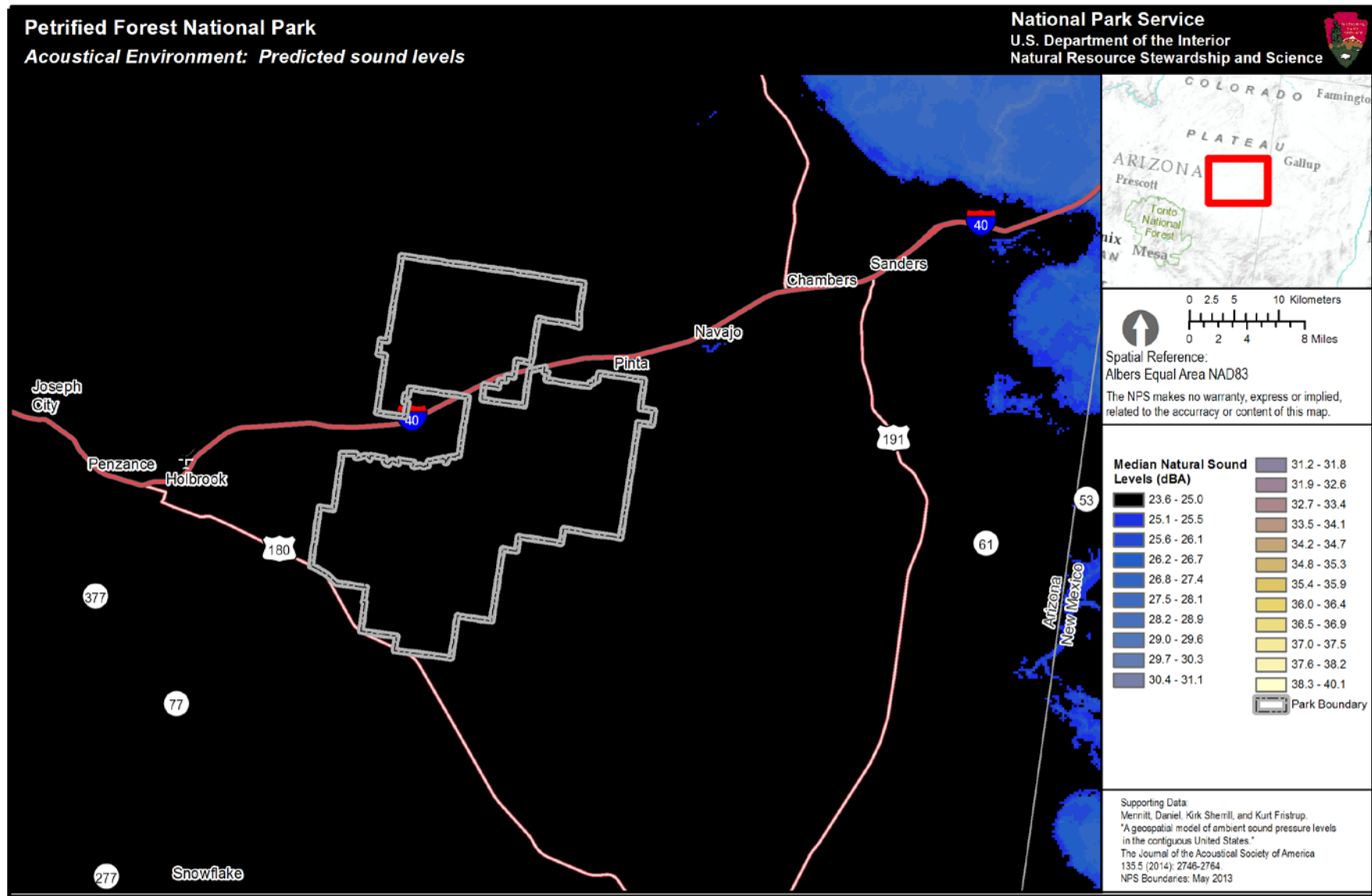
Figure 2. Median natural sound pressure levels for Petrified Forest National Park. This park-specific natural sound level map is generated by ver. 3 of the geospatial model. The color scale indicates the decibel level that is predicted in the park based only on natural sound sources. Sound level is measured in A-weighted decibels, or dBA, with 270 meter resolution. Black and dark blue colors indicate low decibel levels while yellow or white colors indicate higher decibel levels. (note: each figure has different scale values)
