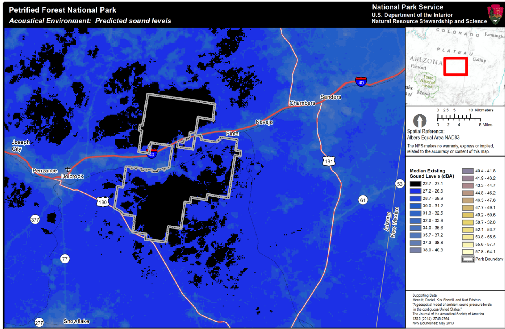
Figure 4. Median existing sound pressure levels for Petrified Forest National Park. This park-specific existing sound level map is generated by ver. 3 of the geospatial model. The color scale indicates the decibel level that is predicted in the park based only on both human-caused and natural sound sources. Sound level is measured in A-weighted decibels, or dBA, with 270 meter resolution. Black and dark blue colors indicate low decibel levels while yellow or white colors indicate higher decibel levels. Sound levels in national parks can vary greatly, depending on location, topography, vegetation, biological activity, weather conditions and other factors. For example, the din of a typical suburban area fluctuates between 50 and 60 decibels (dBA), while the crater of Haleakala National Park is intensely quiet, with levels around 10 dBA. (note: each figure has different scale values)
