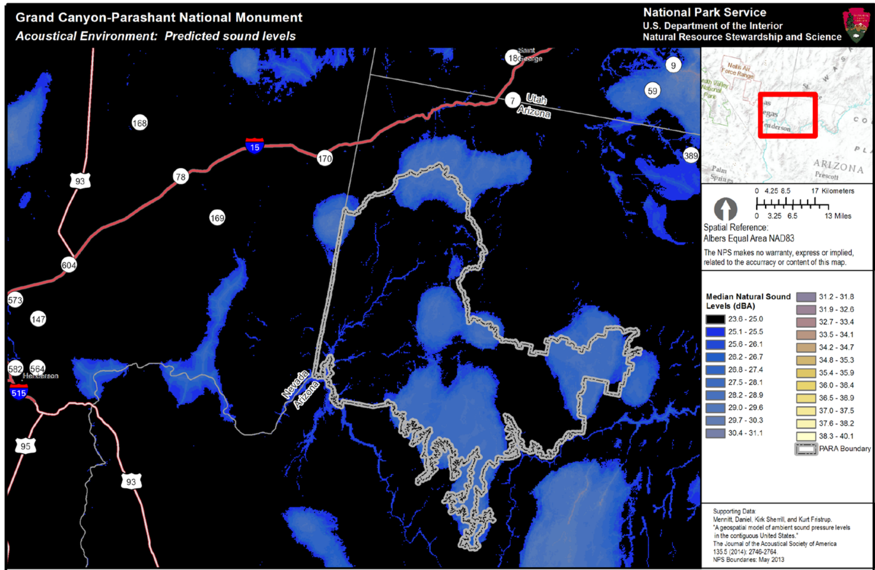
Figure 2. Median natural sound pressure levels for Grand Canyon-Parashant National Monument. This park-specific natural sound level map is generated by version 3 of the geospatial model. The color scale indicates the decibel level that is predicted in the park based only on natural sound sources. Sound level is measured in A-weighted decibels, or dBA, with 270 meter resolution. Black and dark blue colors indicate low decibel levels while yellow or white colors indicate higher decibel levels. (note: each figure has different scale values)
