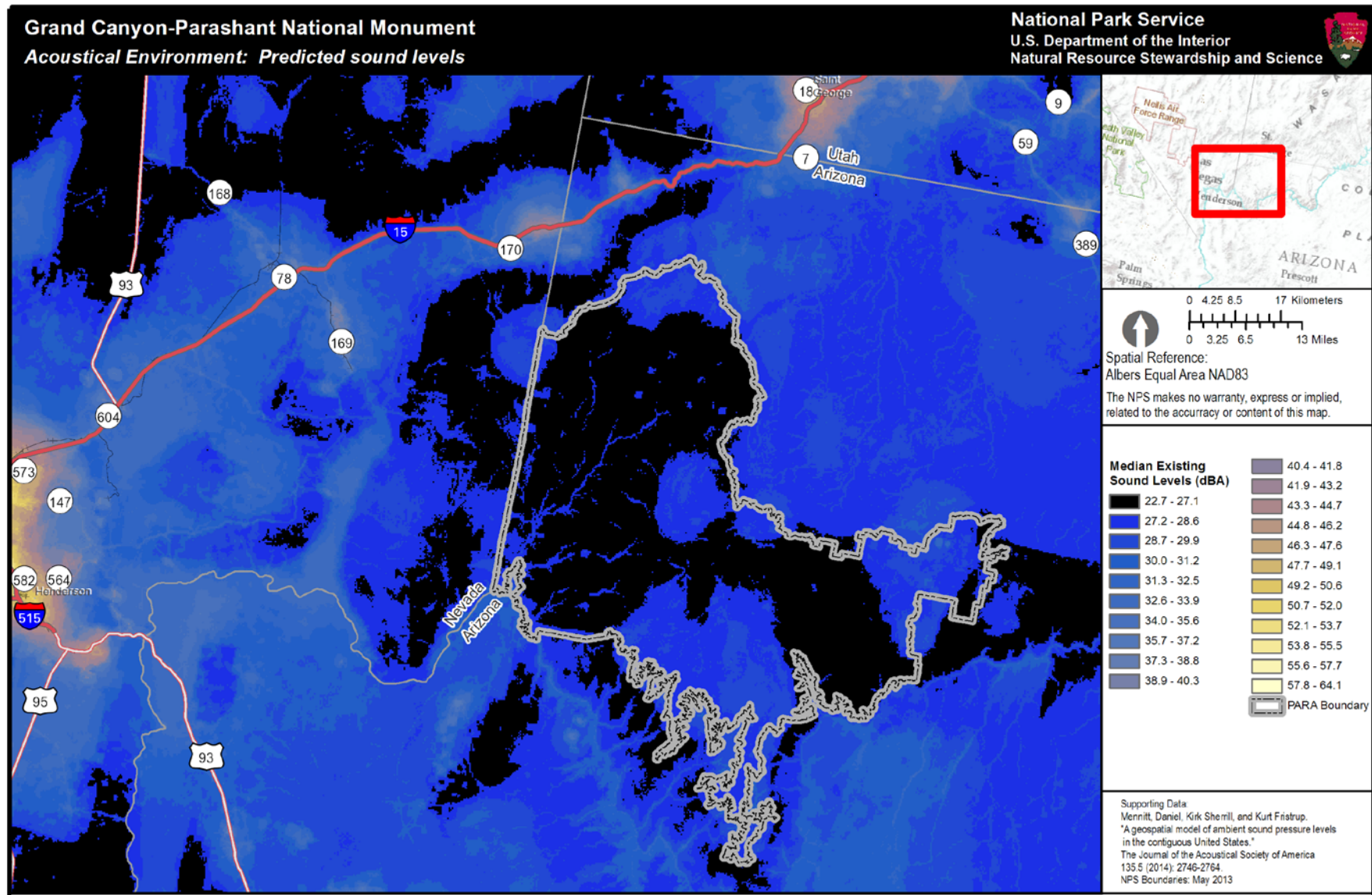
Figure 3. Median existing sound pressure levels for Grand Canyon-Parashant National Monument. This park-specific existing sound level map is generated by version 3 of the geospatial model. The color scale indicates the decibel level that is predicted in the park based only on both human-caused and natural sound sources. Sound level is measured in A-weighted decibels, or dBA, with 270 meter resolution. Black and dark blue colors indicate low decibel levels while yellow or white colors indicate higher decibel levels. Sound levels in national parks can vary greatly, depending on location, topography, vegetation, biological activity, weather conditions and other factors. For example, the din of a typical suburban area fluctuates between 50 and 60 decibels (dBA), while the crater of Haleakala National Park is intensely quiet, with levels around 10 dBA. (note: each figure has different scale values)
