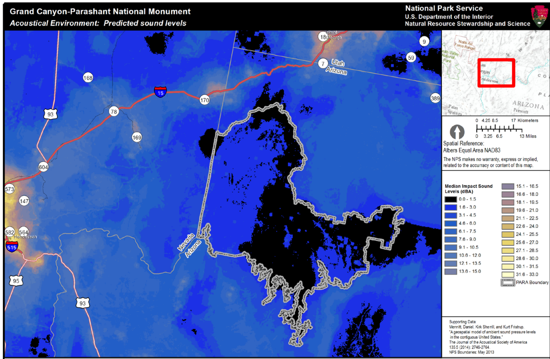
Figure 1. Median sound level impact map for Grand Canyon-Parashant National Monument. This park-specific L50 dBA impact map is generated by version 3 of the geospatial model. The color scale indicates how much anthropogenic noise raises the existing sound pressure levels in a given location (measured in A-weighted decibels, or dBA), with 270 meter resolution. Black and dark blue colors indicate low impacts while yellow or white colors indicate greater impacts. (note: each figure has different scale values)
