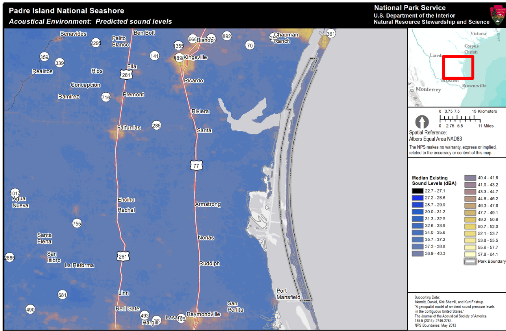
Figure 3. Median existing sound pressure levels for Padre Island National Seashore. This park-specific existing sound level map is generated by version 3 of the geospatial model. The color scale indicates the decibel level that is predicted in the park based only on both human-caused and natural sound sources. Sound level is measured in A-weighted decibels, or dBA, with 270 meter resolution. Black and dark blue colors indicate low decibel levels while yellow or white colors indicate higher decibel levels. Sound levels in national parks can vary greatly, depending on location, topography, vegetation, biological activity, weather conditions and other factors. For example, the din of a typical suburban area fluctuates between 50 and 60 decibels (dBA), while the crater of Haleakala National Park is intensely quiet, with levels around 10 dBA. (note: each figure has different scale values)
