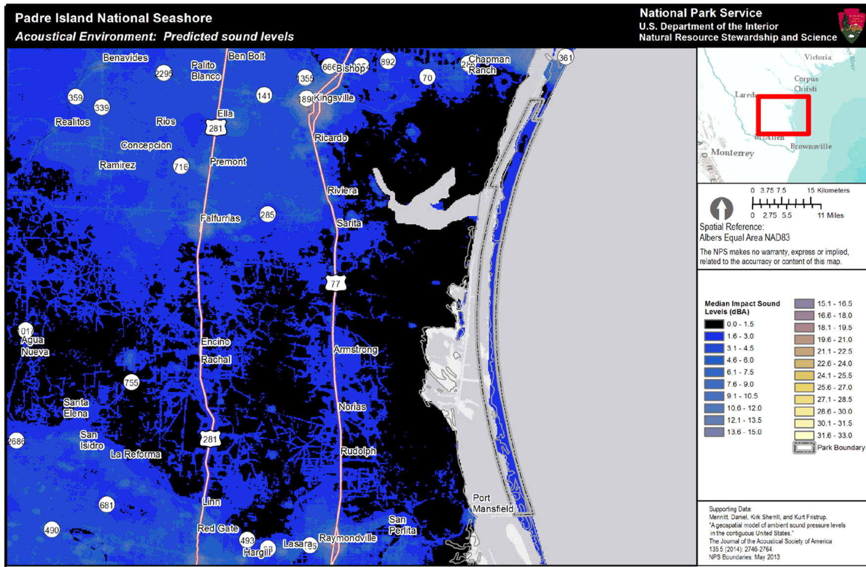
Figure 1. Median sound level impact map for Padre Island National Seashore. This park-specific L50 dBA impact map is generated by version 3 of the geospatial model. The color scale indicates how much anthropogenic noise raises the existing sound pressure levels in a given location (measured in A-weighted decibels, or dBA), with 270 meter resolution. Black and dark blue colors indicate low impacts while yellow or white colors indicate greater impacts. (note: each figure has different scale values)
