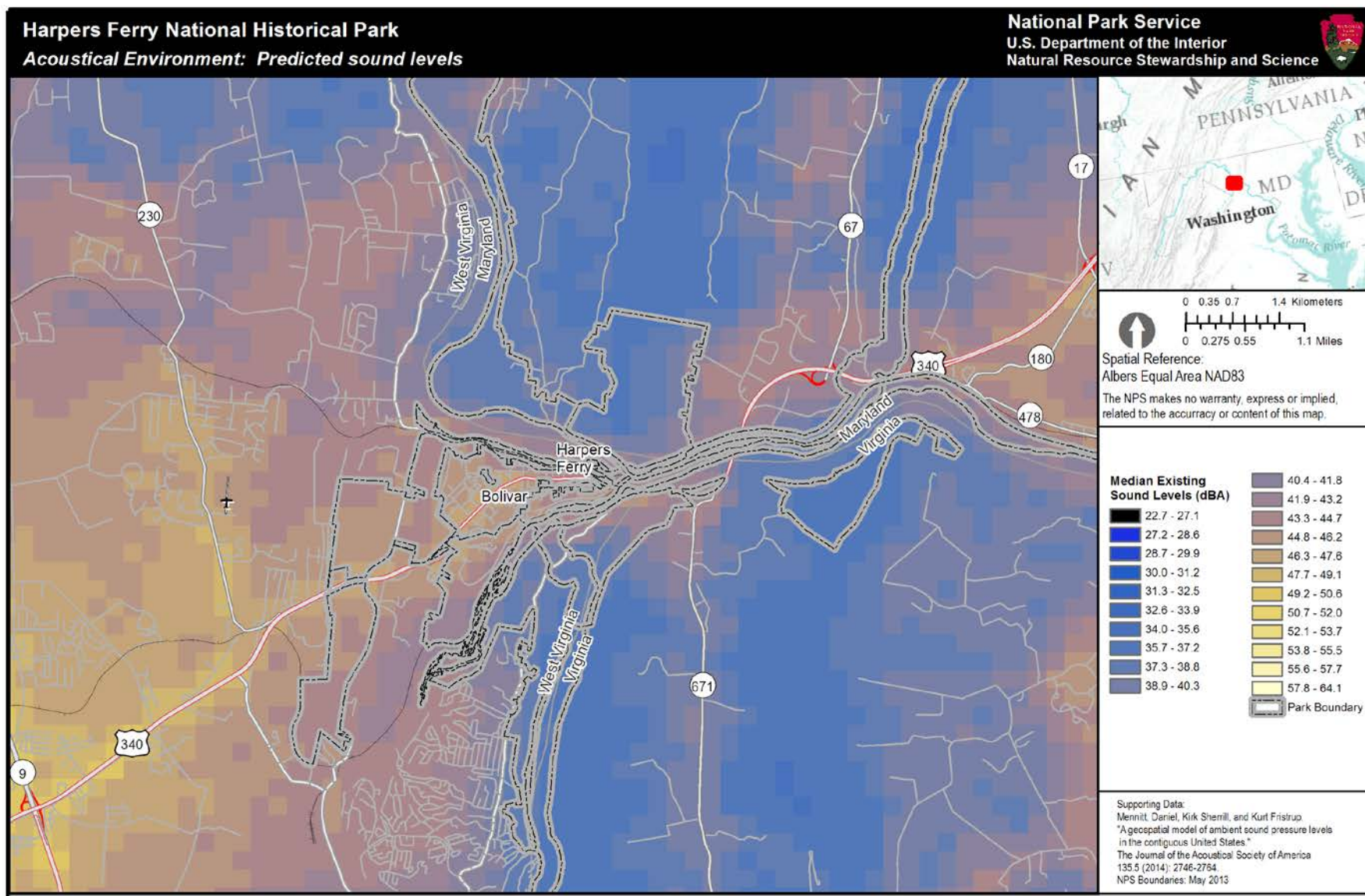
Figure 3. Median existing sound pressure levels for Harpers Ferry NHP. This park-specific existing sound level map is generated by version 3 of the geospatial model. The color scale indicates the decibel level that is predicted in the park based only on both human-caused and natural sound sources. Sound level is measured in A-weighted decibels, or dBA, with 270 meter resolution. Black and dark blue colors indicate low decibel levels while yellow or white colors indicate higher decibel levels. Sound levels in national parks can vary greatly, depending on location, topography, vegetation, biological activity, weather conditions and other factors. For example, the din of a typical suburban area fluctuates between 50 and 60 decibels (dBA), while the crater of Haleakala National Park is intensely quiet, with levels around 10 dBA. (note: each figure has different scale values)
