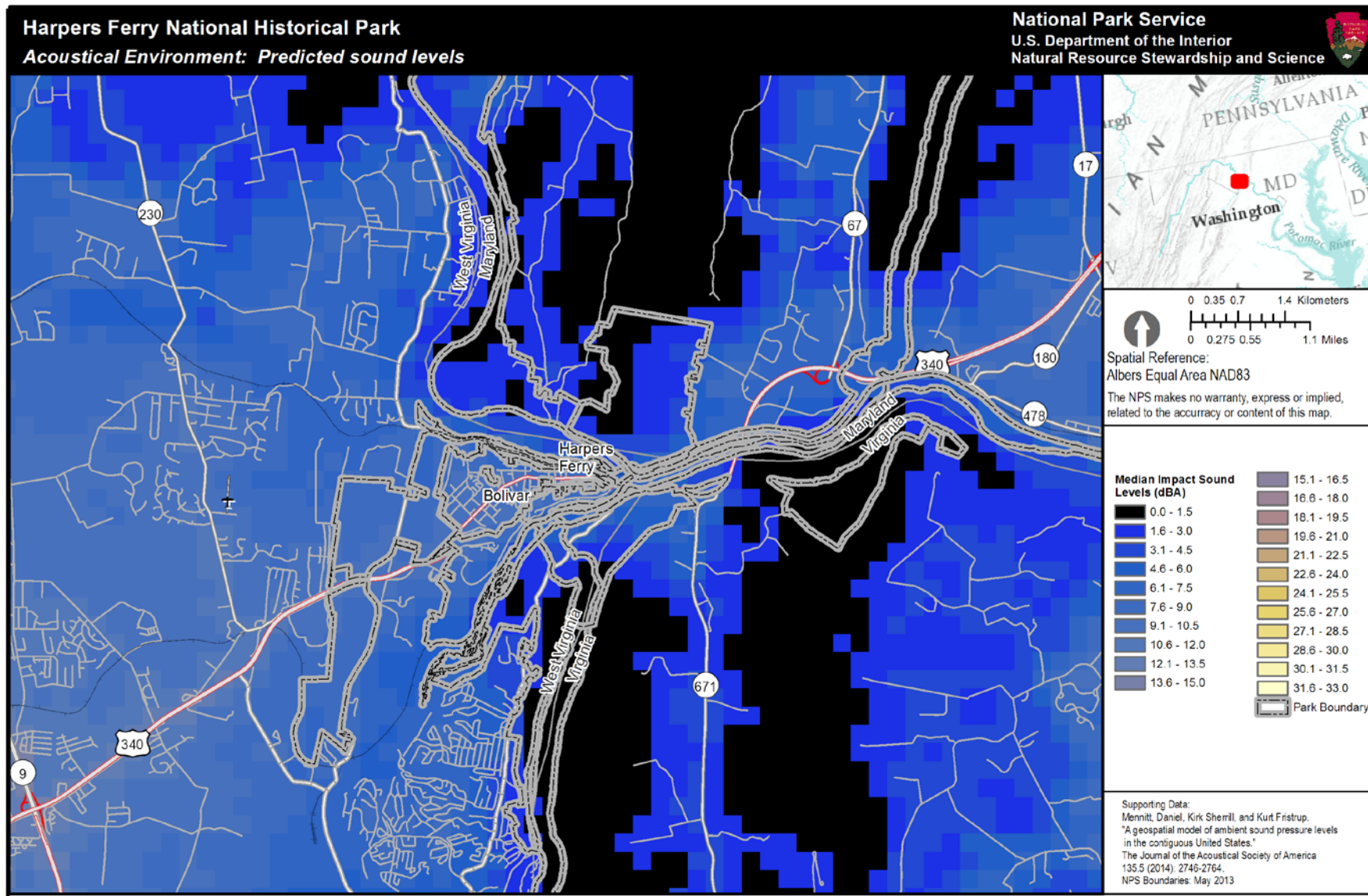
Figure 1. Median sound level impact map for Harpers Ferry NHP. This park-specific L50 dBA impact map is generated by version 3 of the geospatial model. The color scale indicates how much anthropogenic noise raises the existing sound pressure levels in a given location (measured in A-weighted decibels, or dBA), with 270 meter resolution. Black and dark blue colors indicate low impacts while yellow or white colors indicate greater impacts. (note: each figure has different scale values)
