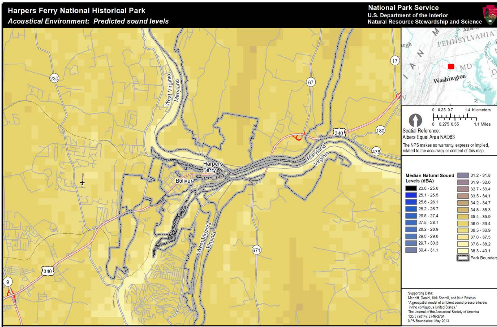
Figure 2. Median natural sound pressure levels for Harpers Ferry NHP. This park-specific natural sound level map is generated by version 3 of the geospatial model. The color scale indicates the decibel level that is predicted in the park based only on natural sound sources. Sound level is measured in A-weighted decibels, or dBA, with 270 meter resolution. Black and dark blue colors indicate low decibel levels while yellow or white colors indicate higher decibel levels. (note: each figure has different scale values)
