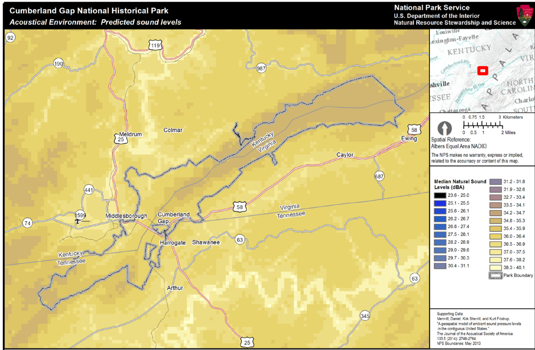
Figure 2. Median natural sound pressure levels for Cumberland Gap NHP. This park-specific natural sound level map is generated by version 3 of the geospatial model. The color scale indicates the decibel level that is predicted in the park based only on natural sound sources. Sound level is measured in A-weighted decibels, or dBA, with 270 meter resolution. Black and dark blue colors indicate low decibel levels while yellow or white colors indicate higher decibel levels. (note: each figure has different scale values)
