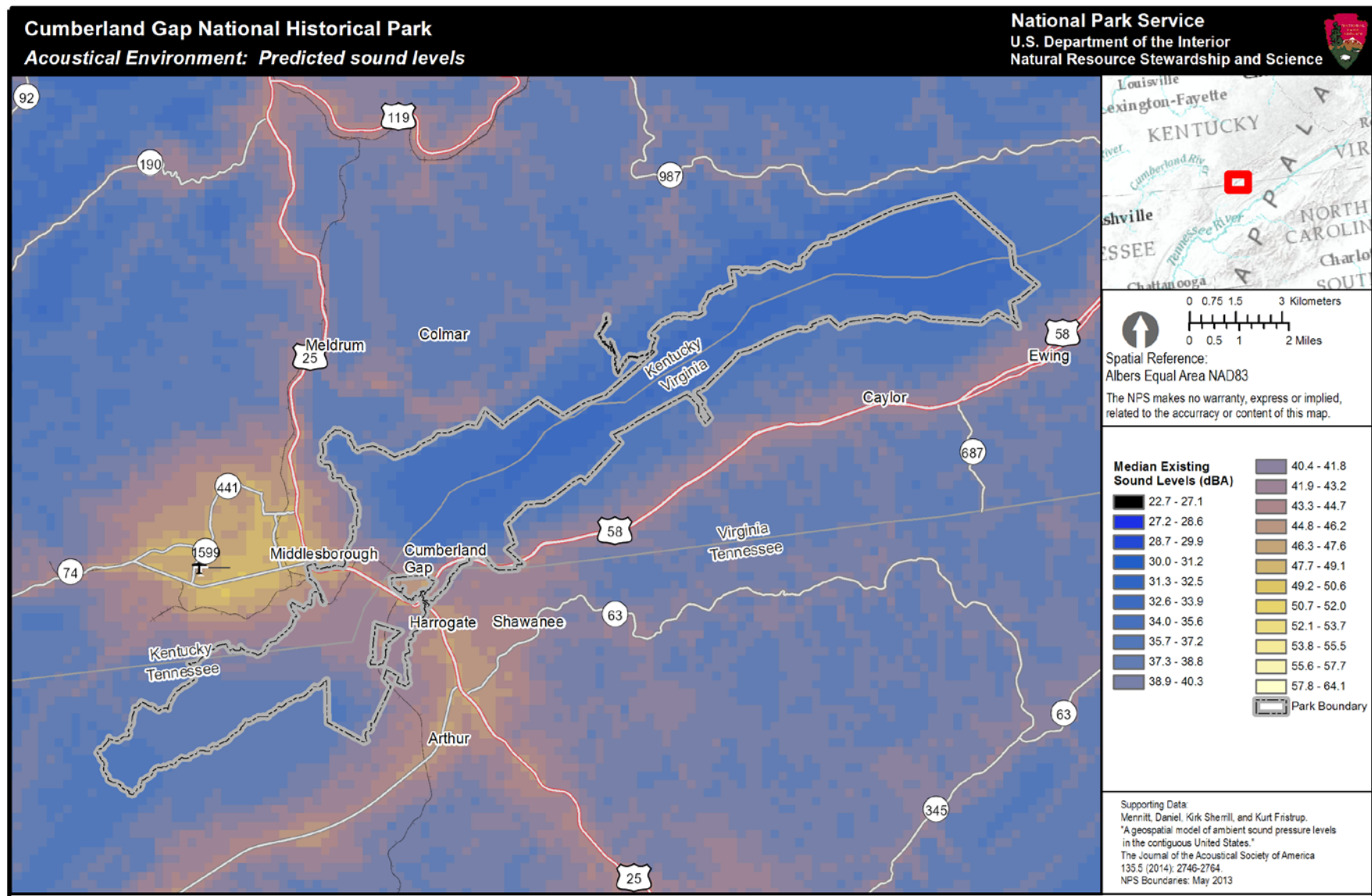
Figure 3. Median existing sound pressure levels for Cumberland Gap NHP. This park-specific existing sound level map is generated by version 3 of the geospatial model. The color scale indicates the decibel level that is predicted in the park based only on both human-caused and natural sound sources. Sound level is measured in A-weighted decibels, or dBA, with 270 meter resolution. Black and dark blue colors indicate low decibel levels while yellow or white colors indicate higher decibel levels. Sound levels in national parks can vary greatly, depending on location, topography, vegetation, biological activity, weather conditions and other factors. For example, the din of a typical suburban area fluctuates between 50 and 60 decibels (dBA), while the crater of Haleakala National Park is intensely quiet, with levels around 10 dBA. (note: each figure has different scale values)
