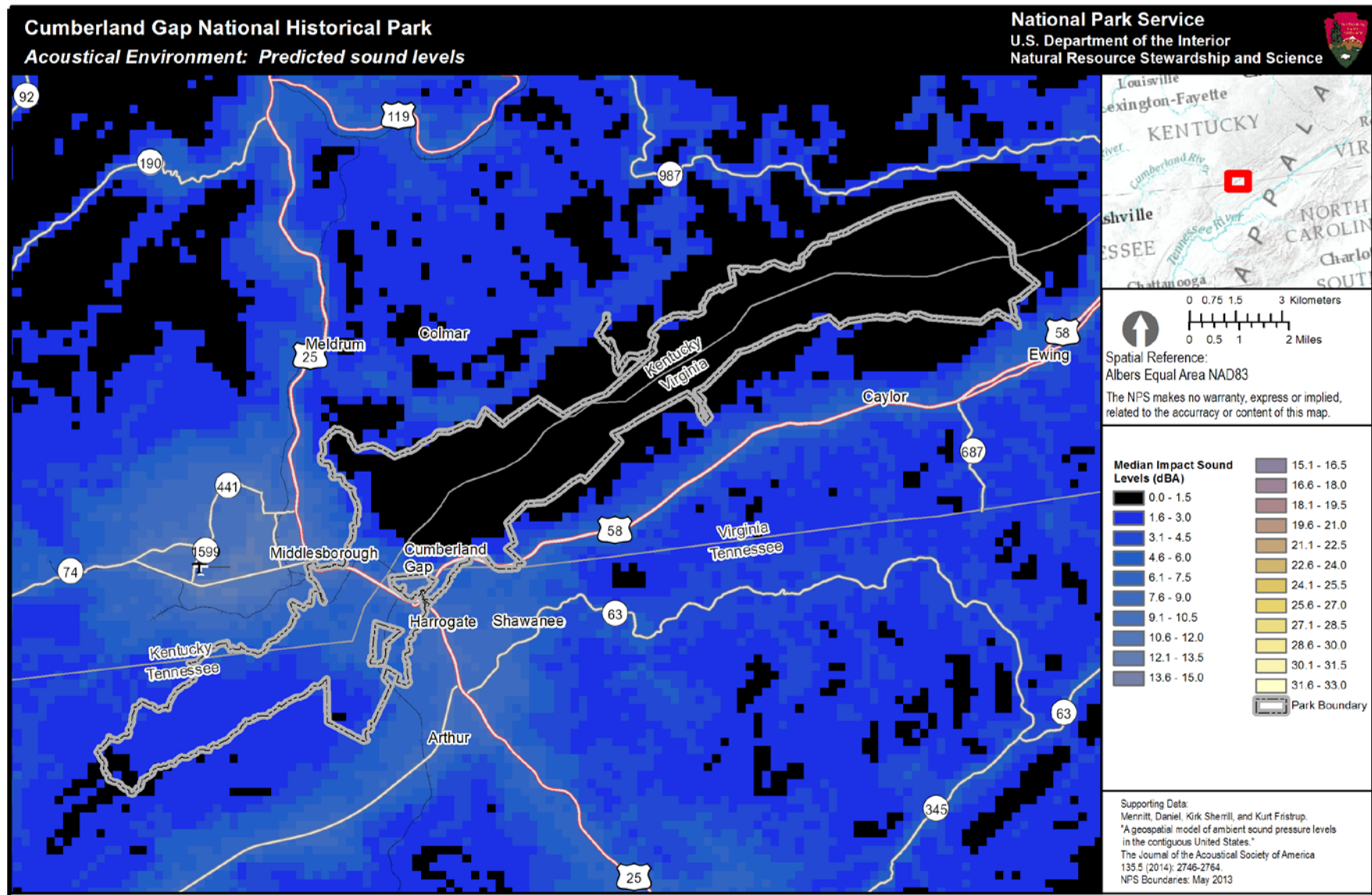
Figure 1. Median sound level impact map for Cumberland Gap NHP. This park-specific L50 dBA impact map is generated by version 3 of the geospatial model. The color scale indicates how much anthropogenic noise raises the existing sound pressure levels in a given location (measured in A-weighted decibels, or dBA), with 270 meter resolution. Black and dark blue colors indicate low impacts while yellow or white colors indicate greater impacts. (note: each figure has different scale values)
