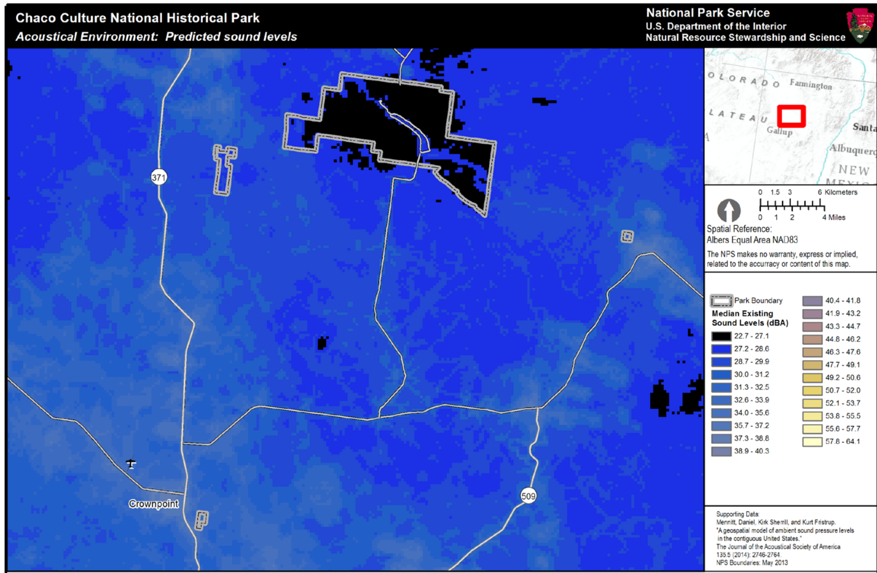
Figure 4. Median existing sound pressure levels for Chaco Culture NHP. This park-specific existing sound level map is generated by ver. 3 of the geospatial model. The color scale indicates the decibel level that is predicted in the park based only on both human-caused and natural sound sources. Sound level is measured in A-weighted decibels, or dBA, with 270 meter resolution. Black and dark blue colors indicate low decibel levels while yellow or white colors indicate higher decibel levels. Sound levels in national parks can vary greatly, depending on location, topography, vegetation, biological activity, weather conditions and other factors. For example, the din of a typical suburban area fluctuates between 50 and 60 decibels (dBA), while the crater of Haleakala National Park is intensely quiet, with levels around 10 dBA. (note: each figure has different scale values)
