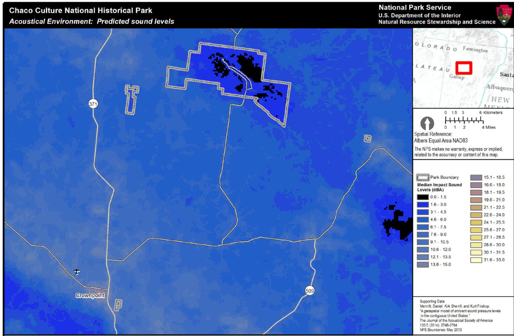
Figure 1. Median sound level impact map for Chaco Culture NHP. This park-specific L50 dBA impact map is generated by ver. 3 of the geospatial model. The color scale indicates how much anthropogenic noise raises the existing sound pressure levels in a given location (measured in A-weighted decibels, or dBA), with 270 meter resolution. Black and dark blue colors indicate low impacts while yellow or white colors indicate greater impacts. (note: each figure has different scale values)
