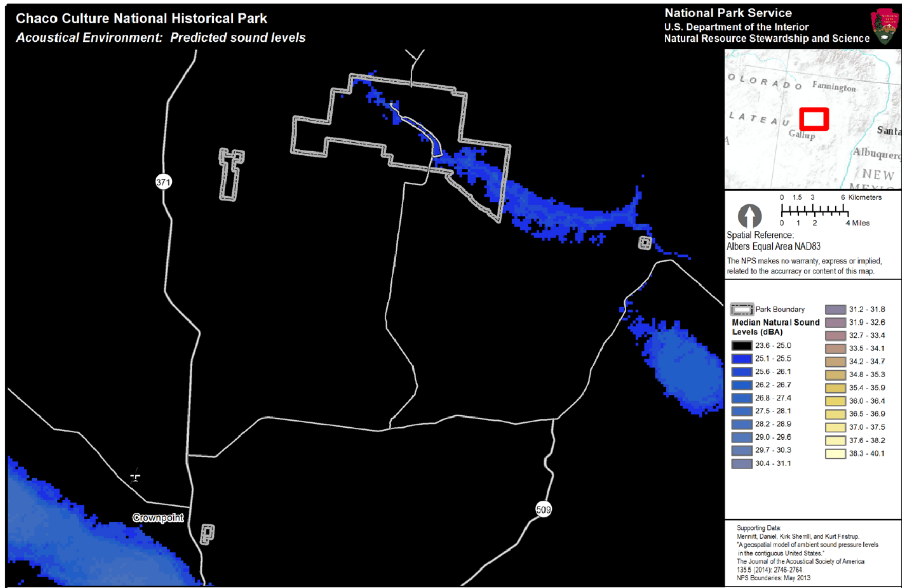
Figure 2. Median natural sound pressure levels for Chaco Culture NHP. This park-specific natural sound level map is generated by ver. 3 of the geospatial model. The color scale indicates the decibel level that is predicted in the park based only on natural sound sources. Sound level is measured in A-weighted decibels, or dBA, with 270 meter resolution. Black and dark blue colors indicate low decibel levels while yellow or white colors indicate higher decibel levels. (note: each figure has different scale values)
