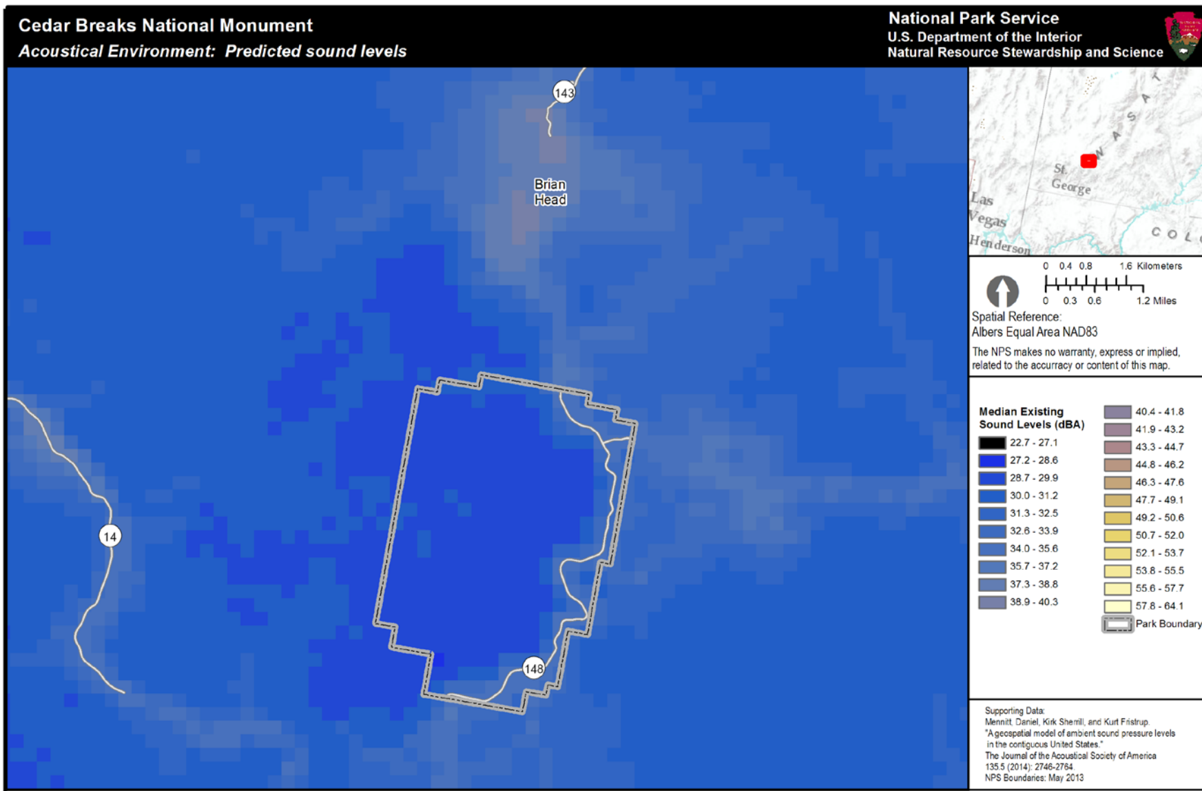
Figure 4. Median existing sound pressure levels for Cedar Breaks NM. This park-specific existing sound level map is generated by ver. 3 of the geospatial model. The color scale indicates the decibel level that is predicted in the park based only on both human-caused and natural sound sources. Sound level is measured in A-weighted decibels, or dBA, with 270 meter resolution. Black and dark blue colors indicate low decibel levels while yellow or white colors indicate higher decibel levels. Sound levels in national parks can vary greatly, depending on location, topography, vegetation, biological activity, weather conditions and other factors. For example, the din of a typical suburban area fluctuates between 50 and 60 decibels (dBA), while the crater of Haleakala National Park is intensely quiet, with levels around 10 dBA. (note: each figure has different scale values)
