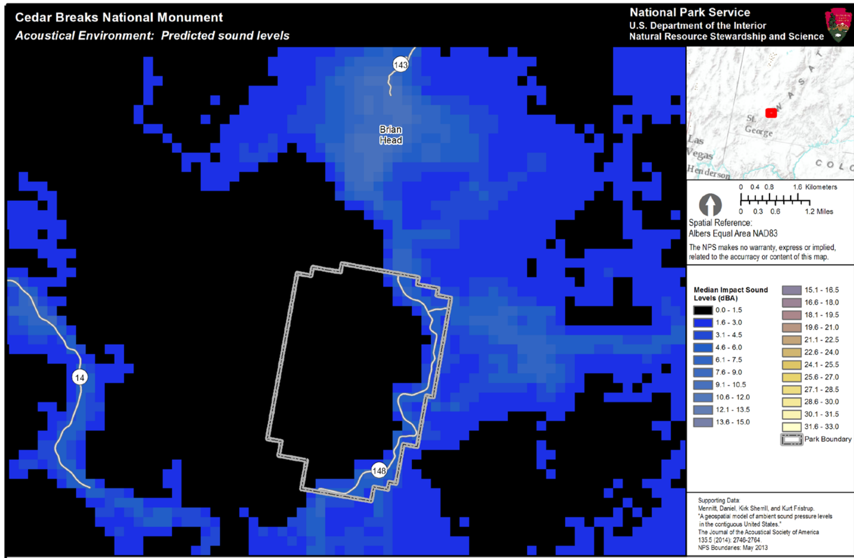
Figure 1. Median sound level impact map for Cedar Breaks NM. This park-specific L50 dBA impact map is generated by ver. 3 of the geospatial model. The color scale indicates how much anthropogenic noise raises the existing sound pressure levels in a given location (measured in A-weighted decibels, or dBA), with 270 meter resolution. Black and dark blue colors indicate low impacts while yellow or white colors indicate greater impacts. (note: each figure has different scale values)
