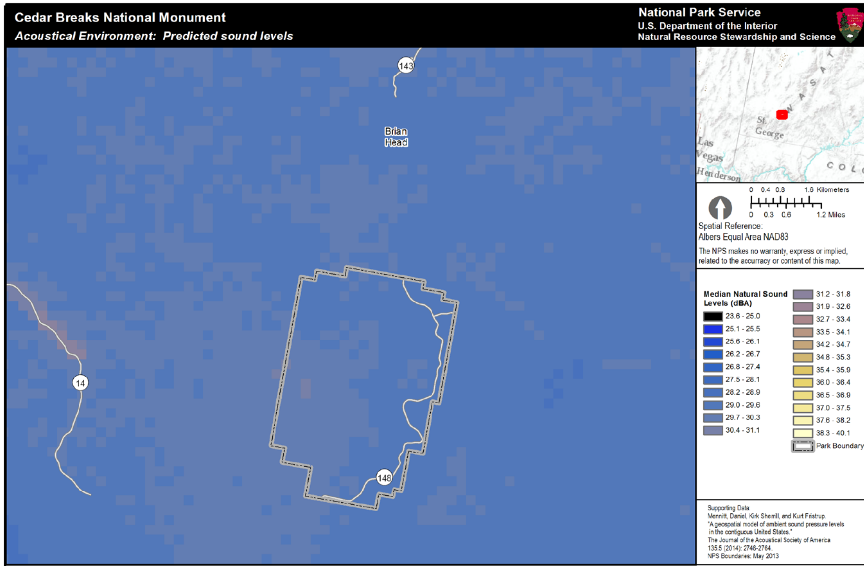
Figure 2. Median natural sound pressure levels for Cedar Breaks NM. This park-specific natural sound level map is generated by ver. 3 of the geospatial model. The color scale indicates the decibel level that is predicted in the park based only on natural sound sources. Sound level is measured in A-weighted decibels, or dBA, with 270 meter resolution. Black and dark blue colors indicate low decibel levels while yellow or white colors indicate higher decibel levels. (note: each figure has different scale values)
