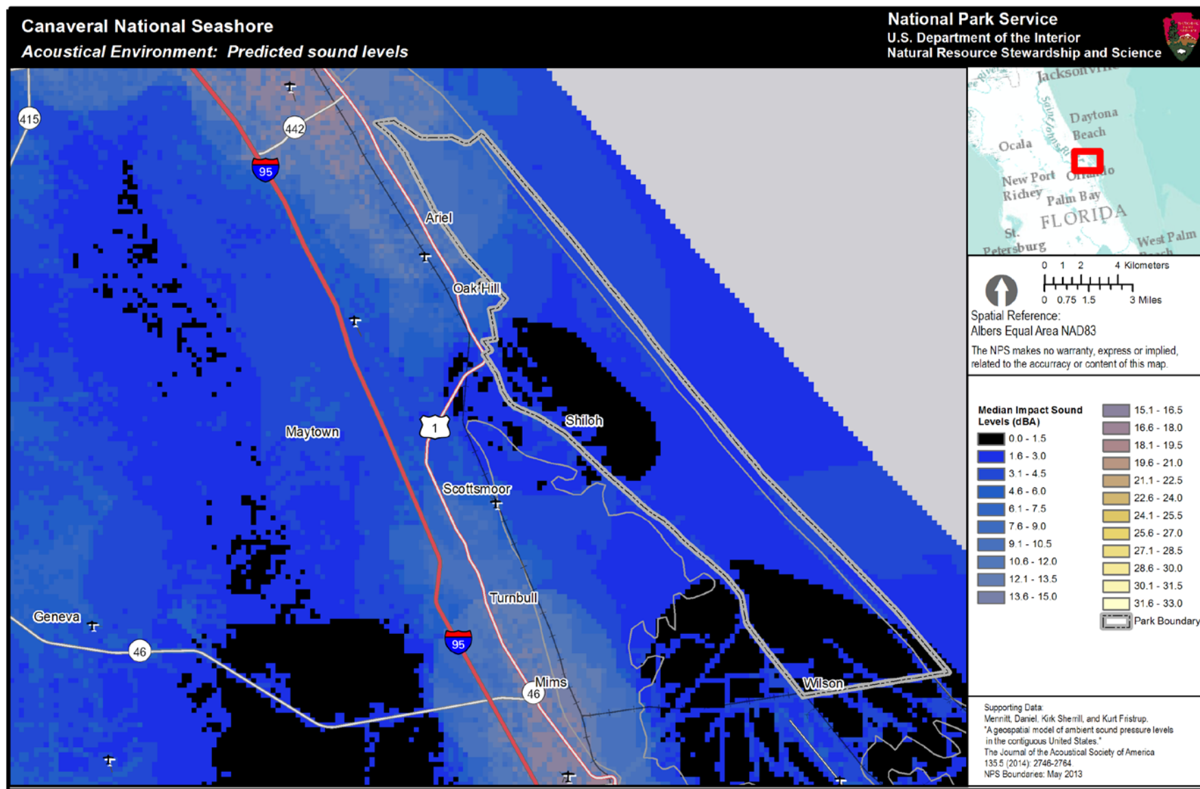
Figure 1. Median sound level impact map for Canaveral National Seashore. This park-specific L50 dBA impact map is generated by ver. 2.31 of the geospatial model. The color scale indicates how much anthropogenic noise raises the existing sound pressure levels in a given location (measured in A-weighted decibels, or dBA), with 270 meter resolution. Black and dark blue colors indicate low impacts while yellow or white colors indicate greater impacts. (note: each figure has different scale values)
