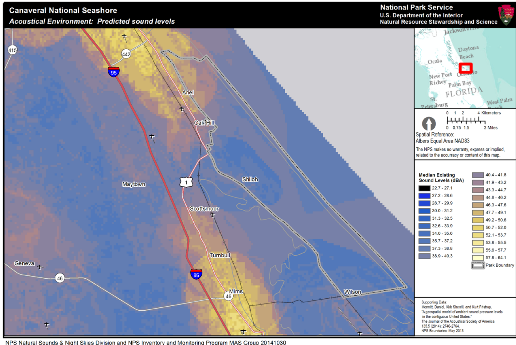
Figure 4. Median existing sound pressure levels for Canaveral National Seashore. This park-specific existing sound level map is generated by ver. 2.31 of the geospatial model. The color scale indicates the decibel level that is predicted in the park based only on both human-caused and natural sound sources. Sound level is measured in A-weighted decibels, or dBA, with 270 meter resolution. Black and dark blue colors indicate low decibel levels while yellow or white colors indicate higher decibel levels. Sound levels in national parks can vary greatly, depending on location, topography, vegetation, biological activity, weather conditions and other factors. For example, the din of a typical suburban area fluctuates between 50 and 60 decibels (dBA), while the crater of Haleakala National Park is intensely quiet, with levels around 10 dBA. (note: each figure has different scale values)
