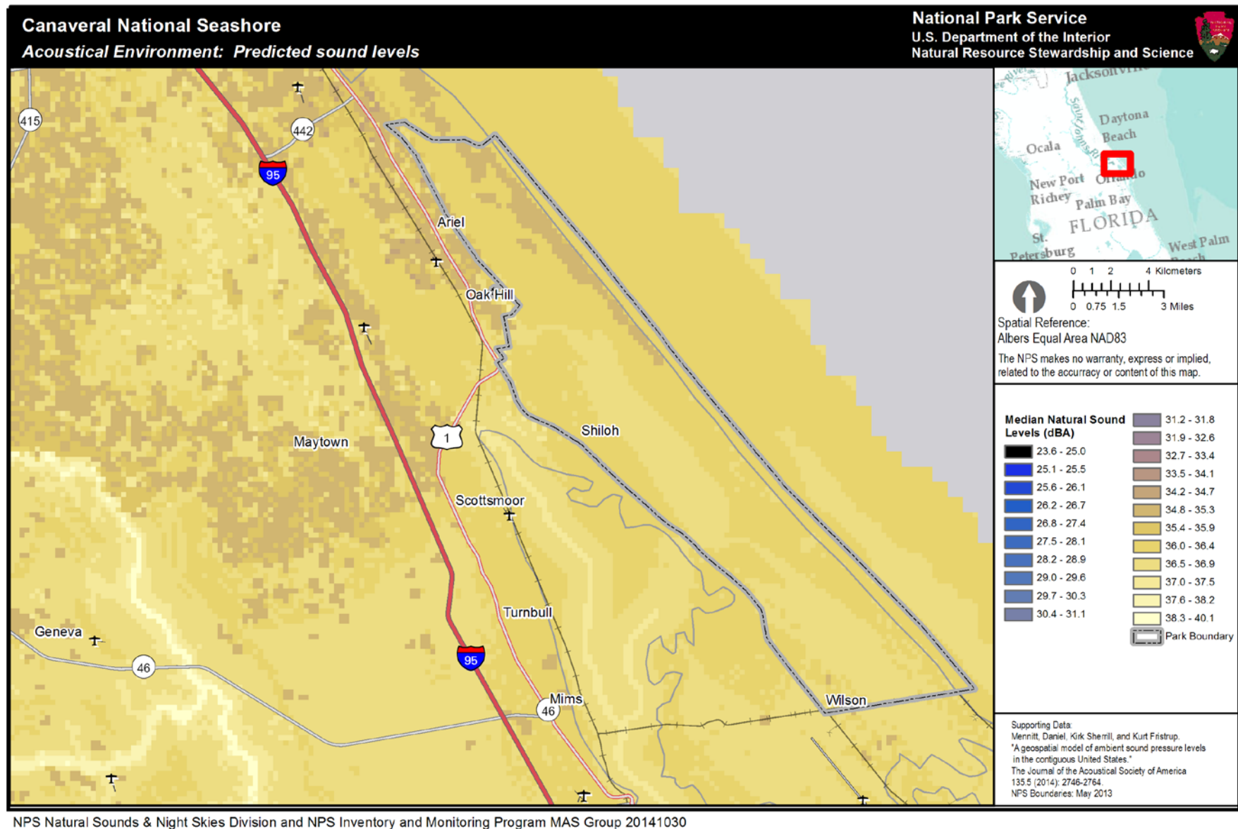
Figure 2. Median natural sound pressure levels for Canaveral National Seashore. This park-specific natural sound level map is generated by ver. 2.31 of the geospatial model. The color scale indicates the decibel level that is predicted in the park based only on natural sound sources. Sound level is measured in A-weighted decibels, or dBA, with 270 meter resolution. Black and dark blue colors indicate low decibel levels while yellow or white colors indicate higher decibel levels. (note: each figure has different scale values)
