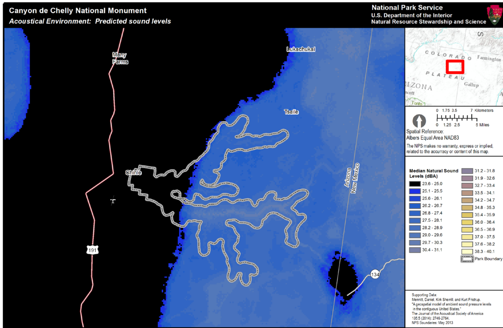
Figure 2. Median natural sound pressure levels for Canyon de Chelly NM. This park-specific natural sound level map is generated by version 3 of the geospatial model. The color scale indicates the decibel level that is predicted in the park based only on natural sound sources. Sound level is measured in A-weighted decibels, or dBA, with 270 meter resolution. Black and dark blue colors indicate low decibel levels while yellow or white colors indicate higher decibel levels. (note: each figure has different scale values)
