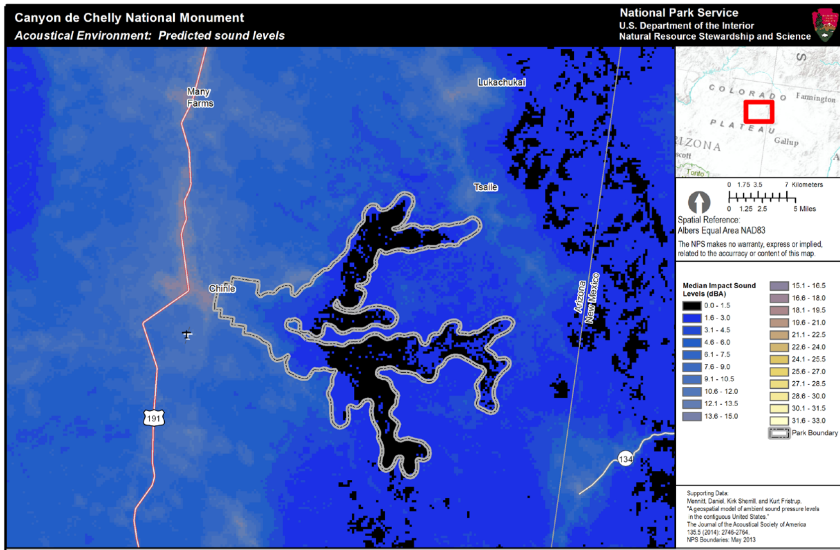
Figure 1. Median sound level impact map for Canyon de Chelly NM. This park-specific L50 dBA impact map is generated by version 3 of the geospatial model. The color scale indicates how much anthropogenic noise raises the existing sound pressure levels in a given location (measured in A-weighted decibels, or dBA), with 270 meter resolution. Black and dark blue colors indicate low impacts while yellow or white colors indicate greater impacts. (note: each figure has different scale values)
