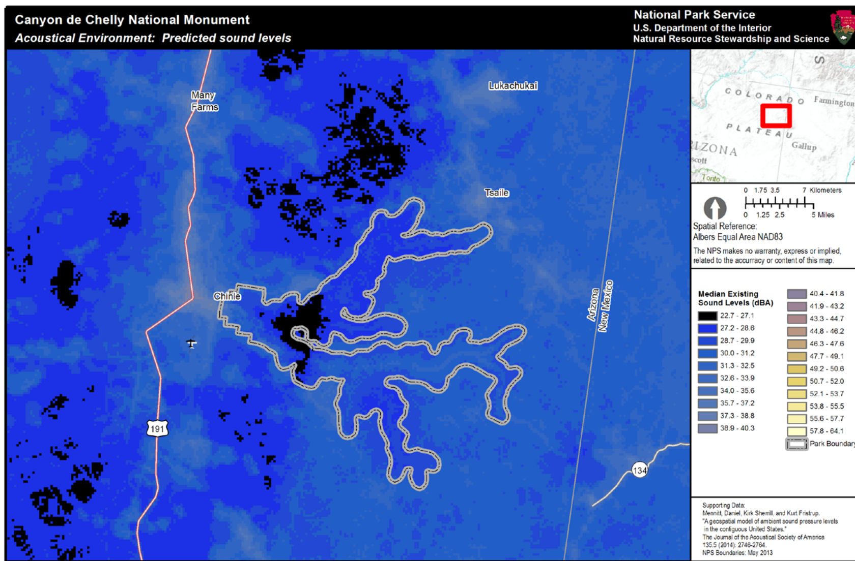
Figure 3. Median existing sound pressure levels for Canyon de Chelly NM. This park-specific existing sound level map is generated by version 3 of the geospatial model. The color scale indicates the decibel level that is predicted in the park based only on both human-caused and natural sound sources. Sound level is measured in A-weighted decibels, or dBA, with 270 meter resolution. Black and dark blue colors indicate low decibel levels while yellow or white colors indicate higher decibel levels. Sound levels in national parks can vary greatly, depending on location, topography, vegetation, biological activity, weather conditions and other factors. For example, the din of a typical suburban area fluctuates between 50 and 60 decibels (dBA), while the crater of Haleakala National Park is intensely quiet, with levels around 10 dBA. (note: each figure has different scale values)
