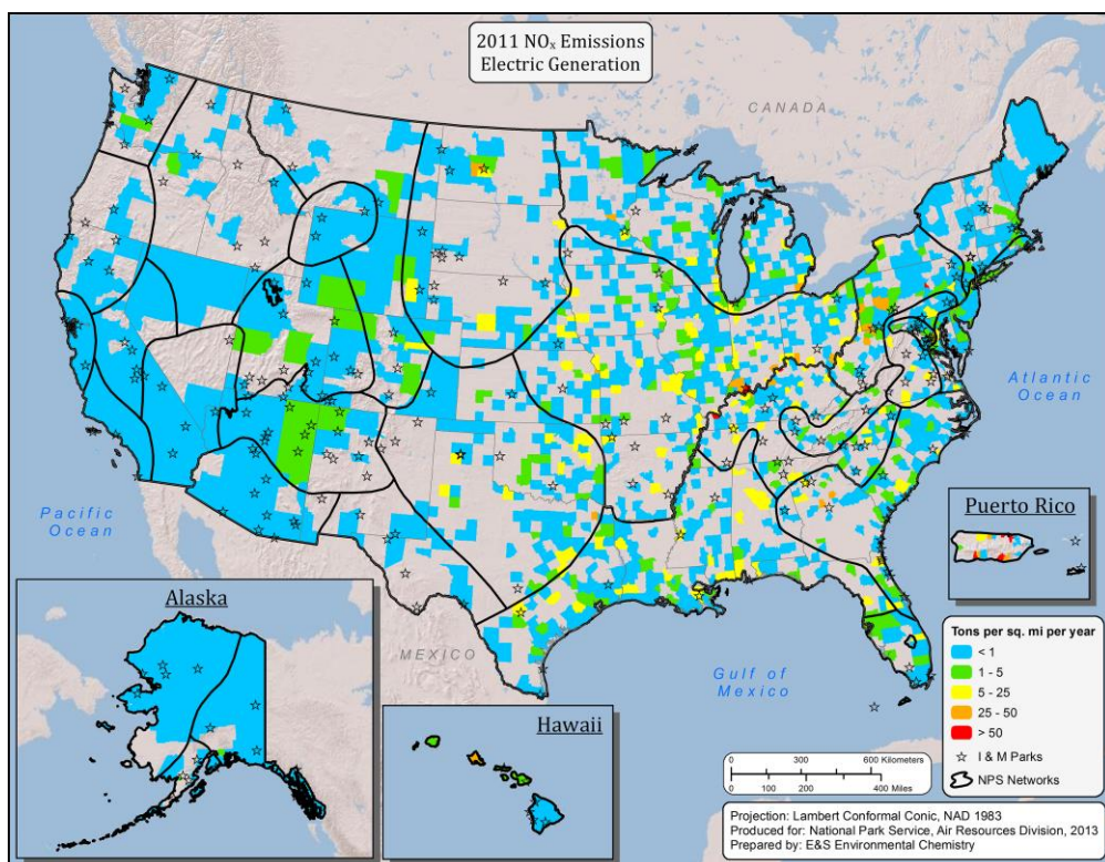
Map A-7. Total NO x emissions, by county, attributable to the electricity generation sector for the years a) 2002 and b) 2011, based on data from the NEI.
