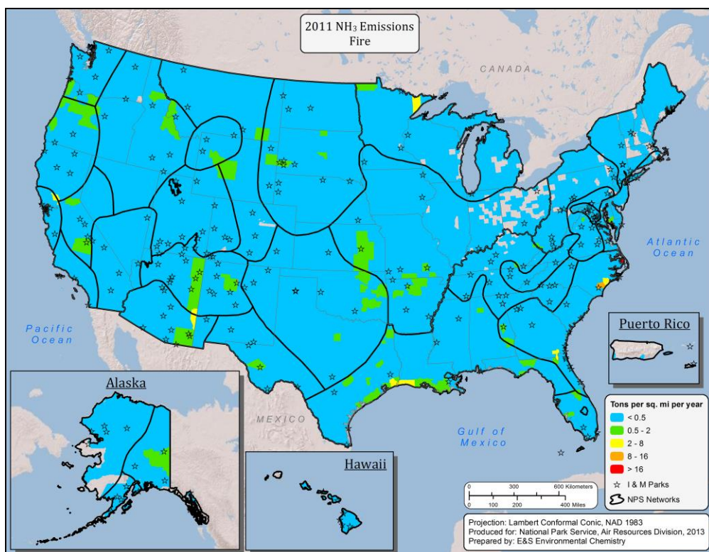
Map A-12. Total NH 3 emissions, by county, attributable to fire for the years a) 2002 and b) 2011, based on data from the NEI.
