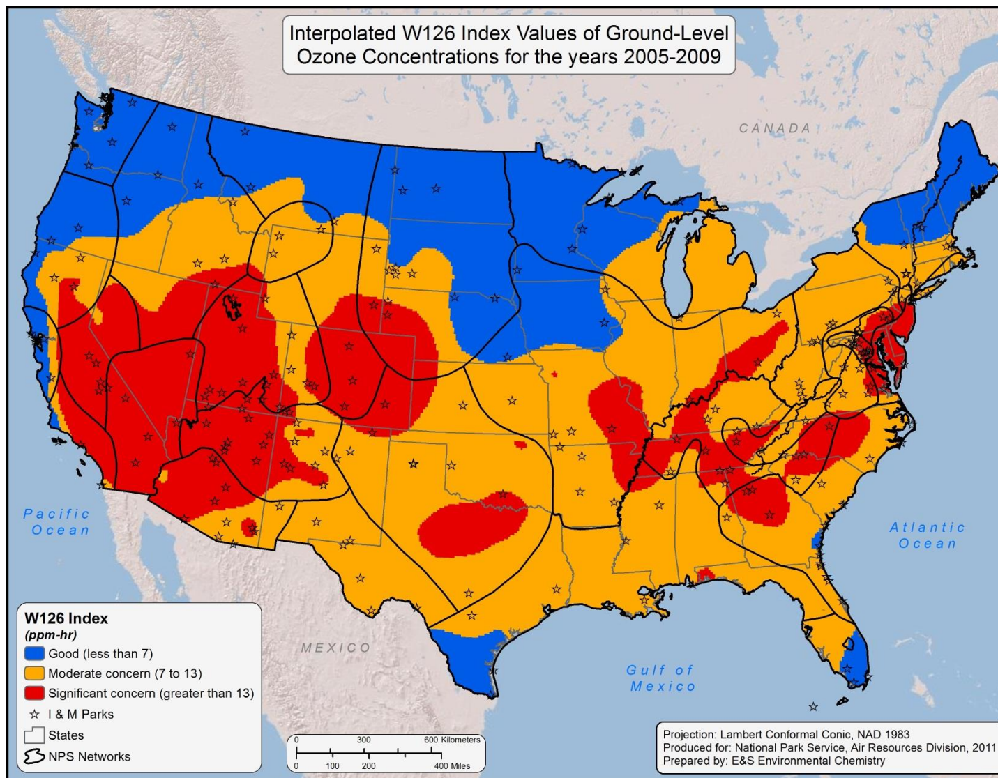
Map 20. Interpolated values of cumulative ozone exposure during the five-year period 2005 through 2009 using the W126-3 mo exposure index.
