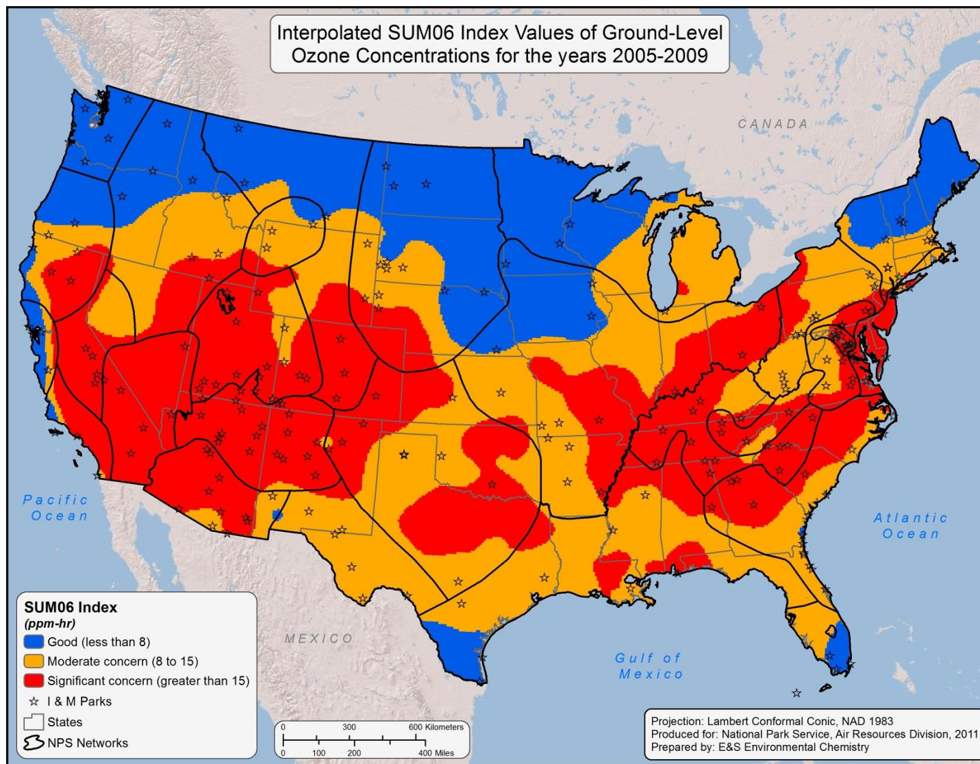
Map 21. Interpolated values of cumulative ozone exposure during the five-year period 2005 through 2009 using the SUM06 exposure index.
