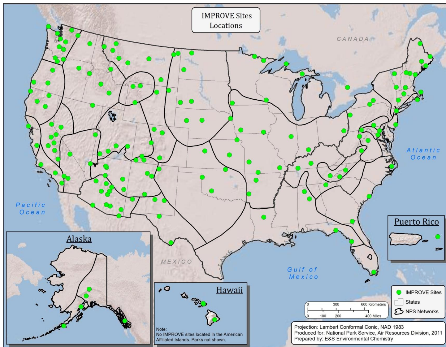
Map 22. Locations of IMPROVE air quality monitoring sites. Also shown are boundaries of park networks.
