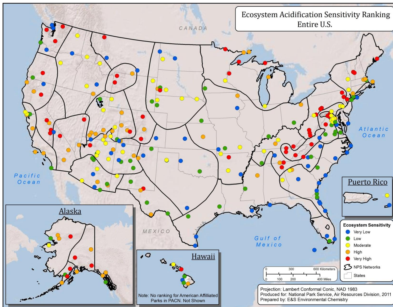
Map 16. Park-specific rankings of I&M parks with respect to inherent Ecosystem Sensitivity to acidification. (Source: Sullivan et al. 2011b)
