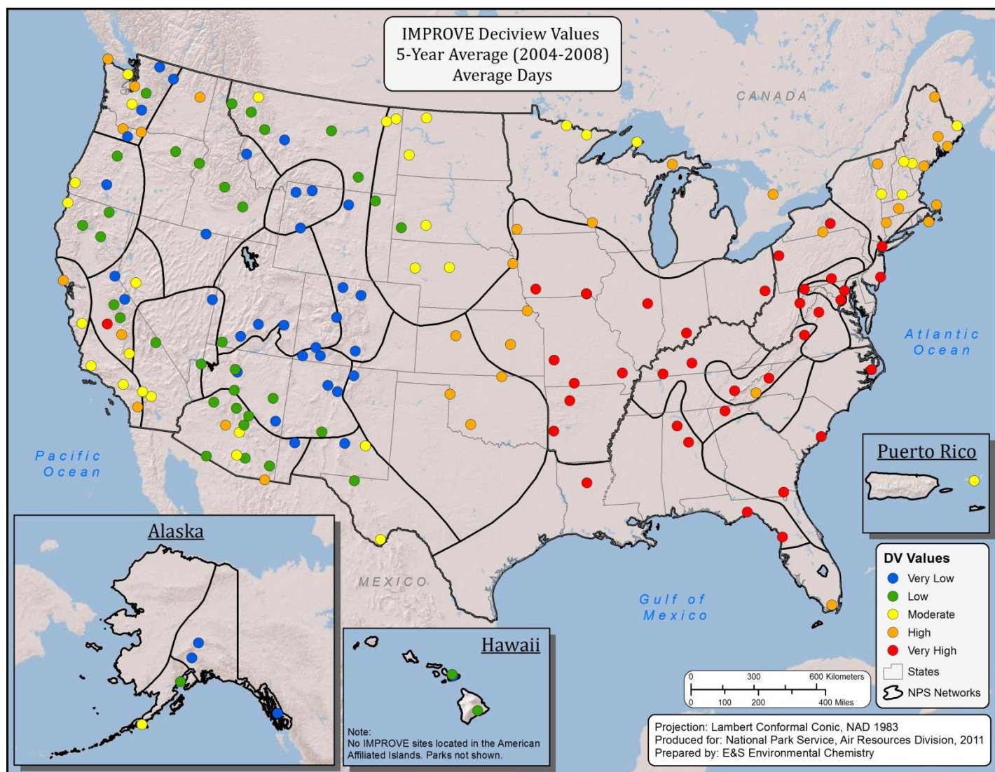
Map 25. Relative ranking of haze measurements at IMPROVE sites, based on the average days at each site. Low dv values correspond to better visibility; as dv increases, visibility decreases.
