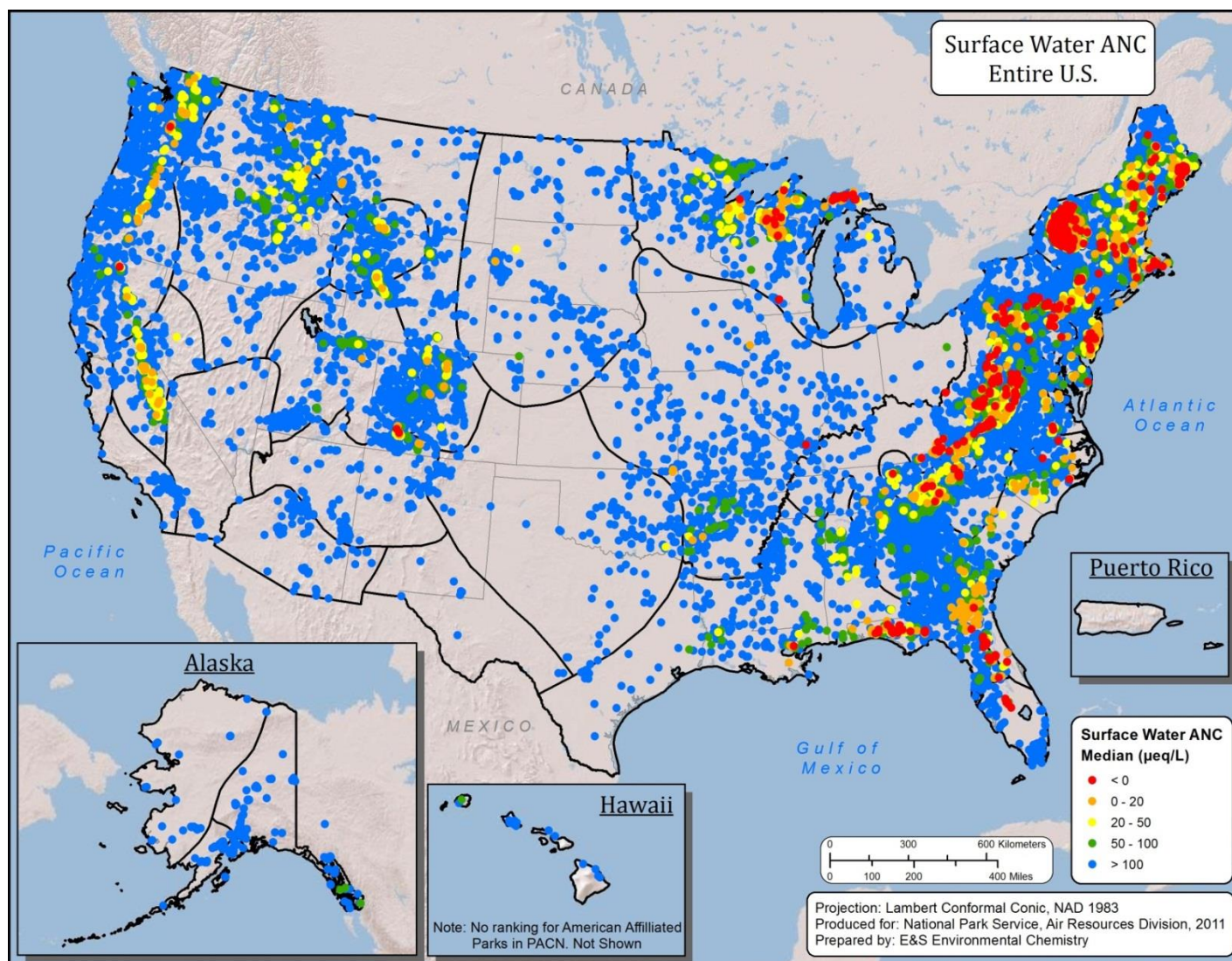
Map 14a. Surface water ANC map, based on data compiled from the data sources listed in Table 10.
