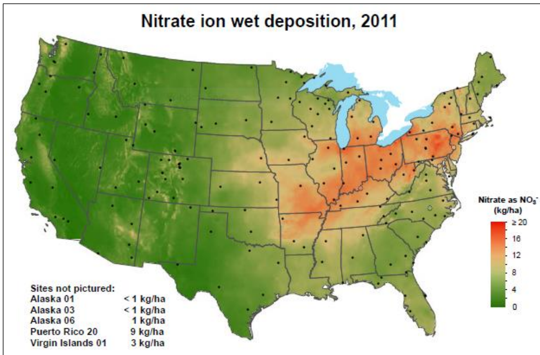
Map 7. Wet \text{NO}_3^- deposition throughout the United States for the most recent year available at the time of this writing. (Source: NADP/NTN) Black dots mark site locations that meet NADP completeness criteria. Open circles designate urban sites, defined as having at least 400 people per square kilometer within a 15-km radius of the site. Urban sites do not contribute to the contour surface.
