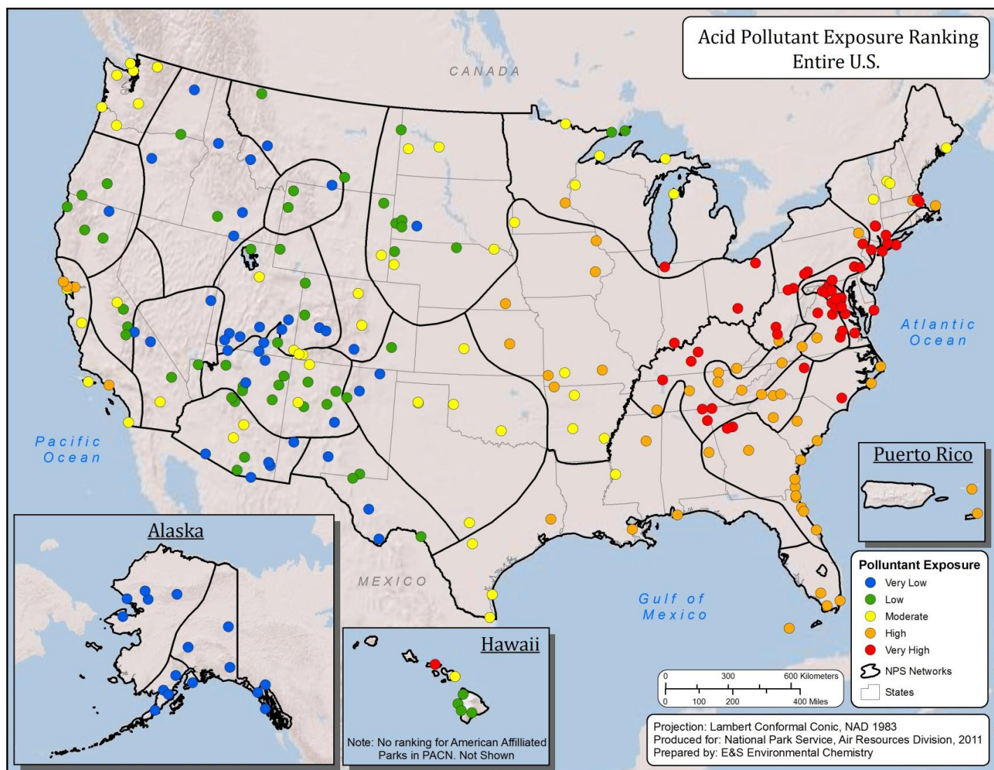
Map 15. Park-specific rankings of I&M parks with respect to acid Pollutant Exposure. (Source: Sullivan et al. 2011b)
