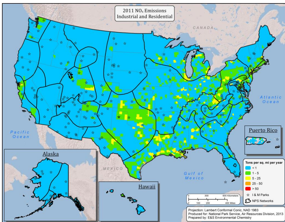
Map A-9. Total NO x emissions, by county, attributable to the industrial and residential sector for the years a) 2002 and b) 2011, based on data from the NEI.
