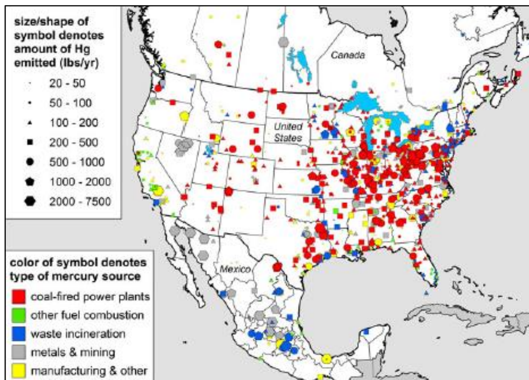
Map 5. Distribution of total Hg annual emissions from point sources in the United States, Canada, and Mexico. Total number of point sources in inventory is 15,892, which equals 155 tons/year (310,000 lbs/yr). Point sources not mapped are those under 20 lbs/year ( n = 3,508 ). Point source emissions in Alaska and Hawaii are minor (under 20 lbs/year) and not depicted here. (Source: Schmeltz et al. 2011)
