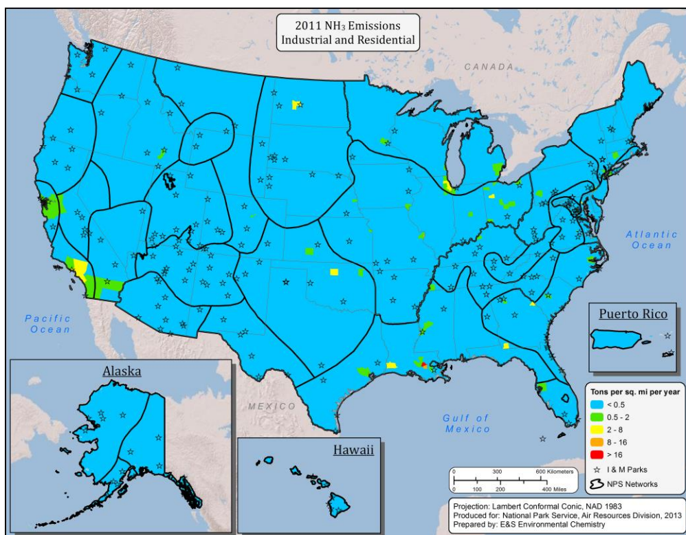
Map A-13. Total NH 3 emissions, by county, attributable to the industrial and residential sector for the years a) 2002 and b) 2011, based on data from the NEI.
