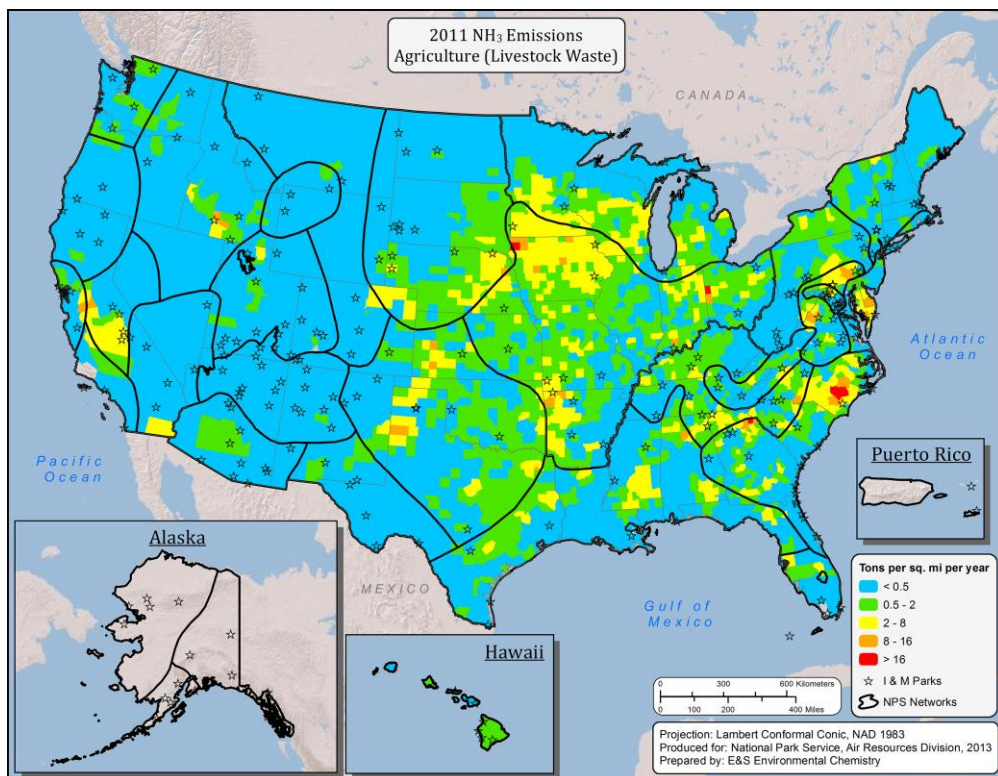
Map A-10. Total NH 3 emissions, by county, attributable to agriculture (livestock waste) for the years a) 2002 and b) 2011, based on data from the NEI.
