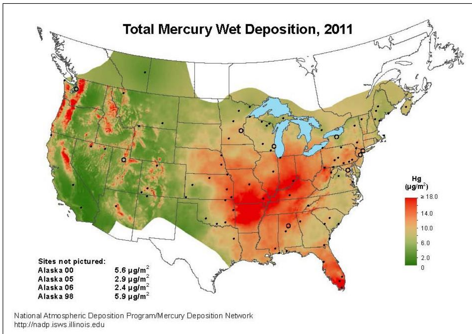
Map 9. Interpolated wet Hg deposition for 2011 determined by the Mercury Deposition Network. (Source: NADP MDN) Black dots mark site locations that meet NADP completeness criteria. Open circles designate urban sites, defined as having at least 400 people per square kilometer within a 15-km radius of the site. Urban sites do not contribute to the contour surface.
