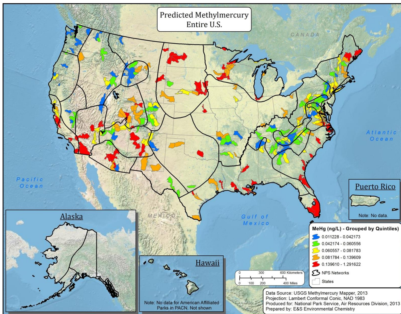
Map 26. Predicted MeHg concentrations in surface waters throughout the conterminous United States by HUCs that contain national parklands. Estimates were generated by USGS (Last modified February 20, 2015). Rankings are based on quintile distributions across all I&M parks having estimates by USGS.
