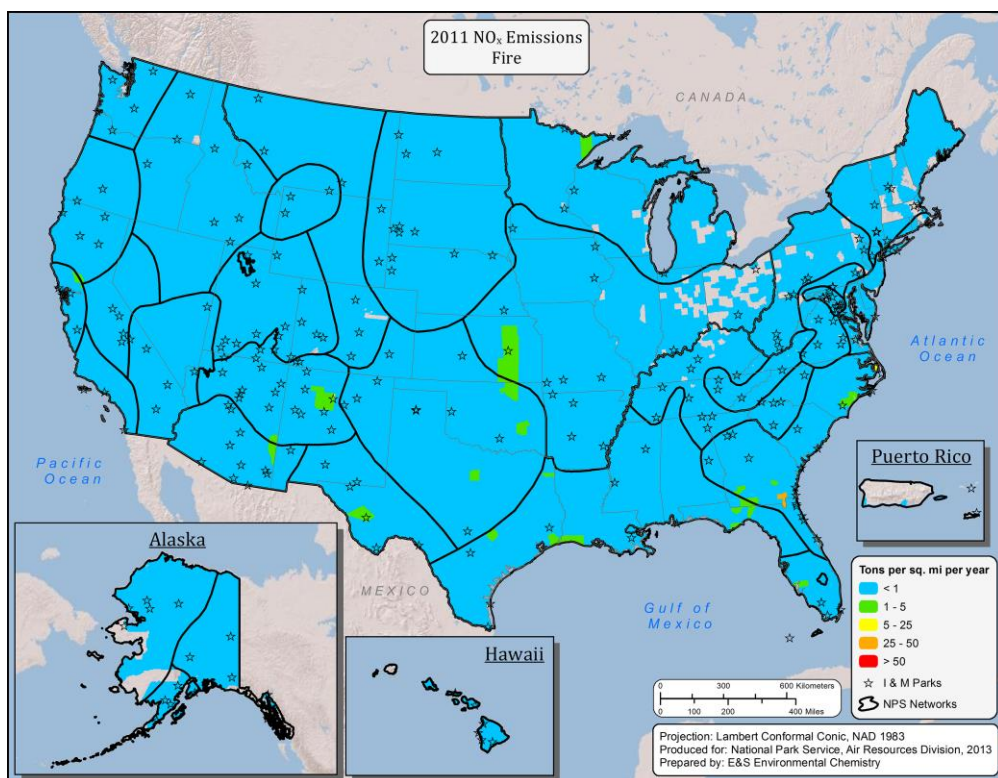
Map A-8. Total NO x emissions, by county, attributable to fire for the years a) 2002 and b) 2011, based on data from the NEI.
