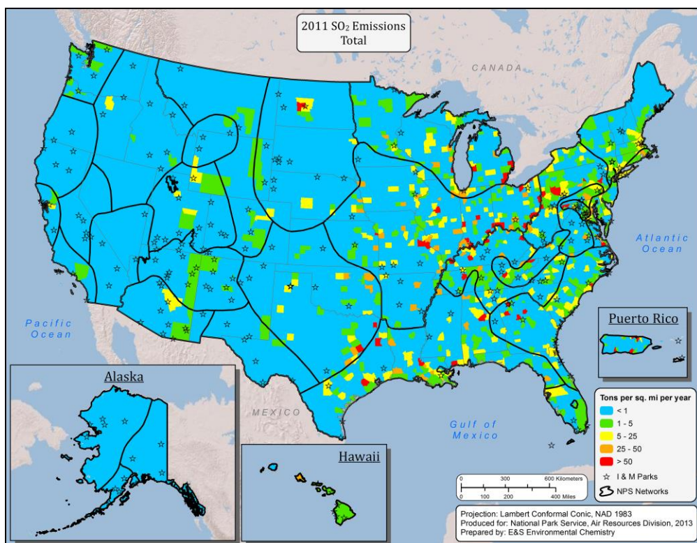
Map 2. Total SO 2 emissions, by county, for the years a) 2002 and b) 2011, based on data from the NEI.
