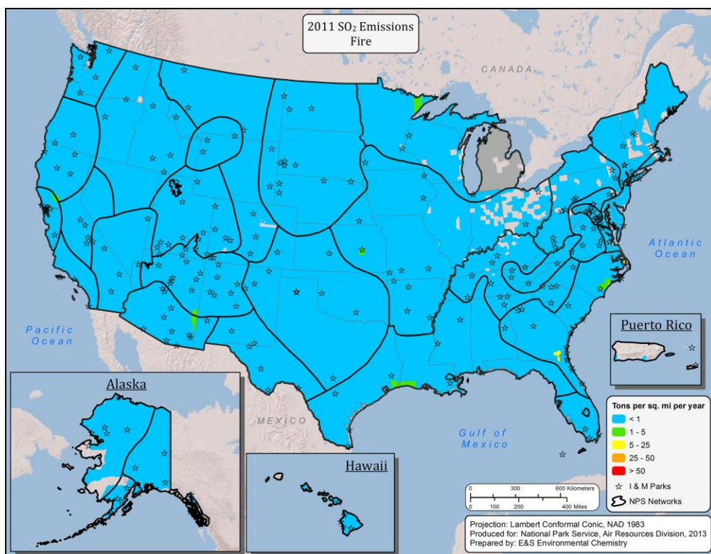
Map A-2. Total SO 2 emissions, by county, attributable to fire, for the years a) 2002 and b) 2011, based on data from the NEI.
