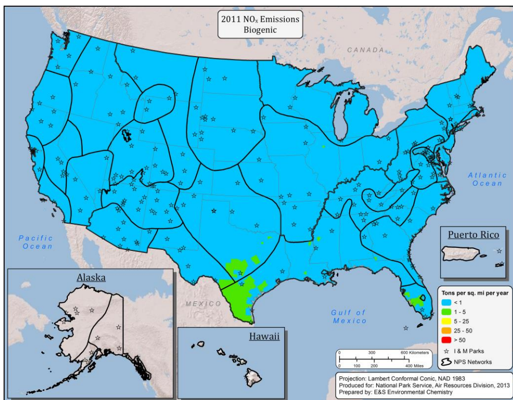
Map A-6. Total NO x emissions, by county, attributable to biogenics for the years a) 2002 and b) 2011, based on data from the NEI.
