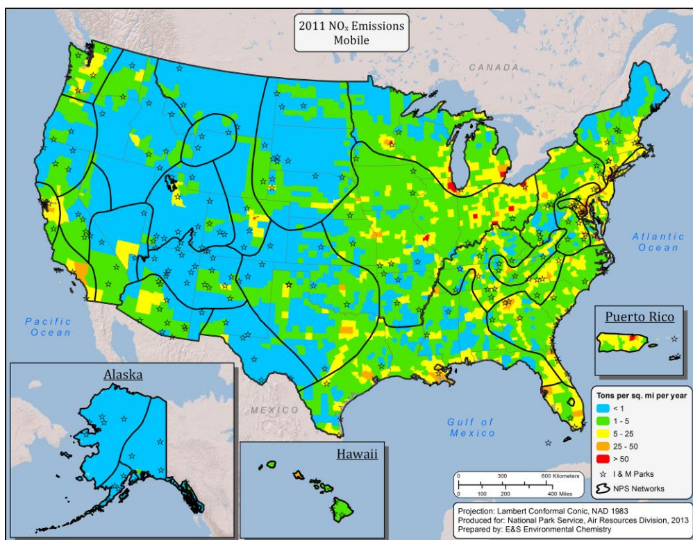
Map A-5. Total NO x emissions, by county, attributable to the mobile sector for the years a) 2002 and b) 2011, based on data from the NEI.
