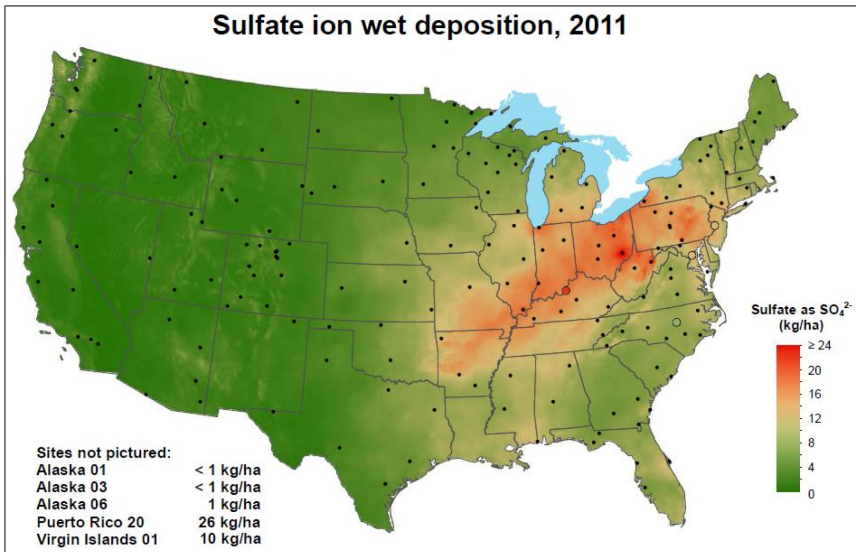
Map 6. Wet \text{SO}_4^{2-} deposition throughout the United States for the most recent year available at the time of this writing. (Source: NADP/NTN) Black dots mark site locations that meet NADP completeness criteria. Open circles designate urban sites, defined as having at least 400 people per square kilometer within a 15-km radius of the site. Urban sites do not contribute to the contour surface.
