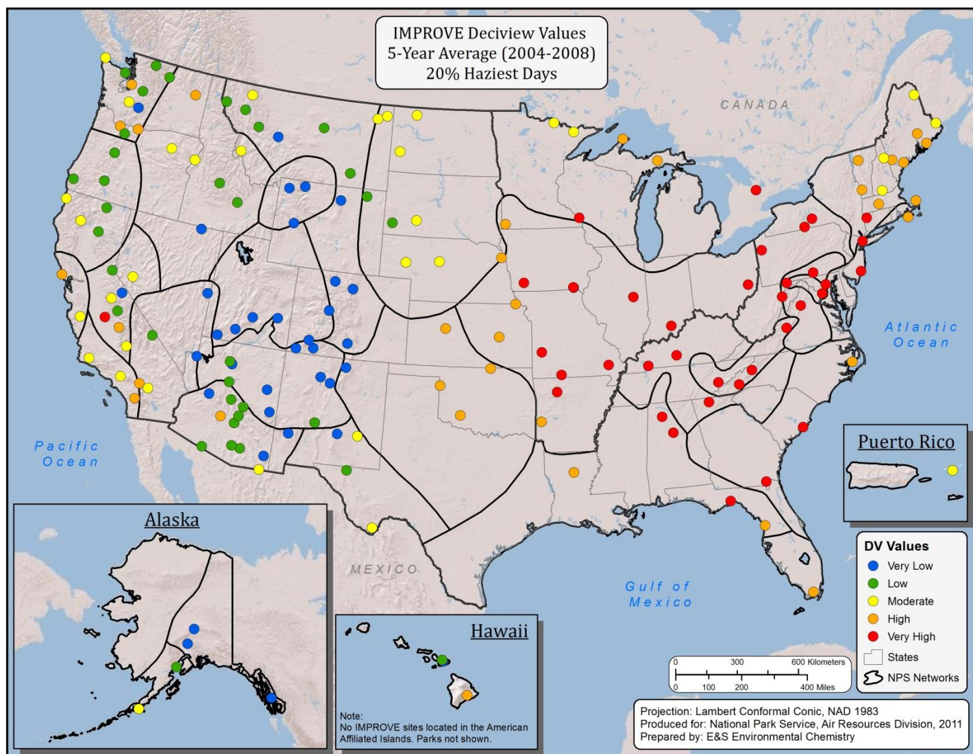
Map 24. Relative ranking of haze measurements at IMPROVE sites for the 20% haziest days during the five-year period 2004 through 2008 . Low dv values correspond to better visibility; as dv increases, visibility decreases.
