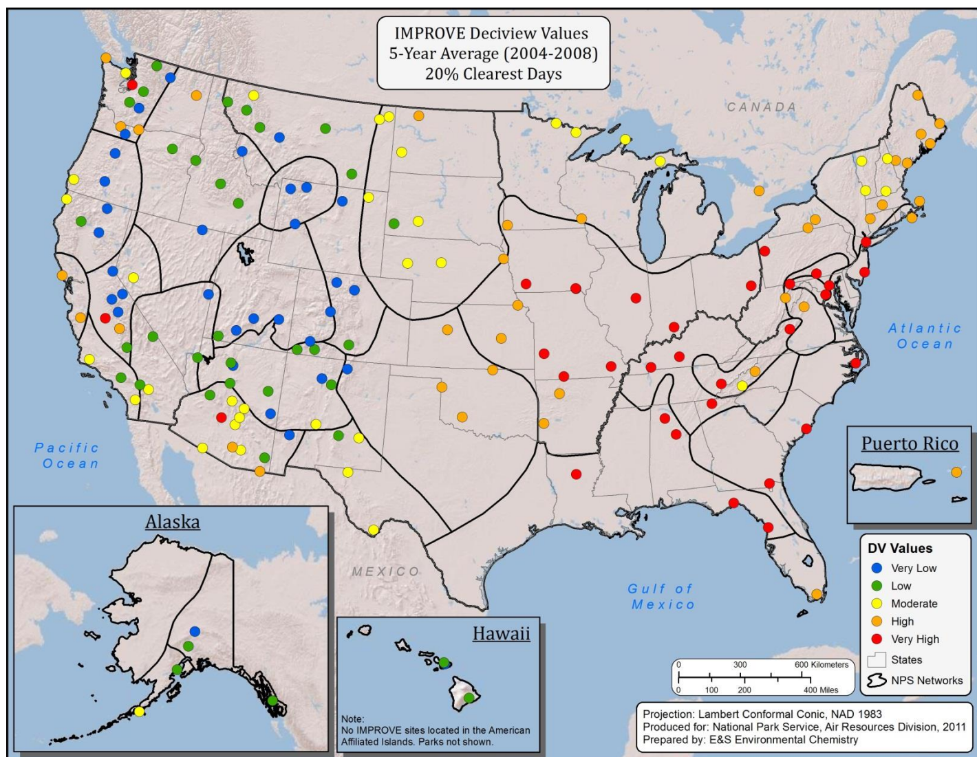
Map 23. Relative ranking of haze measurements at IMPROVE sites for the 20% clearest days during the five-year period 2004 through 2008. Low dv values correspond to better visibility; as dv increases, visibility decreases.
