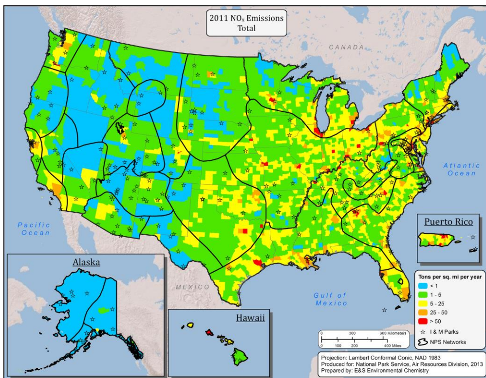
Map 3. Total NO x emissions, by county, for the years a) 2002 and b) 2011, based on data from the NEI.
