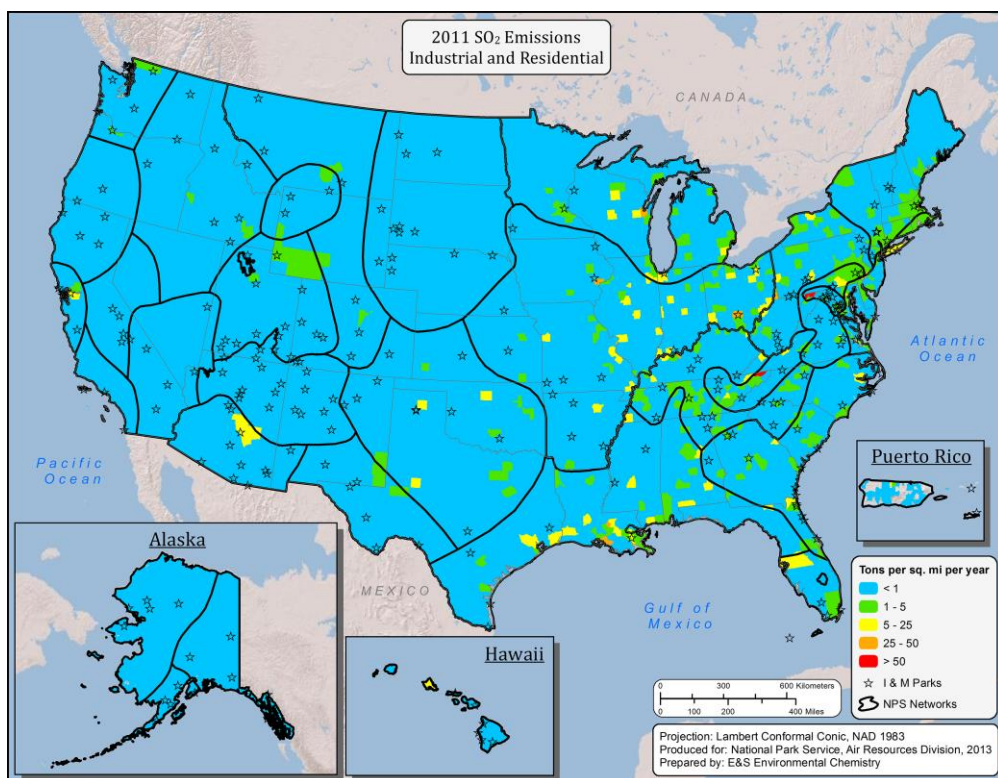
Map A-3. Total SO 2 emissions, by county, attributable to the industrial and residential sector, for the years a) 2002 and b) 2011, based on data from the NEI.
