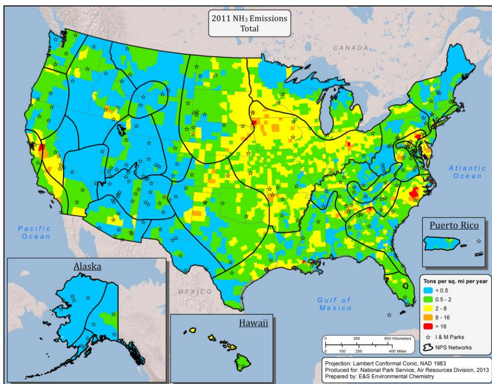
Map 4. Total NH 3 emissions, by county, for the years a) 2002 and b) 2011, based on data from the NEI.
