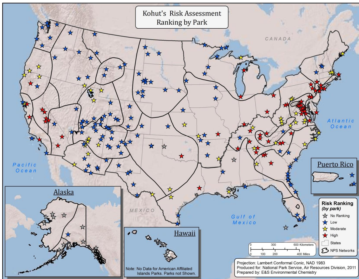
Map 19. Risk ranking for exposure of vegetation in I&M parks throughout the United States to ground-level ozone. (Source of data: Kohut 2007b).
