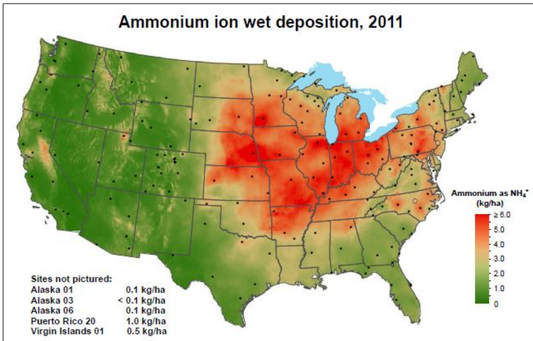
Map 8. Wet \text{NH}_4^+ deposition throughout the United States for the most recent year available at the time of this writing. (Source: NADP/NTN) Black dots mark site locations that meet NADP completeness criteria. Open circles designate urban sites, defined as having at least 400 people per square kilometer within a 15-km radius of the site. Urban sites do not contribute to the contour surface.
