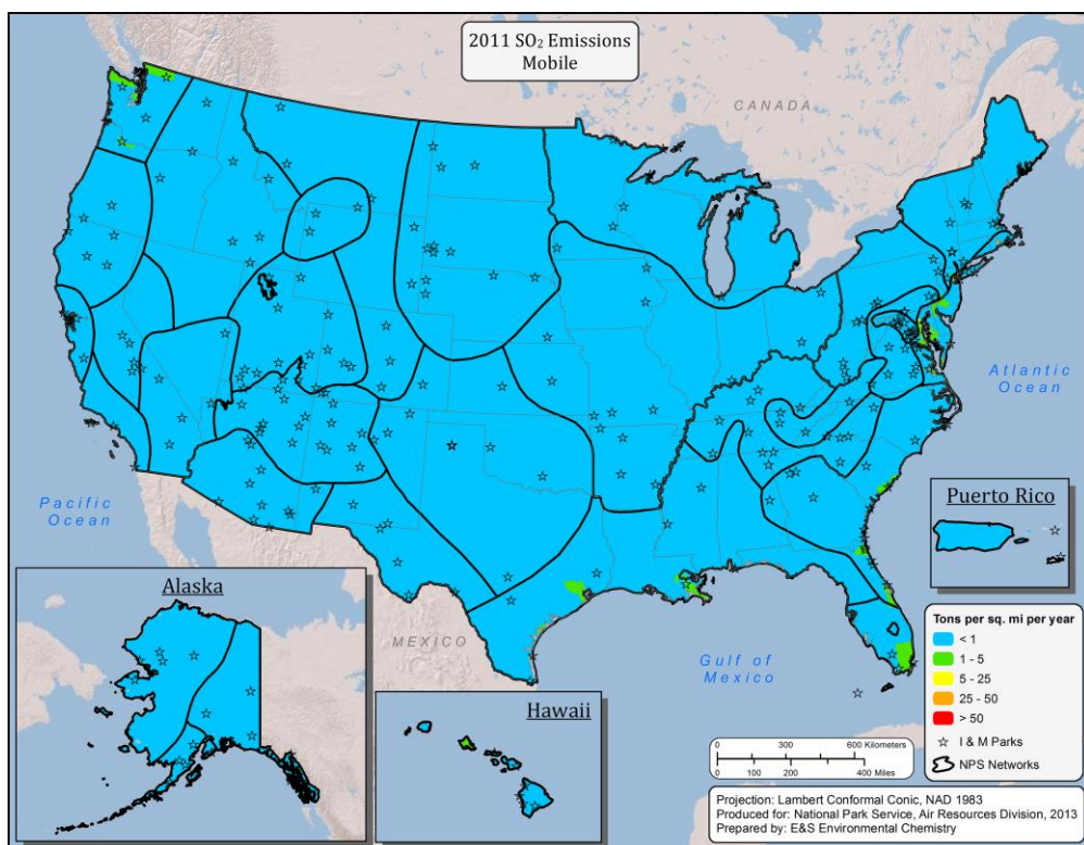
Map A-4. Total SO 2 emissions, by county, attributable to the mobile sector, for the years a) 2002 and b) 2011, based on data from the NEI.
