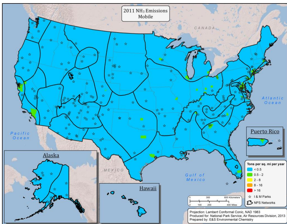
Map A-14. Total NH 3 emissions, by county, attributable to the mobile sector for the years a) 2002 and b) 2011, based on data from the NEI.
