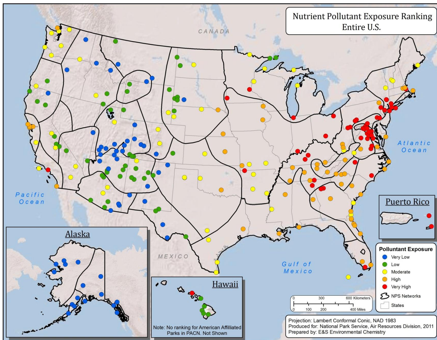
Map 17. Park-specific rankings of I&M parks with respect to nutrient N Pollutant Exposure. (Source: Sullivan et al. 2011a)
