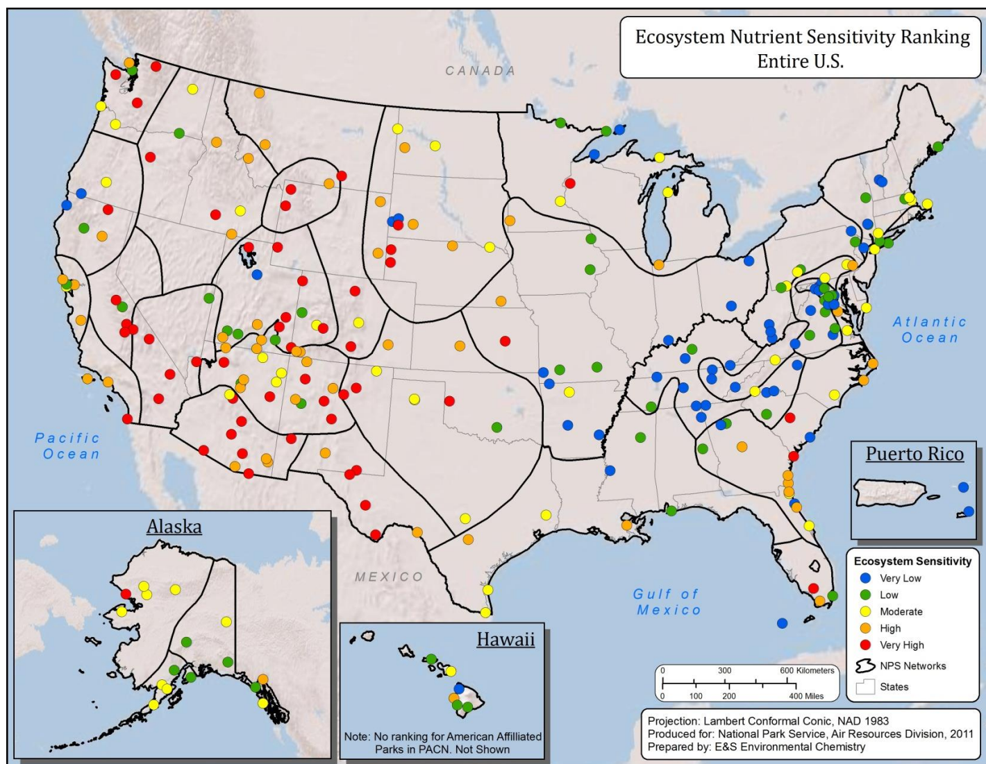
Map 18. Park-specific rankings of I&M parks with respect to inherent Ecosystem Sensitivity to nutrient enrichment. (Source: Sullivan et al. 2011a)
