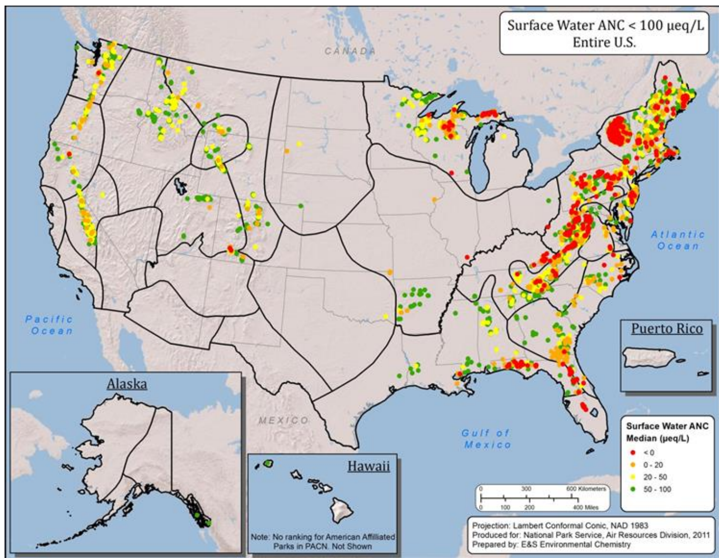
Map 14b. Surface water ANC map, shown as a subset of data represented in Map 14a, but only showing sites having median ANC \leq 100 µeq/L.
