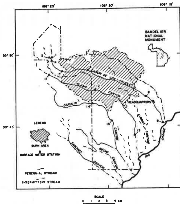
Fig. 1. La Mesa fire and surface water sampling stations.
