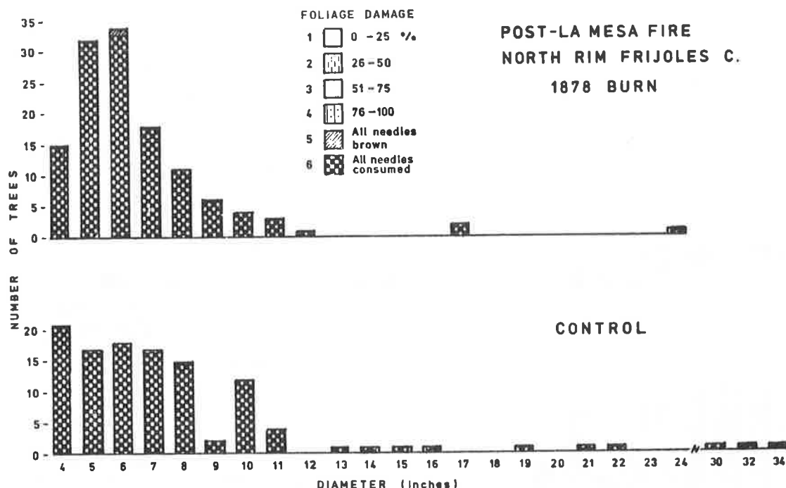
Fig. 8. Relative foliar damage in six categories to mature ponderosa pine on North Rim Frijoles Canyon based on the line-strip plots, 1977.
