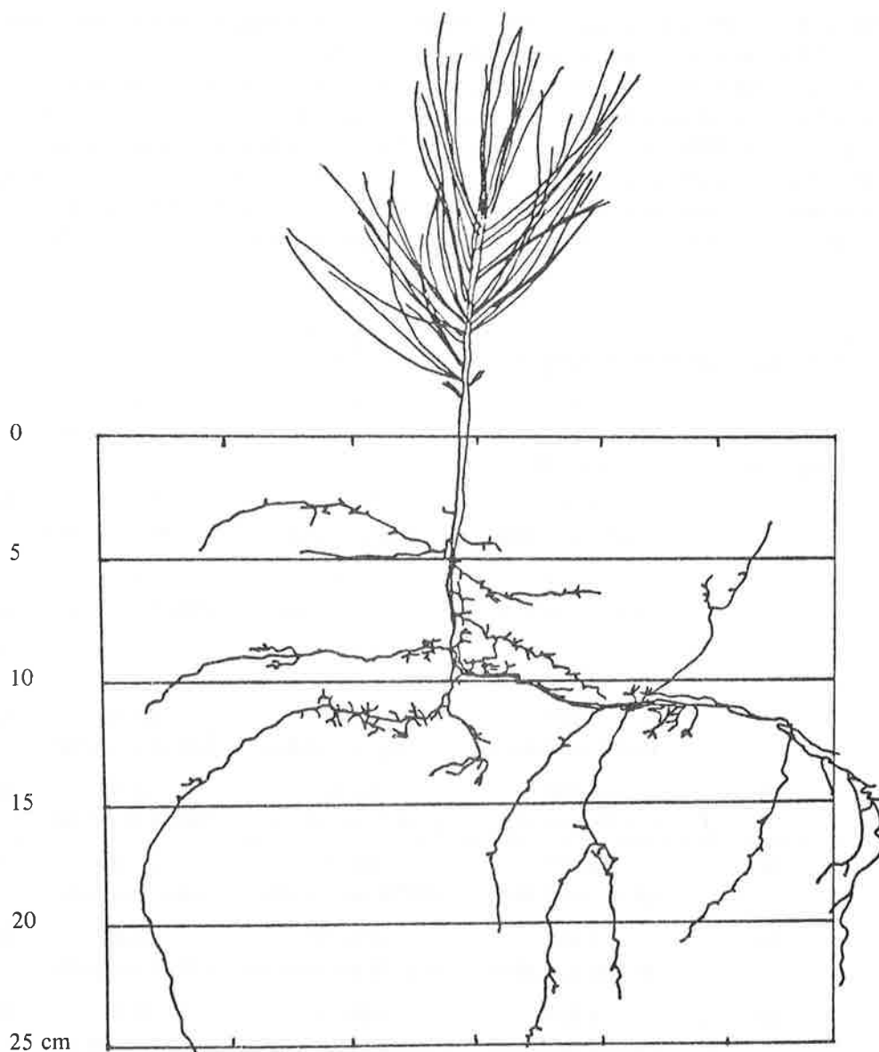
Fig. 10. Root structure of 3-year-old P. ponderosa seedling.
