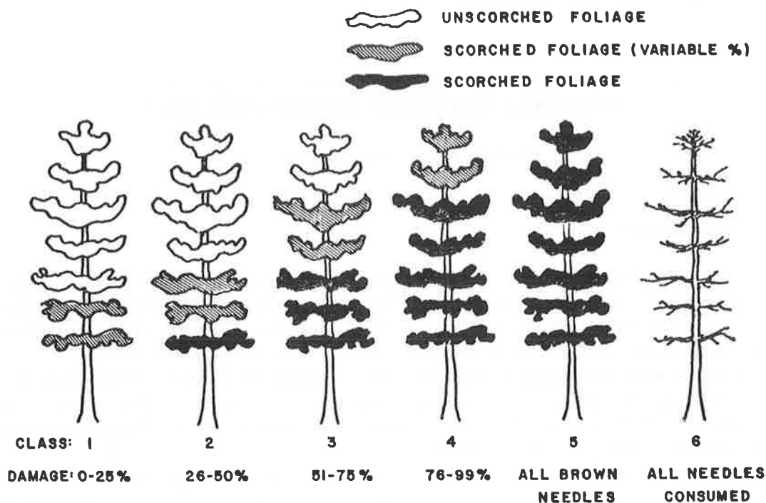
Fig. 1. Foliar damage categories.
