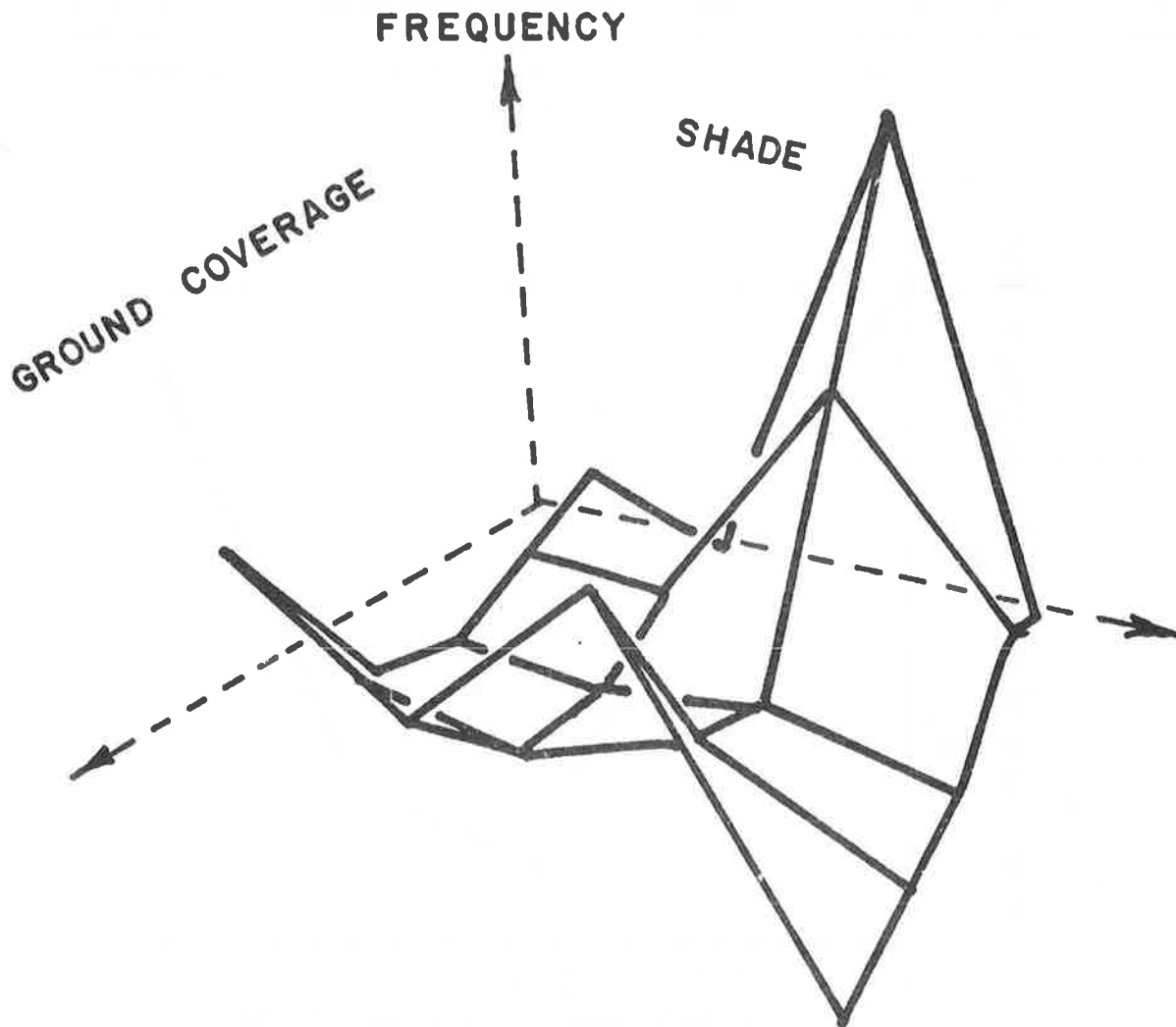
Fig. 10. Relationship between potential shade, ground cover, and ponderosa pine seedling frequency.
