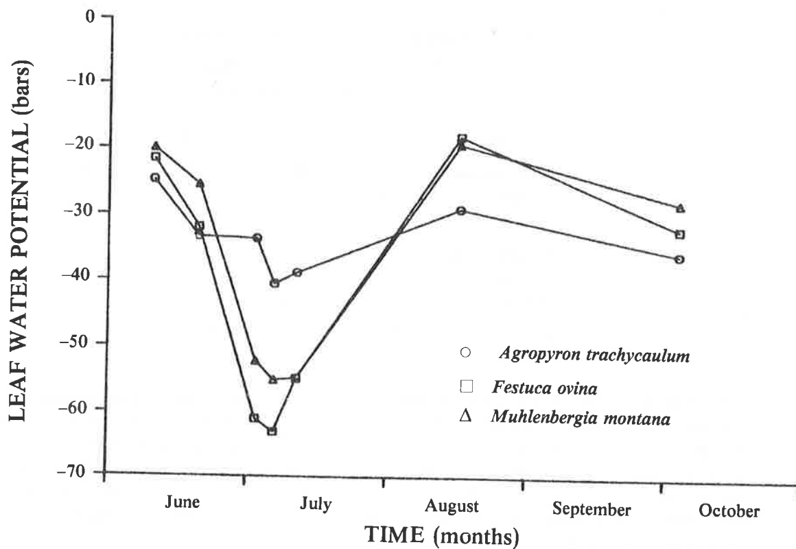
Fig. 3. Seasonal changes in LWP at site 4.
