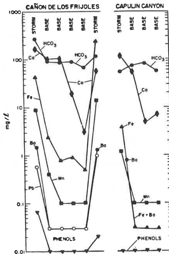
Fig. 4. Base flow and storm runoff chemical constituent variations in Cañon de los Frijoles and Capulin Canyon after La Mesa fire.
