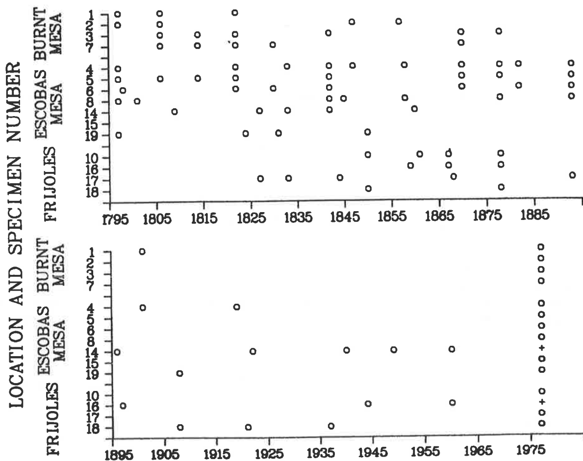
Fig. 3. Fire frequency of fifteen fire-scarred trees.
