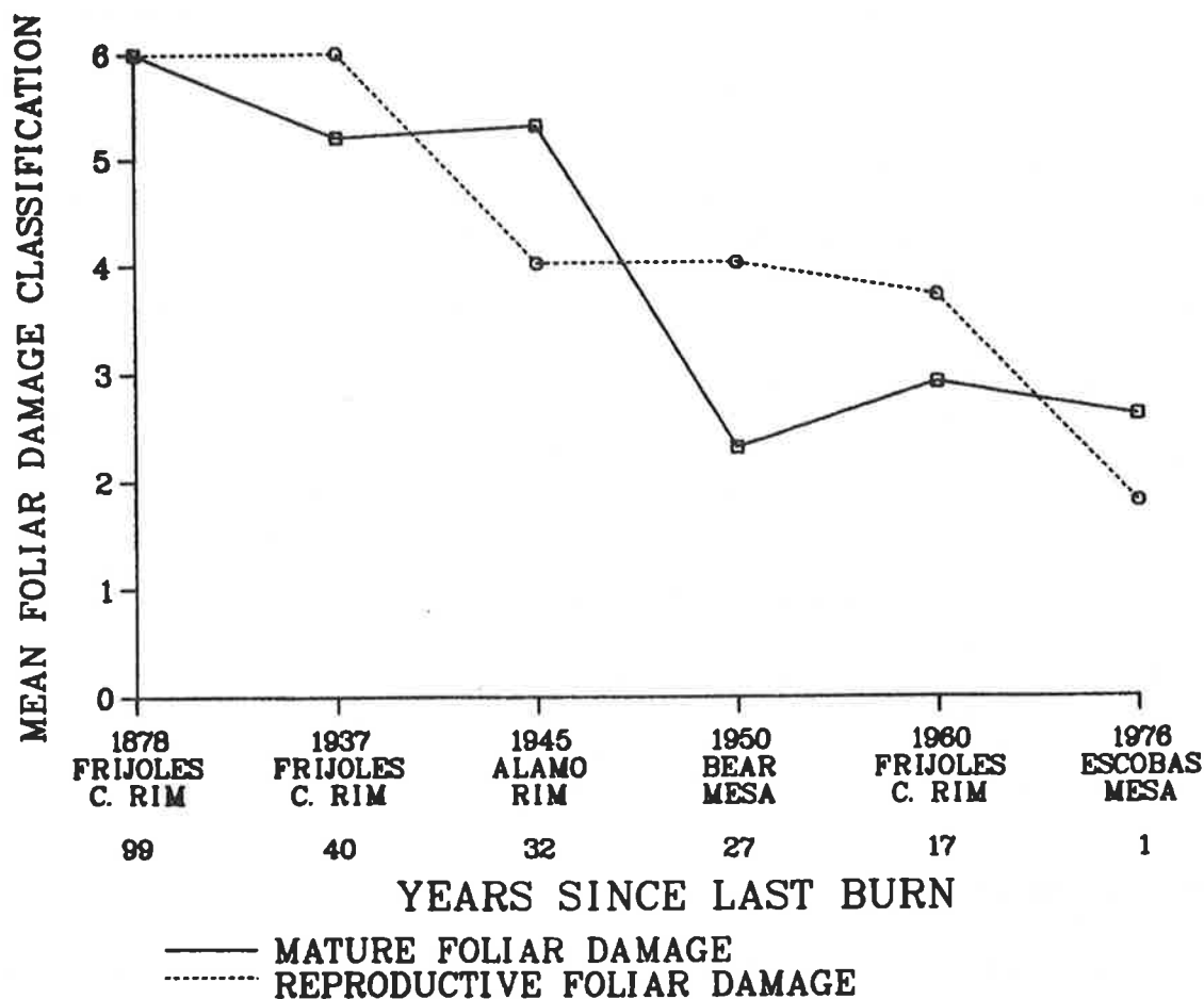
Fig. 11. Effect of fire interval on foliage in six plateau stands of ponderosa pine.
