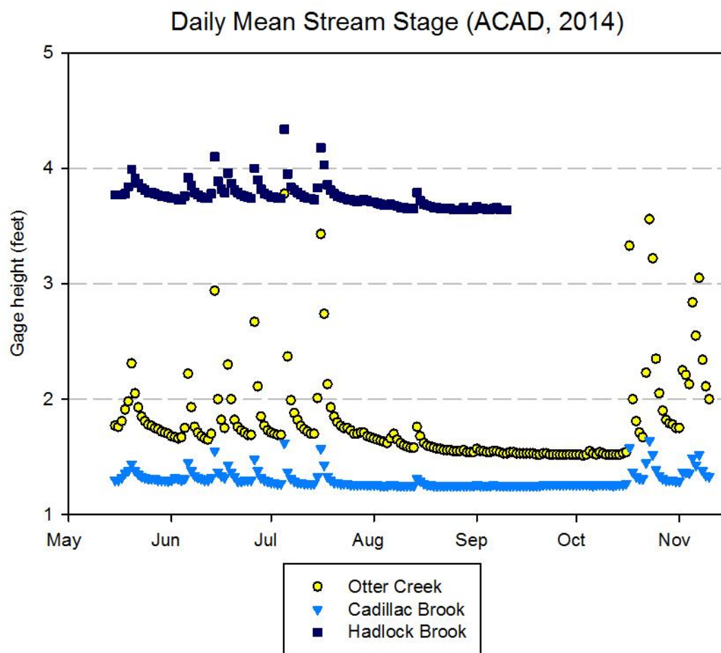
Figure 34. Daily mean stream stage measured in 2014 at NETN permanent record stream monitoring sites in Acadia NP.
