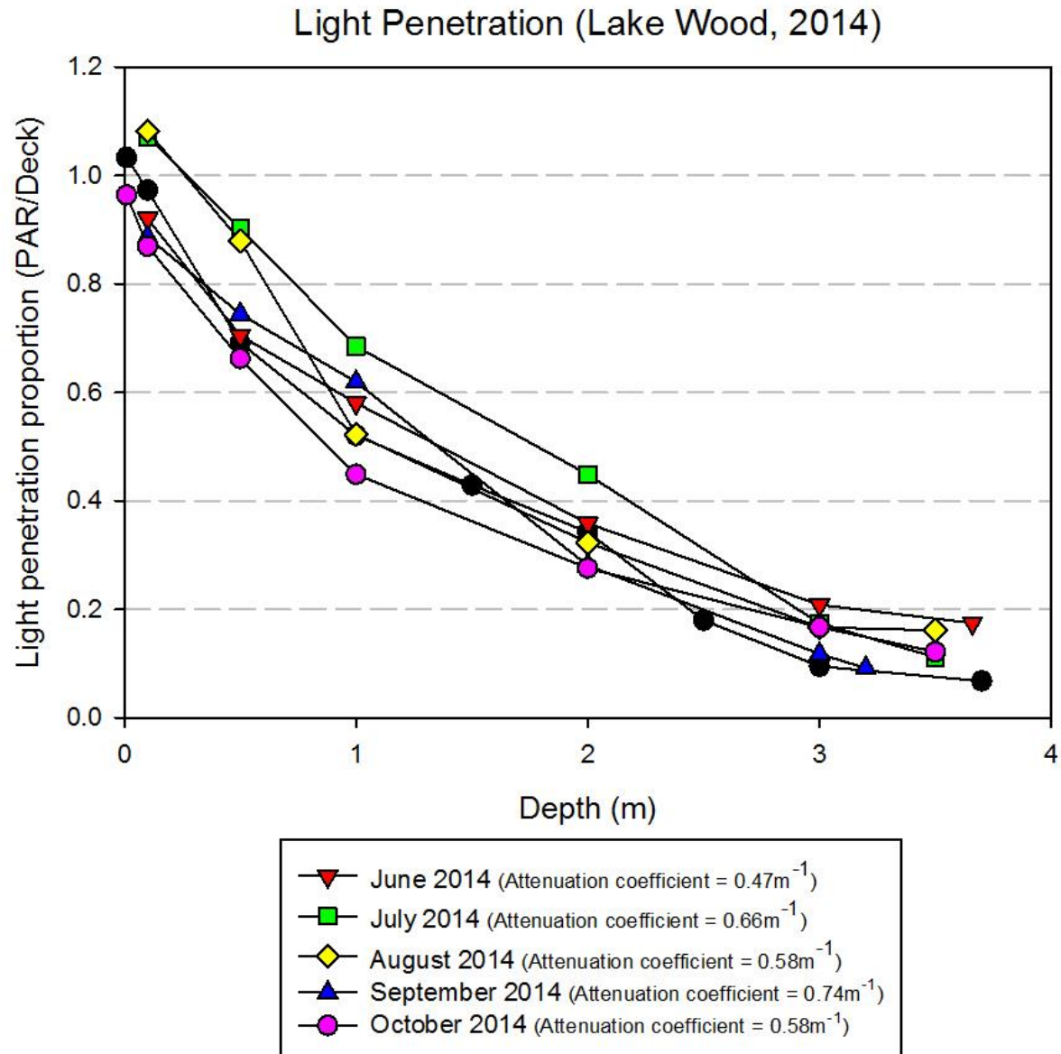
Figure 19. Light penetration profiles from Lake Wood.
