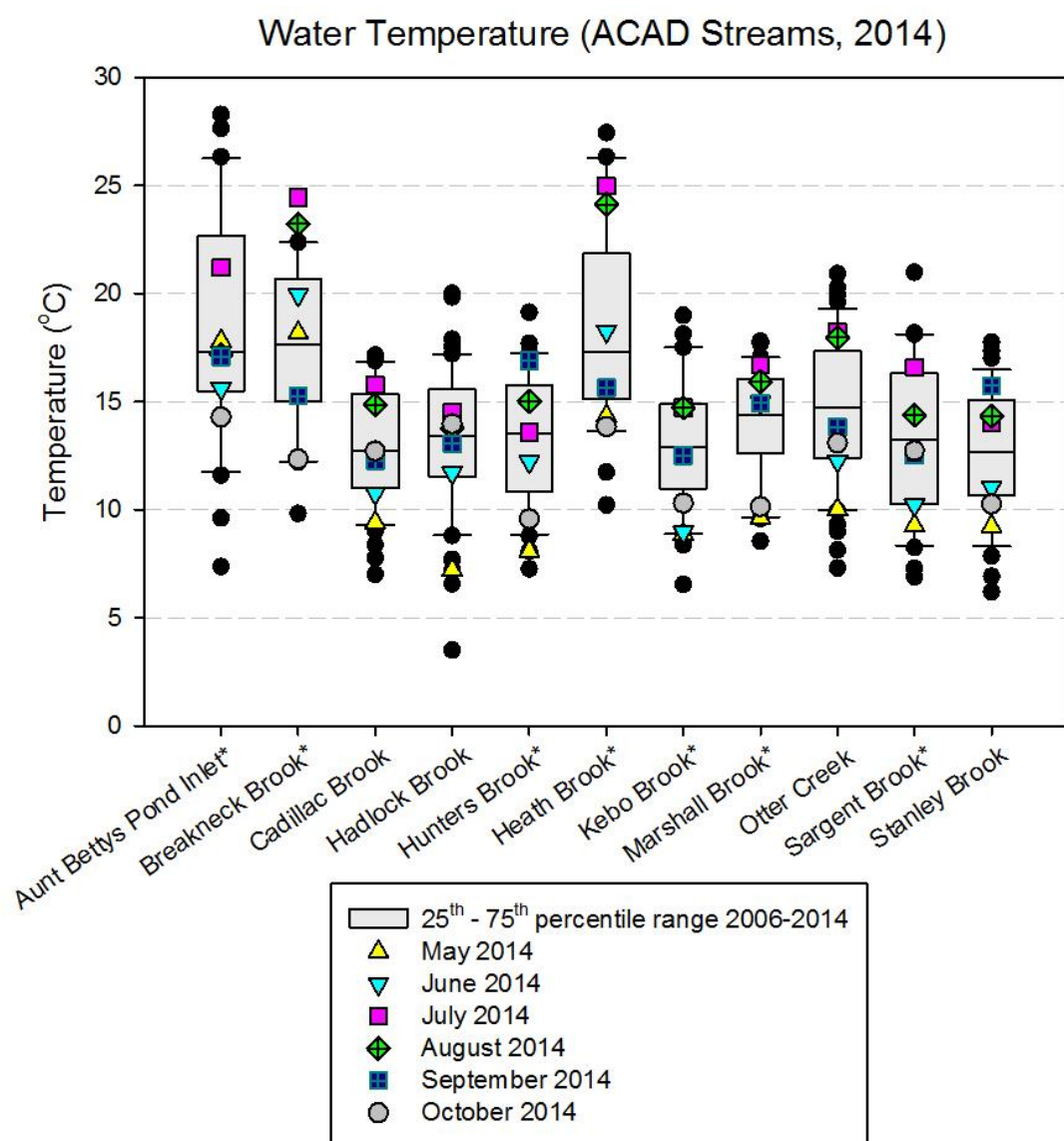
Figure 8. Stream water temperature (surface) from 2014 YSI sonde in-situ measurements overlaid on a box plot of measurements taken from 2006-2014. Sites marked with an asterisk (*) are rotating partial-record sites with data from 2006, 2008, 2010, 2012, and 2014 only.
