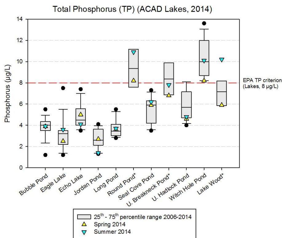
Figure 23. Lake and pond total phosphorus (TP) from 2014 spring and summer water samples. The data are overlaid on a box plot of measurements taken from 2006-2014. Sites marked with an asterisk (*) are
