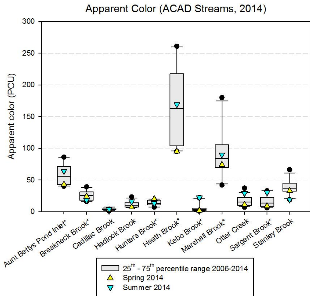
Figure 14. Stream apparent color from 2014 spring and summer water samples overlaid on a box plot of measurements taken from 2006-2014. Sites marked with an asterisk (*) are rotating partial-record sites with data from 2006, 2008, 2010, 2012, and 2014 only.
