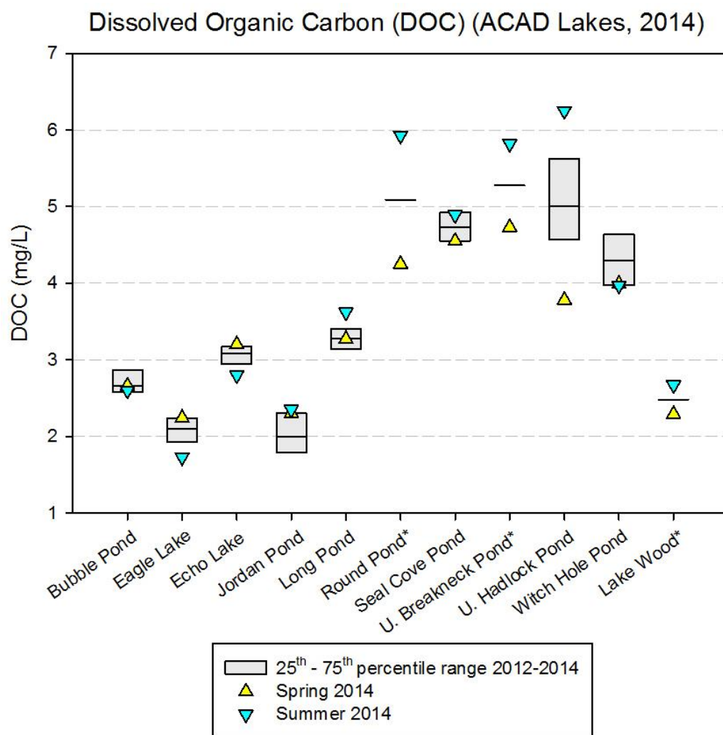
Figure 15. Lake and pond dissolved organic carbon (DOC) from 2014 spring and summer water samples overlaid on a box plot of measurements taken from 2012-2014. Sites marked with an asterisk (*) are rotating sites with data from 2014 only.
