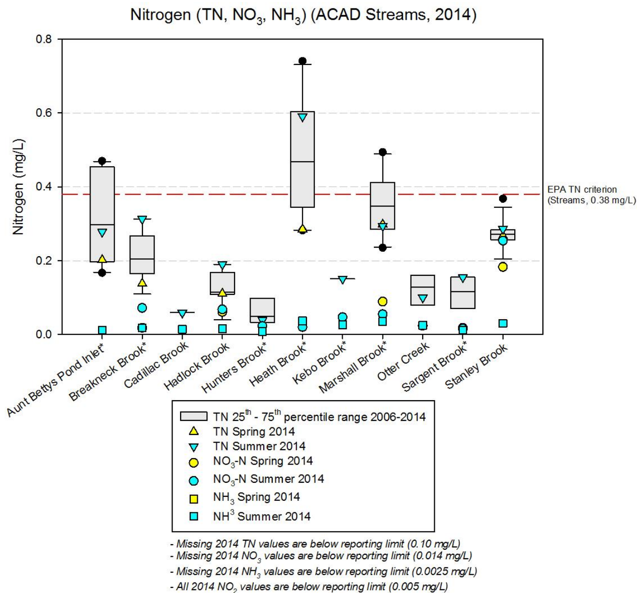
Figure 26. Stream total nitrogen (TN) and the nitrogen component of nitrate ( \text{NO}_3\text{-N} ) and ammonia ( \text{NH}_3 ) from 2014 spring and summer water samples. The data are overlaid on a box plot of TN measurements taken from 2006-2014. Sites marked with an asterisk (*) are rotating partial-record sites with data from 2006, 2008, 2010, 2012, and 2014 only.
