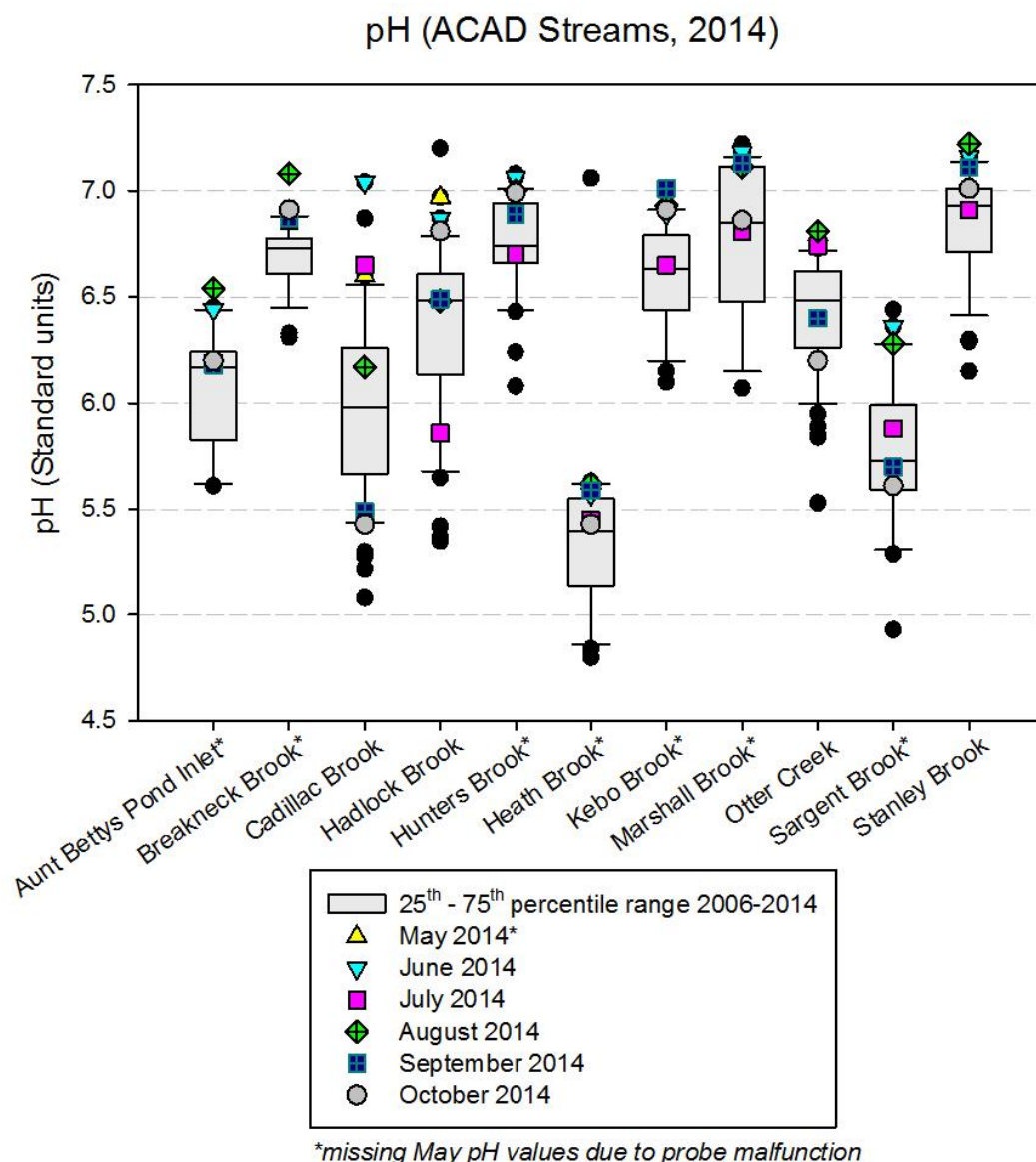
Figure 6. Stream pH from 2014 YSI sonde in-situ measurements overlaid on a box plot of measurements taken from 2006-2014. Sites marked with an asterisk (*) are rotating partial-record sites with data from 2006, 2008, 2010, 2012, and 2014 only.
