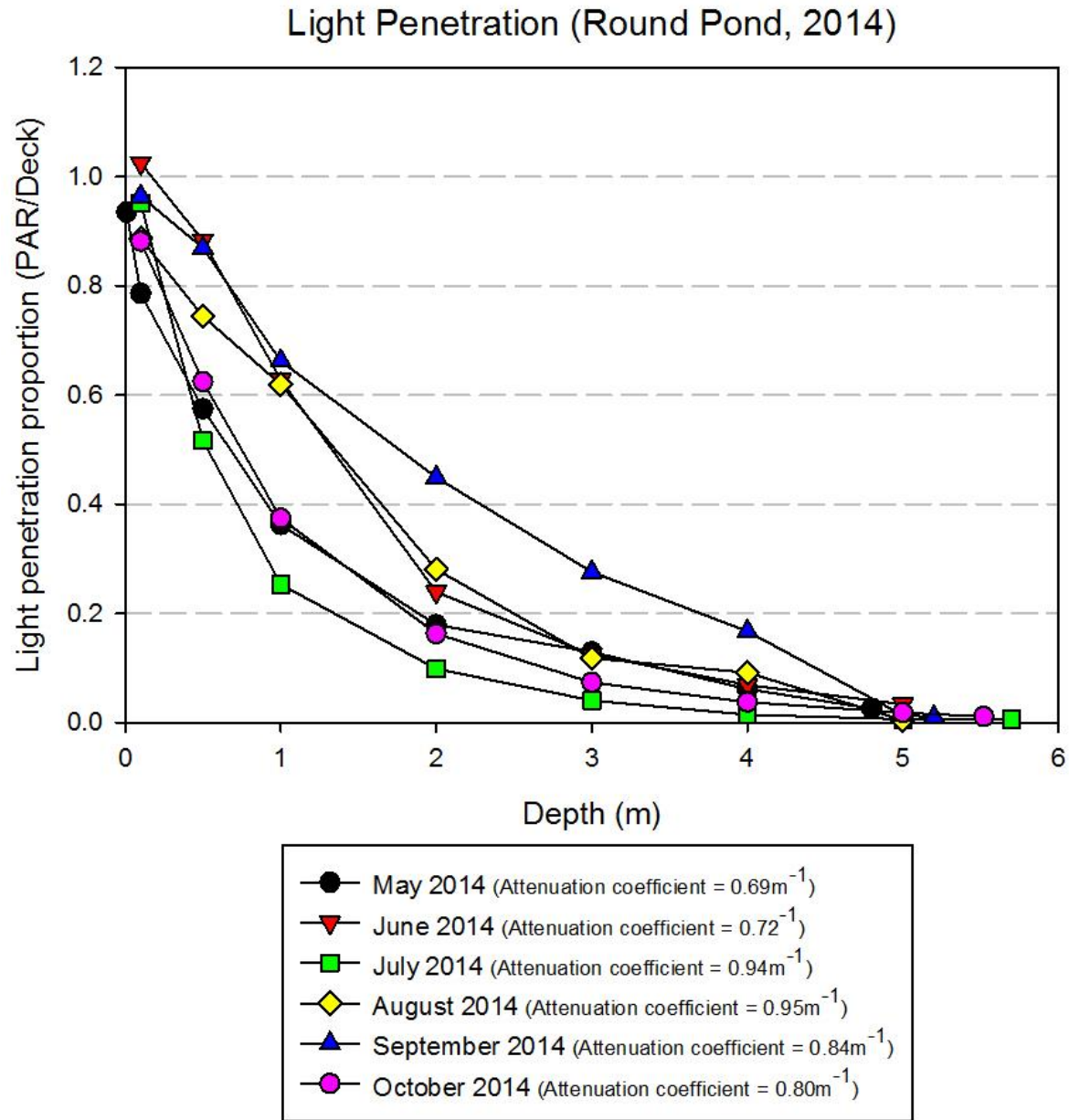
Figure 10. Light penetration profiles from Round Pond
