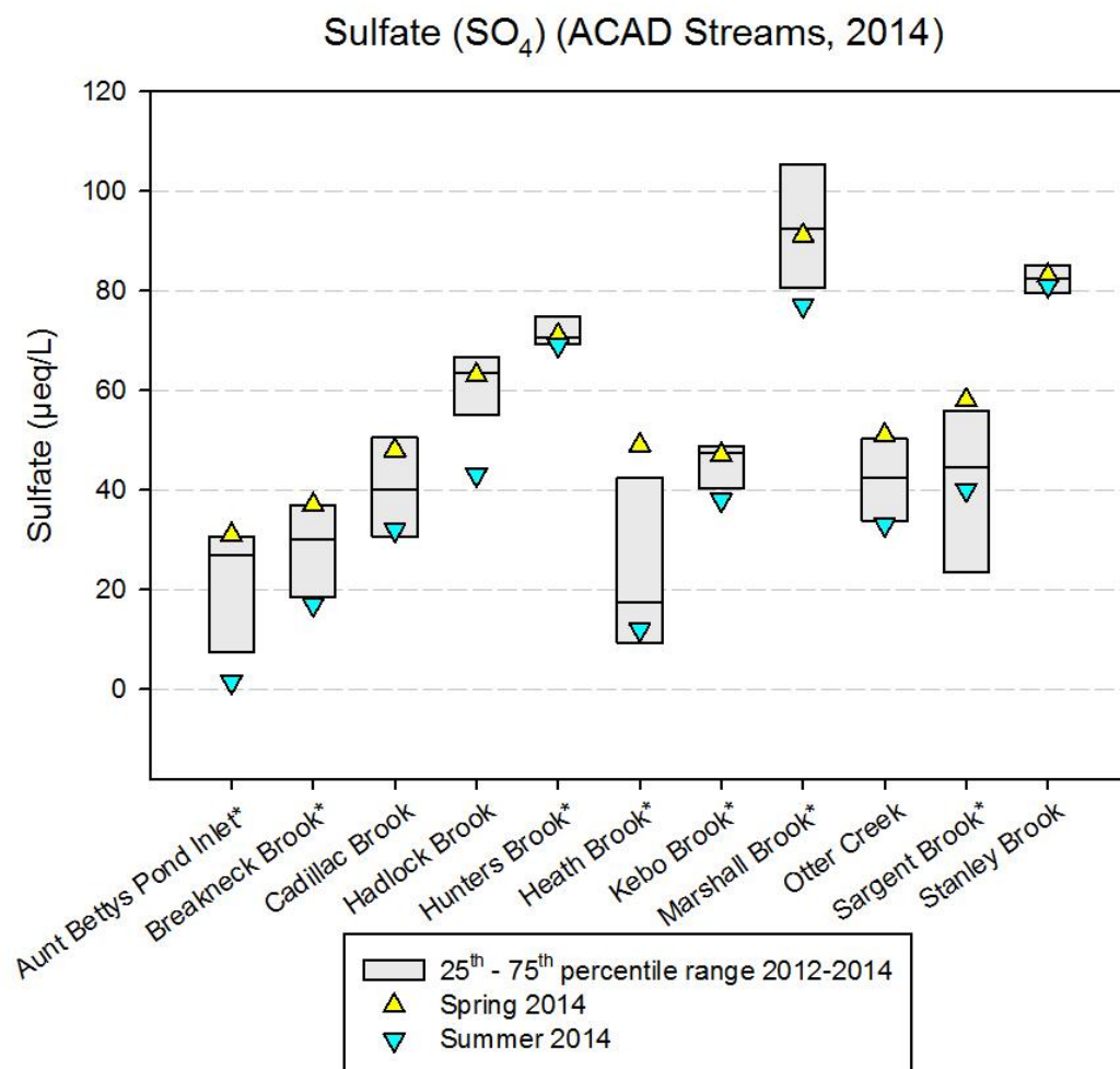
Figure 31. Stream sulfate from 2014 spring and summer water samples. The data are overlaid on a box plot of measurements taken from 2012-2014. Sites marked with an asterisk (*) are rotating sites with data from 2012 and 2014 only.
