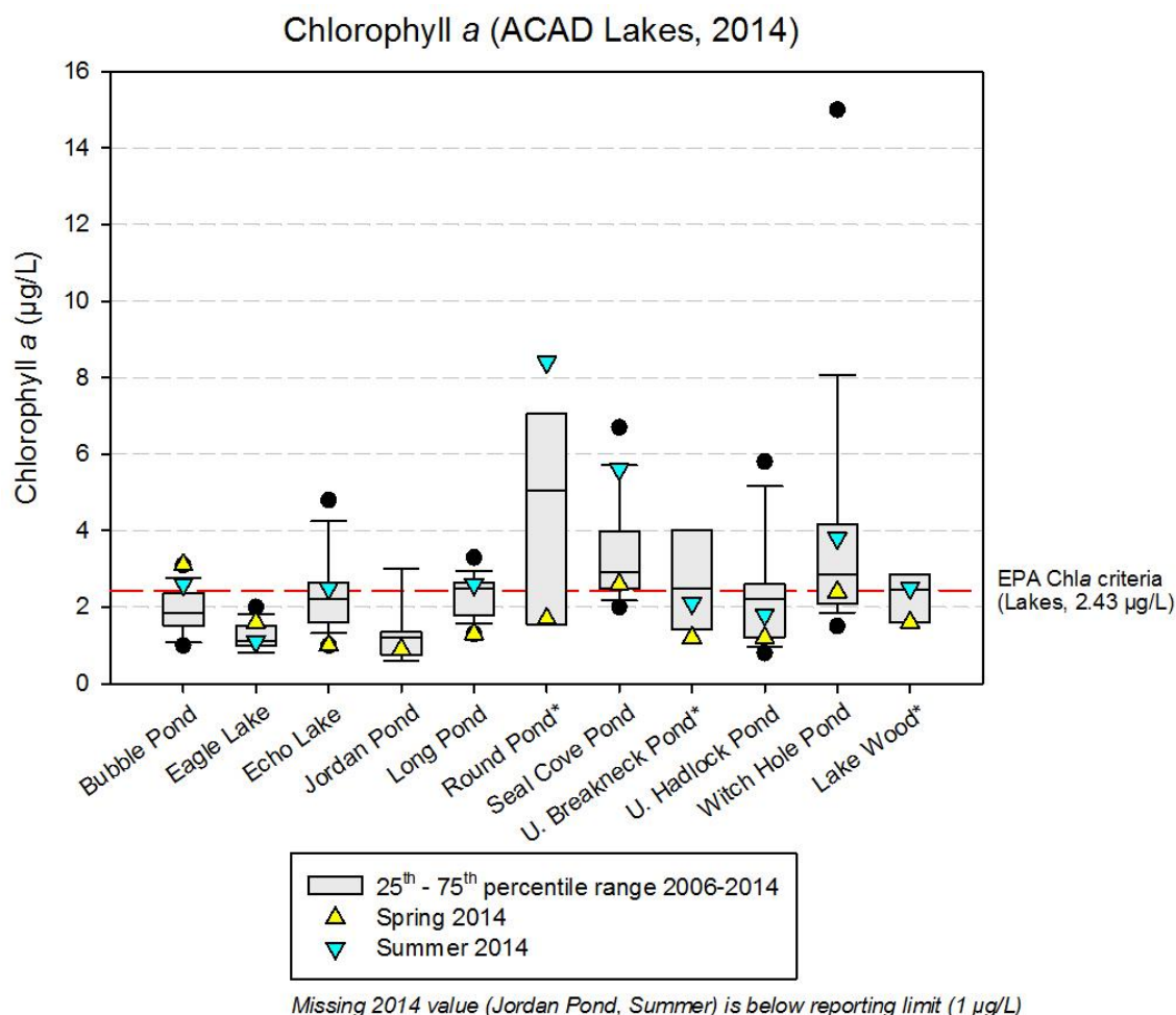
Figure 27. Lake and pond chlorophyll a from 2014 spring and summer water samples. The data are overlaid on a box plot of measurements taken from 2006-2014. Sites marked with an asterisk (*) are rotating sites with data from 2008, 2011, and 2014 only.
