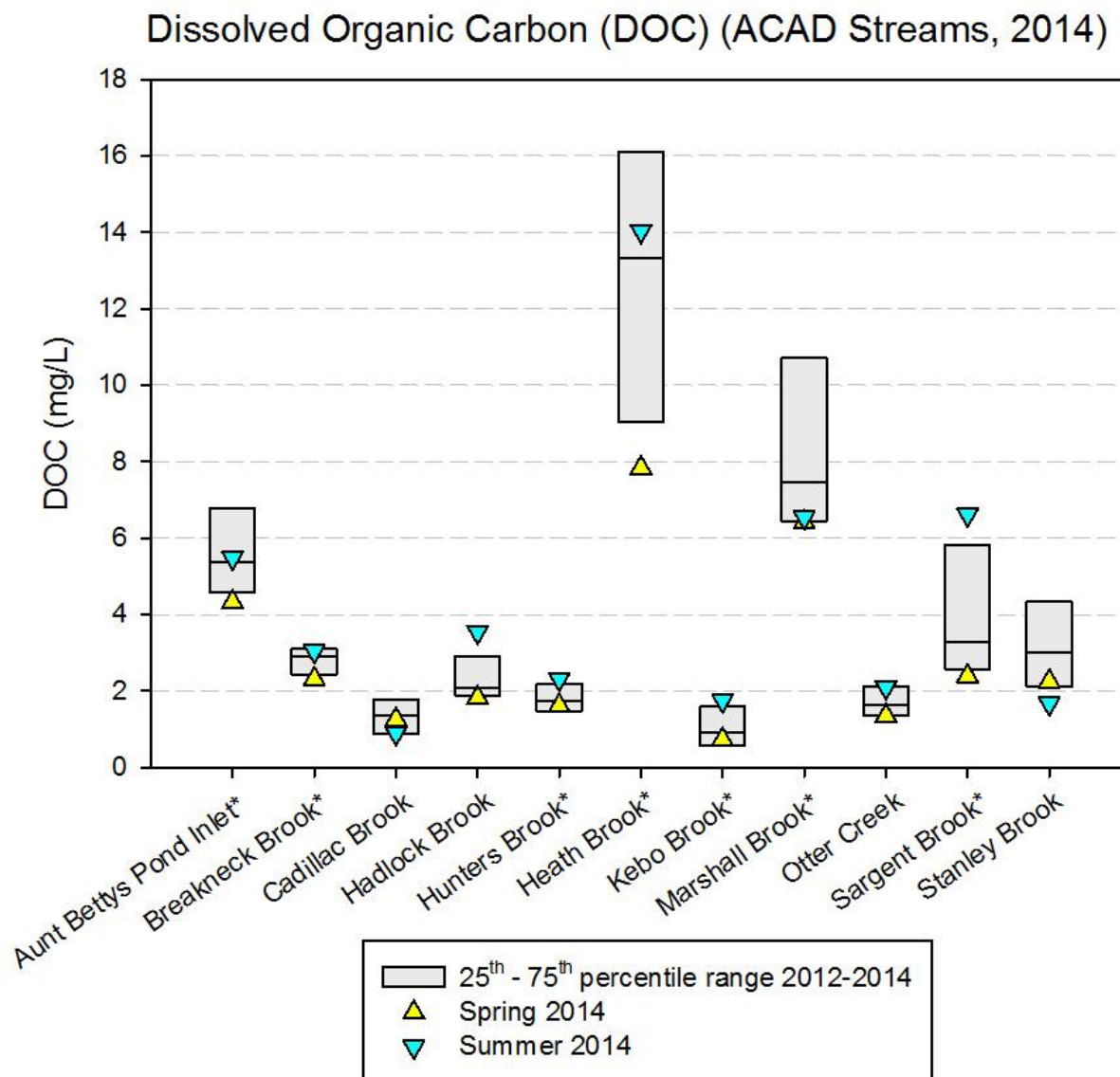
Figure 16. Stream dissolved organic carbon (DOC) from 2014 spring and summer water samples overlaid on a box plot of measurements taken from 2012-2014. Sites marked with an asterisk (*) are rotating sites with data from 2012 and 2014 only.
