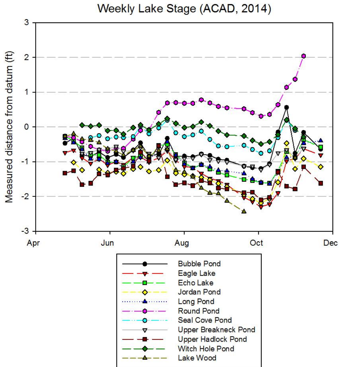
Figure 35. Weekly lake stage measured in 2014 at NETN monitoring sites in Acadia NP.
