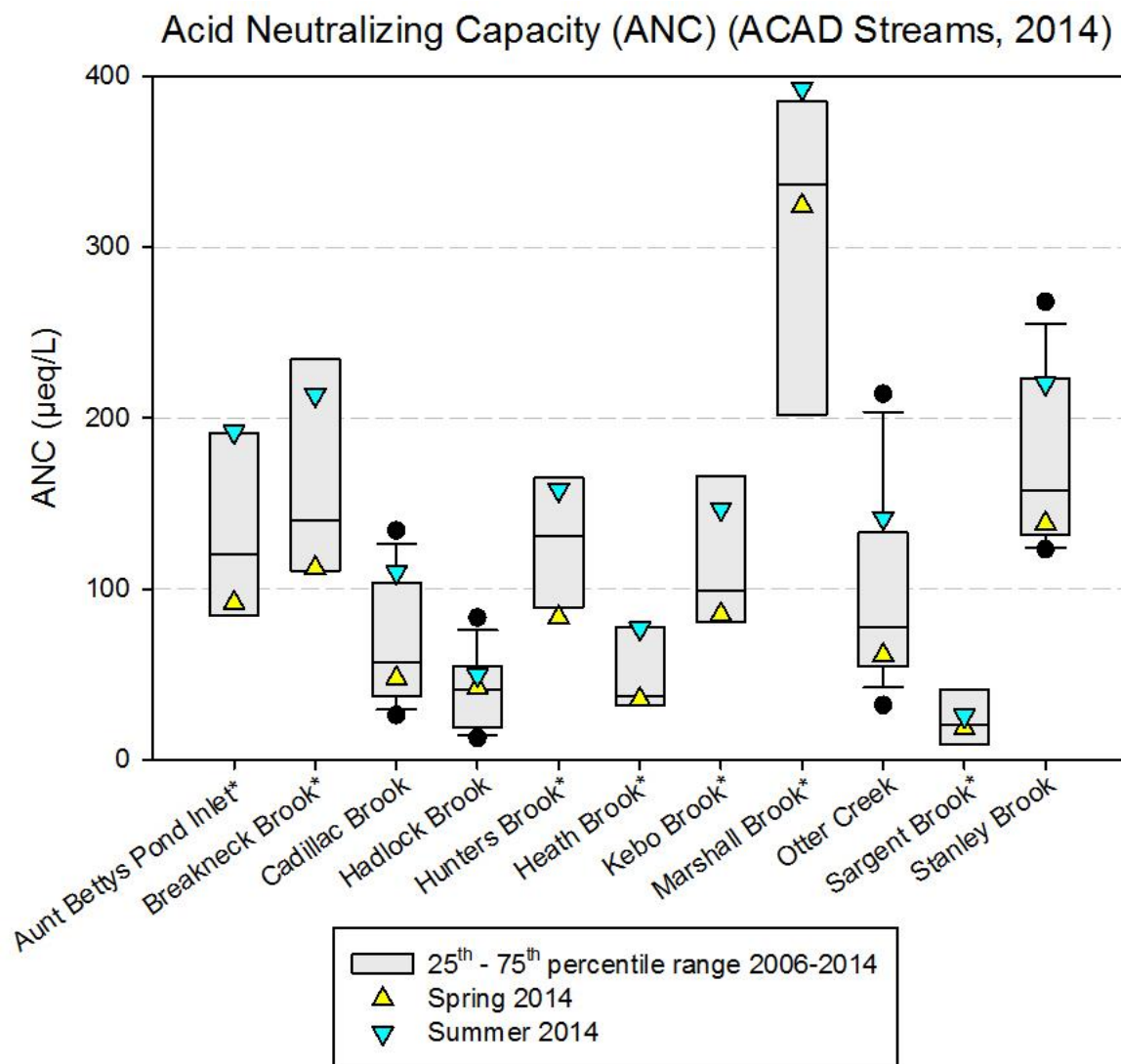
Figure 12. Stream acid neutralizing capacity from 2014 spring and summer water samples overlaid on a box plot of measurements taken from 2006-2014. Sites marked with an asterisk (*) are rotating partial-record sites with data from 2006, 2008, 2010, 2012, and 2014 only.
