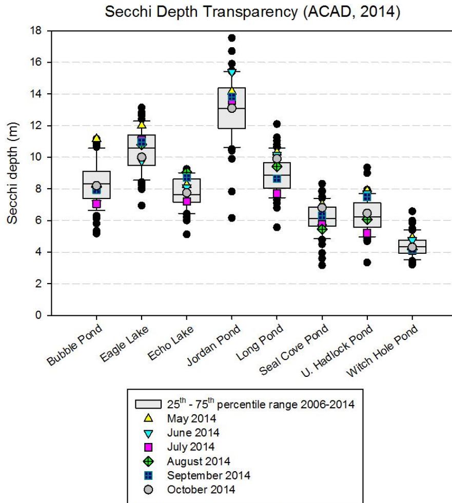
Figure 17. Secchi disk transparency from 2014 monthly measurements overlaid on a box plot of measurements taken from 2006-2014. Sites marked with an asterisk (*) are rotating sites with data from 2008, 2011, and 2014 only.
