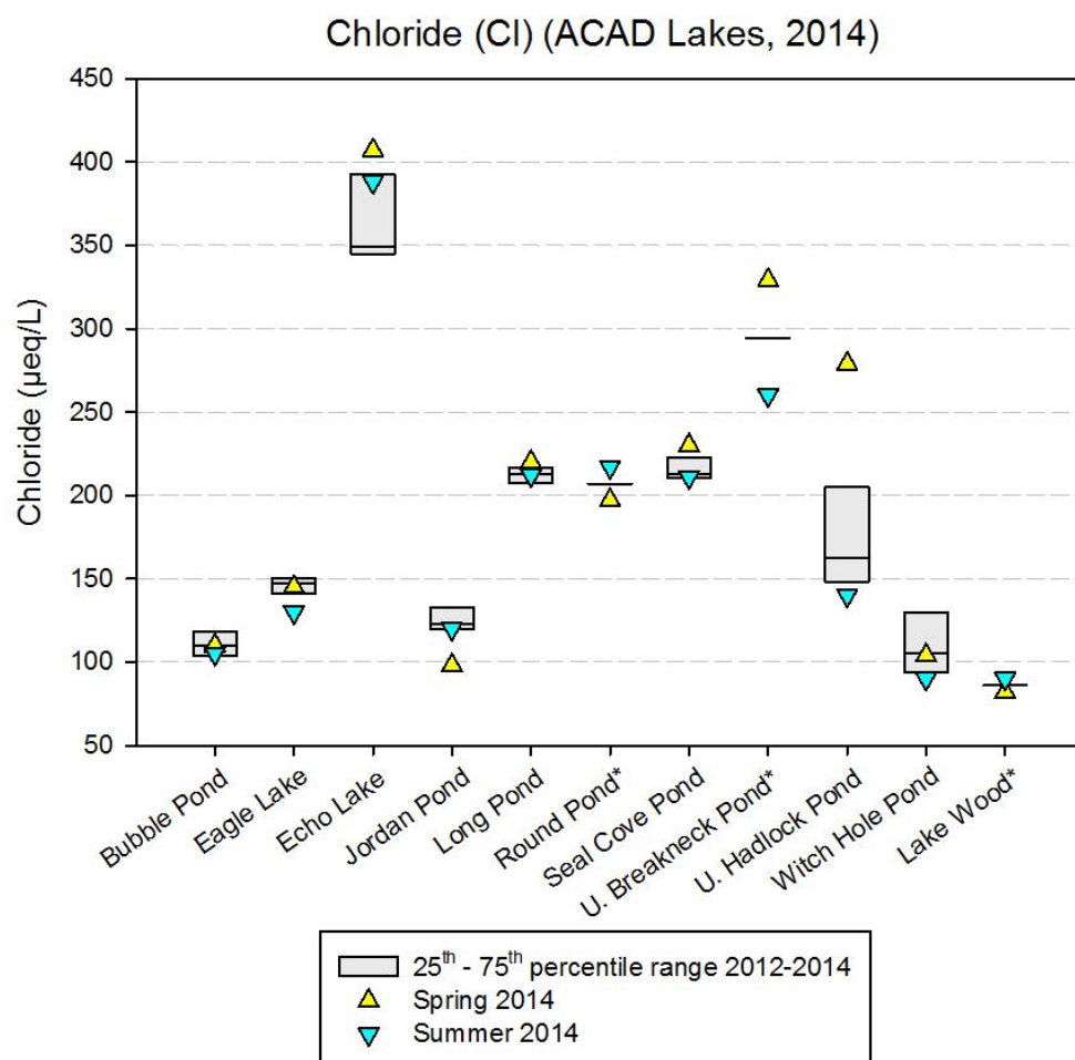
Figure 28. Lake and pond chloride from 2014 spring and summer water samples. The data are overlaid on a box plot of measurements taken from 2012-2014. Sites marked with an asterisk (*) are rotating sites with data from 2014 only.
