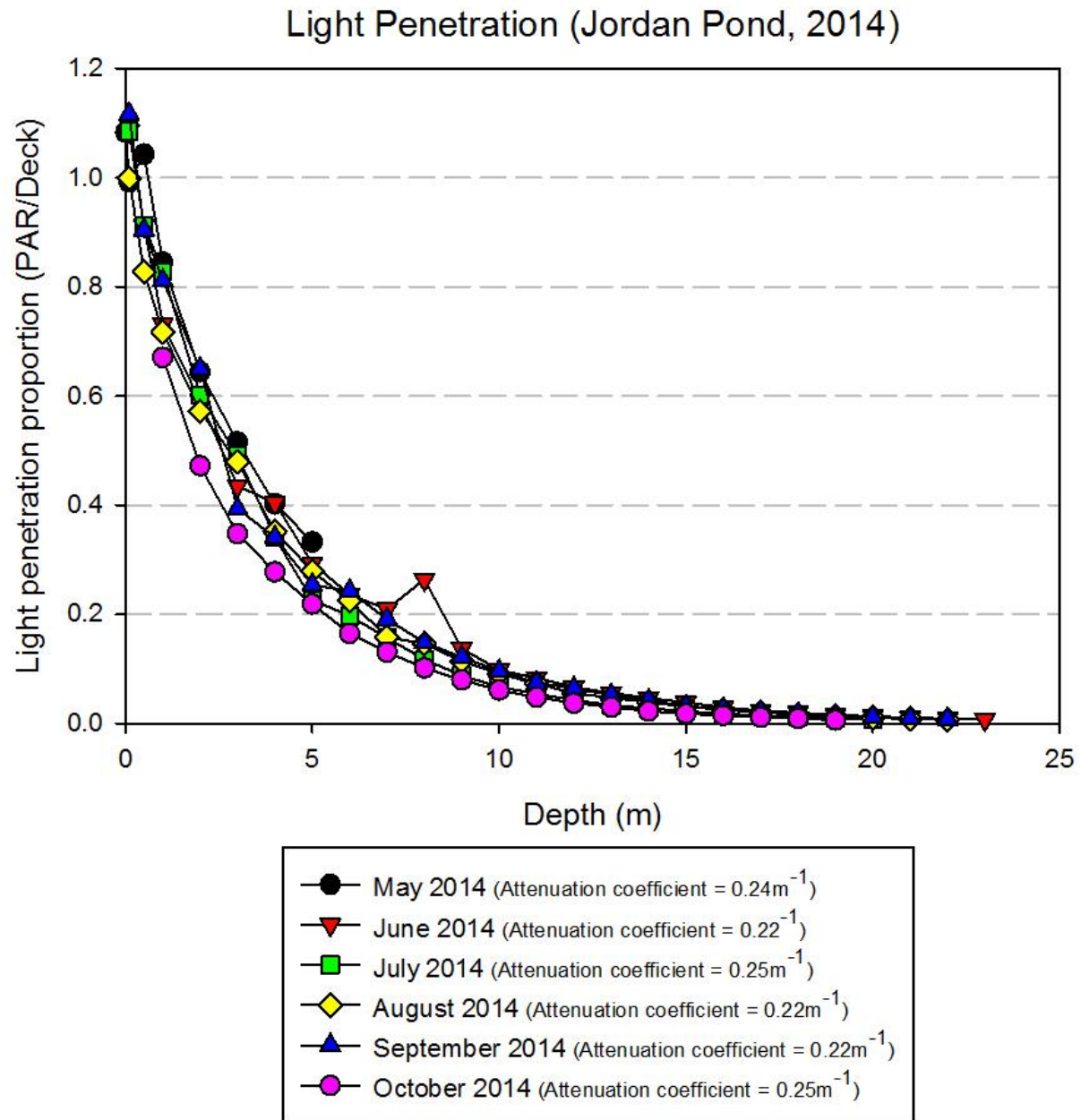
Figure 18. Light penetration profiles from Jordan Pond.
