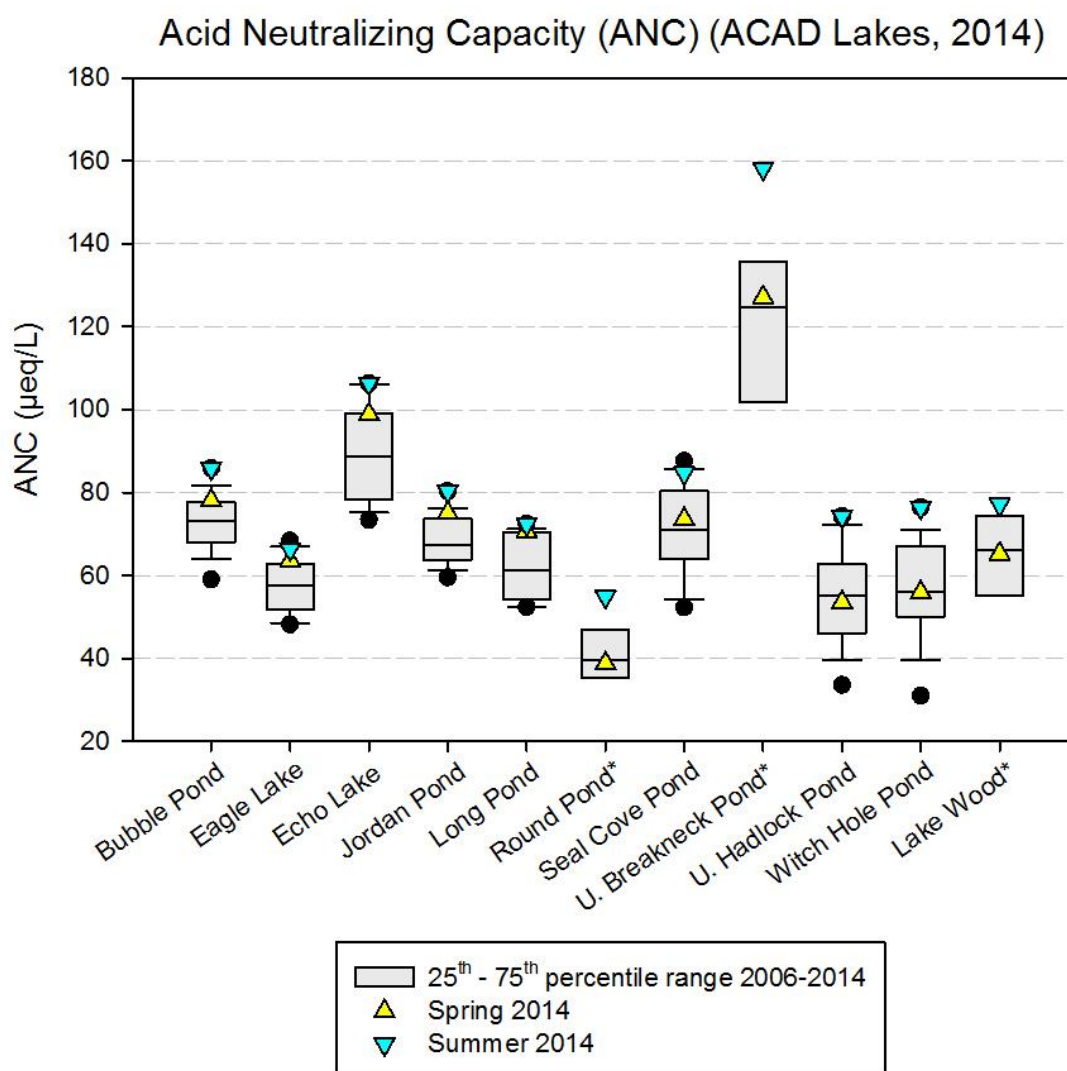
Figure 11. Lake and pond acid neutralizing capacity from 2014 spring and summer water samples overlaid on a box plot of measurements taken from 2006-2014. Sites marked with an asterisk (*) are rotating sites with data from 2008, 2011, and 2014 only.
