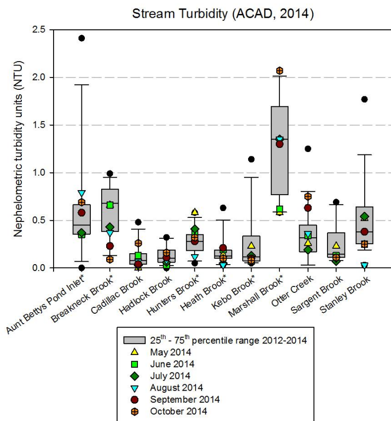
Figure 22. Stream turbidity from 2014 monthly measurements overlaid on a box plot of measurements taken from 2012-2014. Sites marked with an asterisk (*) are rotating sites with data from 2012 and 2014 only.
