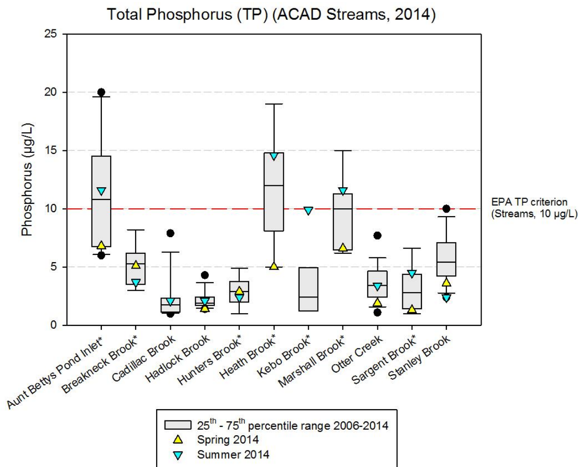
Figure 24. Stream total phosphorus (TP) from 2014 spring and summer water samples. The data are overlaid on a box plot of measurements taken from 2006-2014. Sites marked with an asterisk (*) are rotating partial-record sites with data from 2006, 2008, 2010, 2012, and 2014 only. There is no numeric Maine state water quality TP standard.
