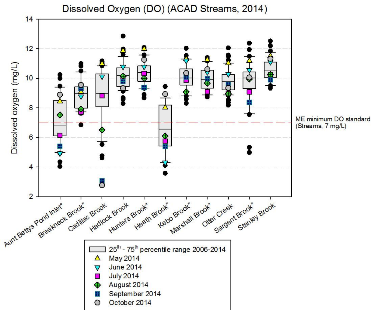
Figure 10. Stream dissolved oxygen (surface) from 2014 YSI sonde in-situ measurements overlaid on a box plot of measurements taken from 2006-2014. Sites marked with an asterisk (*) are rotating partial-record sites with data from 2006, 2008, 2010, 2012, and 2014 only.
