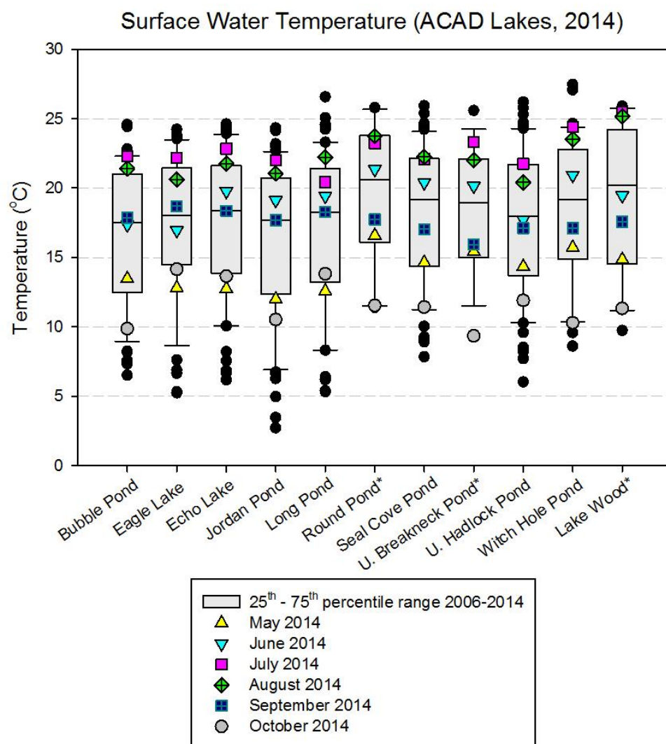
Figure 7. Lake and pond water temperature (surface) from 2014 YSI sonde in-situ measurements overlaid on a box plot of measurements taken from 2006-2014. Sites marked with an asterisk (*) are rotating sites with data from 2008, 2011, and 2014 only.
