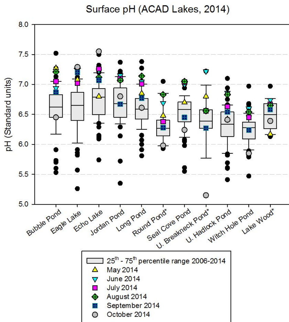
Figure 5. Lake and pond pH from 2014 YSI sonde in-situ measurements overlaid on a box plot of measurements taken from 2006-2014. Sites marked with an asterisk (*) are rotating sites with data from 2008, 2011, and 2014 only.
