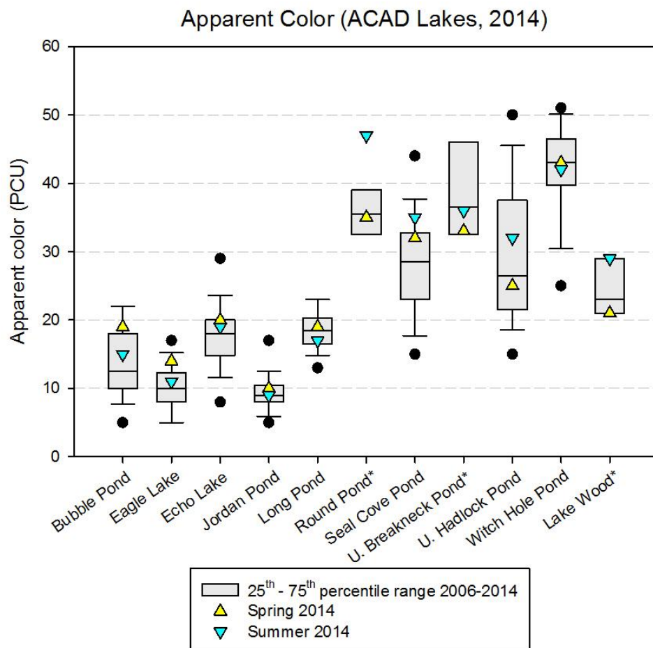
Figure 13. Lake and pond apparent color from 2014 spring and summer water samples overlaid on a box plot of measurements taken from 2006-2014. Sites marked with an asterisk (*) are rotating sites with data from 2008, 2011, and 2014 only.
