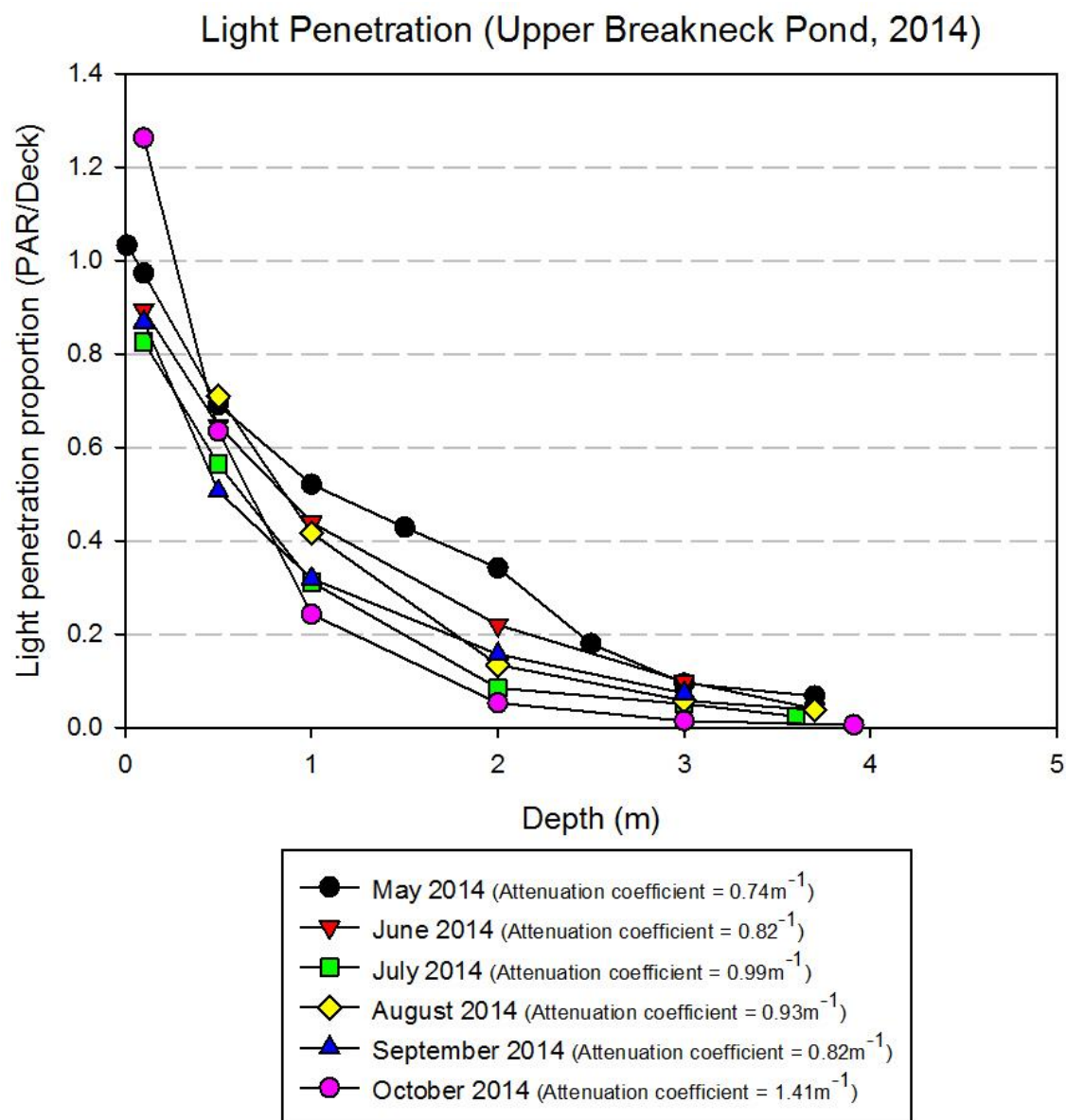
Figure 21. Light penetration profiles from Upper Breakneck Pond
