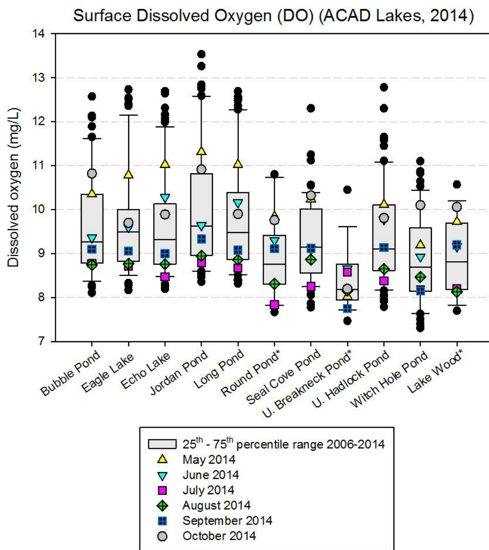
Figure 9. Lake and pond dissolved oxygen (surface) from 2014 YSI sonde in-situ measurements overlaid on a box plot of measurements taken from 2006-2014. Sites marked with an asterisk (*) are rotating sites with data from 2008, 2011, and 2014 only.
