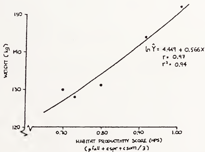
Figure 2. Annual variation in adult female weight relative to averaged habitat productivity scores of the previous autumn and the following spring and summer.
