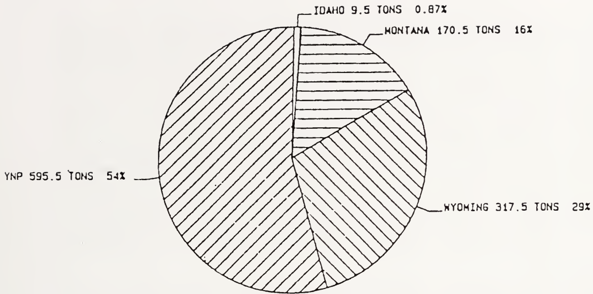
Figure 17. Distribution of winter kill carrion by area in the Yellowstone ecosystem.
