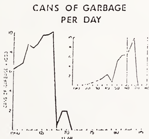
Figure 12. Garbage availability in Yellowstone National Park open-pit dumps. Inset shows garbage availability since 1910.
