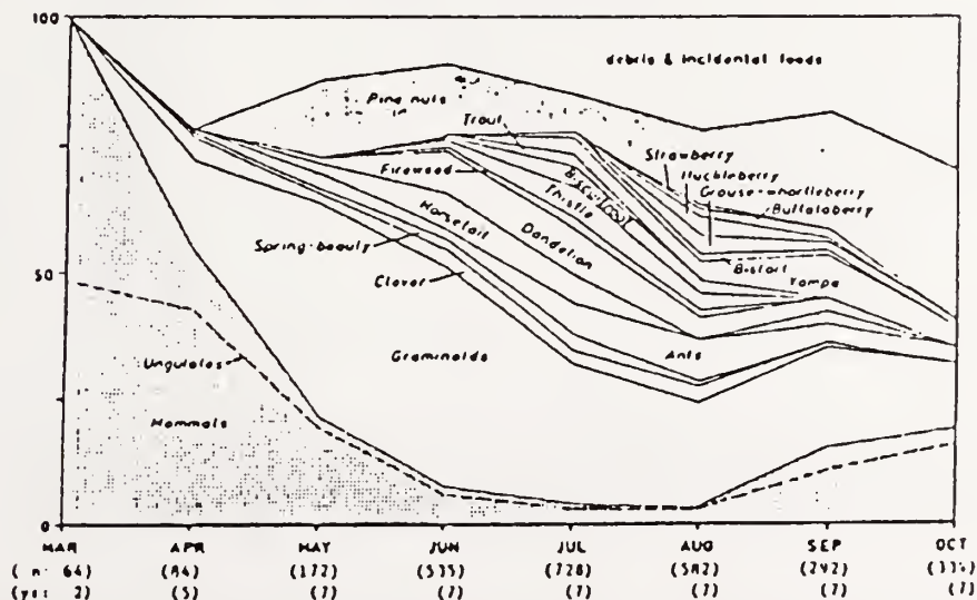
Figure 6. Overall food habits by season for Yellowstone ecosystem grizzly bears. N = number of scats/month in collection. Yr = number of years of collection.
