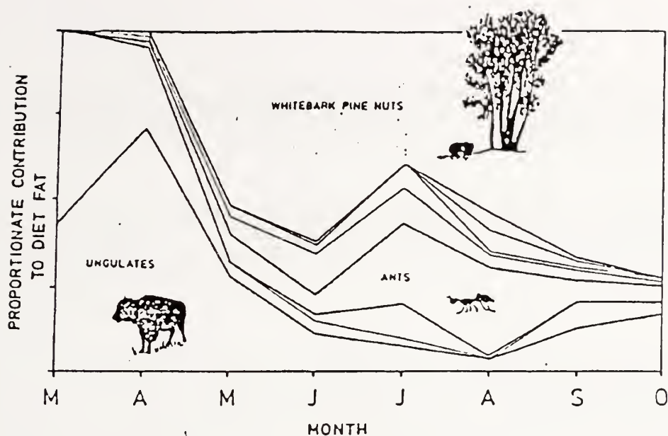
Figure 10. Proportionate seasonal contribution of major food items to diet fat for Yellowstone ecosystem grizzly bears.
