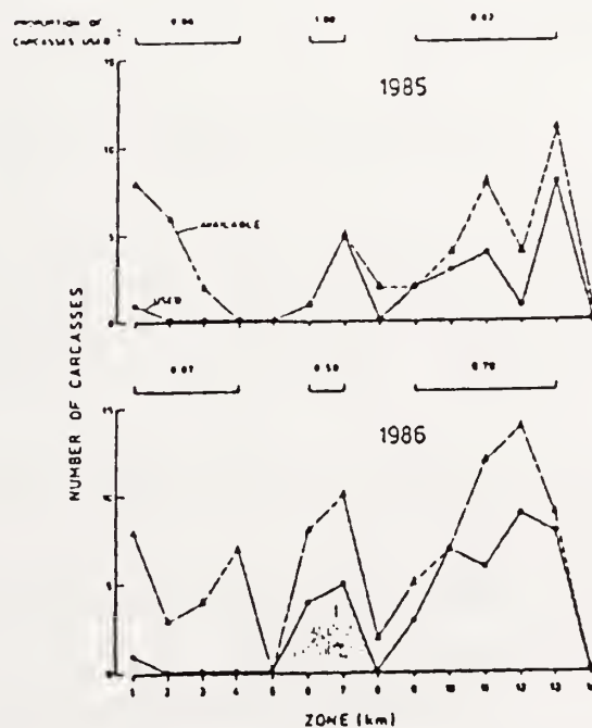
Figure 18. Number of carcasses used as a proportion of the number available by distance from the Old Faithful developed area from March to May 1985-86.
