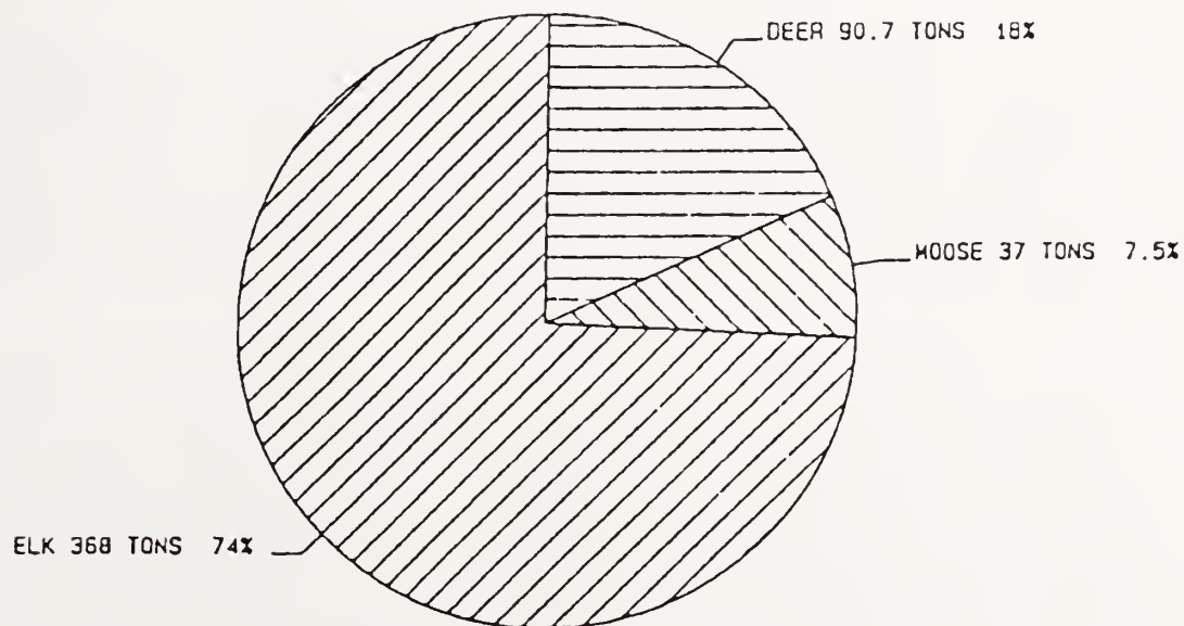
Figure 19. Total sport hunt related carrion available in autumn in the Yellowstone ecosystem.
