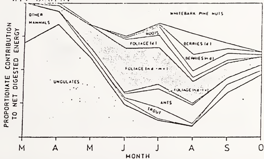
Figure 8. Proportionate contribution to net digested energy of major food items by season for Yellowstone ecosystem grizzly bears.
