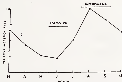
Figure 5. Relative ingestion rate from den emergence to den entry showing period of hyperphagia.
