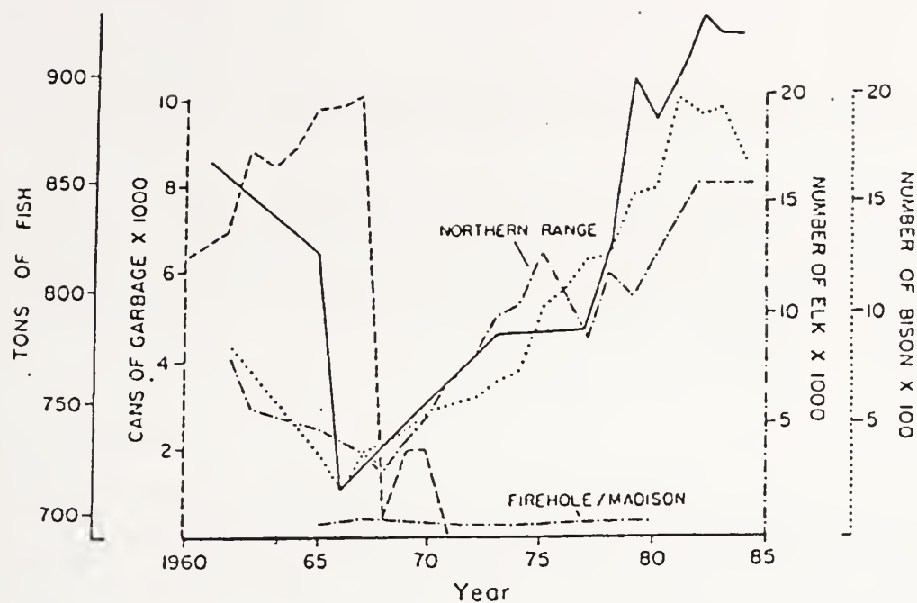
Figure 21. The relationship between elk, bison and cutthroat trout populations and garbage in Yellowstone National Park, 1960-1985.
