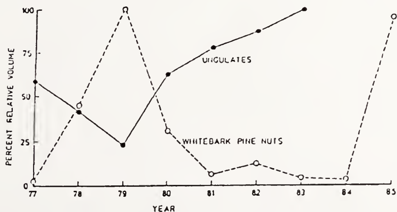
Figure 11. Use of white bark pine nuts and ungulates as both carrion and as a result of predation for Yellowstone ecosystem grizzly bears.
