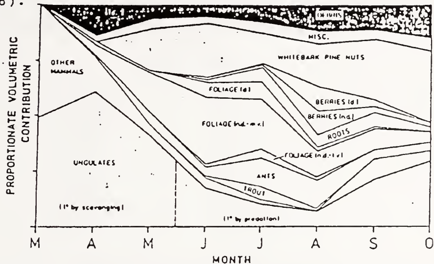
Figure 7. Proportionate volumetric contribution of food items by season for Yellowstone ecosystem grizzly bears.
