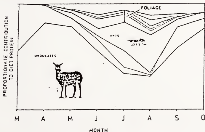
Figure 9. Proportionate seasonal contribution to diet protein of major food items for Yellowstone ecosystem grizzly bears.
