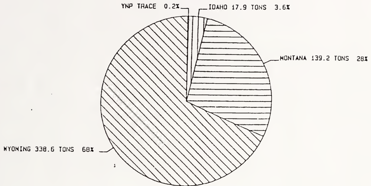
Figure 20. Distribution of sport hunt related carrion available in the autumn in the Yellowstone ecosystem.
