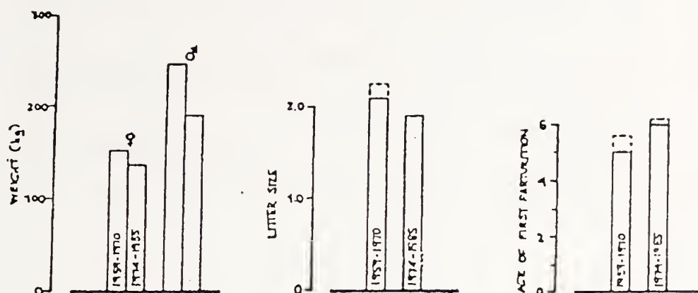
Figure 1. Comparison of body weight, mean litter size, and mean age at first reproduction between the 1959-70 period when the garbage dumps were open and the 1974-85 period when garbage was not available to bears.
