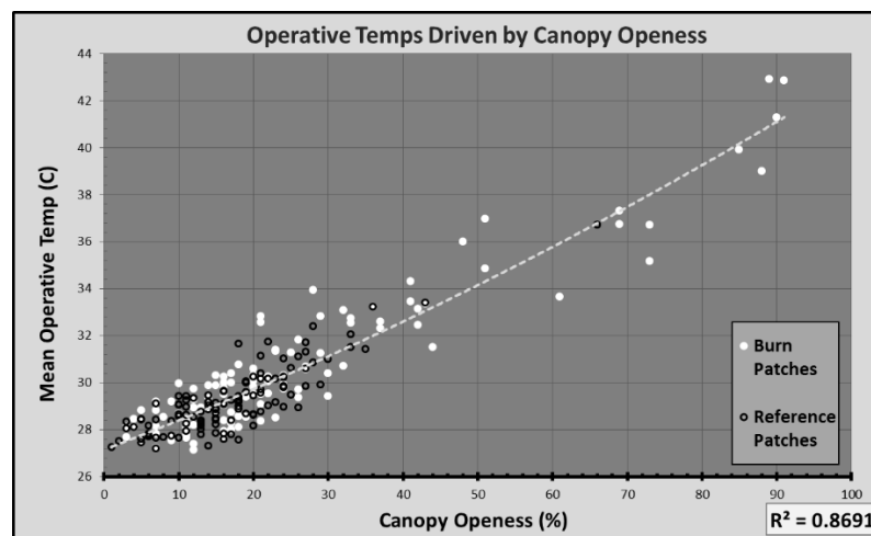
Figure 3.11: Operative temp mean, variability, and canopy openness. Study duration means are used for the top and bottom graphs, as canopy coverage was not recorded daily. The middle graph incorporates daily values for each station.
