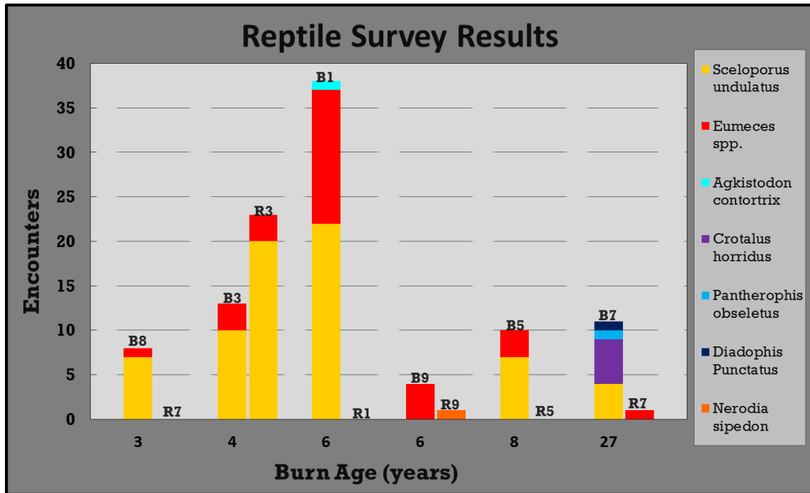
Figure 3.6: Reptile survey results. All species encountered during surveys are included. Burn/reference pairs are grouped and arranged along the x-axis by burn age. Site labels at the top of each bar correspond to maps presented in Figures 2.5 and 2.6.
