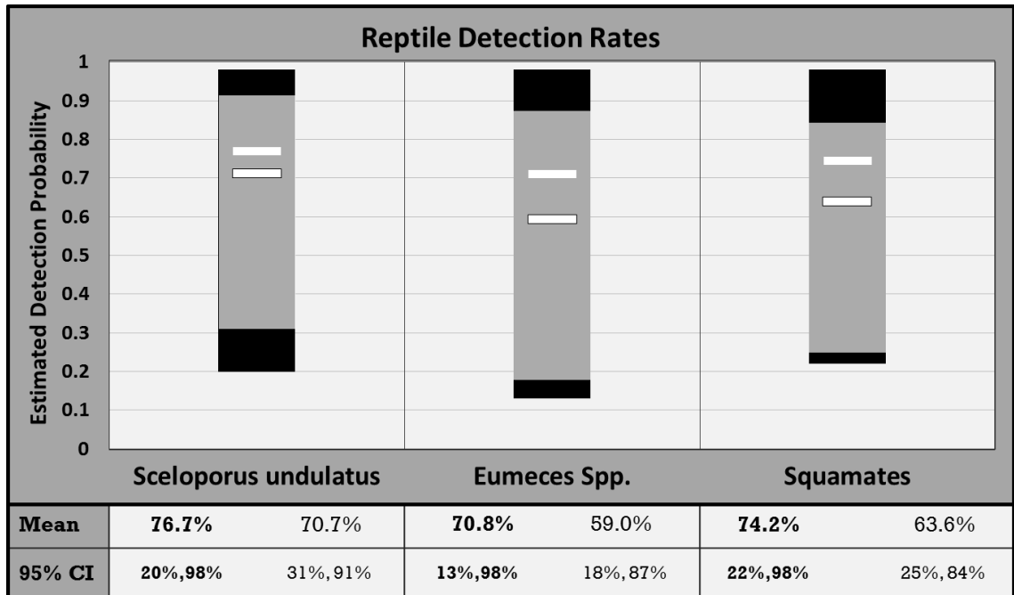
Figure 3.10: Reptile detection rates. In the upper graph, white bars represent median values for reptile detection rates; the marker with no outline represents median detection in sunny to partly sunny conditions, while the outlined marker represents median detection in overcast weather. Similarly, the black box indicates the 95% credibility interval for detection in sunny conditions and the grey box credibility intervals for overcast conditions. In the table below, values in bold (left) correspond to sunny conditions and values in regular width font (right) correspond with overcast conditions.
