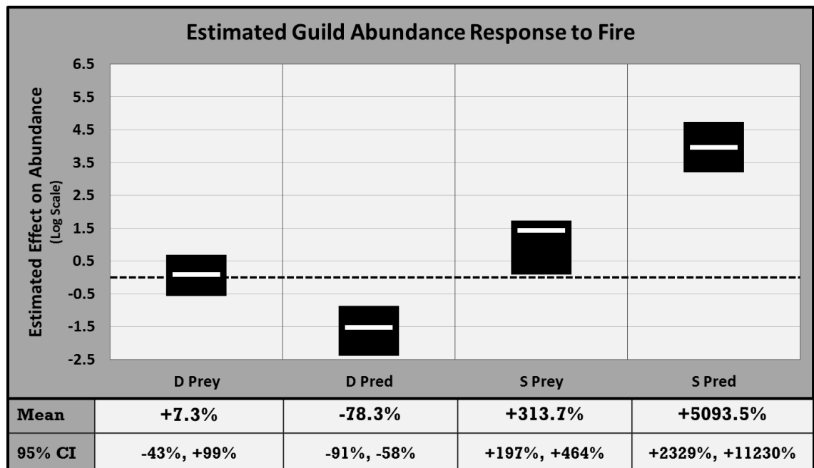
Figure 3.3: Fire's effect on salamander abundance. In the upper graph, white bars represent untransformed median values for the burn effect parameter and black boxes the extent of 95% credibility intervals. Values provided below are transformed rates of change; thus, +7% indicates abundance on burns is estimated to be 107% that of reference sites. 95% credibility intervals are also given as transformed rates of change. Intervals including zero indicate fire may have no effect on abundance of that taxon.
