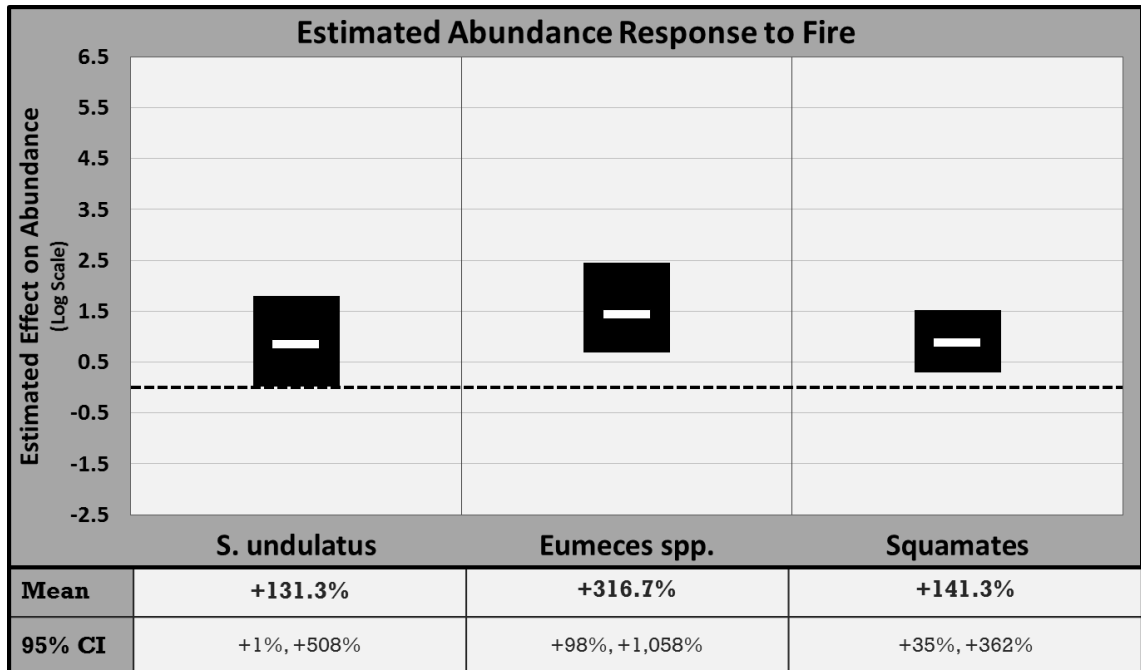
Figure 3.8: Fire's effect on reptile abundance. In the upper graph, white bars represent untransformed median values for the burn effect parameter and black boxes the extent of 95% credibility intervals. Values provided below are transformed rates of change; thus, +131% indicates abundance on burns is estimated to be 231% that of reference sites. 95% credibility intervals are also given as transformed rates of change. Intervals including zero indicate fire may have no effect on abundance of that taxon.
