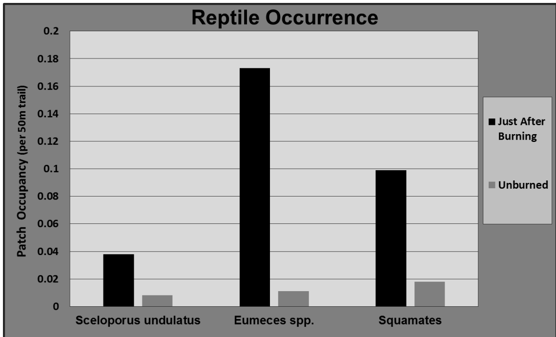
Figure 3.5: Reptile occupancy following fire. Estimated patch occupancy per 50m of GSMNP trail is shown. All reptiles are estimated to occur more frequently in burned areas. The relationship between occupancy and time since burning was not well determined for S. undulatus or squamates as a whole. See Figure 3.7 for the estimated relationship between Eumeces Spp. occupancy and burn age.
