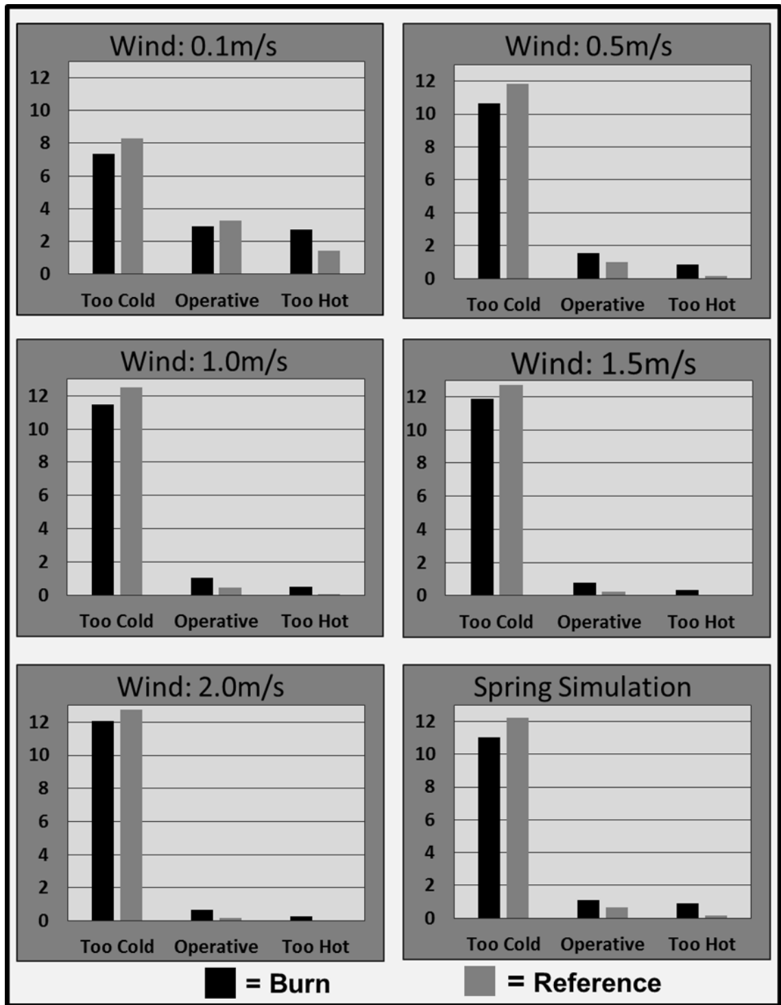
Figure 3.12: Influence of wind and season on daily activity. The distribution of daily activity on burn and reference sites is shown for various relevant wind velocities. To represent the month of May, distribution of daily activity is also given when 5°C is subtracted from each air and surface temperature measurement taken in the study.
