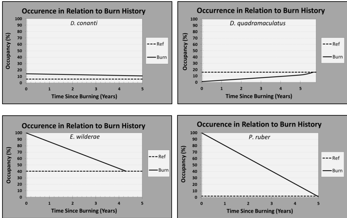
Figure 3.1: Salamander occurrence in relation to burn history. Estimated occupancy per trap is shown in relation to years since experiencing an episode of fire. Our models suggest D. conanti occurrence is unrelated to fire. Thus, the relationship between time since burning and D. conanti occurrence was not well determined. The very steep P. ruber trend is likely resulting from the influence of Site B3, where 81 P. ruber were observed in just 90 traps.
