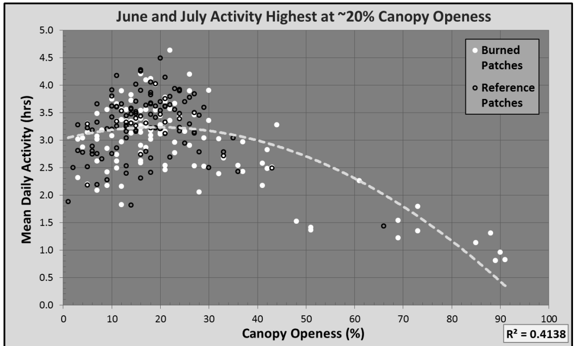
Figure 3.14: Canopy's influence on activity hours. Unlike many of the other canopy correlations examined, the relationship between canopy openness and activity period is curvilinear for the months of June and July.
