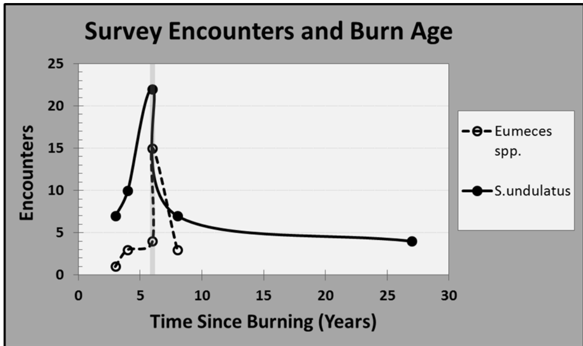
Figure 3.9: Lizard survey encounters and burn age. Although our model was unable to determine the relationship between burn age and lizard abundance, results of surveys suggest lizard abundance peaks at about six years (lightly pigmented vertical line) post fire.
