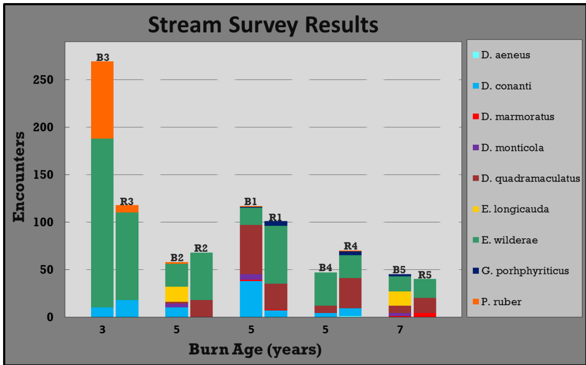
Figure 3.2: Salamander survey results. All species encountered during surveys are included. Burn/reference pairs are grouped and arranged along the x-axis by burn age. Site labels at the top of each bar correspond to maps presented in Figures 2.2 and 2.3.
