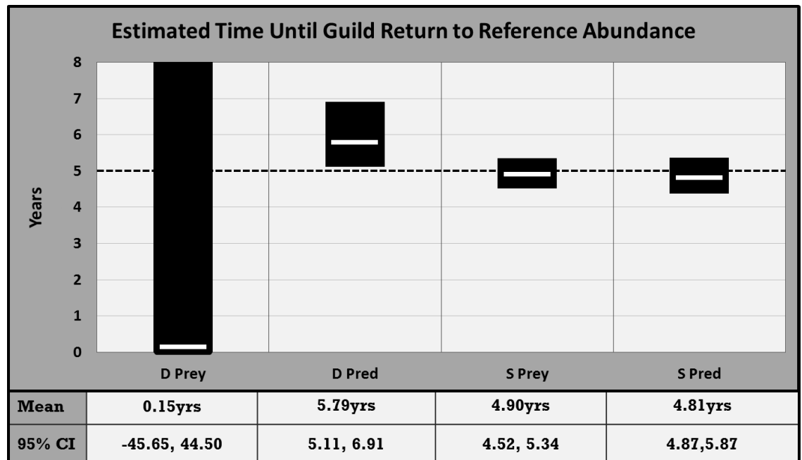
Figure 3.4: Time until salamander return to reference abundance. In the upper graph, white bars represent median values for the burn persistence parameter and black boxes the extent of 95% credibility intervals. Values provided below are in the same units, but reveal the extent of the credibility interval for D. conanti . Intervals including zero indicate fire may have no effect on abundance of that taxon.
