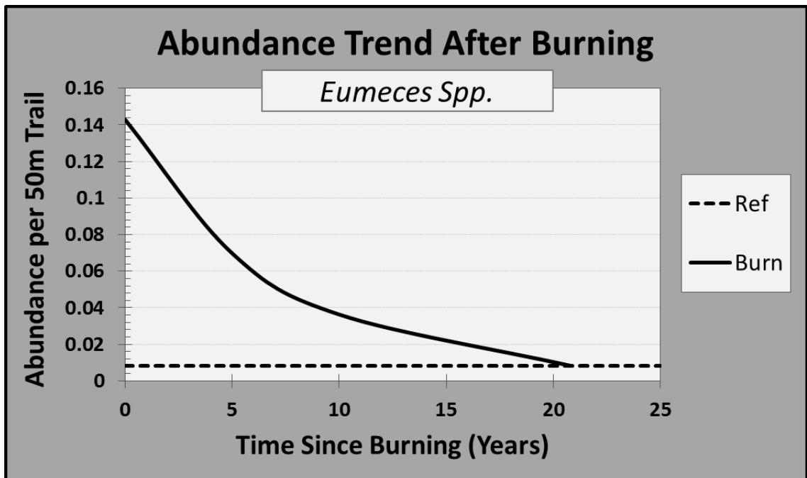
Figure 3.7: Eumeces occurrence and abundance related to burn age. It should be noted the slope value relating Eumeces spp. occurrence and abundance to burn age was not well determined by the model. Those parameter estimates were even less precise for S. undulatus , and as a result all squamates, thus graphs were not included for those taxa.
