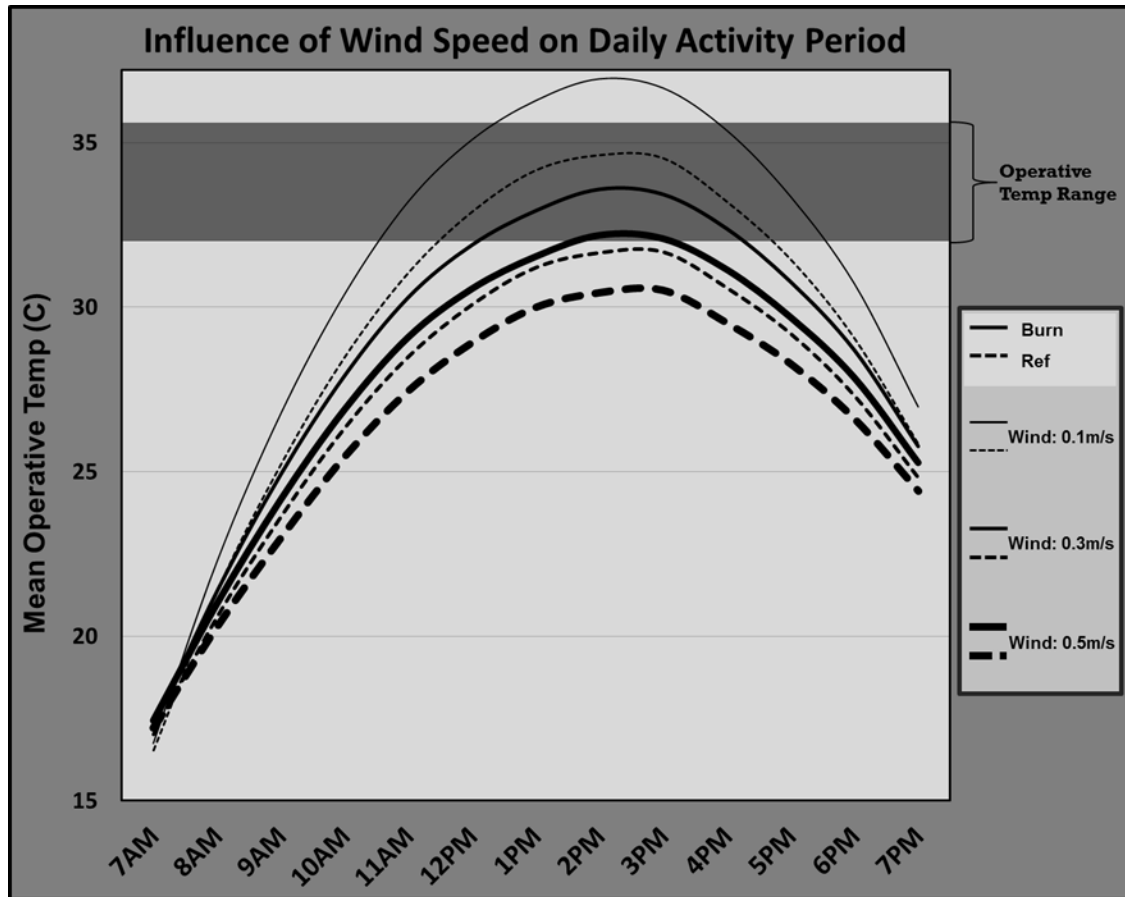
Figure 3.13: Diurnal operative temp trajectories at different wind speeds. Daily diurnal operative temperature trajectories are given for burn (solid line) and reference (dashed line) sites under various wind velocities. The thickness of trajectory lines increases with wind speed. S. undulatus operative range is represented by the dark grey band covering 32.0-35.6°C.
