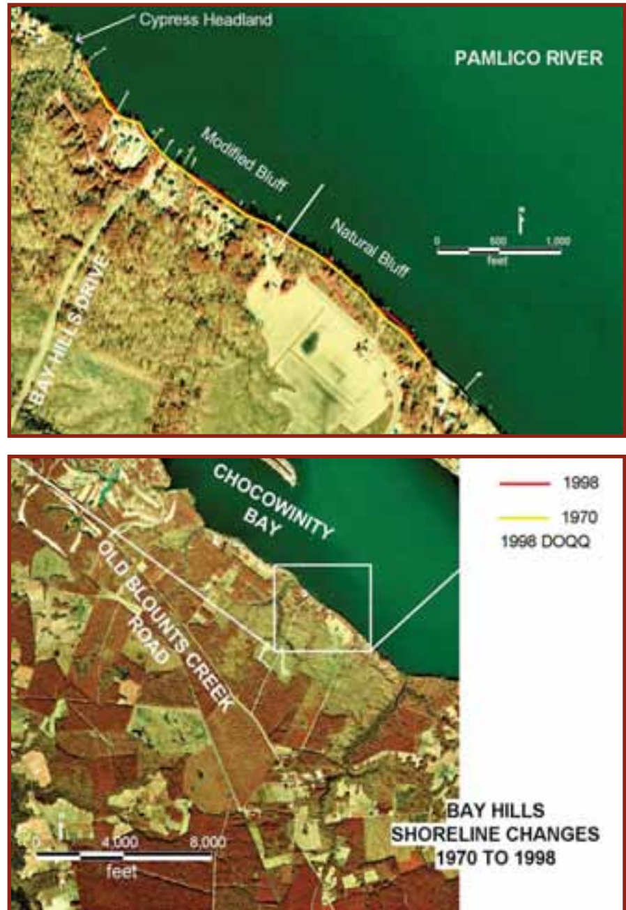
FIGURE 8-4-16. The Bay Hills site 1998 Digital Orthophoto Quarter Quadrangle (DOQQ) with digitized shorelines for 1970 and 1998.
