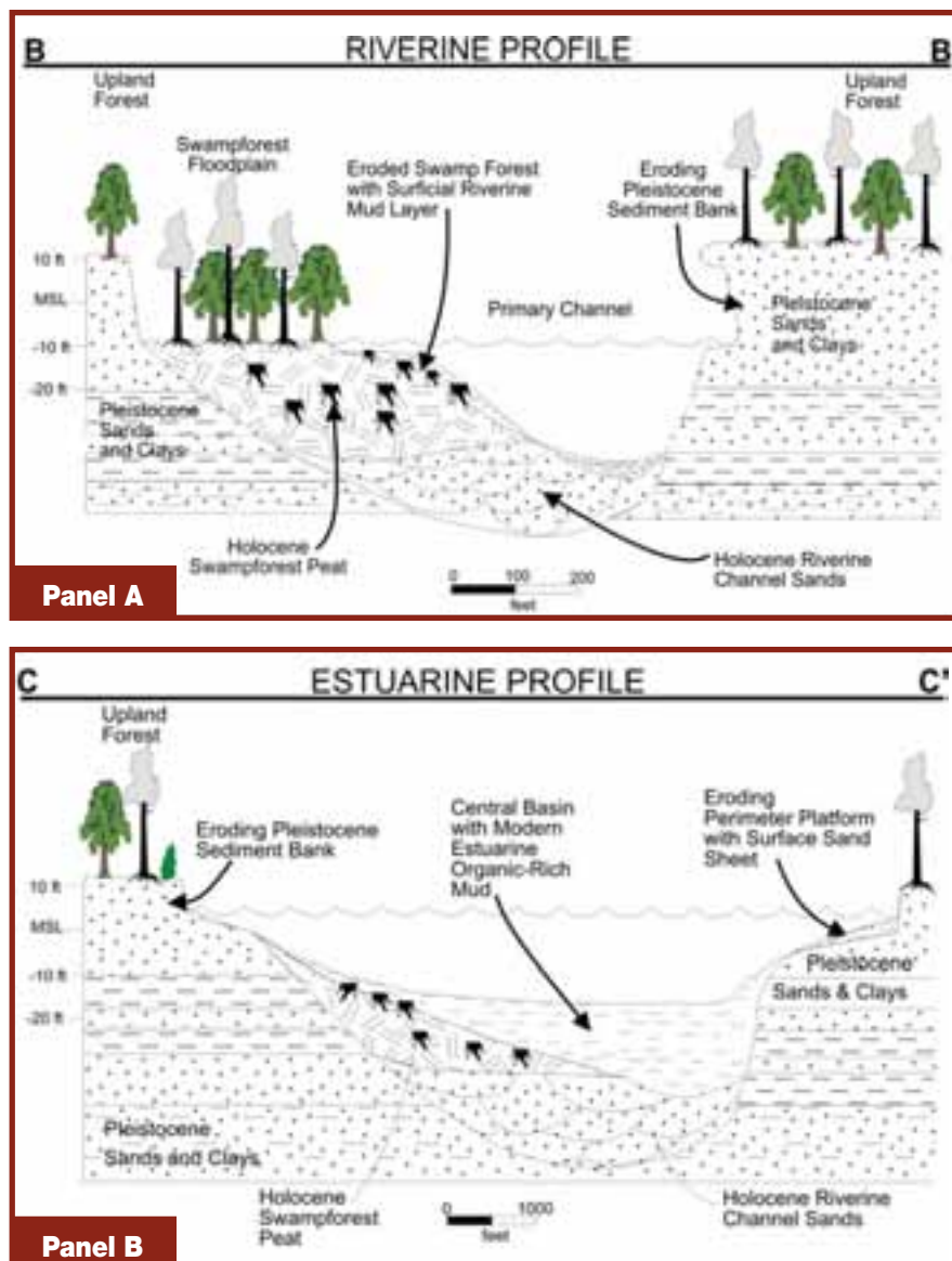
FIGURE 3-2-4. Schematic cross-sectional profiles of the transition zone from riverine to estuarine ecosystems within the drowned-river estuaries of North Carolina. See Figure 3-2-2 for location of profiles B-B' and C-C'. PANEL A. Schematic cross-sectional profile B-B' across the riverine portion of the drainage system. Notice the riverine channel is characterized by deposition of sand and gravel, while the associated floodplain is characterized by deposition of organic matter and riverine mud to form peat, muddy peat, and peaty mud sediment. PANEL B. Schematic cross-sectional profile C-C' across the upper estuarine portion of the drainage system. Notice how the swampforest floodplain peat deposit has been largely eroded away and only locally buried and preserved in the transition from a riverine to an estuarine system. A sediment inversion has taken place with the organic-rich mud being deposited within the central basin and sand deposition occurring on the shallow perimeter platform in response to shoreline erosion of the older sediment units.
