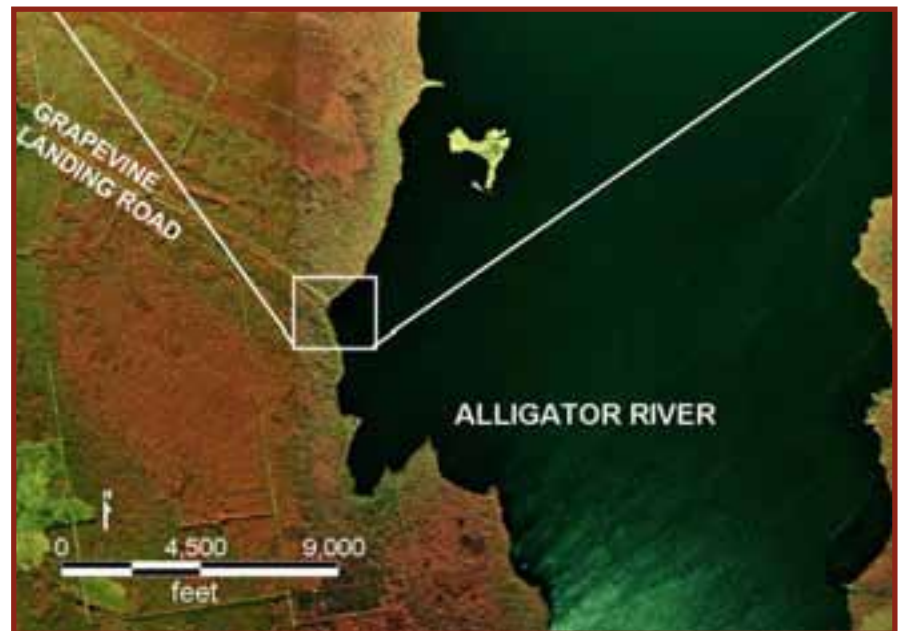
FIGURE 8-3-9. The Grapevine Landing site 1998 Digital Orthophoto Quarter Quadrangle (DOQQ) with digitized shorelines for 1981 and 1998.
