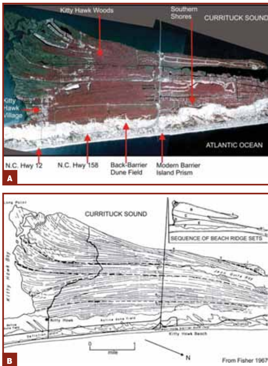
FIGURE 4-5-3. PANEL A. A 1983 infrared aerial photograph of the complex barrier island in the Kitty Hawk area of North Carolina. The photo shows the many beach ridges that constitute Kitty Hawk Woods fronted by a back-barrier dune field and the modern beach prism. Infrared aerial photograph was flown on 4/24/1982 by the High Altitude Program of the U.S. Department of Agriculture. PANEL B. Map shows the interpretation of individual beach ridges and sequence of the seven beach ridge sets for the Kitty Hawk Woods by Fisher (1967).
