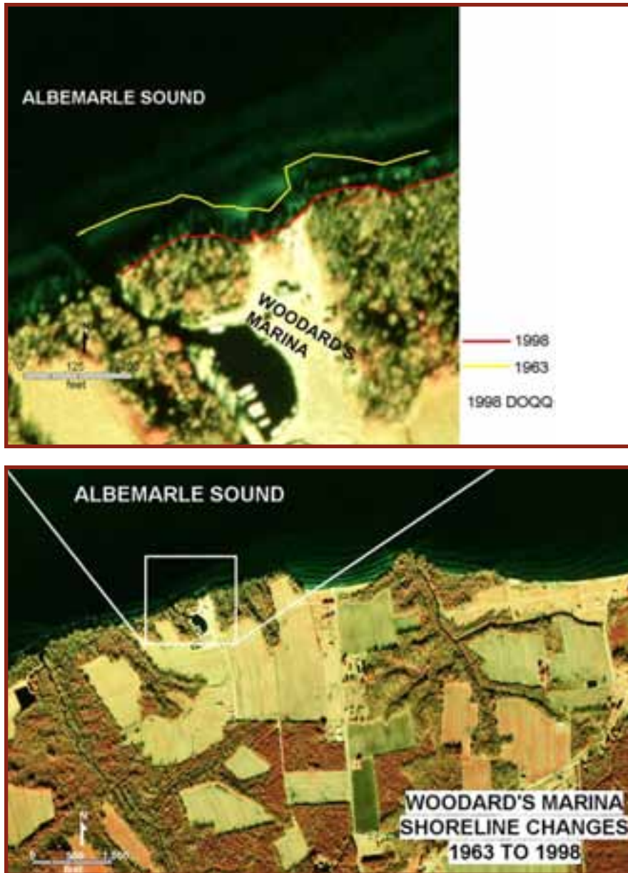
FIGURE 8-3-6. The Woodard's Marina site 1998 Digital Orthophoto Quarter Quadrangle (DOQQ) with digitized shorelines for 1963 and 1998.
