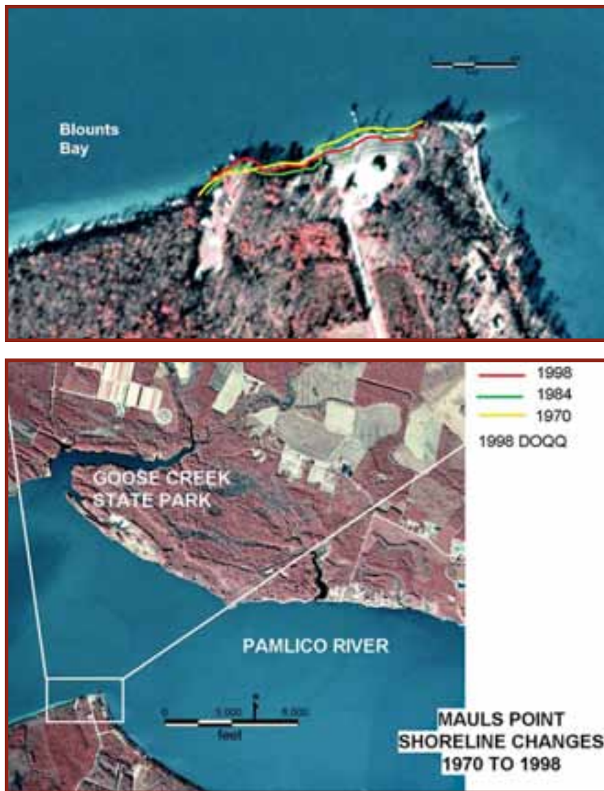
FIGURE 8-4-13. The Mauls Point site 1998 Digital Orthophoto Quarter Quadrangle (DOQQ) with digitized shorelines for 1970, 1984, and 1998.
