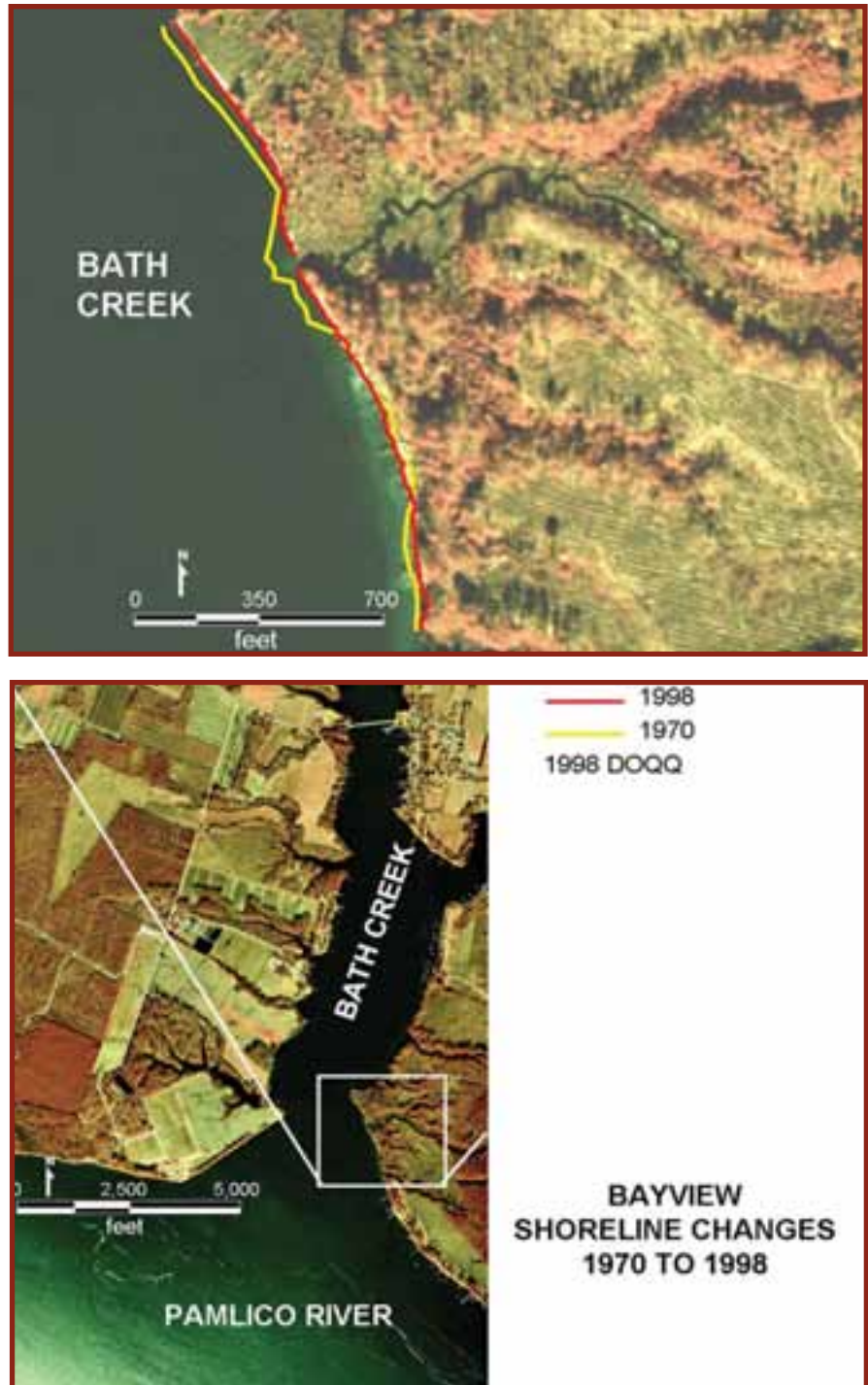
FIGURE 8-4-9. The Bayview site 1998 Digital Orthophoto Quarter Quadrangle (DOQQ) with digitized shorelines for 1970 and 1998. Notice the small drainage system that flows west off the upland to form a small cypress headland in the middle of the study area.
