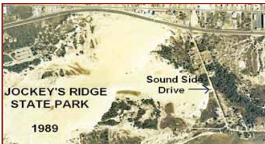
FIGURE 8-2-13. The Jockey's Ridge site aerial photograph time slices from 1962, 1971 and 1989. In 1962, the study site behind Jockey's Ridge was essentially an all active sand dune with very little vegetation. Erosion of the dune field provided the sand for an extensive strandplain beach. A large portion of the dune field along Roanoke Sound became vegetated with pine and scrub-shrub through time, as indicated on the 1971 and 1989 aerial photographs. This changed the small-scale pattern of the shoreline from a smooth curved shoreline to the present irregular shoreline with numerous vegetated headlands and coves (Fig. 8-2-11).
