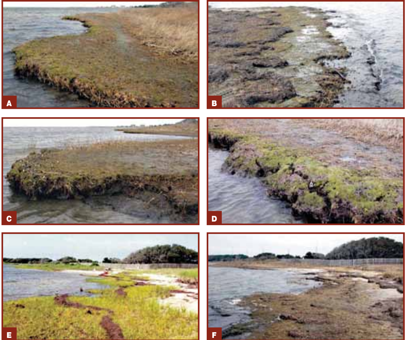
FIGURE 8-2-8. Photographs of the Salvo Day-Use site. PANEL A. Winter photograph looking north along the outer portion of the peat platform. Low wind tide has exposed the eroding wave-cut scarp in peat along the front side of the marsh platform. Notice that the outer zone is stripped of marsh vegetation by storms and is rapidly colonized by green algae. PANEL B. Winter photograph looking south along the outer portion of the peat platform during low wind tide. Notice how different layers of peat are eroded off in a stair-step fashion and the occurrence of a high water berm composed of dead submerged aquatic vegetation (SAV) with no sand. PANEL C. Close-up of the eroding marsh during a low wind tide. Notice the tough modern root mass forms a sloping overhang (on the left side of the photo) as the softer underlying peat (visible on the lower right side) is easily eroded. PANEL D. Close-up of a block of the modern, root-bound, upper peat surface as it begins to finally crack and break off. PANEL E. Summer photograph of the very narrow Spartina alterniflora marsh platform in front of a sand upland dominated by maritime forest and the Salvo cemetery. Notice the occurrence of a high-water level, thin sand berm perched on top of the marsh platform and a low water level, SAV wrack berm without any sand. Photograph is from Murphy (2002). PANEL F. Winter photograph taken at the same spot as Panel E. Notice that there are two SAV wrack berms with most of the sand gone that was associated with the upper sand berm in the previous photo. Also, the marsh grasses have been mostly stripped off the peat surface due to winter wave action.
