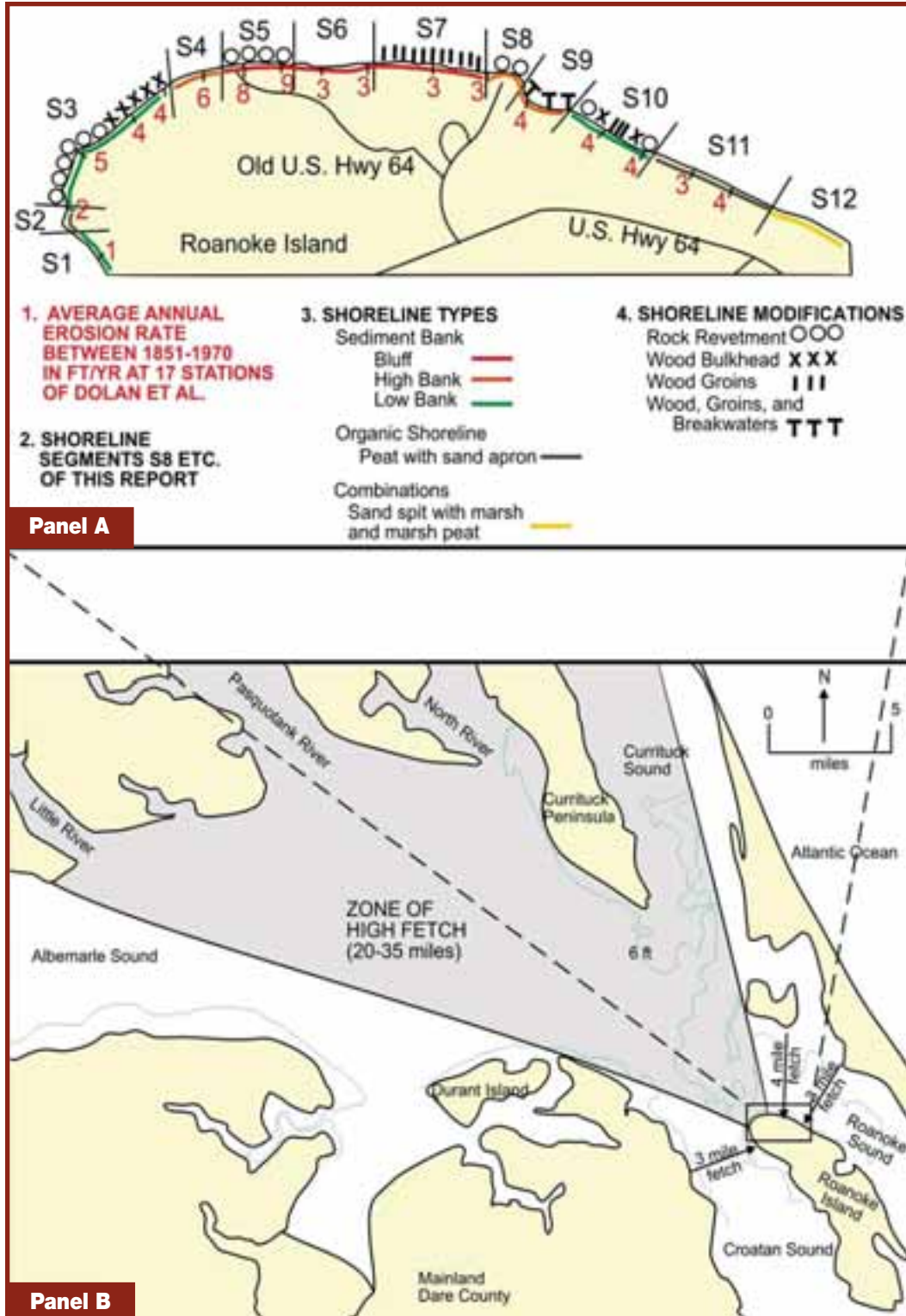
FIGURE 8-3-1. Maps of northern Roanoke Island showing the average annual estuarine shoreline erosion rates by shoreline segment, shoreline types, types and locations of shoreline erosion-control structures, and the relationship between erosion rates and distance of open water (fetch) that impact different shoreline segments. Actual erosion rates for any given shoreline segment are dependent upon the type of shoreline, in concert with the fetch and a whole series of other variables (see Chapter 5).
