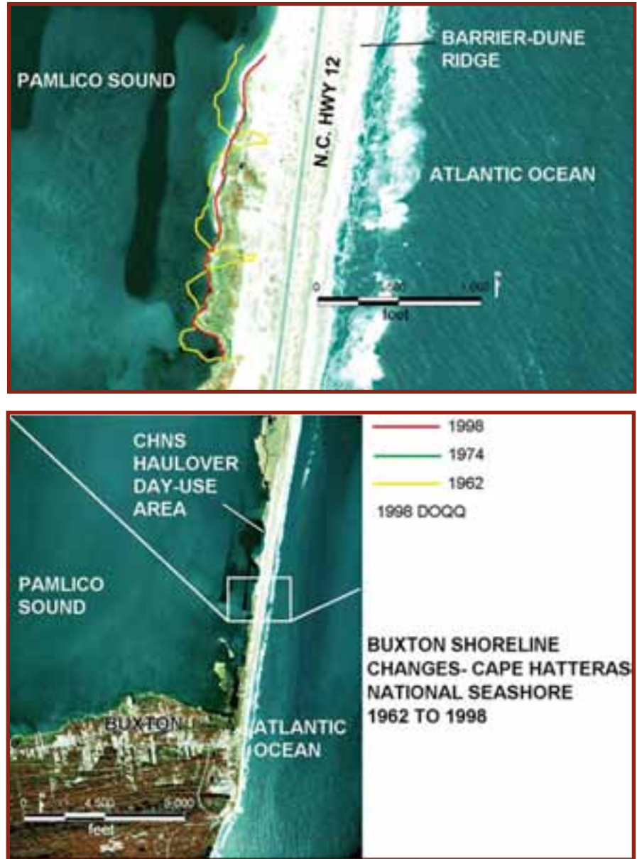
FIGURE 8-2-6. The Buxton Inlet site 1998 Digital Orthophoto Quarter Quadrangle (DOQQ), with digitized shorelines for 1962, 1974, and 1998.
