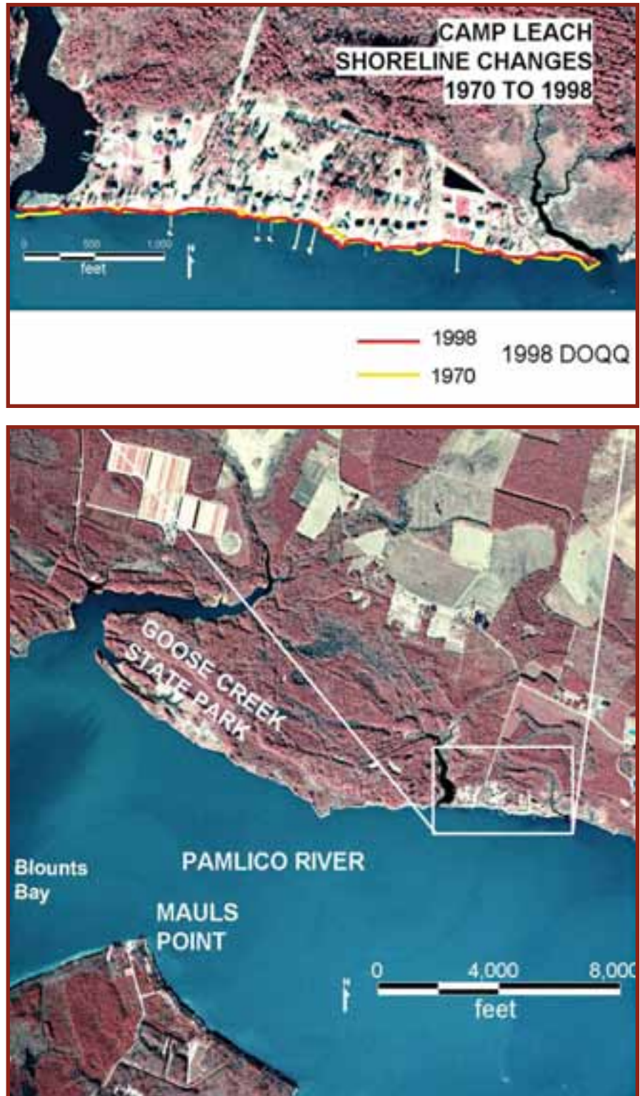
FIGURE 8-4-11. The Camp Leach site 1998 Digital Orthophoto Quarter Quadrangle (DOQQ) with digitized shorelines for 1970 and 1998.
