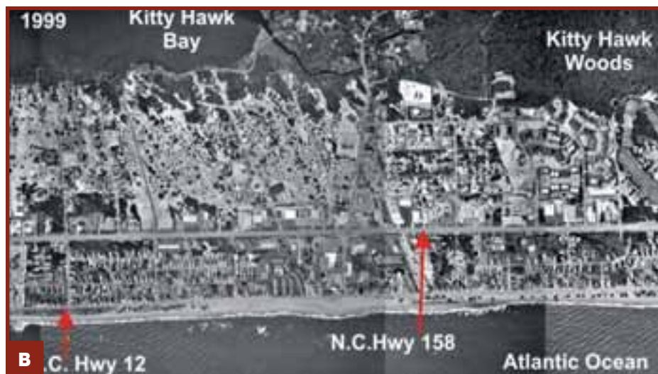
FIGURE 4-5-4. Comparison of the coastal portion of a complex barrier island (Fig. 4-5-1B) in the Kitty Hawk area using aerial photographs from 1932 and 1999. Due to the high and wide character of this complex barrier island segment, ocean processes do not influence the estuarine shoreline. Rather, it totally responds to estuarine erosion dynamics similar to the rest of the North Carolina estuarine system. PANEL A. The aerial photo of this barrier island segment just postdates the construction of N.C. Hwy. 12, but predates any shoreface modification such as construction of barrier dune ridges and most buildings. The photo was flown after a major nor'easter in 1932 and was done for the Beach Erosion Board (1935) as background data for a beach erosion study. Notice that overwash is restricted to the modern beach prism, which extends to slightly west of N.C. Hwy. 12. The limited overwash fans subsequently supply sand for development of the back-barrier dune field, which nestles up against the beach ridge system and maritime forest of Kitty Hawk Woods. The 1932 aerial photograph is from the Field Research Facility of the U.S. Army Corps of Engineers, Duck, N.C. PANEL B. This barrier island segment has been dominated by the barrier dune ridges and ever increasing urban development since the 1930s, both of which prevent oceanic overwash. The photo postdates Hurricane Dennis, which impacted this coastal segment in late August and early September 1999. Recent storm activity has totally eroded away the barrier dune ridge through most of the area, as well as eliminating many ocean front houses. The 1999 aerial photograph is from the N.C. Department of Transportation, Raleigh, N.C.
