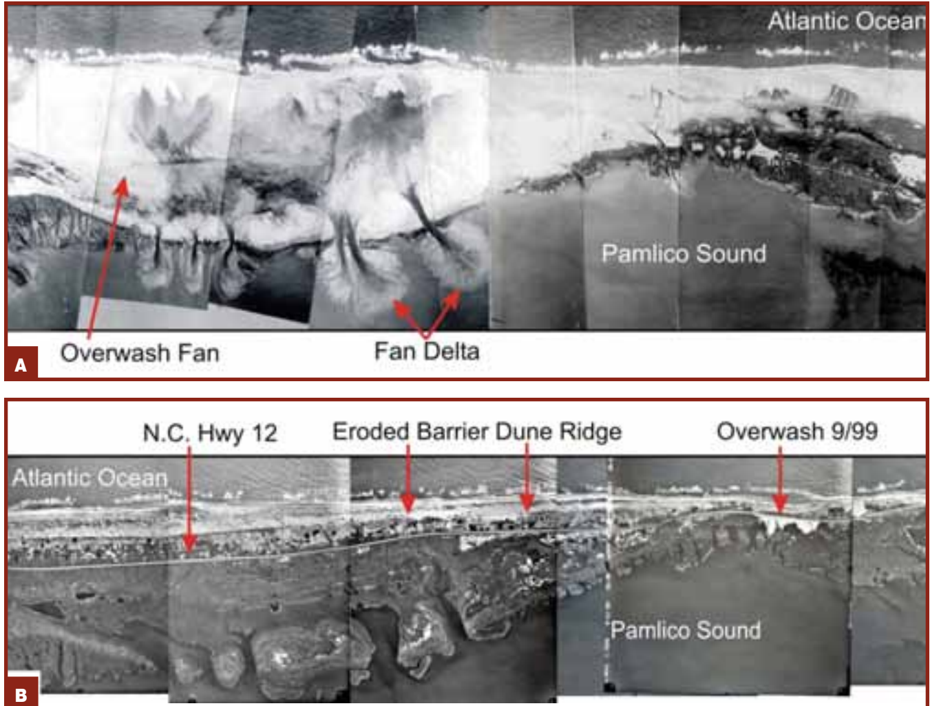
FIGURE 4-5-2. Comparison of aerial photographs from 1932 and 1999 for a portion of Pea Island immediately north of Rodanthe on the northern Outer Banks. This sediment poor barrier island segment (Fig. 4-5-1A) was dominated by overwash processes that dramatically controlled the back-barrier estuarine shoreline by depositing extensive overwash fans over the island and fan deltas into Pamlico Sound. PANEL A. The aerial photo of this barrier island segment predates any shoreface modification, such as construction of barrier dune ridges, roads, and buildings that would have inhibited the overwash process. The photos were taken after a major nor'easter in March 1932 by the Beach Erosion Board (1935) as background data for a beach erosion study. Notice the massive overwash fan that deposited beach sediment across the entire island and into Pamlico Sound. This renews the estuarine shoreline and produces broad shallow flats for subsequent growth of marsh and submerged aquatic vegetation. The 1932 aerial photographs are from the Field Research Facility of the U.S. Army Corps of Engineers, Duck, N.C. PANEL B. This barrier island segment has been dominated by extensive barrier dune ridges since the late 1930s, which minimized oceanic overwash and allowed for the extensive growth and development of a major vegetative cover. Today, the estuarine shorelines are dominated by eroding salt marsh with local and thin strandplain beaches in coves between the peat headlands. The photo post-dates Hurricane Dennis, which had a major impact upon this coastal segment in late August and early September 1999. Notice that the barrier dune ridge has been severely damaged and was totally eroded away in a few areas, allowing for small overwash fans to develop. However, only in a few areas did overwash cover the roads and in no place did it get back to the estuarine shoreline to naturally renourish the back-barrier beach. To what extent have our changes to barrier island dynamics accentuated the rate of back-barrier estuarine shoreline erosion? The 1999 aerial photographs are from the N.C. Department of Transportation, Raleigh, N.C.
