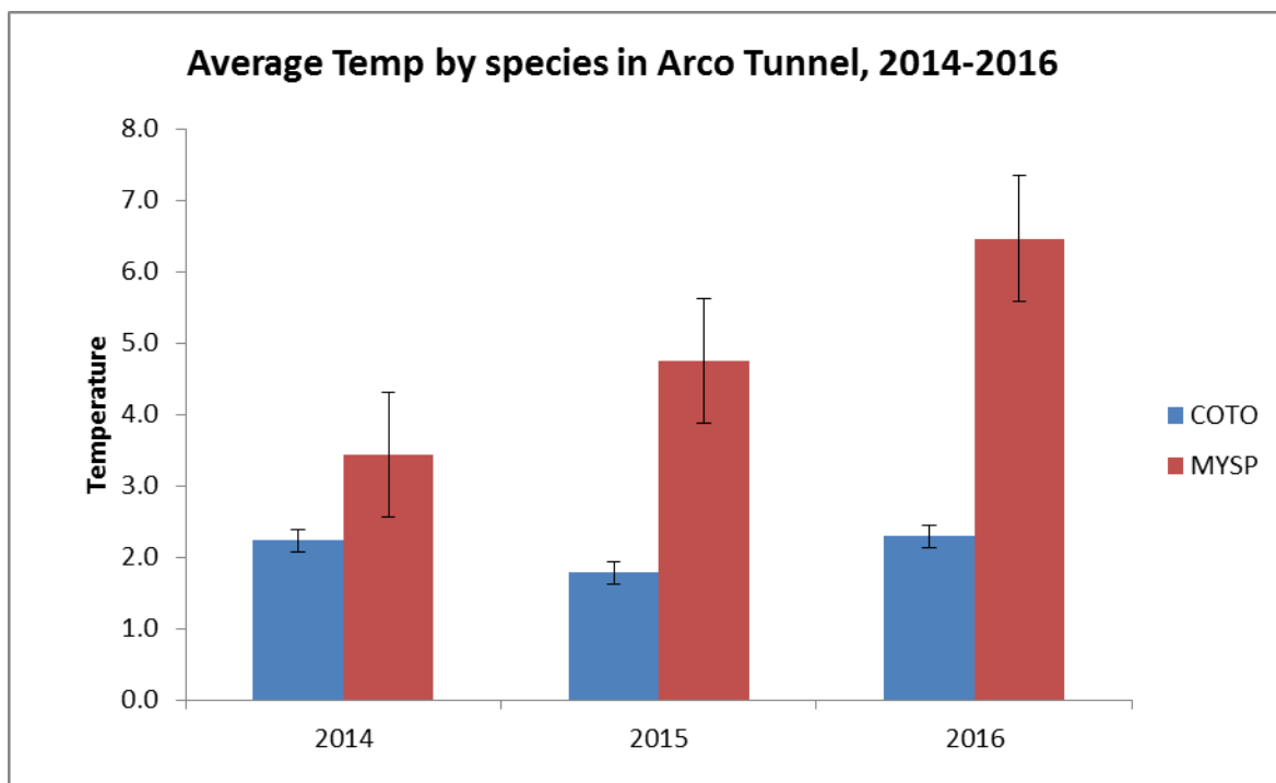
Figure 4. Average temperature and standard deviation in the immediate space of hibernating bats by species from 2014-2016.
