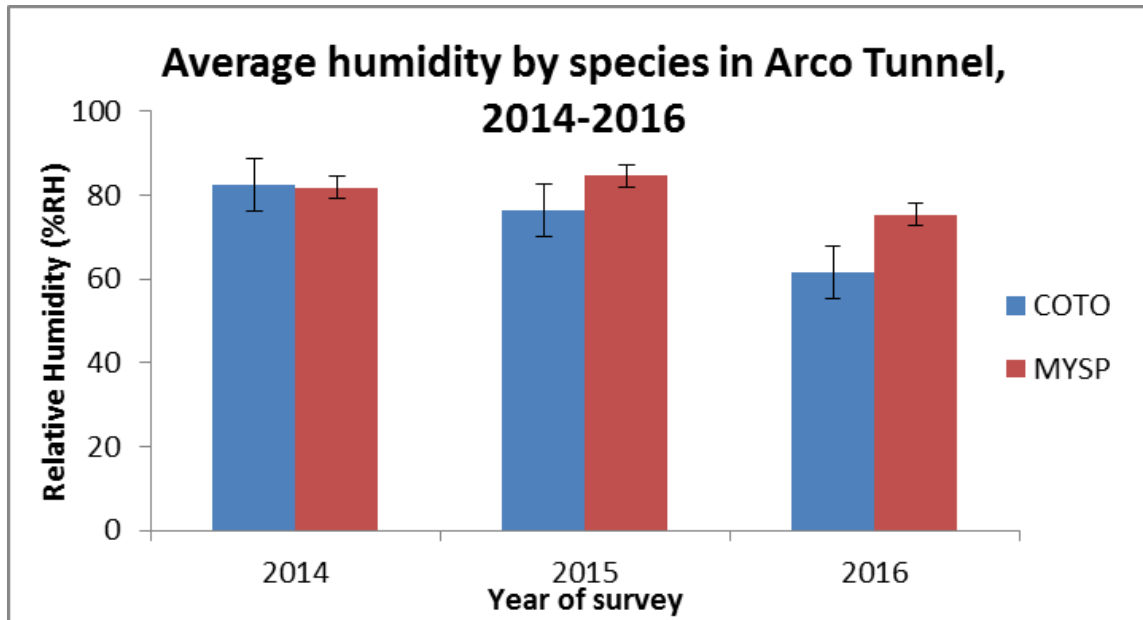
Figure 3. Average humidity and standard deviation in the immediate space of hibernating bats, by species between 2014-2016.
