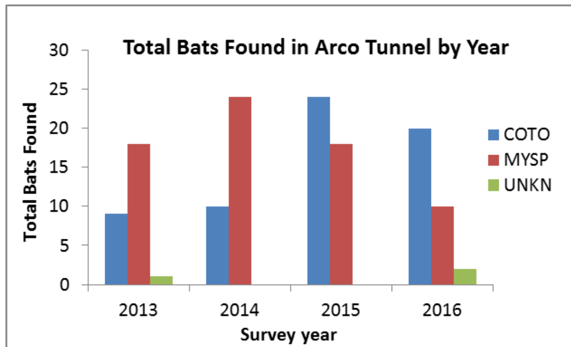
Figure 2. Total number of bats found in Arco Tunnel by year of survey.
