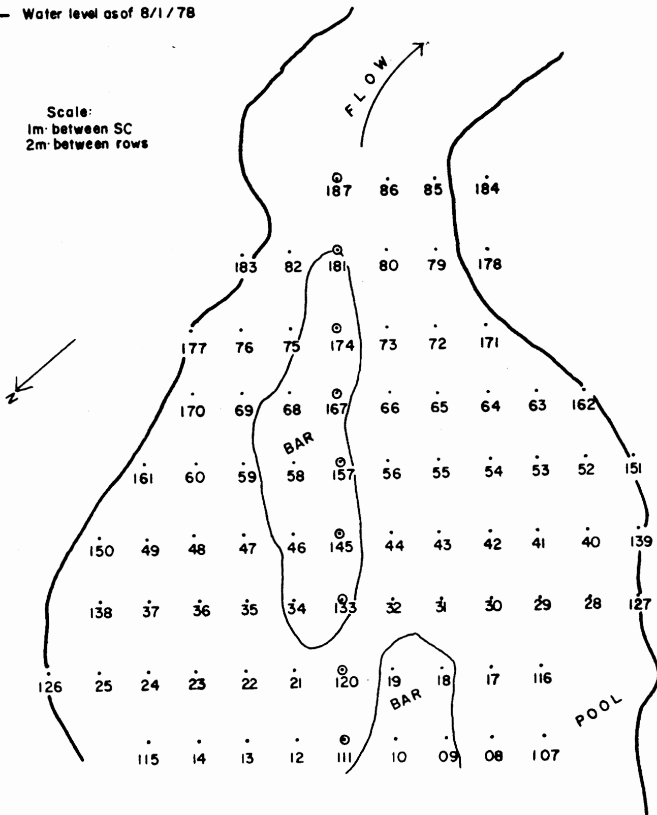
Figure 4: Scour chain array set on PC II riffle
