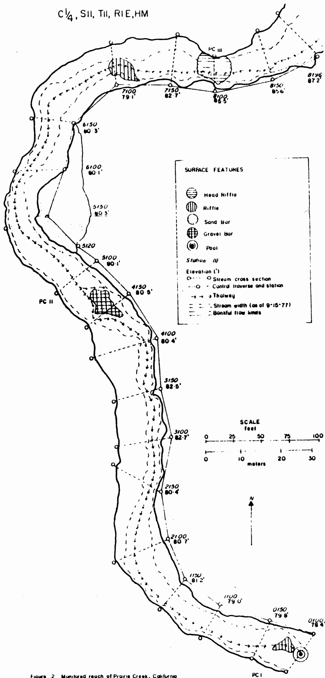
Figure 2 Monitored reach of Prairie Creek, California
