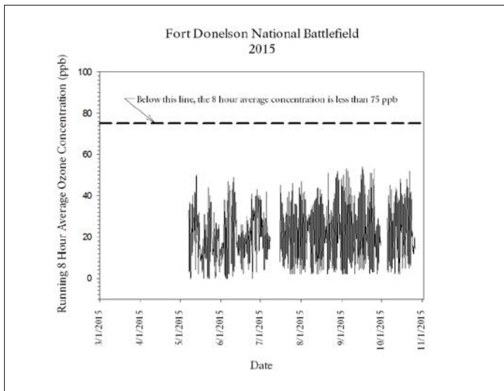
Figure 6. Running 8-hour average ozone concentration at Fort Donelson National Battlefield in 2015.
