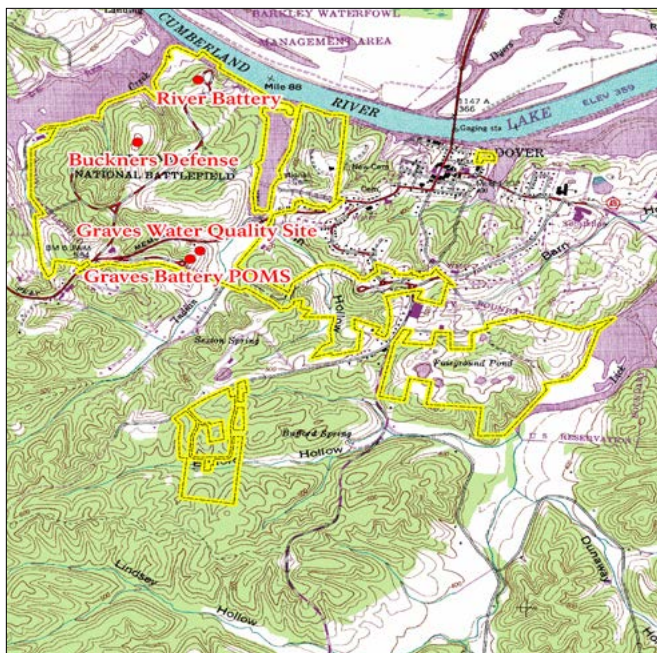
Figure 1. Map of ozone and foliar injury sites at Fort Donelson National Battlefield. NPS map by Lillian Scoggins.
