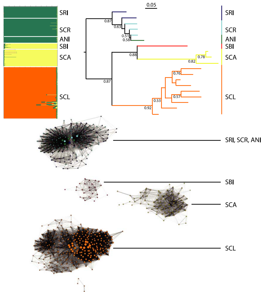
Figure 3. Results of analyses of genetic differentiation based on microsatellite allele frequencies. Top left, STRUCTURE results indicating K = 3 . Top right, neighbour-joining tree based on Nei's genetic distance; bootstrap values > 50\% are reported below branches. Bottom, EdeNetwork with automatic thresholding (0.5) based on allele sharing. Island abbreviations as in Table 1.
