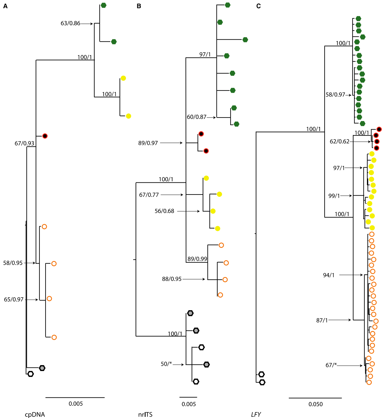
Figure 2. Eriogonum arborescens and E. giganteum consensus trees estimated from: A, plastid DNA with E. fasciculatum as an outgroup; B, nrITS; and C, LFY data, with duplicate sequences removed. Garli ML bootstrap support values above and MrBayes posterior probabilities below selected branches are shown. Taxon symbols as in Fig. 1. *Posterior probability < 0.50.
