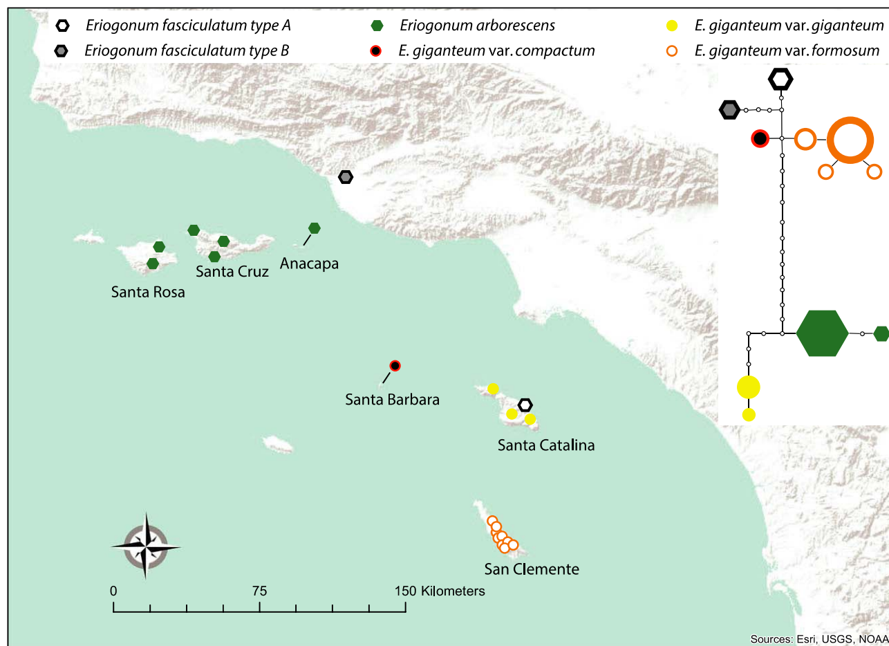
Figure 1. Plastid haplotype network (symbol size proportional to the number of copies recovered; inferred changes indicated by small black circle) and approximate locations of the California Channel Islands and sampled Eriogonum populations: Eriogonum arborescens (solid hexagons: Anacapa, Santa Cruz and Santa Rosa Islands), E. giganteum var. giganteum (solid circles: Santa Catalina Island), E. giganteum var. compactum (filled circle: Santa Barbara Island), E. giganteum var. formosum (open circles: San Clemente Island) and E. fasciculatum (open and filled hexagons, Santa Catalina Island and mainland California).
